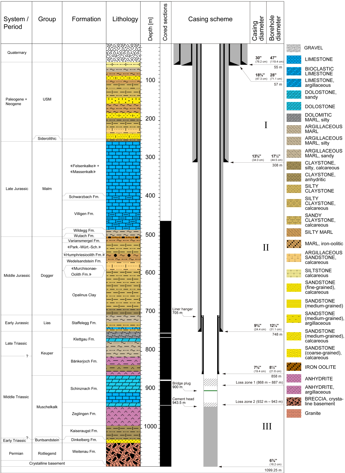
Fig. 1-3: Lithostratigraphic profile and casing scheme for the MAR1-1 borehole 3
