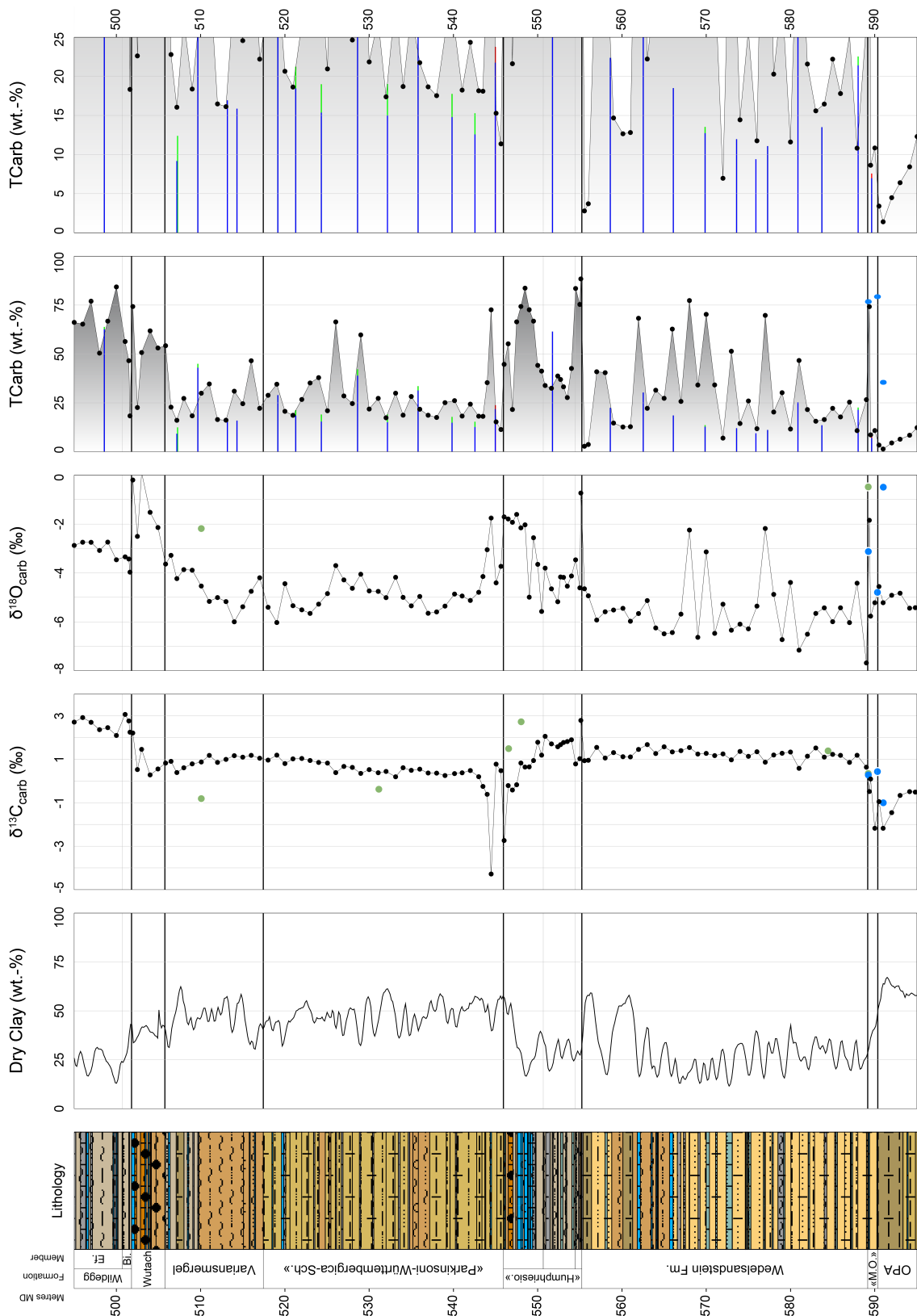
Fig. 3-6: Bulk rock (carbonate) isotopic data from the upper part of the Dogger Group Geochemical data from 594.13 – 495.00 m, additional explanations and references see text at the beginning of Section 3.4.
