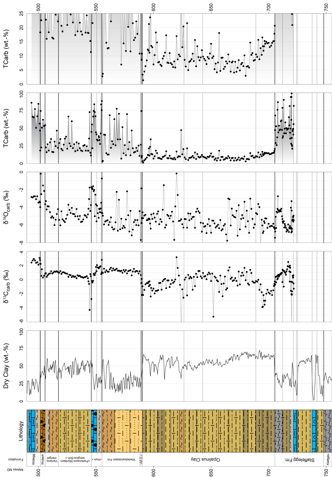
Fig. 3-8: Whole bulk rock (carbonate) isotopic data from MAR1-1
