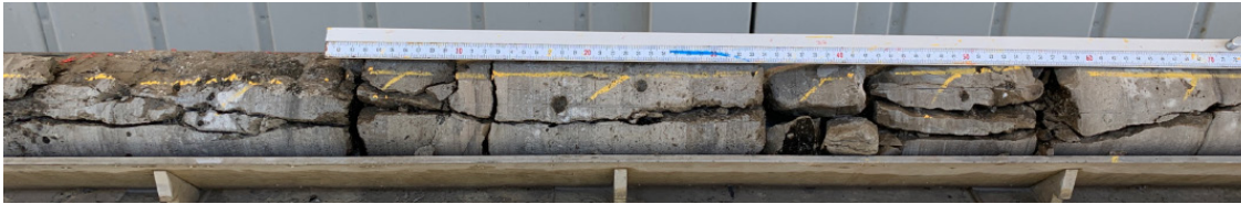
Fig. 3-9: Core picture of the vertical fracture in first encountered loss zone
