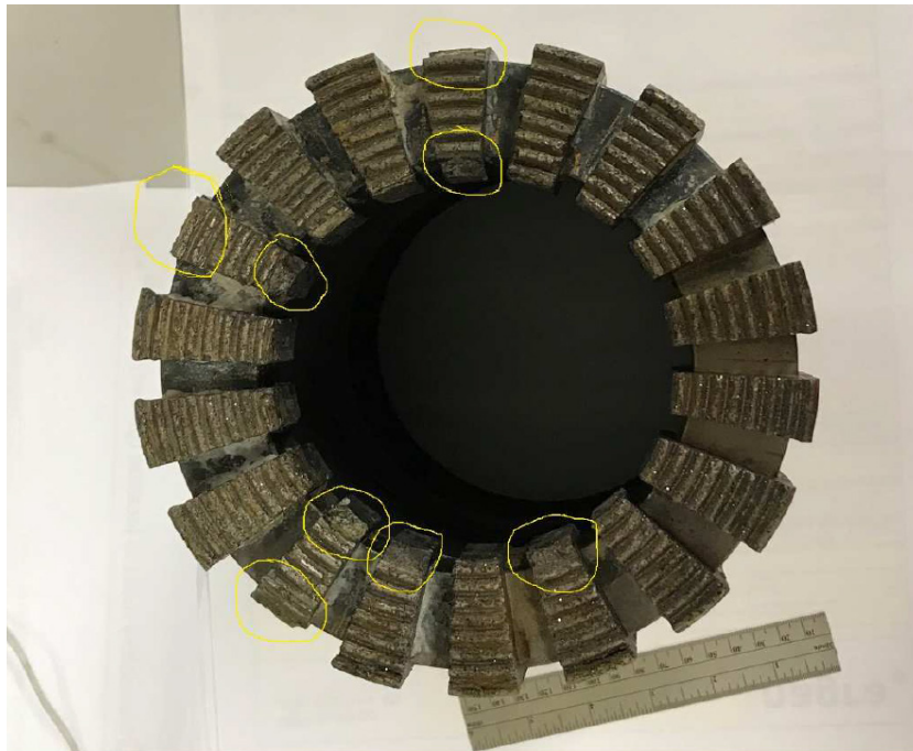
Fig. 3-6: Impregnated core bit after POOH from a depth of 503 m MD
