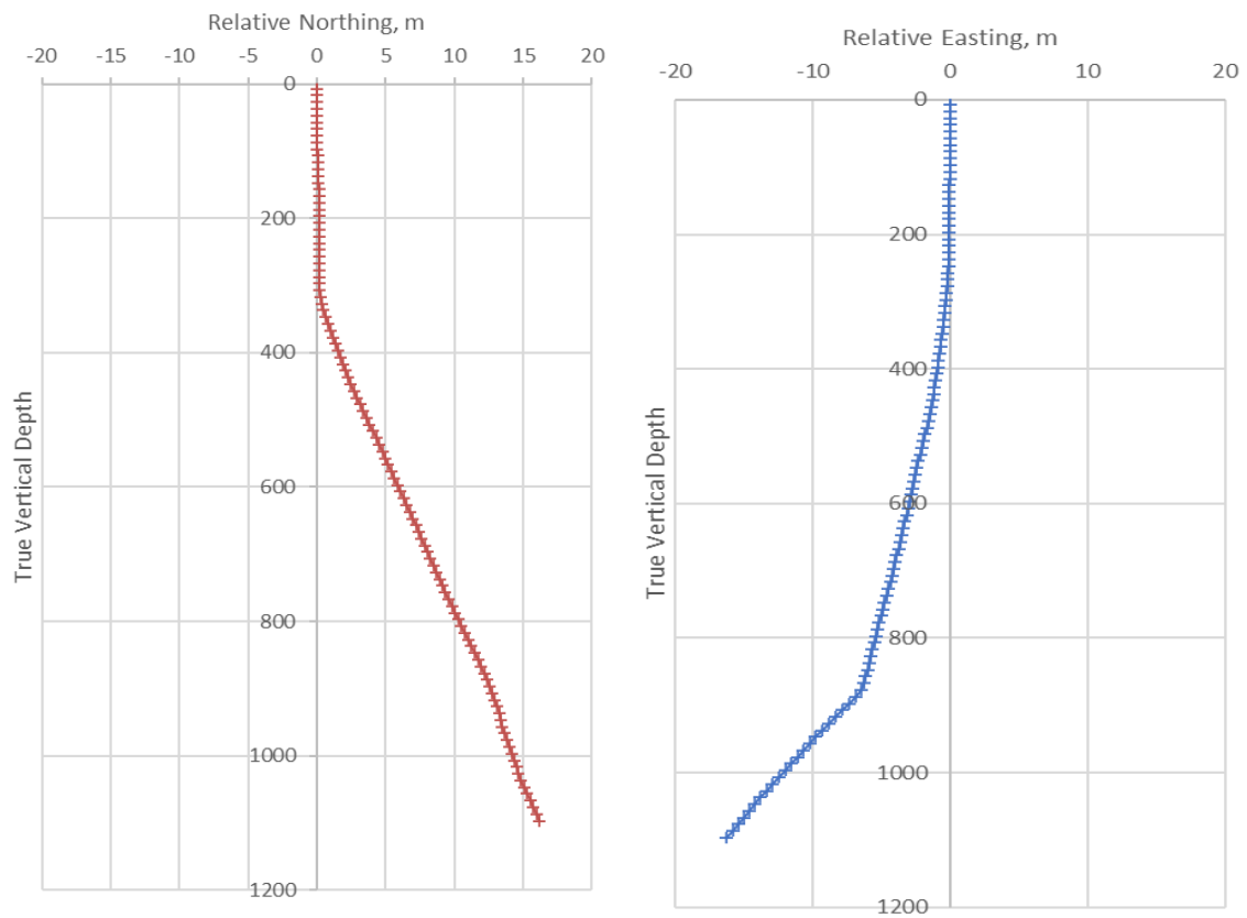
Fig. 3-16: Profile view: relative northing and relative easting – relative elevation (TVD)
