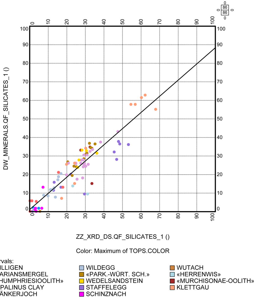
Fig. 4-4: Weight-% of QF-silicates (y-axis) compared to core XRD data (x-axis), Villigen to Schinznach Formation
