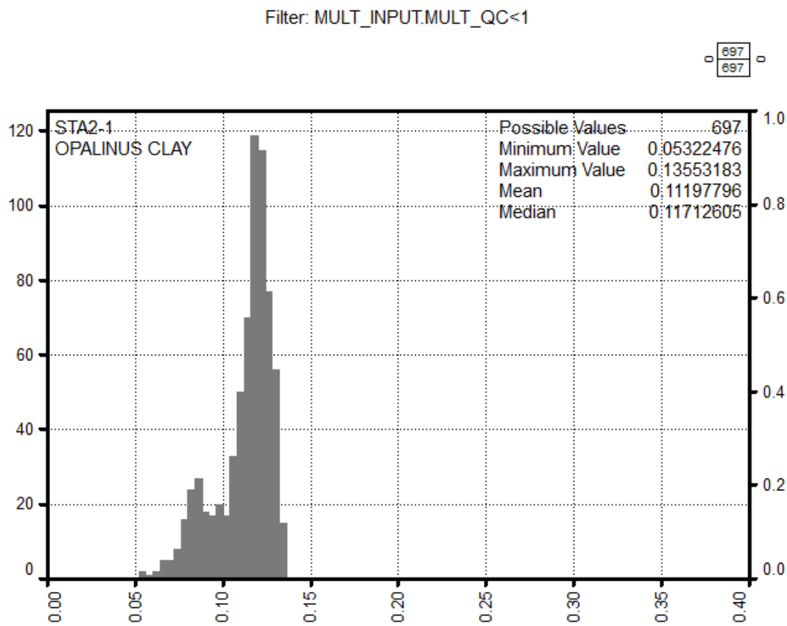
Fig. 4-14: Total porosity frequency histogram in the Opalinus Clay X-axis is the total porosity v/v from MultiMin, y-axis the number of points per bin (100 bins).
