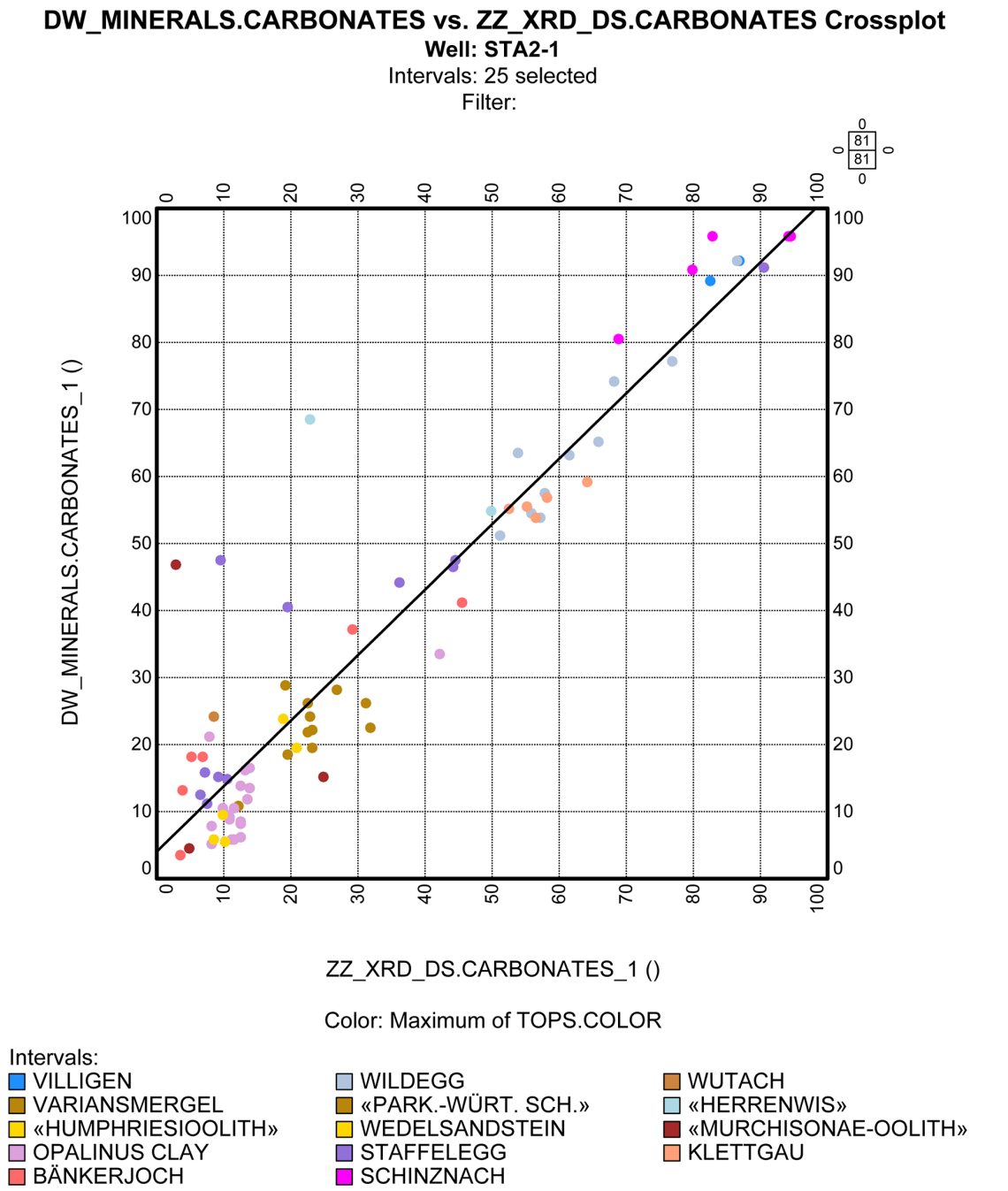
Fig. 4-5: Weight-% of carbonates (y-axis) compared to core XRD data (x-axis), Villigen to Schinznach Formation The carbonates include the calcite, dolomite and siderite content. The calibration to core XRD data is good ( cc = 0.94 ), despite a few outliers and local heterogeneities.
