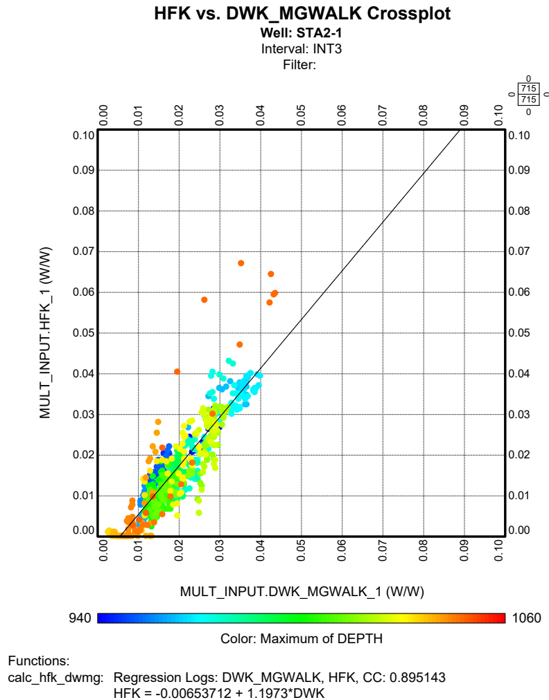
Fig. 2-2: HNGS HFK versus ECS DWK_ALKNA in INT3
