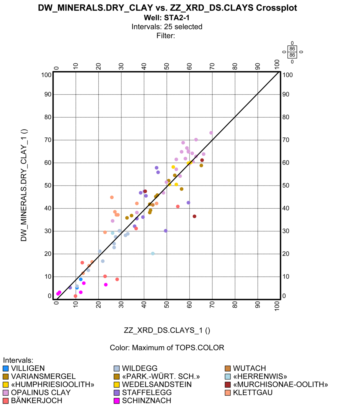
Fig. 4-1: Weight-% of dry clay (y-axis) compared to core XRD data (x-axis), Villigen to Schinznach Formation) The MultiMin dry clay content is well correlated to the core XRD data (cc = 0.92).
