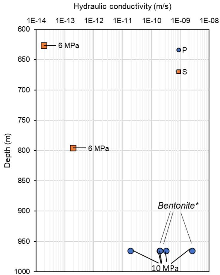
Fig. 6-19: Hydraulic conductivity versus depth
