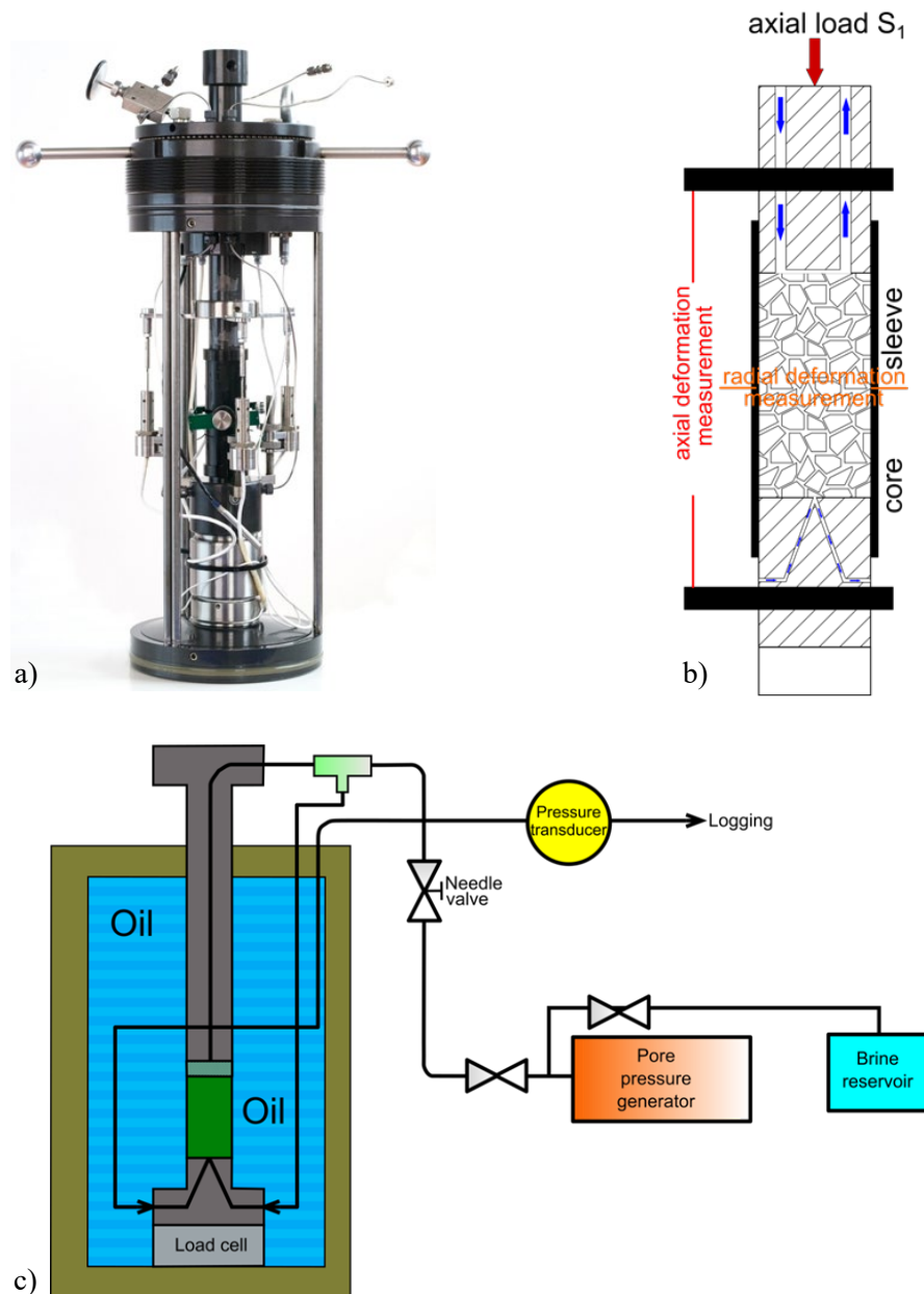
Fig. 4-4: Triaxial testing configuration used for rock-mechanical testing
