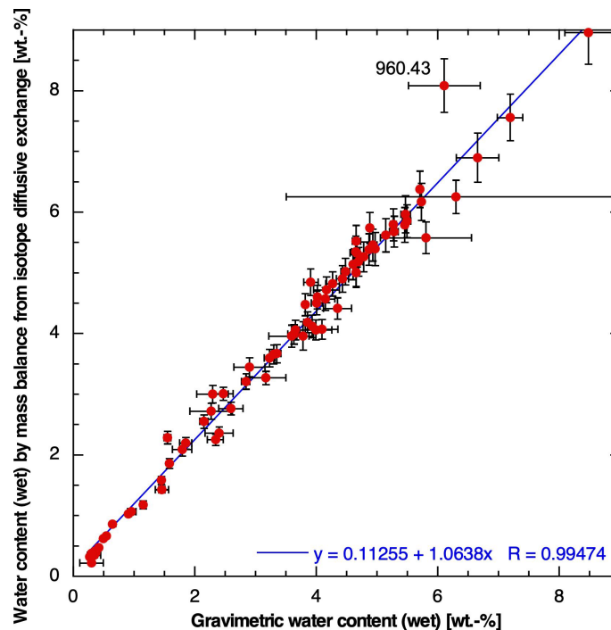
Fig. 4.3-2: Correlation of water contents based on gravimetry and on isotope diffusive exchange Black bars of gravimetric water content indicate 1\sigma variability among 2 aliquots of the same sample. Black bars for water content from isotope diffusive exchange represent the propagated analytical error. Note that only the 2 gravimetric water contents obtained from the aliquots used for the isotope diffusive exchange experiments were considered in this graph, so the correlation refers to identical sample materials. This is particularly important for anhydrite-bearing samples, given the fact that only the anhydrite-poorest portions of such samples were used for diffusive-exchange experiments. The marked sample was not considered in the linear regression.
