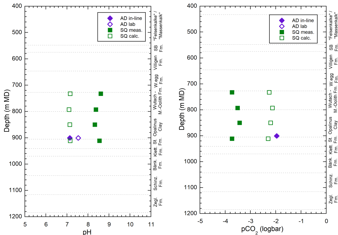
Fig. 5.5-1: pH (left) and p\text{CO}_2 values (right) from AD and SQ (see text) Solid symbols: measured pH, p\text{CO}_2 ; calc. from measured pH and TIC Open symbols: models based on calcite equilibrium (see text)
