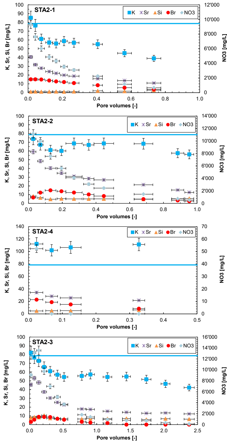
Fig. 4.7-10: Evolution of minor components during advective displacement experiments
