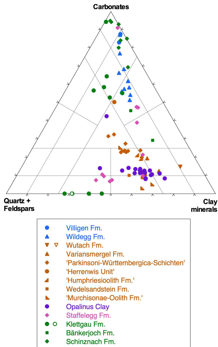
Fig. 4.2-3: Mineralogical composition of studied samples in the Füchtbauer triangle
