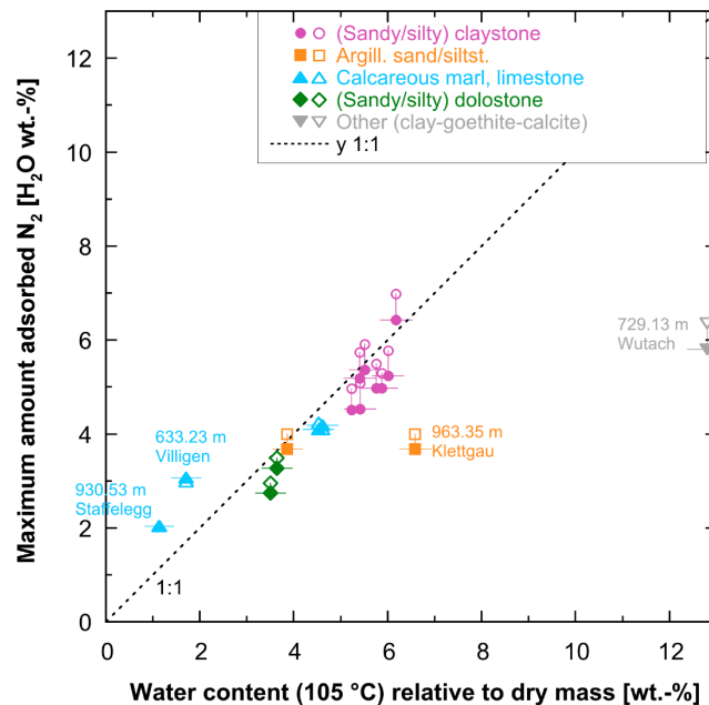
Fig. 4.3-20: Comparison of maximum amount of adsorbed N 2 (recalculated to H 2 O wt.-%) with water content per dry sample mass Open symbols: adsorption, closed symbols: desorption
