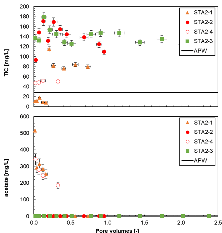
Fig. 4.7-13: Evolution of select carbon components during advective displacement experiments STA2-1 = STA2-1-778.43-AD («Humphriesioolith Fm.»); STA2-2 = STA2-1-895.02-AD (Opalinus Clay); STA2-4 = STA2-1-900.81-AD (Opalinus Clay); STA2-3 = STA2-1-923.27-AD (Staffellegg Fm.). Pore volume fractions relate to transport time based on water content. Experiment duration is 56 – 257 days. Horizontal length of symbol bar covers the sampling interval, vertical bars are an estimate of combined uncertainties. Horizontal lines represent the composition of the injected APW. Concentrations below detection (acetate) are plotted at 0; STA2-1. STA2-2, STA2-3 experiments are compromised by artefacts summarised in Section 4.7.8.
