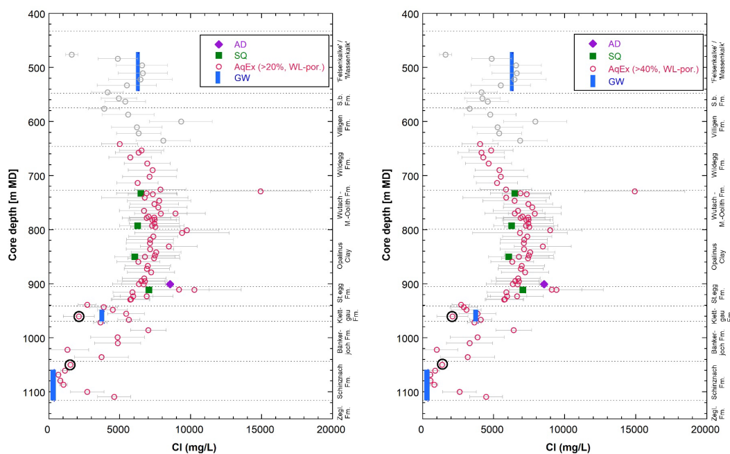
Fig. 5.2-2: Cl profile with data from squeezing, advective displacement, aqueous extraction, and groundwater samples; AqEx data recalculated from water-loss porosity assuming 20 wt.-% clay-mineral content (left) and 40 wt.-% (right) and as threshold for linear extrapolation of f_{Cl} values (see text)
