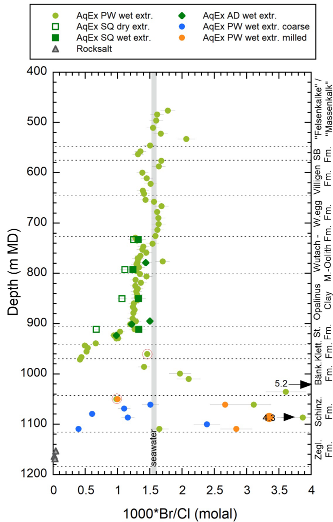
Fig. 4.4-2: Depth profile of the molar Br/Cl ratio in aqueous extracts at a S/L ratio of about 1. The samples with contamination by the drilling fluid are circled in red. The blue samples in the Schinz Formation are considered the least affected by fluid inclusions.
