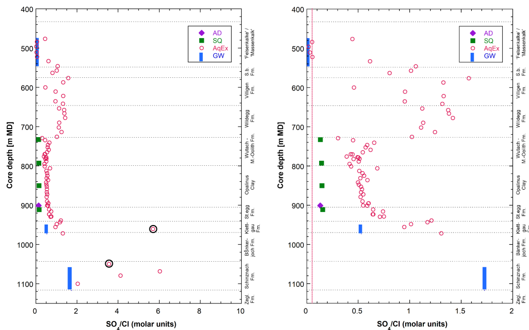
Fig. 5.3-2: Profiles showing molar \text{SO}_4/\text{Cl} ratios obtained from different methods at different scales
