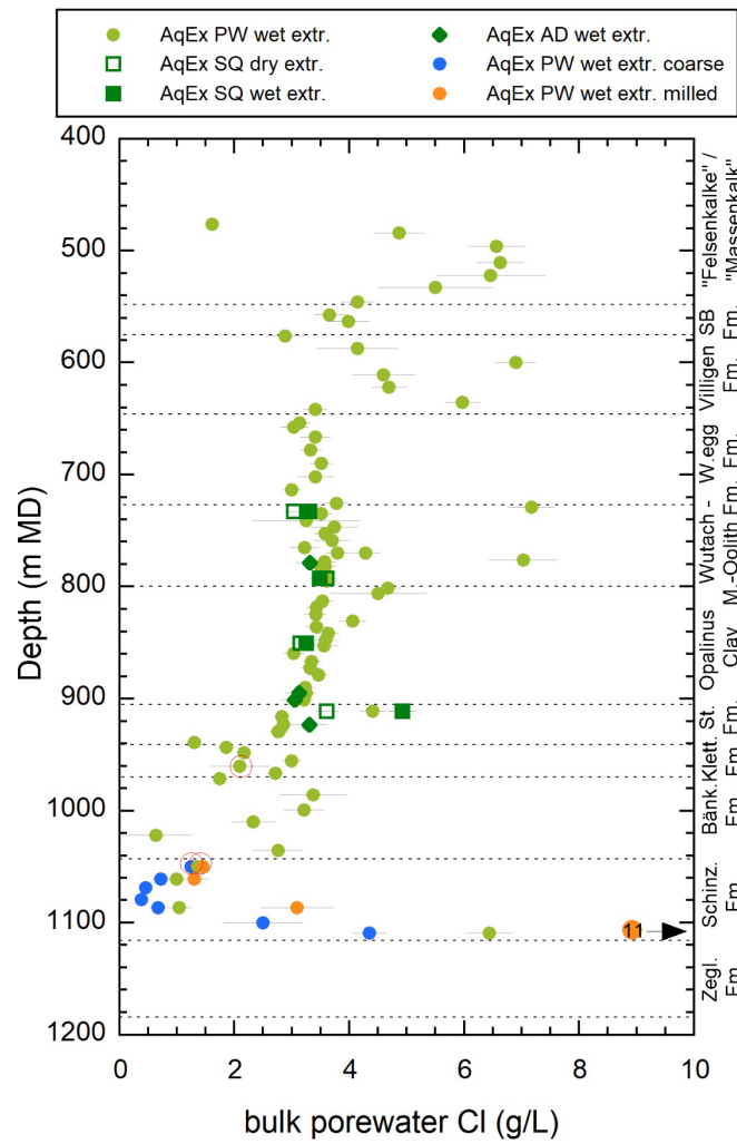
Fig. 4.4-7: Bulk porewater Cl concentrations versus depth from aqueous extracts of PW, AD and SQ samples
