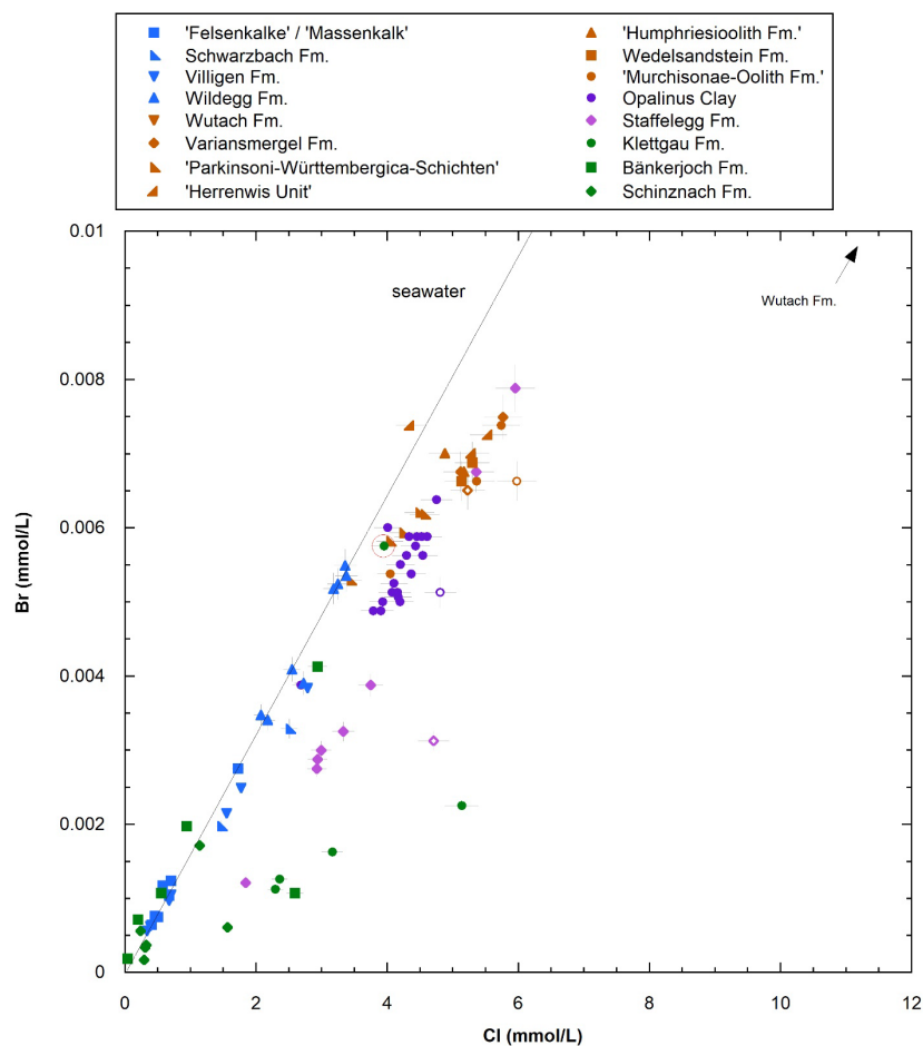
Fig. 4.4-1: Molar Br versus Cl concentrations in aqueous extracts at a S/L ratio of about 1 Empty symbols mark aqueous extracts from dry material. The sample with contamination by the drilling fluid is circled in red.
