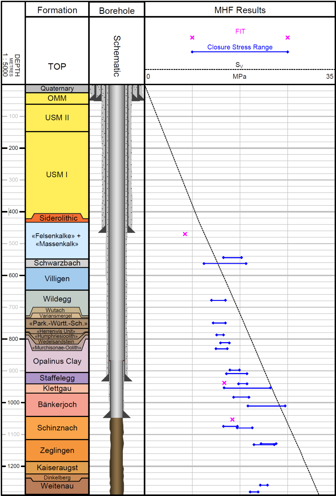
Fig. 5-3: Comparison of the quicklook closure stress range obtained from the STA2-1 MHF tests with the overburden vertical stress (S v ) from the integration of density over depth and the maximum pressures attained during the formation integrity tests (FIT)
