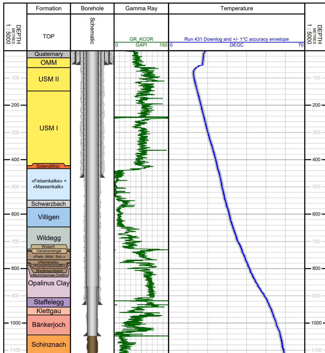
Fig. 3-9: Post-completion temperature log from the downlog pass of Run 4.3.1 (04.07.2022)
