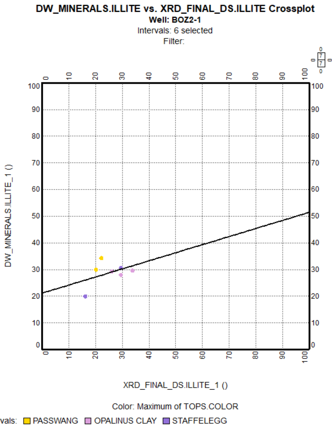
Fig. 4-3: Weight of illite (y axis) compared to core XRD data (x axis), XRD data in the Passwang to Staffelegg Formation)
