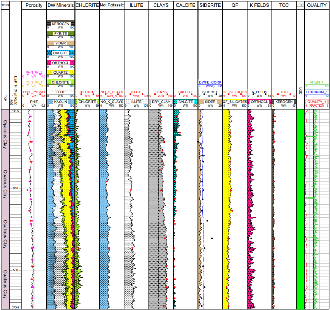
Fig. 4-14: Main log and core results in the Opalinus Clay The back line in the all clay minerals track represents a 40% baseline.
