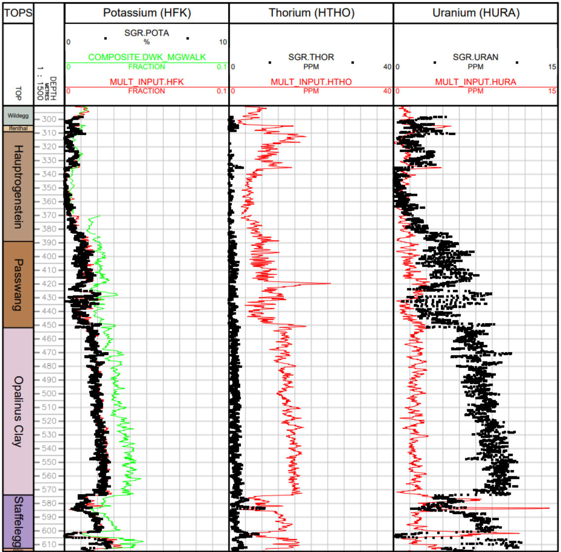
Fig. 2-3: Core (black dots: spectral gamma ray) and wireline HNGS (red curves) spectral gamma ray elements comparison
