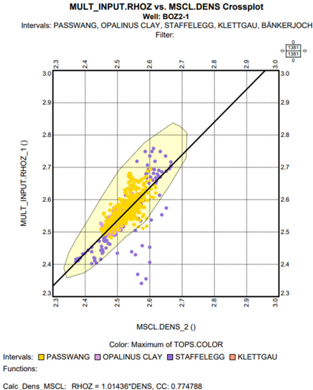
Fig. 3-3: TLD bulk density (RHOZ) versus MSCL bulk density in BOZ2-1
