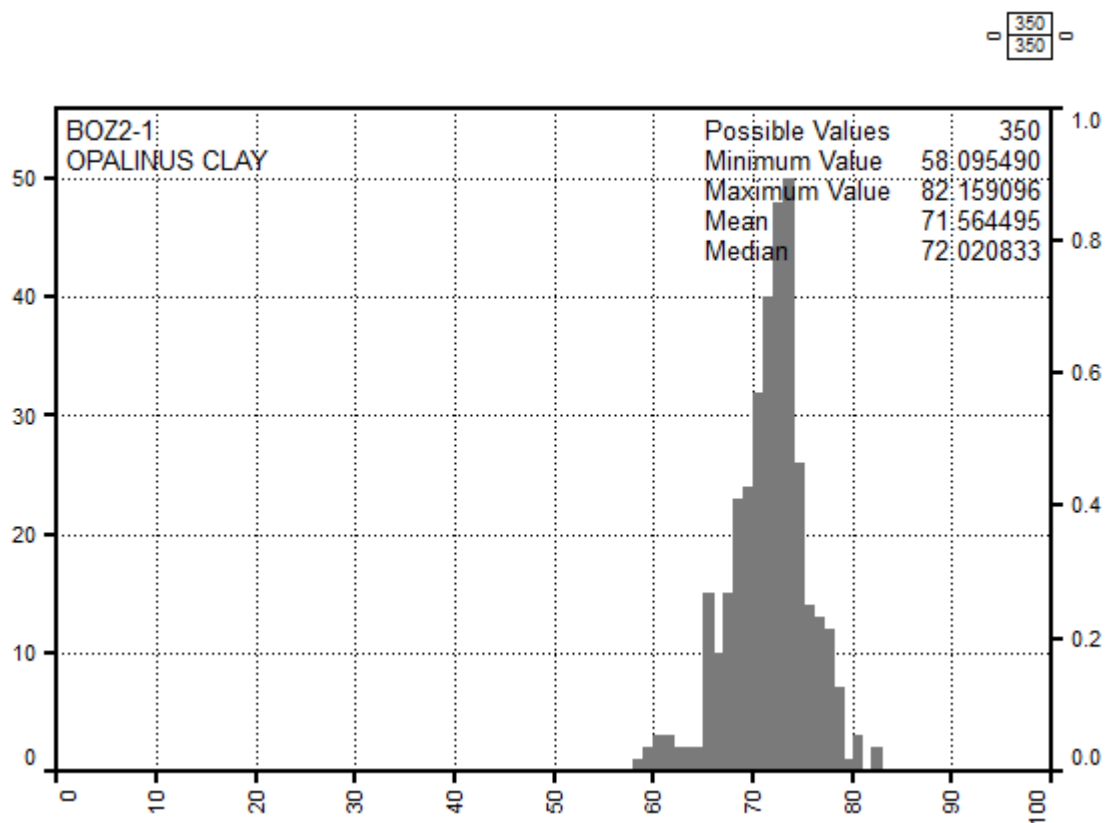
Fig. 4-9: Dry clay weight percentage frequency histogram in the lower section of the Opalinus Clay (below 520.5 m)
