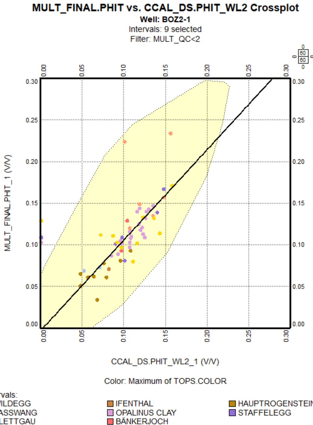
Fig. 4-6: Total porosity (v/v, y axis) compared to core data (x axis), Wildegg to Bänkerjoch Formation
