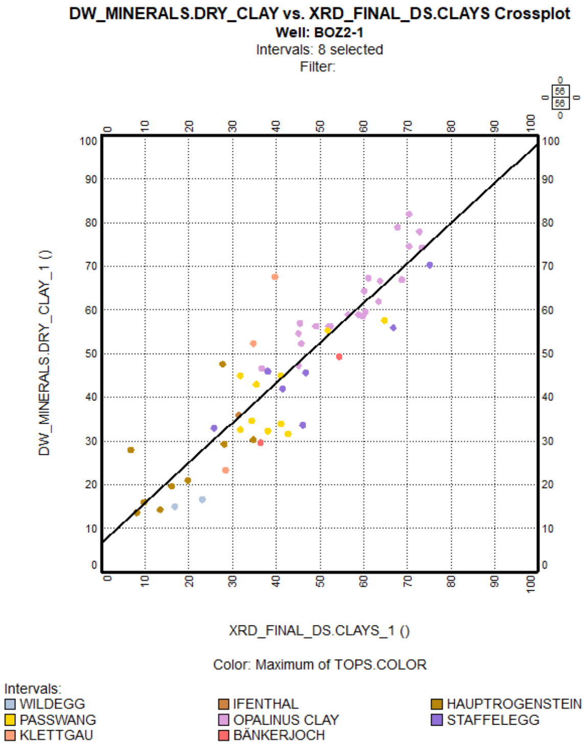
Fig. 4-1: Weight % of dry clay (y-axis) compared to core XRD data (x-axis), Wildegg to Bänkerjoch Formation The MultiMin dry clay content is well correlated to the core XRD data (cc = 0.90).
