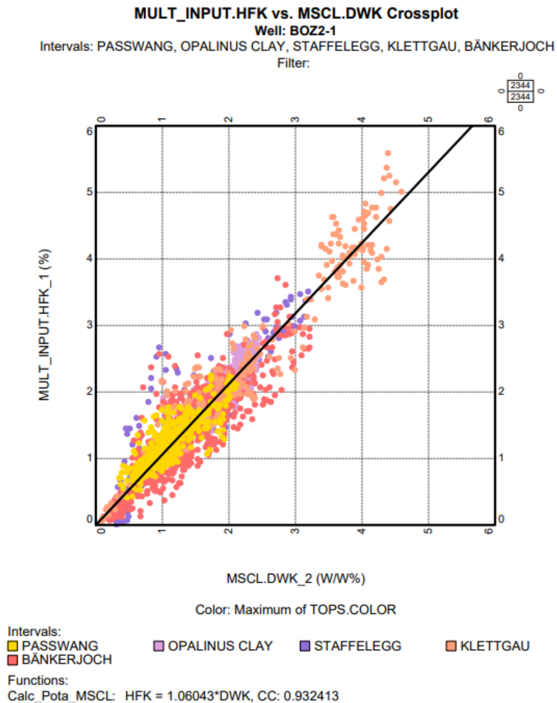
Fig. 3-1: HNGS potassium (HFK) versus MSCL potassium in BOZ2-1
