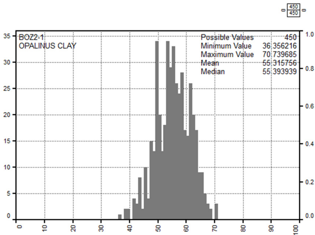
Fig. 4-8: Dry clay weight percentage frequency histogram in the upper section of the Opalinus Clay (above 520.5 m) X-axis is the dry clay wt.-% from MultiMin, y-axis the number of points per bin (100 bins).
