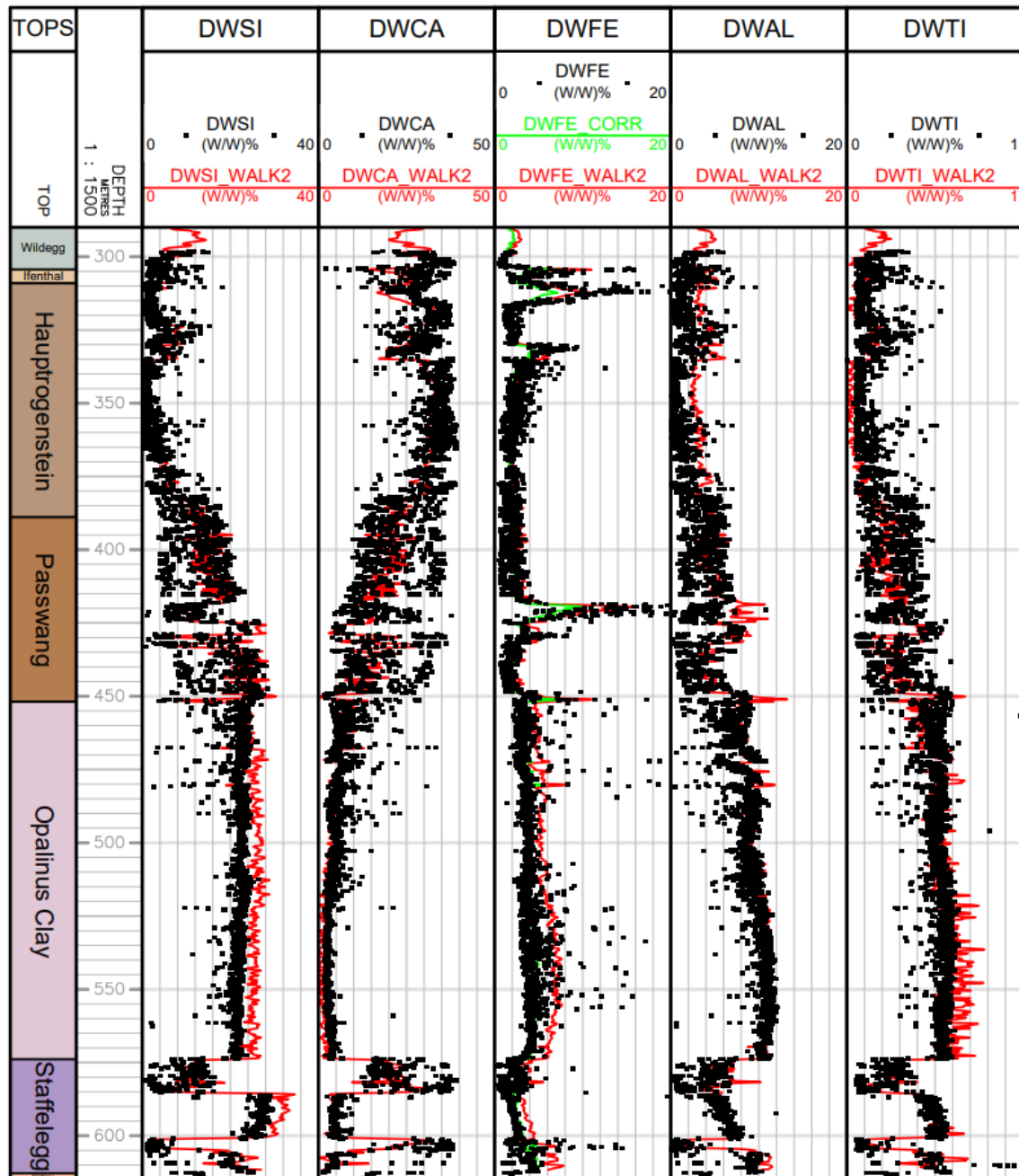
Fig. 2-2: XRF (black dots) and ECS WALK2 (red curves) elements comparison
