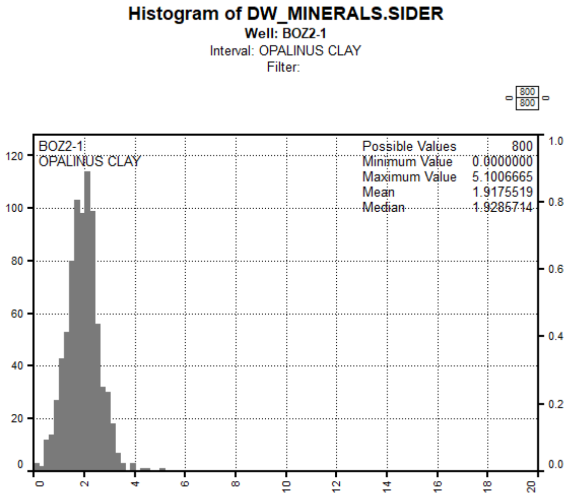
Fig. 4-11: Siderite weight percentage frequency histogram in the Opalinus Clay X-axis is the siderite wt.-% from MultiMin, y-axis the number of points per bin (100 bins).
