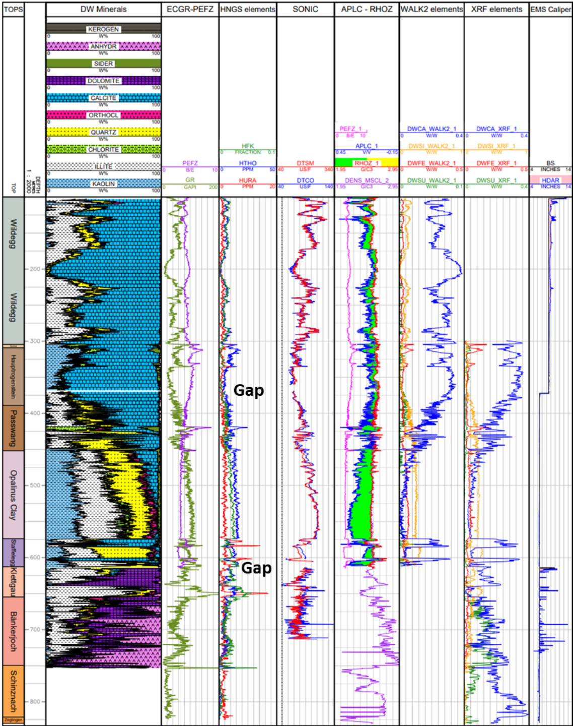
Fig. 2-1: Petrophysical log availability and gaps in the BOZ2-1 borehole Please note that ECS elements are displayed as measured (in weight/weight, 0 – 1 w/w range) and are not converted to wt.-% (weight percentage) here.
