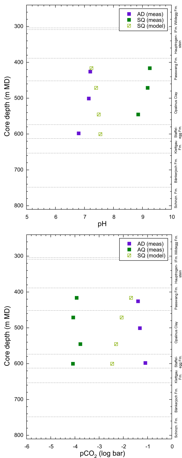
Fig. 5.5-1: pH (above) and P CO2 values (below) from AD and SQ (see text)
