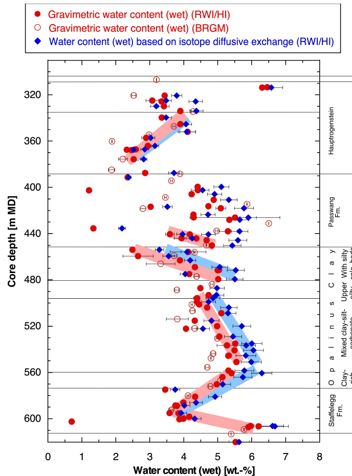
Fig. 4.3-4: Water content (wet) as a function of depth in the Lias – Dogger interval
