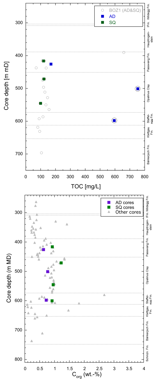
Fig. 5.5-2: TOC concentrations (above) from AD and SQ and organic carbon content in rock (below) in AD, SQ and other cores
