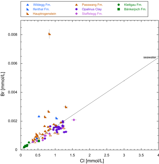
Fig. 4.4-1: Molar Br versus Cl concentrations in aqueous extracts at a S/L ratio of about 1 Open symbols mark dry aqueous extracts.
