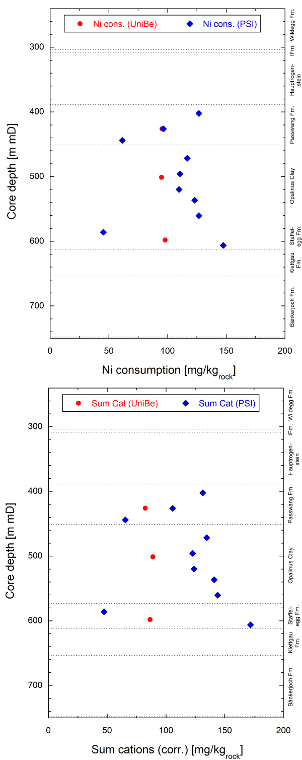
Fig. 5.6-2: Comparison of CEC data from University of Bern and from PSI; Ni consumption data (above) and corrected sum of cations data (below)
