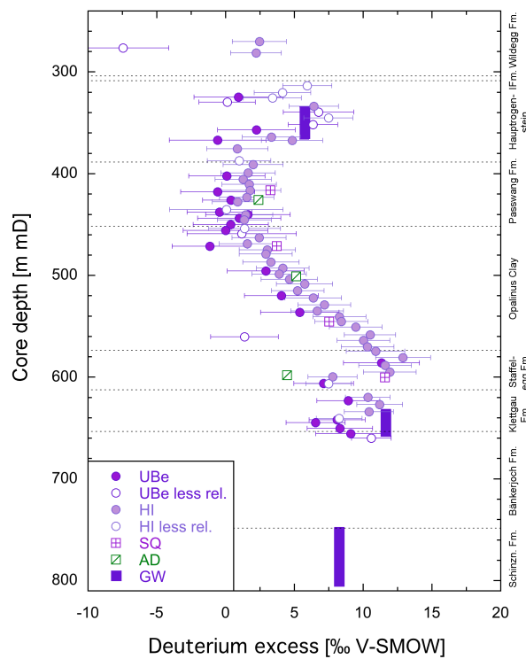
Fig. 5.7-3: Depth trends of the Deuterium excess in groundwater and porewater derived by all techniques
