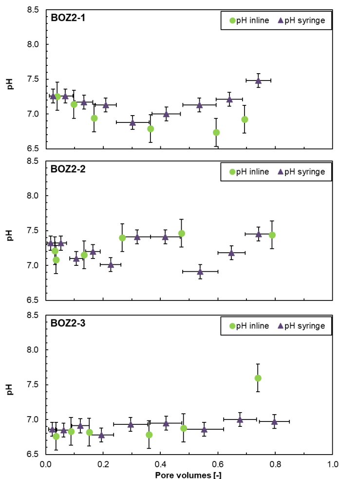
Fig. 4.7-14: Evolution of pH during advective displacement experiments
