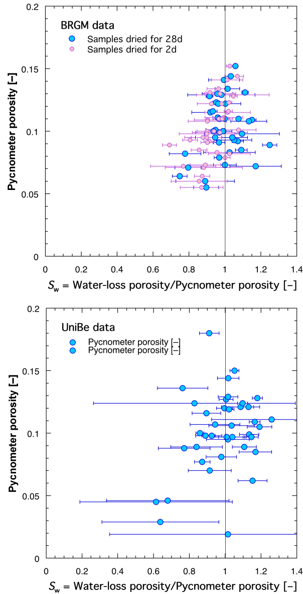
Fig. 3.4-2: Comparison of ratios of water-loss porosity (calculated from WC_{dry\ 28d} and WC_{dry\ 2d} in the case of BRGM) and pycnometer porosity obtained from measurements at BRGM and at the University of Bern
