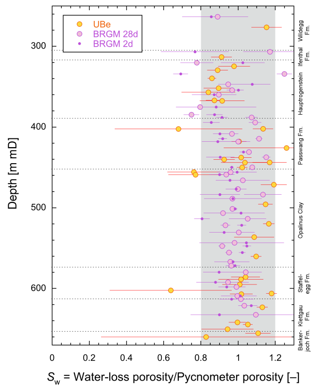
Fig. 3.4-3: Depth profile of ratios of water-loss porosity (calculated from WC_{dry\ 28d} and WC_{dry\ 2d} in the case of BRGM) and pycnometer porosity obtained from measurements at BRGM and at the University of Bern
