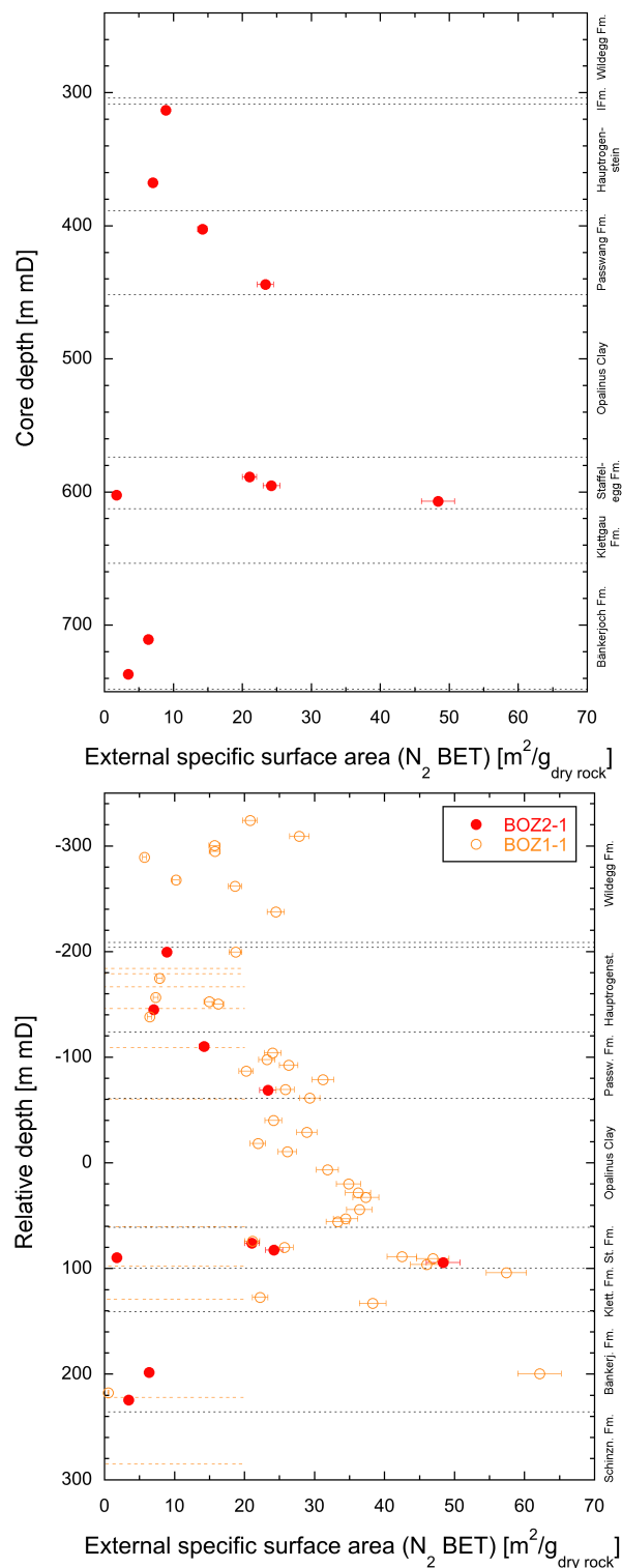
Fig. 4.3-13: Specific surface area ( S_{\text{BET}} ) derived from N 2 adsorption as a function of depth
