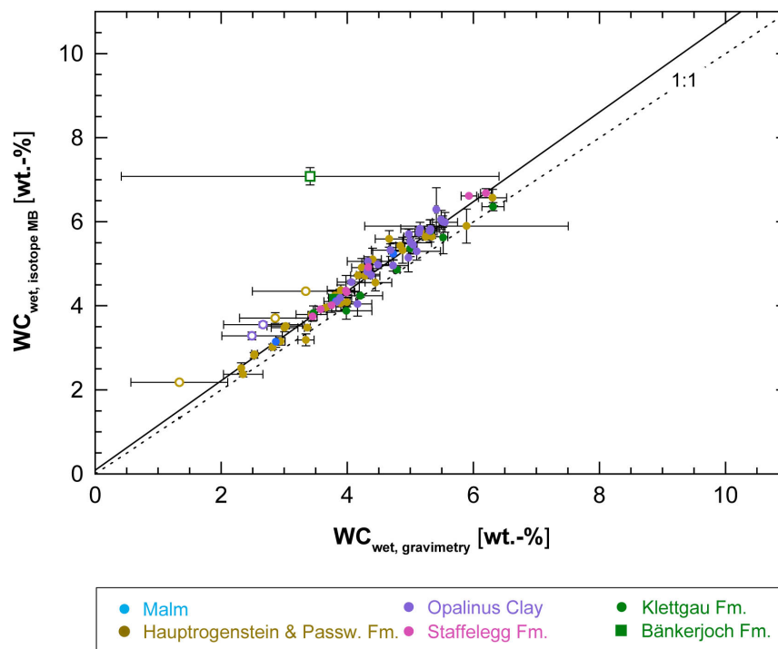
Fig. 4.8-2: Average water content obtained by water-loss at 105 °C ( WC_{\text{wet, gravimetry}} ) of subsamples LAB and NGW/ICE vs. average water content calculated from \delta^{18}\text{O} and \delta^2\text{H} mass balance from NGW/ICE diffusive-exchange experiments ( WC_{\text{wet, isotope MB}} )
