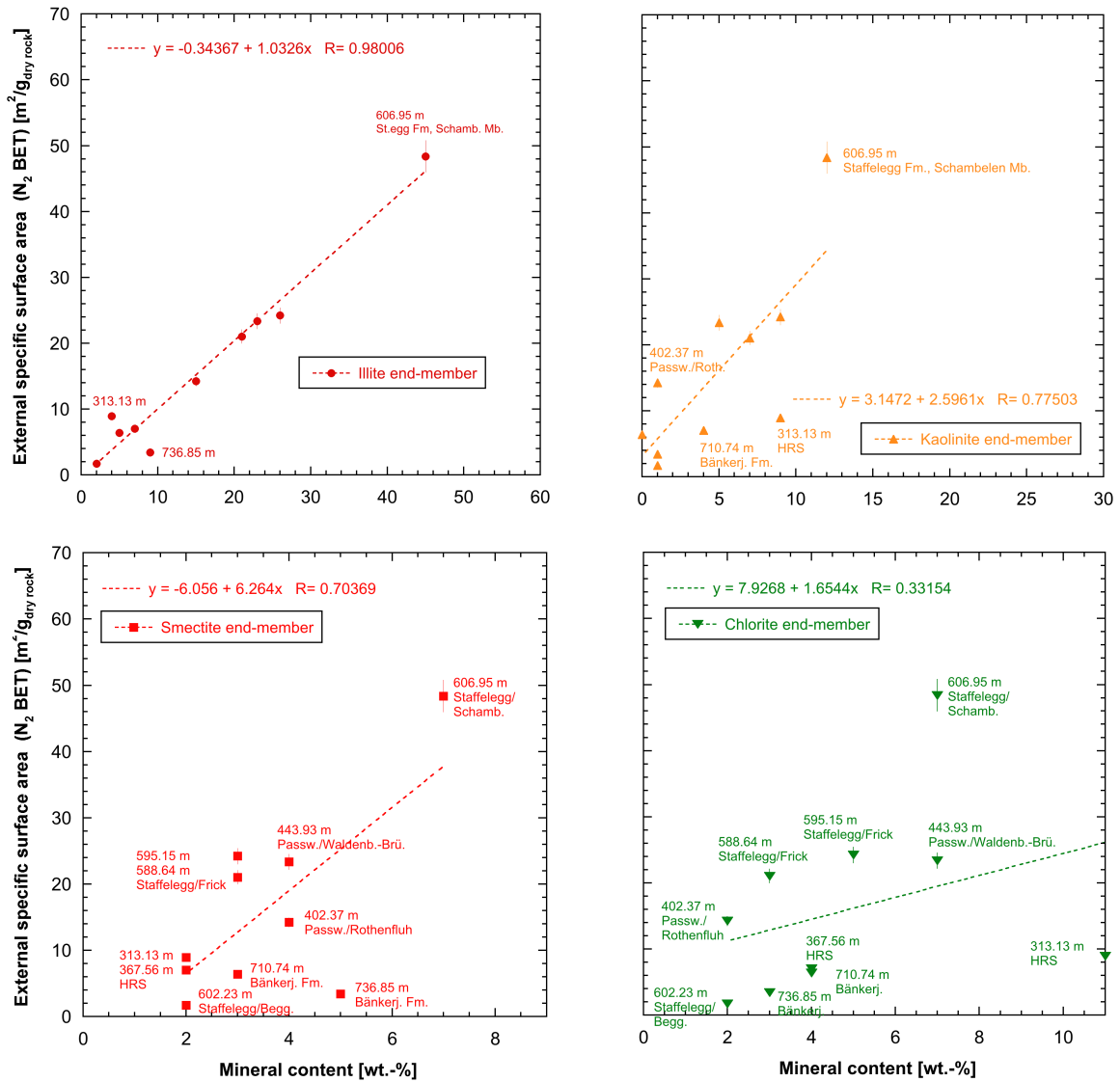
Fig. 4.3-16: Relation between external specific surface area ( S_{BET} ) derived from N_2 adsorption and contents of specific clay mineral end-members
