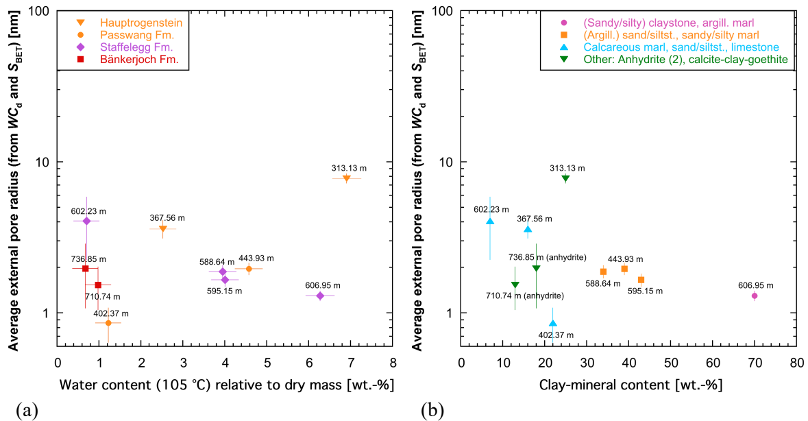
Fig. 4.3-17: Average external pore radius calculated from S_{BET} and the gravimetric water content (assuming insignificant interlayer pore volume) plotted against the gravimetric water content per dry mass of the samples (a) and against the total clay-mineral content (b)
