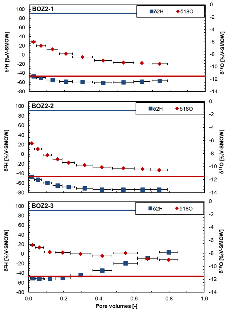
Fig. 4.7-15: Evolution of \delta^2\text{H} and \delta^{18}\text{O} during advective displacement experiments
