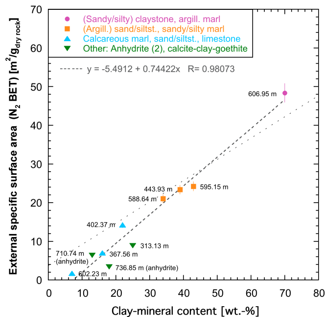
Fig. 4.3-15: Relation between external specific surface area ( S_{BET} ) derived from N_2 adsorption and content of clay minerals
