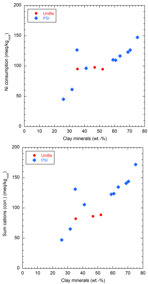
Fig. 5.6-3: CEC data as a function of the clay-mineral content; Ni consumption data (above) and corrected sum of cations (below)
