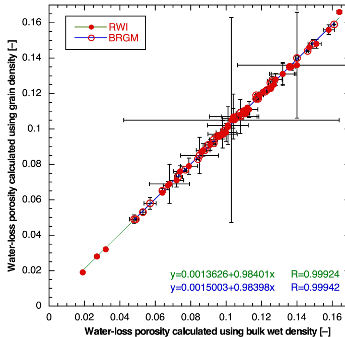
Fig. 4.3-7: Water-loss porosity calculated from gravimetric water content using either bulk wet or grain density
