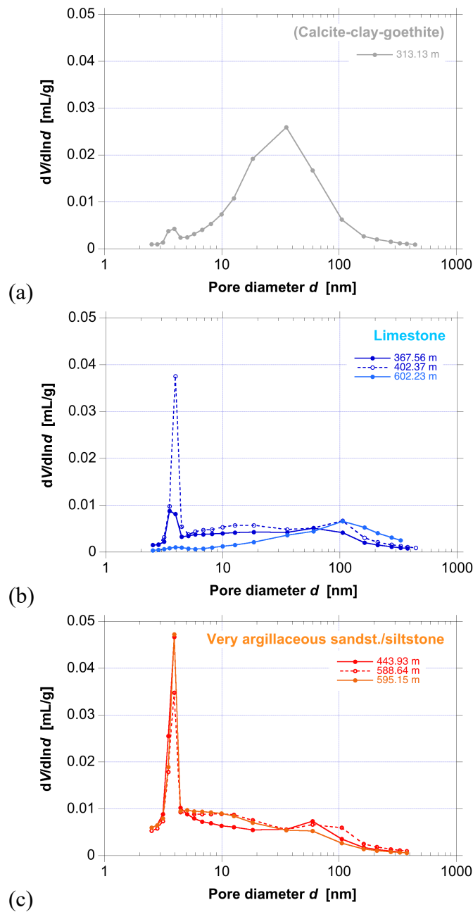
Fig. 4.3-18: Distribution of (external) pore diameters derived from N 2 desorption
