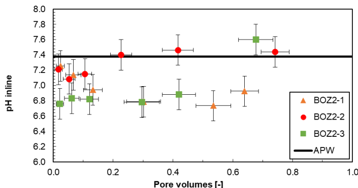
Fig. 4.7-7: Evolution of inline pH during advective displacement experiments
