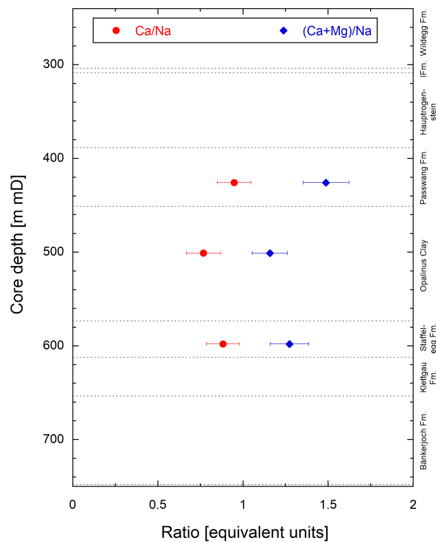
Fig. 4.5-3: Depth profiles of Ca/Na and (Ca+Mg)/Na ratios in Ni-en extracts (University of Bern data)
