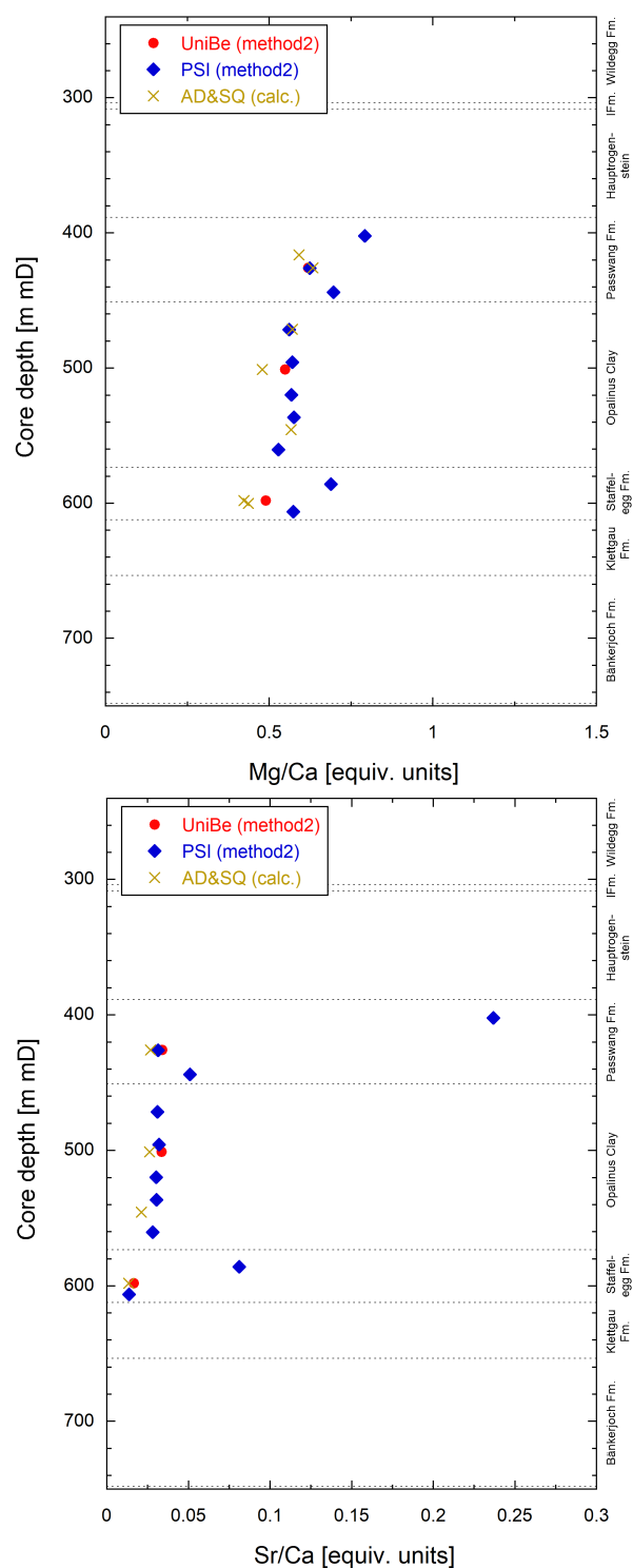
Fig. 5.6-9: Mg/Ca ratios (above) and Sr/Ca ratios (below) according to University of Bern and PSI data and "back calculated" from AD/SQ data
