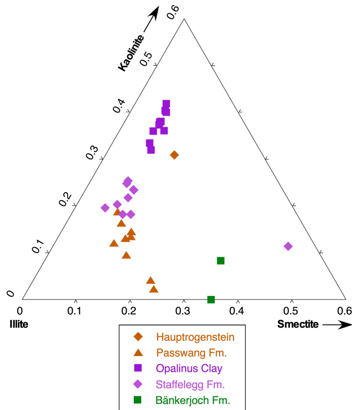
Fig. 4.2-6: Relative mass proportions of illite, smectite and kaolinite end-member clays
