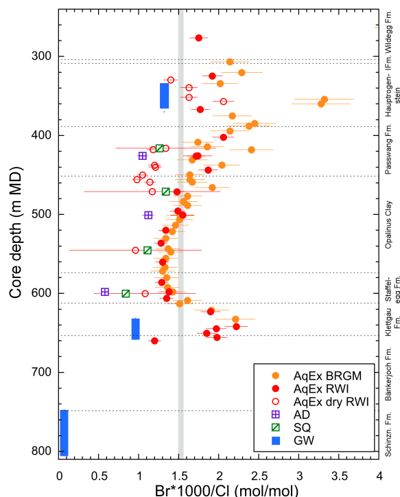
Fig. 5.2-3: 1'000 \cdot \text{Br/Cl} (molar units) profile with data from squeezing, advective displacement, aqueous extraction, and groundwater samples
