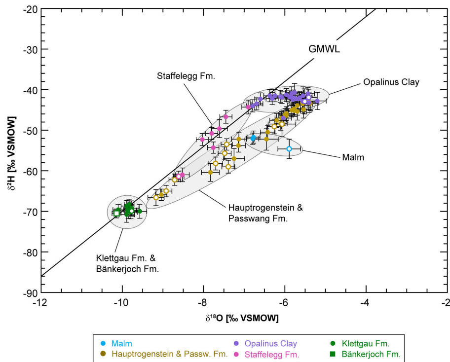
Fig. 4.8-5: \delta^2\text{H} vs. \delta^{18}\text{O} values of porewater obtained from isotope diffusive-exchange experiments
