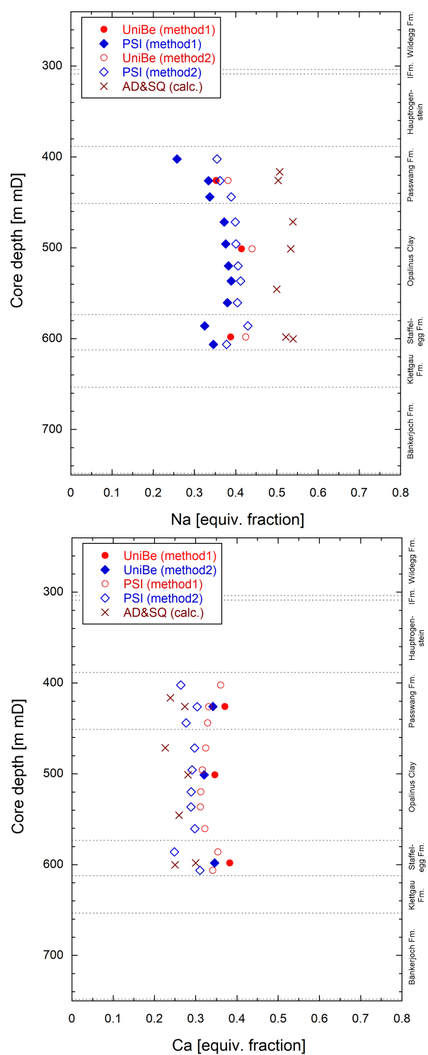
Fig. 5.6-5: Na (above) and Ca (below) occupancies according to University of Bern and PSI data and "back calculated" from AD/SQ data
