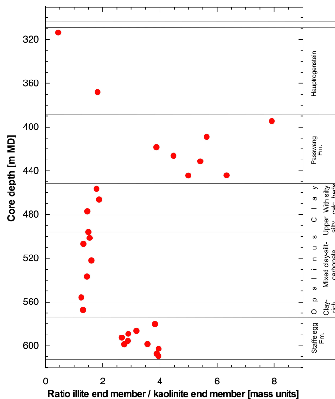
Fig. 4.2-8: Ratio of the illite to kaolinite end-member clays as a function of depth
