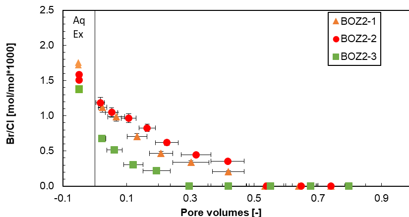
Fig. 4.7-18: Breakthrough of Cl/Br during advective displacement experiments
