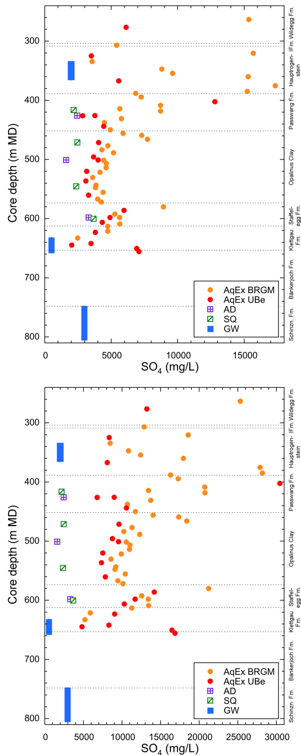
Fig. 5.3-1: \text{SO}_4 profiles with data from squeezing, advective displacement, aqueous extraction, and groundwater samples
