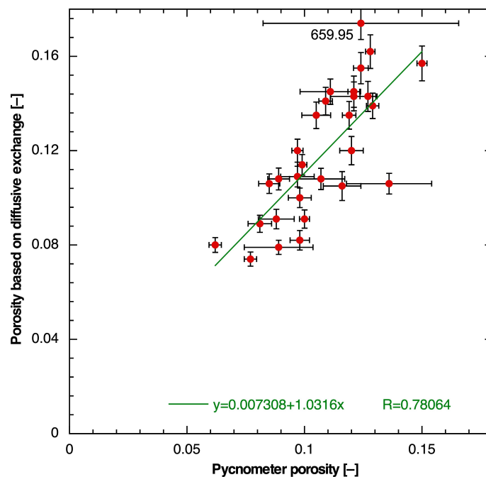
Fig. 4.3-9: Correlation of pycnometer porosity and porosity from isotope diffusive exchange
