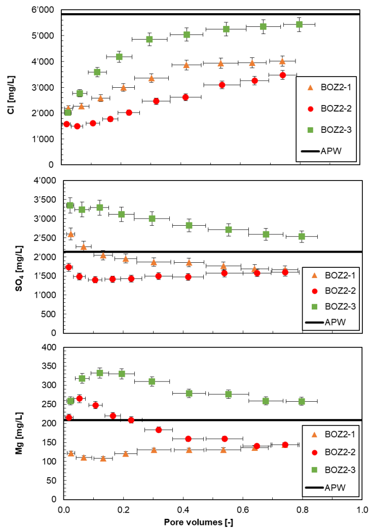
Fig. 4.7-9: Evolution of Cl, SO 4 and Mg during advective displacement experiments
