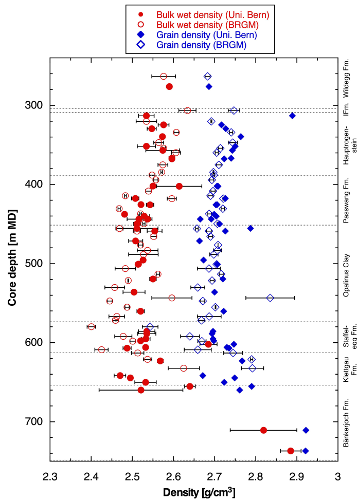
Fig. 4.3-5: Depth profile of bulk wet and grain densities
