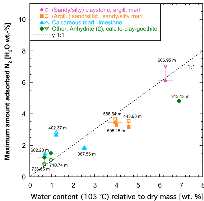
Fig. 4.3-19: Comparison of maximum amount of adsorbed N_2 (recalculated to H_2O wt.-%) with water content per dry sample mass
