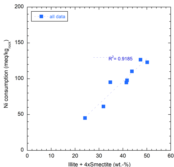
Fig. 5.6-4: Ni consumption as function of the sum of illite end-member content and 4× smectite end-member content.
