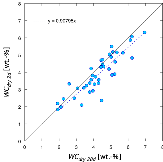
Fig. 3.4-1: Comparison of water contents WC_{dry} obtained by BRGM by drying at 105 °C over 2 d and over 28 d
