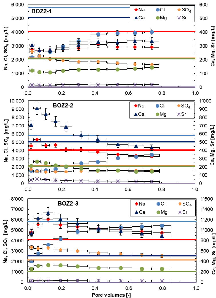
Fig. 4.7-8: Evolution of major components during advective displacement experiments
