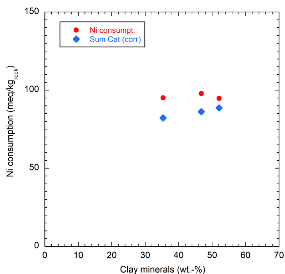
Fig. 5.6-1: Ni consumption and sum of (corr.) cations as a function of the clay-mineral content (data of University of Bern)
