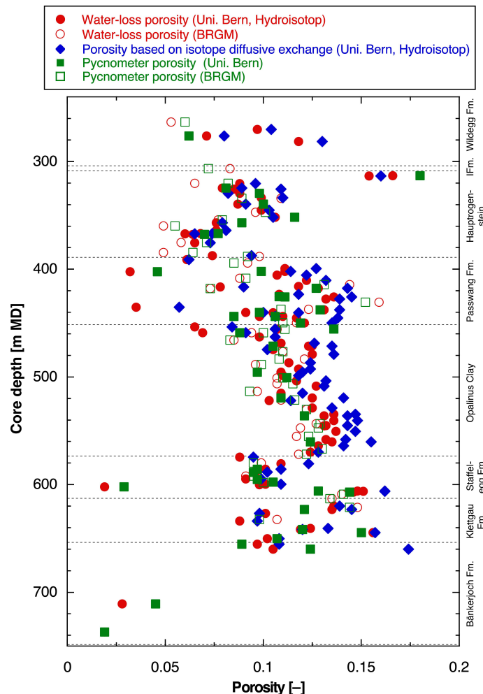
Fig. 4.3-11: Depth trends of porosities obtained by different methods and laboratories
