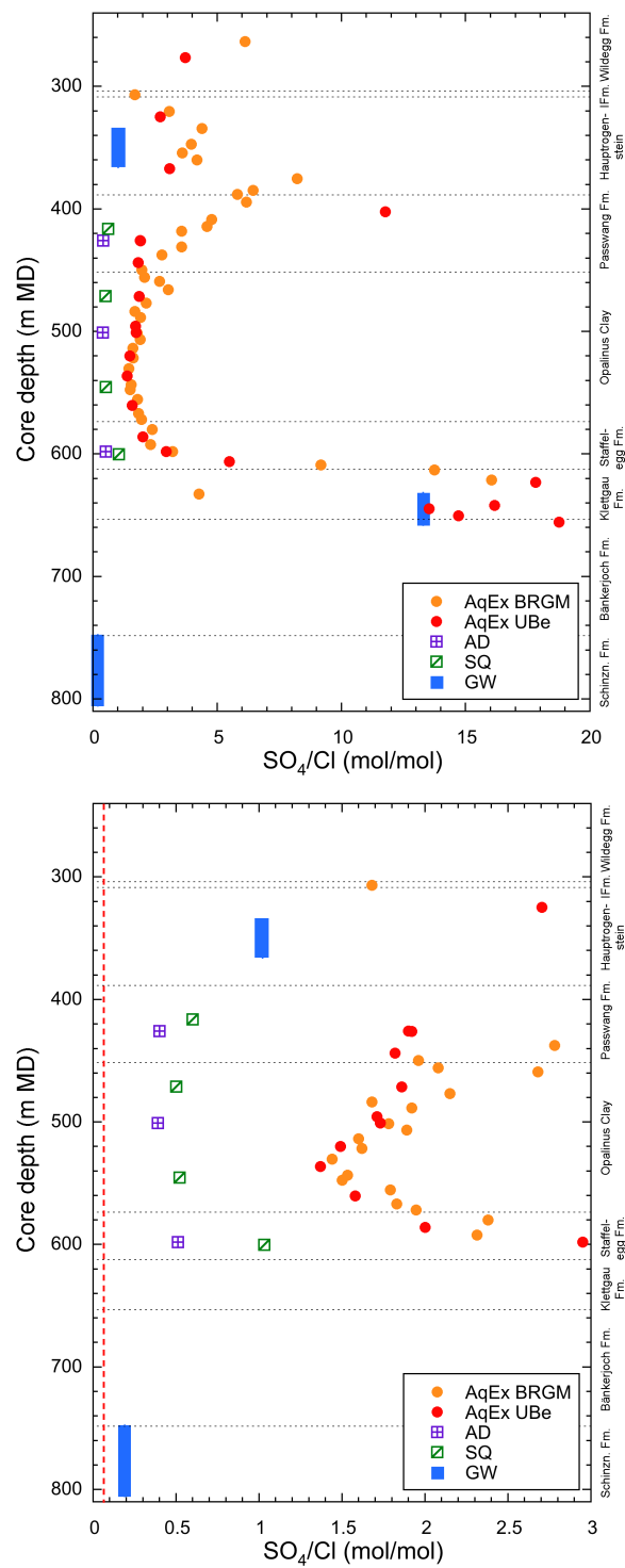
Fig. 5.3-2: Profiles showing molar \text{SO}_4/\text{Cl} ratios obtained from different methods at different scales
