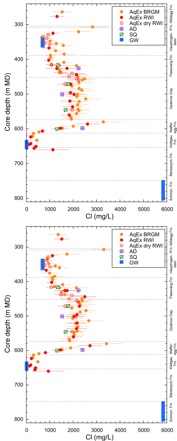
Fig. 5.2-1: Cl profile with data from squeezing, advective displacement, aqueous extraction, and groundwater samples
