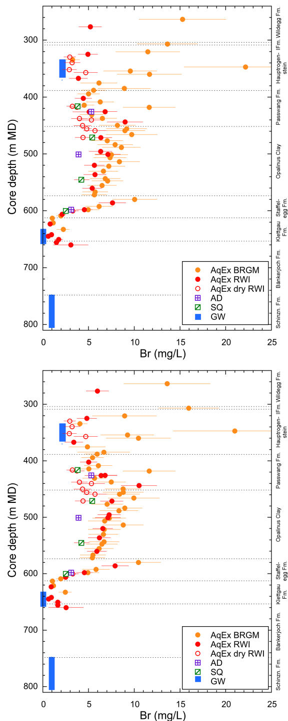
Fig. 5.2-2: Br profile with data from squeezing, advective displacement, aqueous extraction, and groundwater samples
