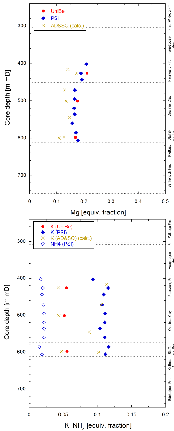
Fig. 5.6-6: Mg (above) and K, NH 4 (below) occupancies according to Uni versity of Bern and PSI data and "back calculated" from AD/SQ data
