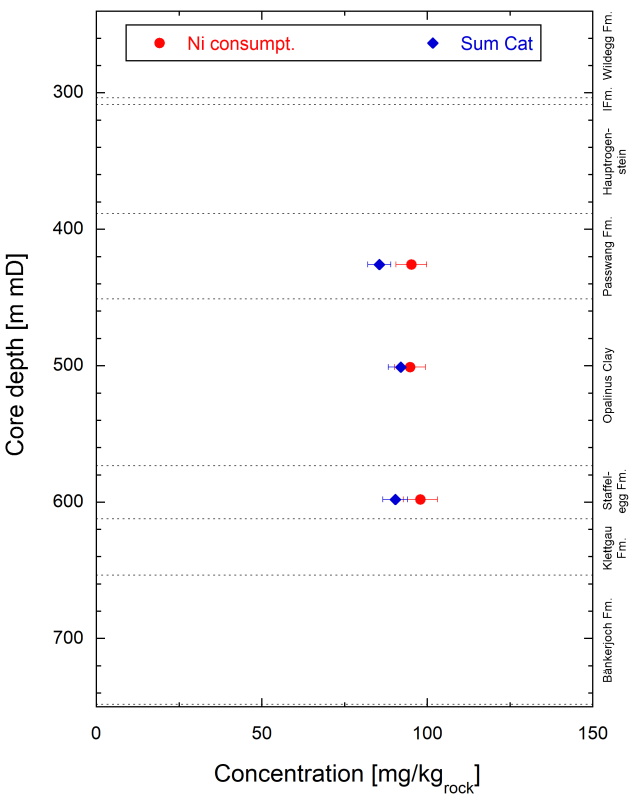
Fig. 4.5-1: Depth profile of Ni consumption and sum of cations (uncorrected, University of Bern data) Errors reflect propagated analytical uncertainties.
