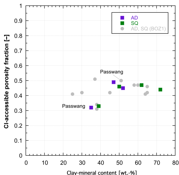
Fig. 5.1-1: Cl-accessible porosity fraction as a function of the clay-mineral content from AD and SQ data
