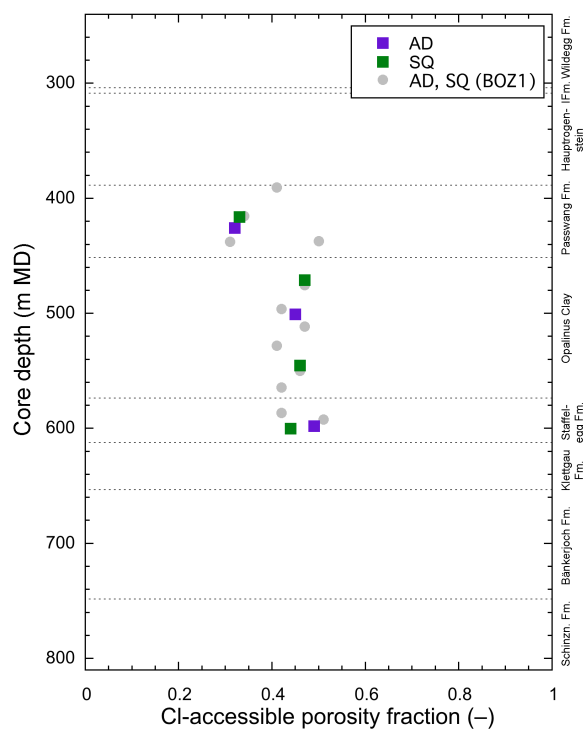
Fig. 5.1-3: CI-accessible porosity fraction as a function of depth
