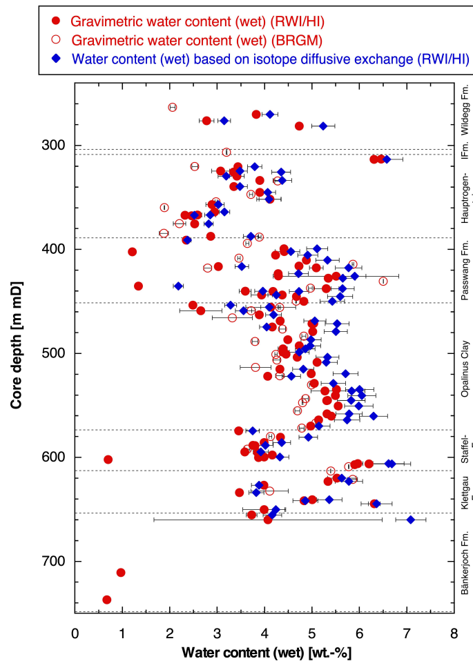
Fig. 4.3-1: Water content as a function of depth
