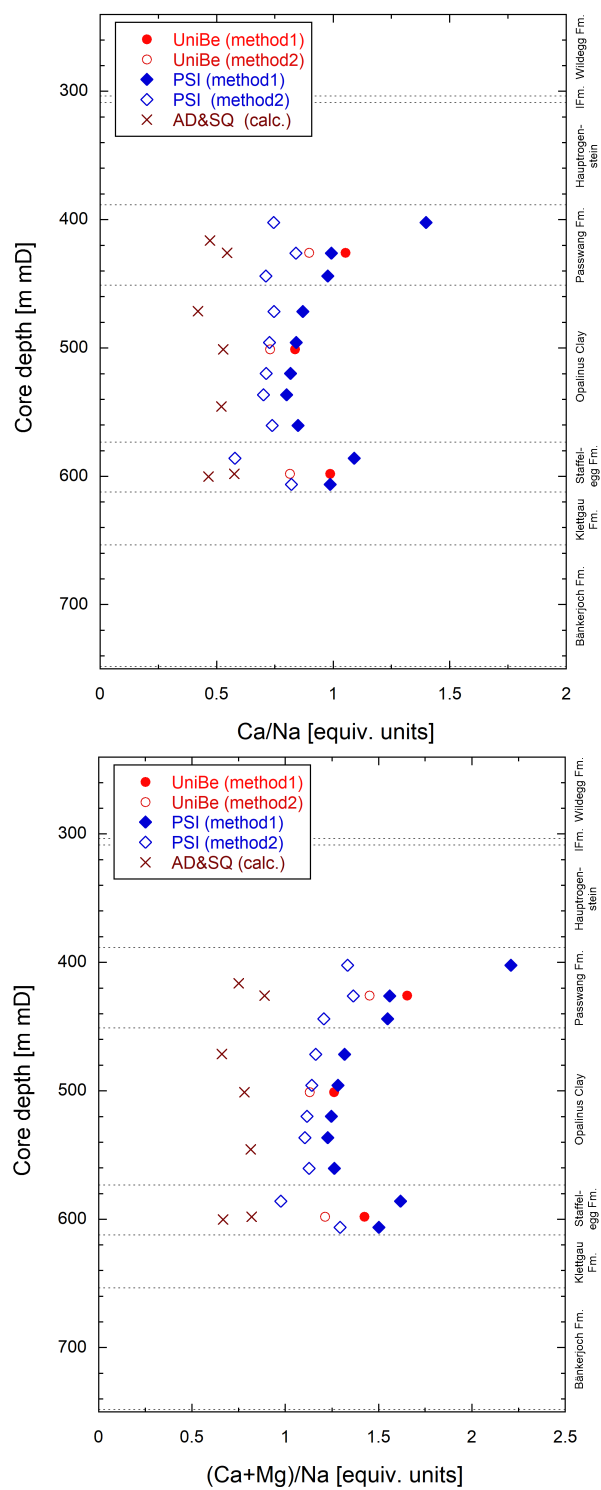
Fig. 5.6-8: Ca/Na ratios (above) and (Ca+Mg)/Na (below) according to University of Bern and PSI data and "back calculated" from AD/SQ data
