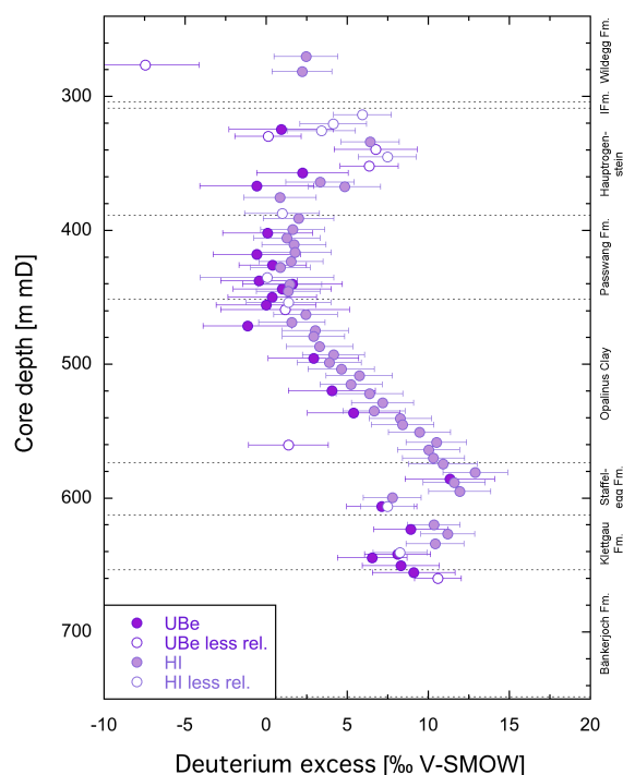
Fig. 4.8-4: Depth trend of deuterium excess in porewater based on the isotope diffusive exchange technique
