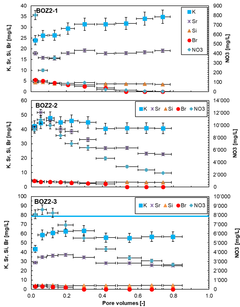
Fig. 4.7-10: Evolution of minor components during advective displacement experiments
