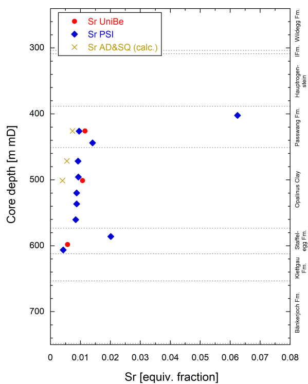
Fig. 5.6-7: Sr occupancies according to University of Bern and PSI data and "back calculated" from AD/SQ data
