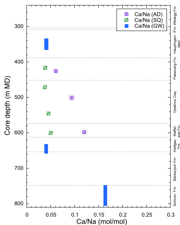
Fig. 5.4-3: Ca/Na ratio (molar units) for SQ and AD samples and groundwater
