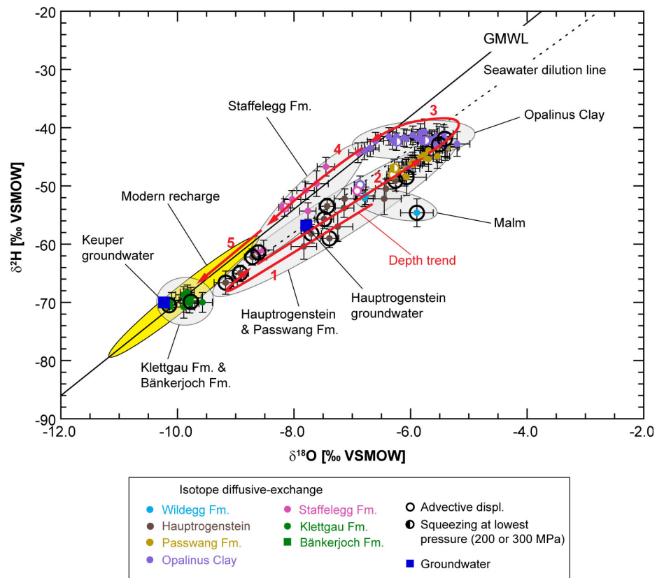
Fig. 5.7-2: \delta^{18}\text{O} vs. \delta^2\text{H} for groundwater and porewater derived by all techniques
