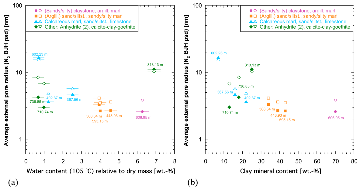
Fig. 4.3-20: Average external pore radius (assuming insignificant interlayer pore volume) based on the BJH pore size distribution from the N 2 isotherms (closed symbols: adsorption; open symbols: desorption) plotted against the gravimetric water content per dry mass of the samples (a) and against the total clay-mineral content (b)
