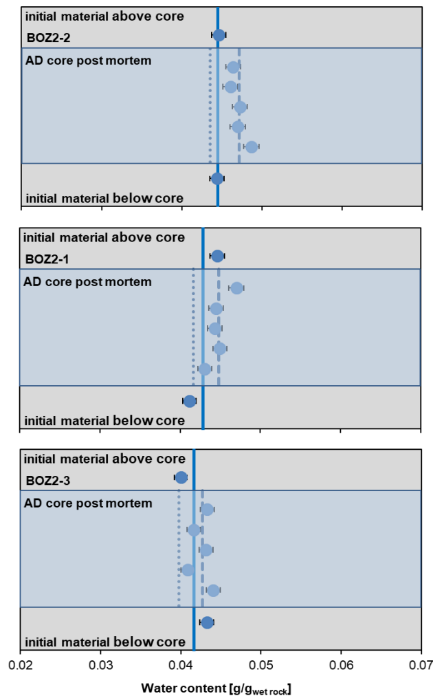
Fig. 4.7-3: Details of water content measurements before and after AD experiments
