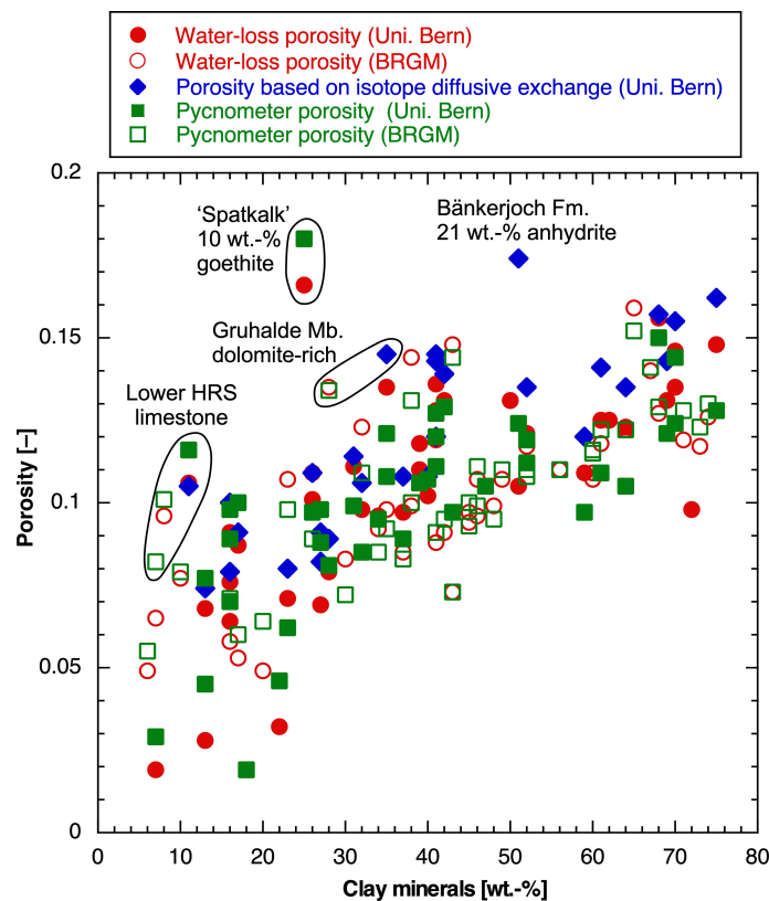
Fig. 4.3-12: Porosity as a function of clay-mineral content
