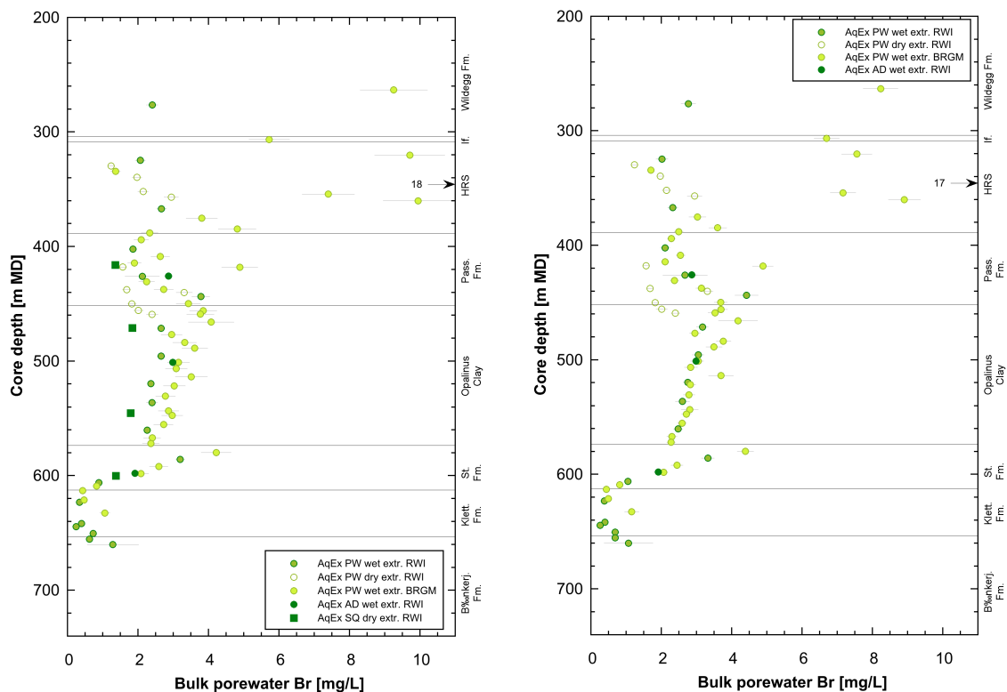
Fig. 4.4-8 Bulk porewater Br concentrations versus depth from aqueous extracts of PW, AD and SQ samples
