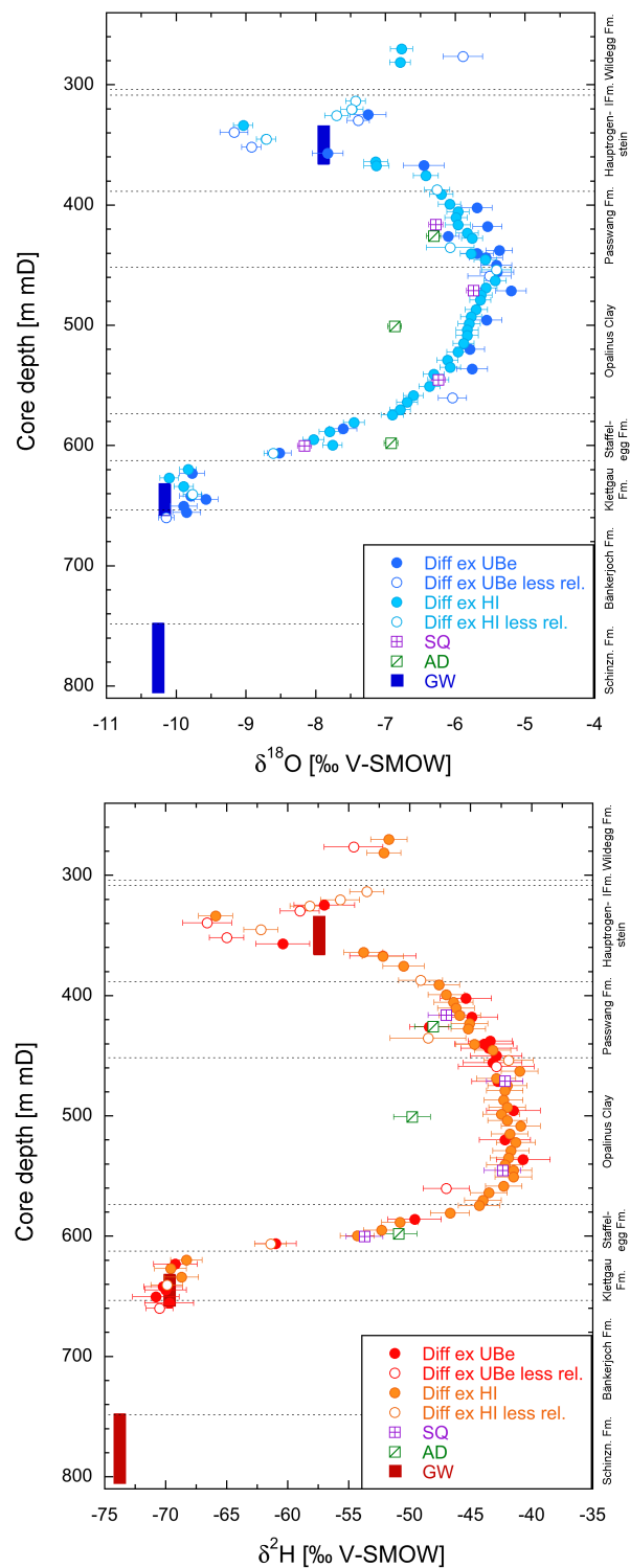
Fig. 5.7-1: Depth trends of \delta^{18}\text{O} and \delta^2\text{H} in groundwater and porewater derived by all techniques
