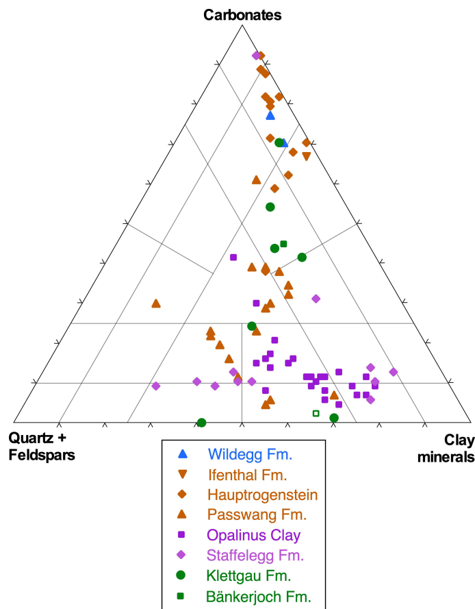
Fig. 4.2-3: Mineralogical composition of studied samples in the Füchtbauer triangle
