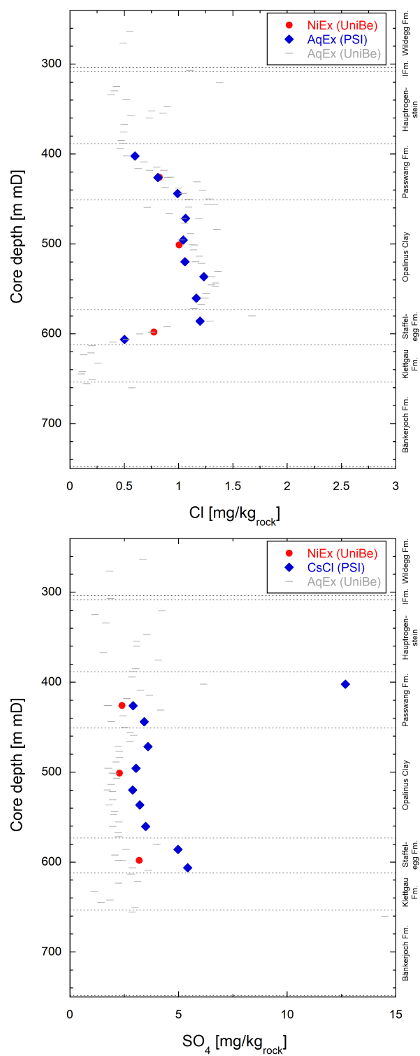
Fig. 5.6-10: Extracted Cl (above) and SO 4 (below) according to University of Bern and PSI data
