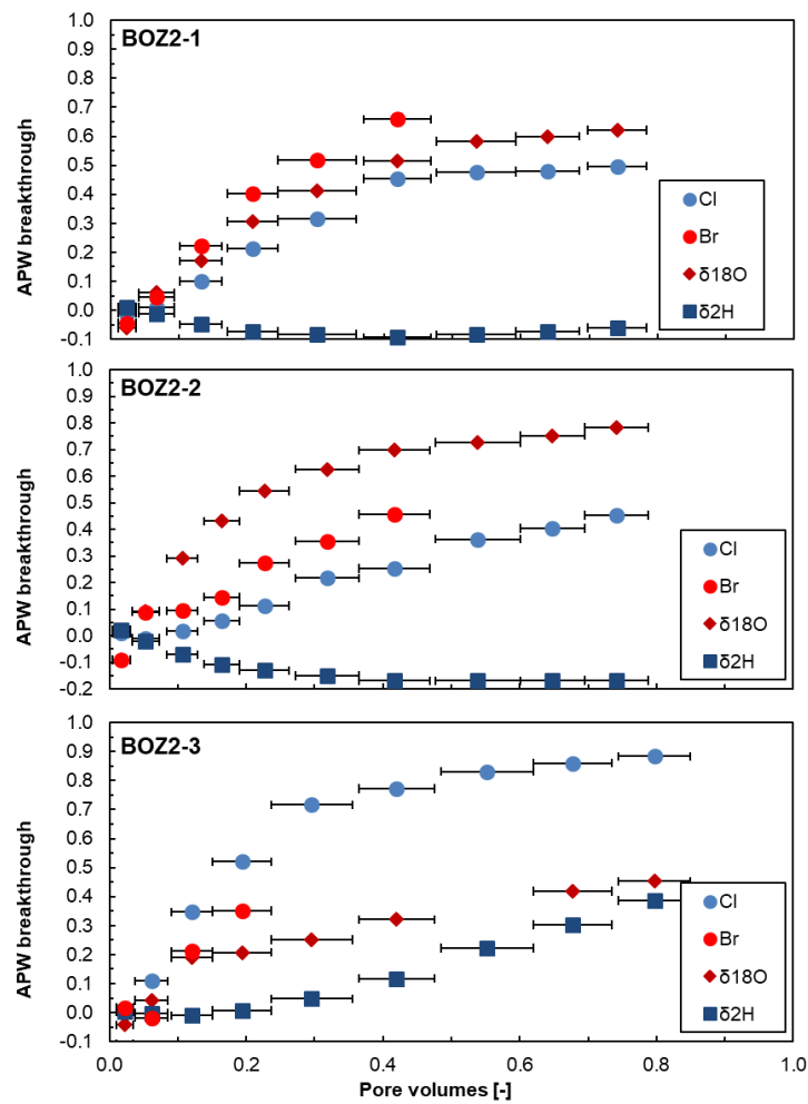
Fig. 4.7-17: Breakthrough of Cl, Br, \delta^2\text{H} and \delta^{18}\text{O} during advective displacement experiments
