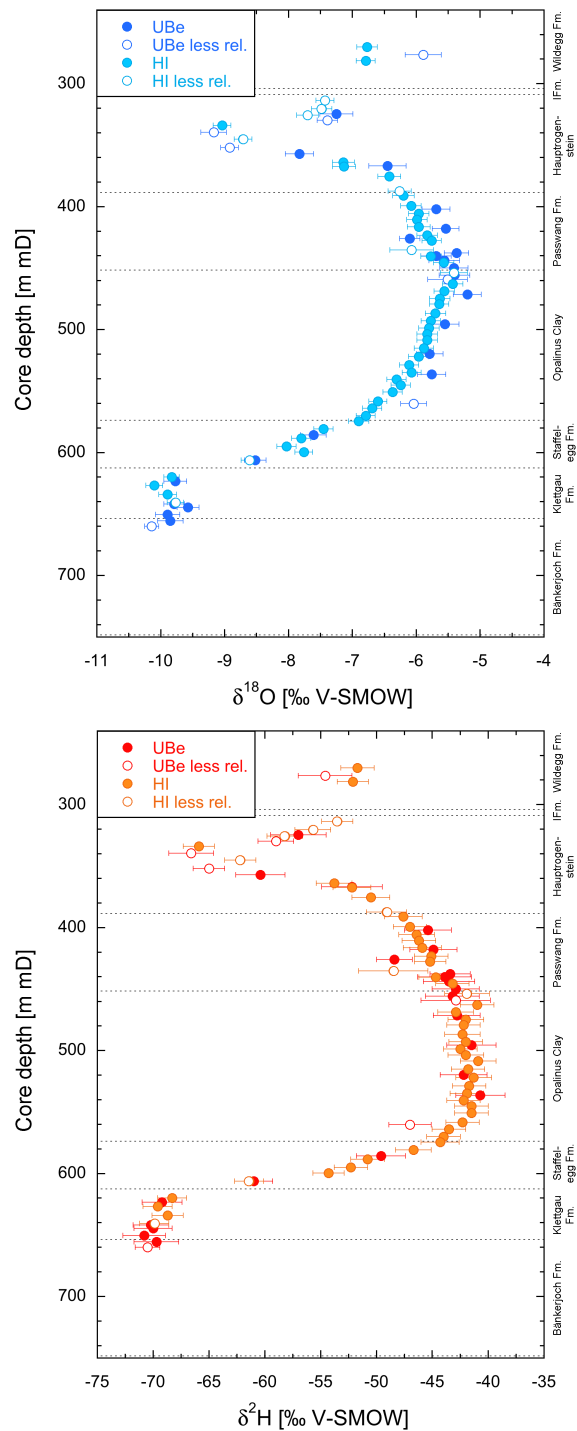
Fig. 4.8-3: Depth distribution of porewater \delta^{18}\text{O} and \delta^2\text{H} values obtained from isotope diffusive-exchange experiments
