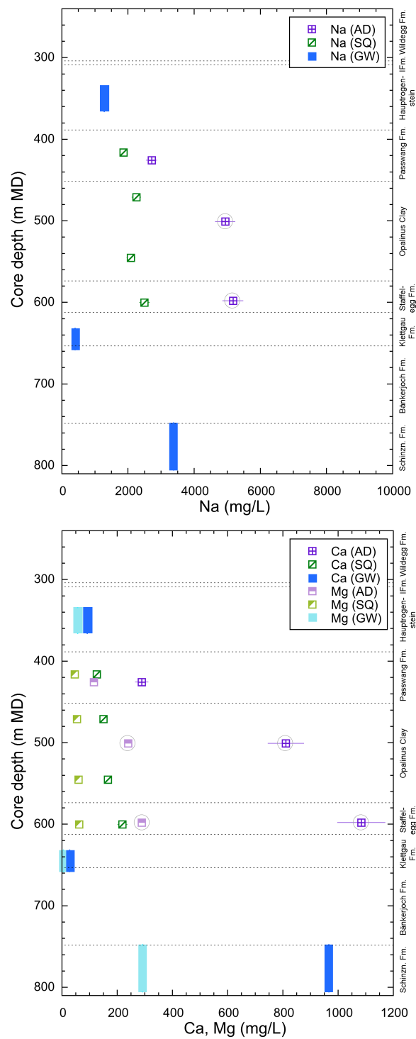
Fig. 5.4-1: Profiles for Na, Ca, Mg, K and Sr in porewater with data from squeezing, advective displacement and groundwater samples
