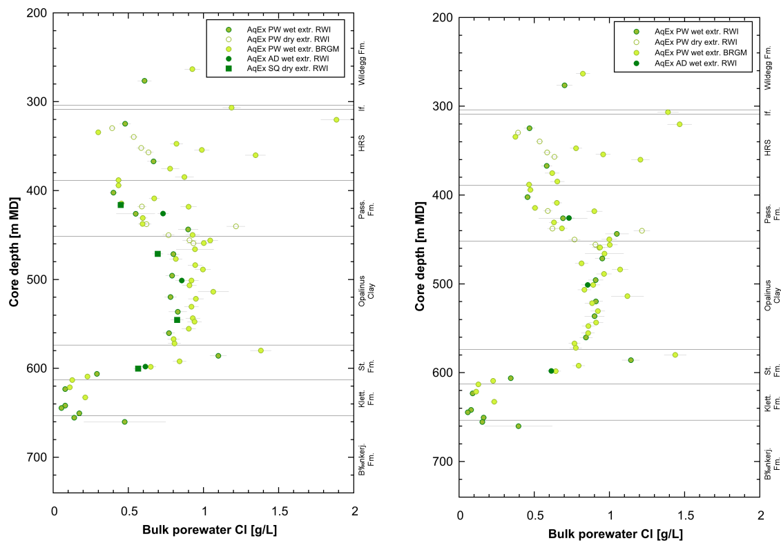
Fig. 4.4-7: Bulk porewater Cl concentrations versus depth from aqueous extracts of PW, AD and SQ samples
