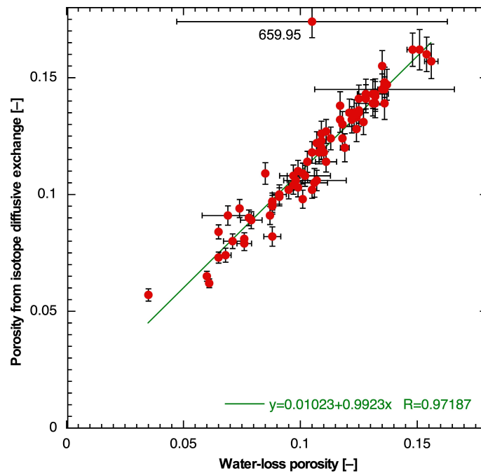
Fig. 4.3-8: Correlation of water-loss porosity and porosity from isotope diffusive exchange
