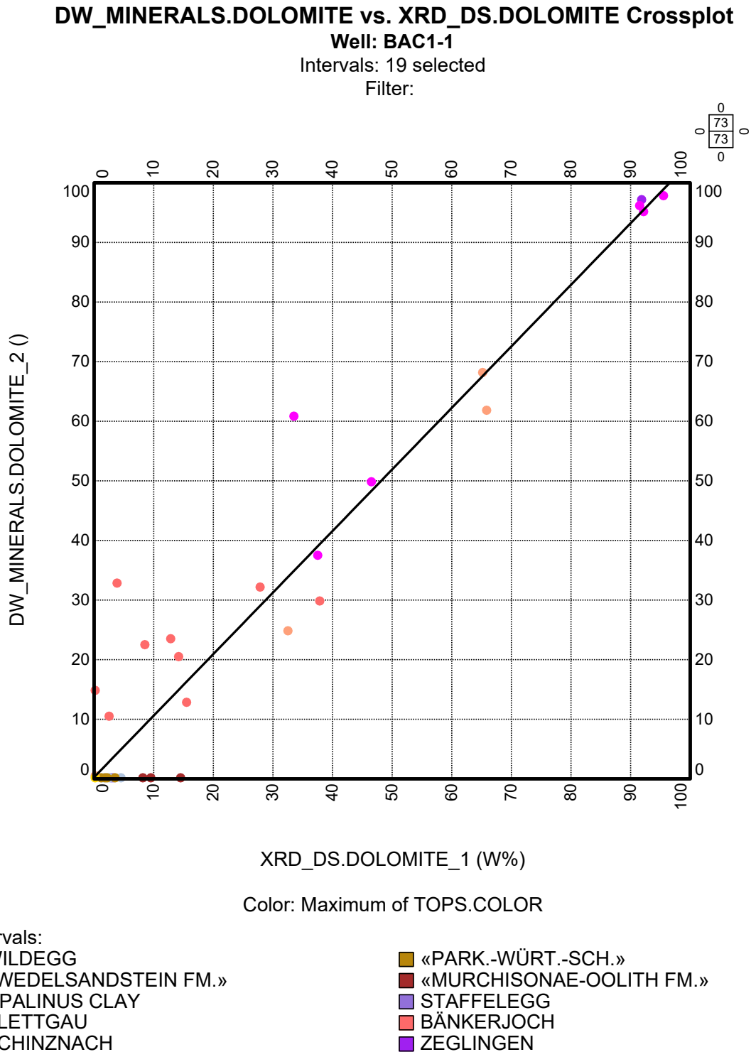
Fig. 4-6: Weight % of dolomite from MultiMin (y-axis) compared to core XRD data (x-axis), Wildegg to Zeglingen Formations
