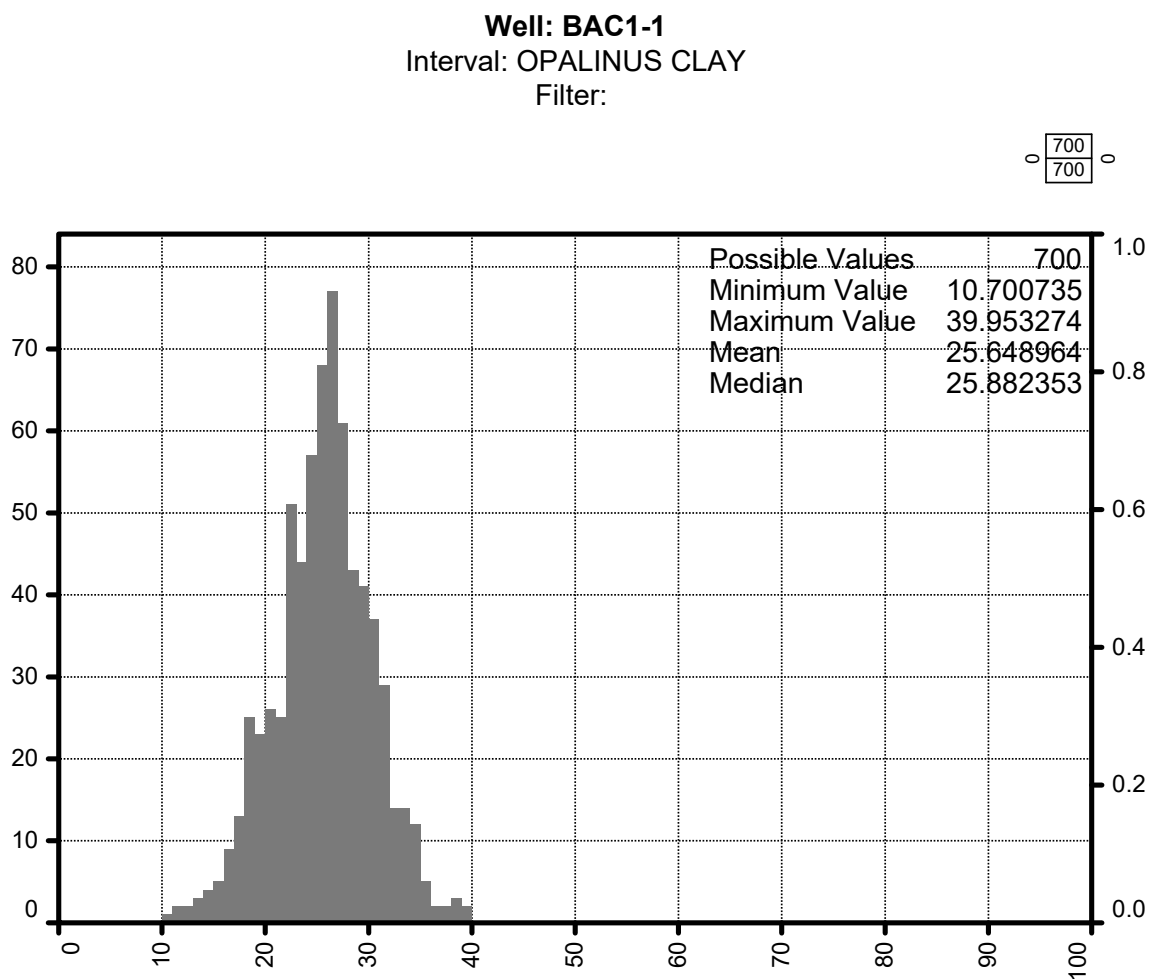
Fig. 4-13: QF-silicates (quartz and feldspars) weight percentage frequency histogram in the Opalinus Clay
