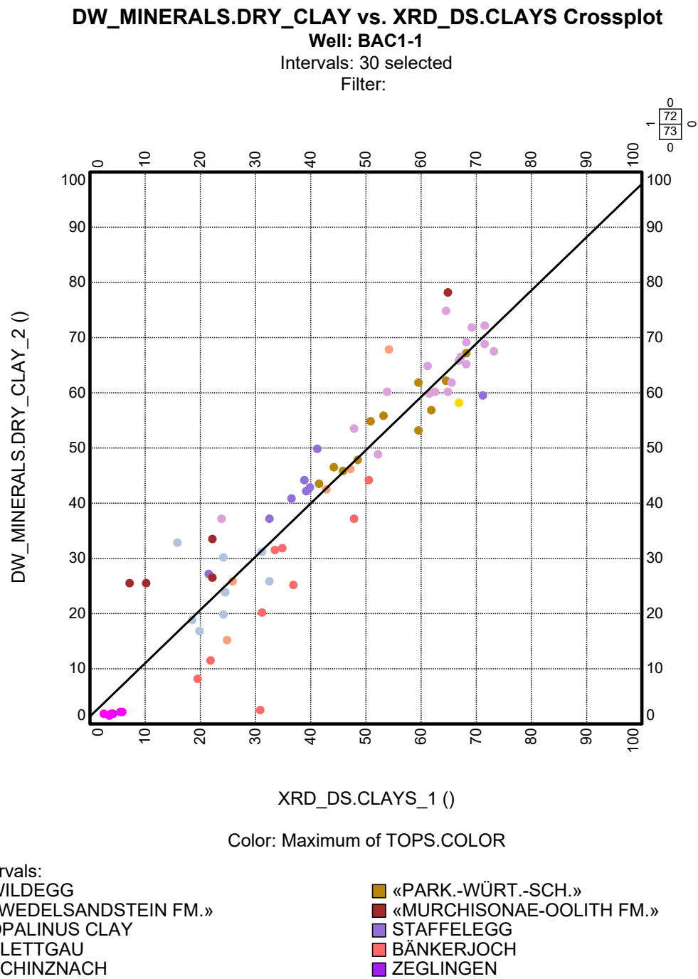
Fig. 4-1: Weight % of dry clay from MultiMin (y-axis) compared to core XRD data (x-axis), Wildegg to Zeglingen Formations
