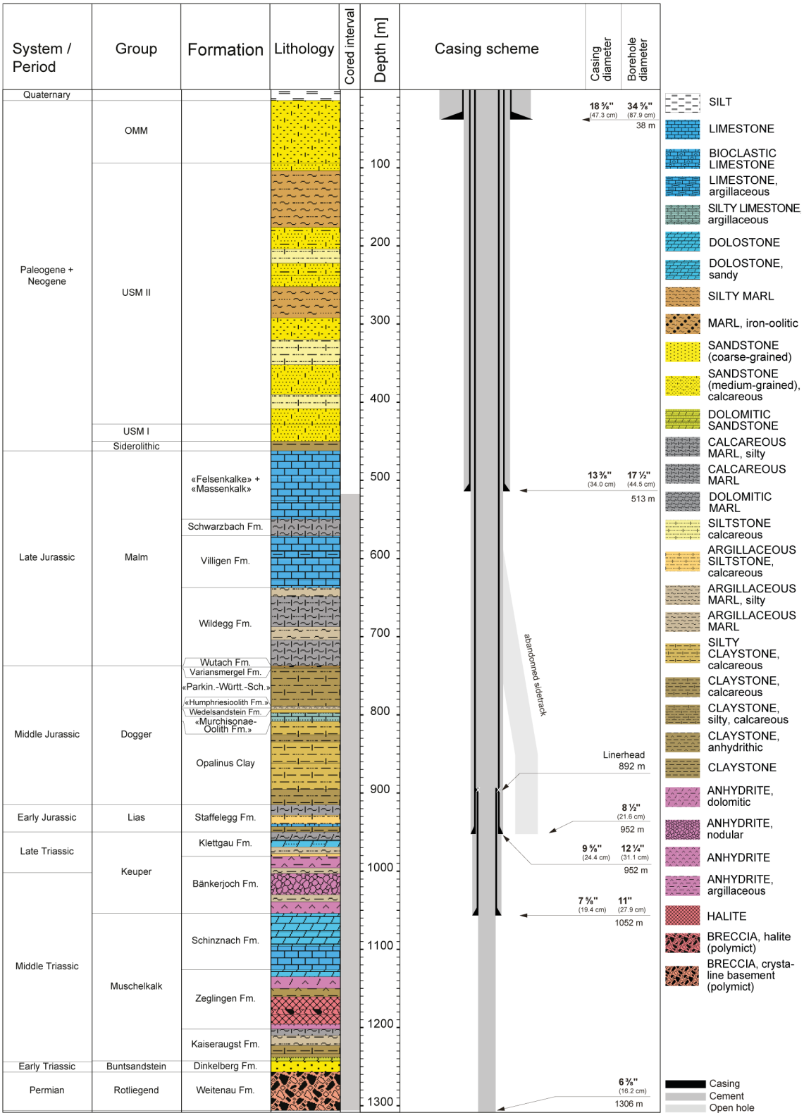
Fig. 1-3: Lithostratigraphic profile and casing scheme for the BAC1-1 borehole 5
