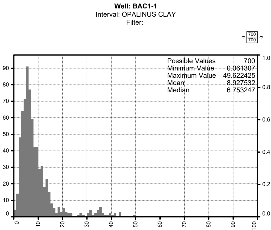
Fig. 4-11: Calcite weight percentage frequency histogram in the Opalinus Clay
