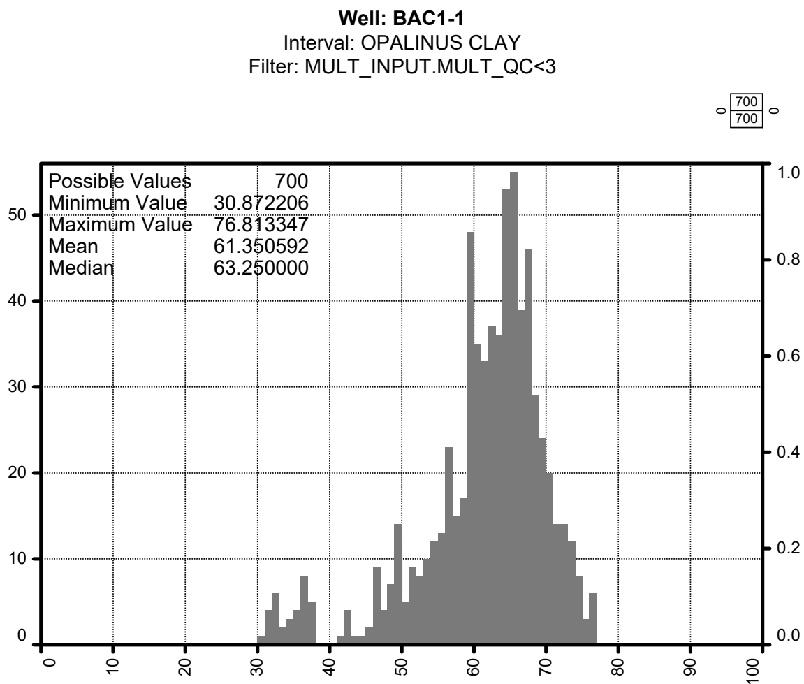
Fig. 4-8: Dry clay weight percentage frequency histogram in the Opalinus Clay
