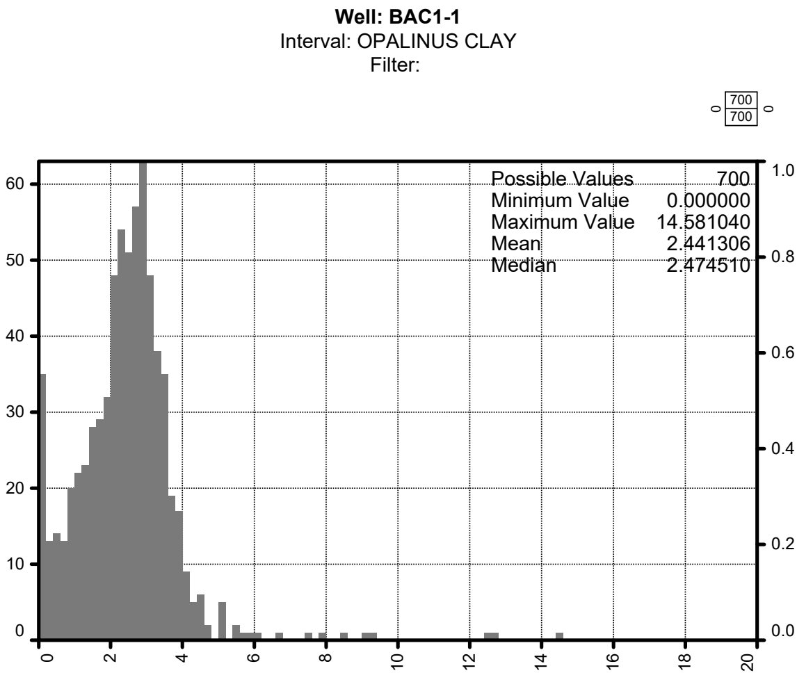
Fig. 4-12: Siderite weight percentage frequency histogram in the Opalinus Clay X-axis is the siderite weight % from MultiMin, y-axis the number of points per bin (100 bins).
