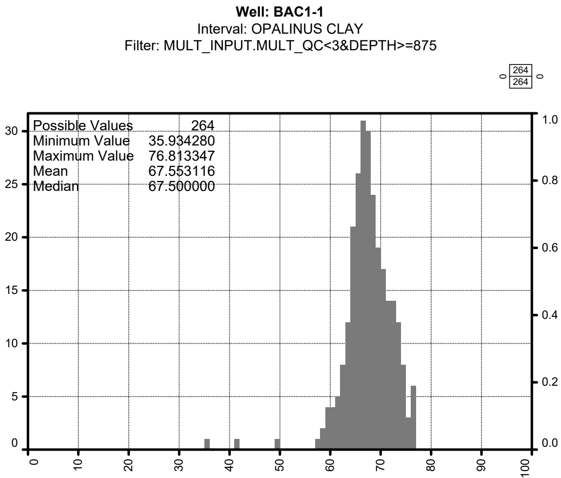
Fig. 4-10: Dry clay weight percentage frequency histogram in the lower section of the Opalinus Clay (below 875.0 m)
