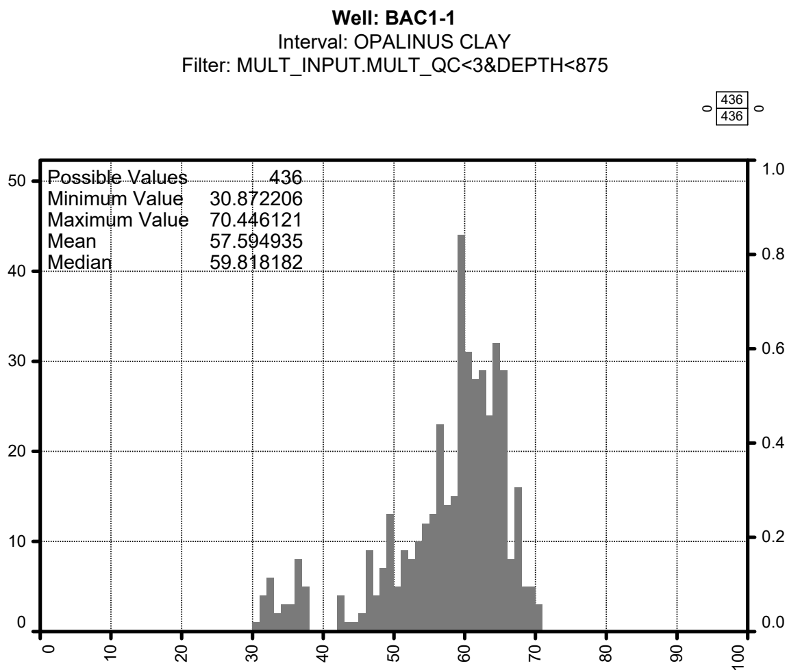
Fig. 4-9: Dry clay weight percentage frequency histogram in the upper section of the Opalinus Clay (above 875.0 m)
