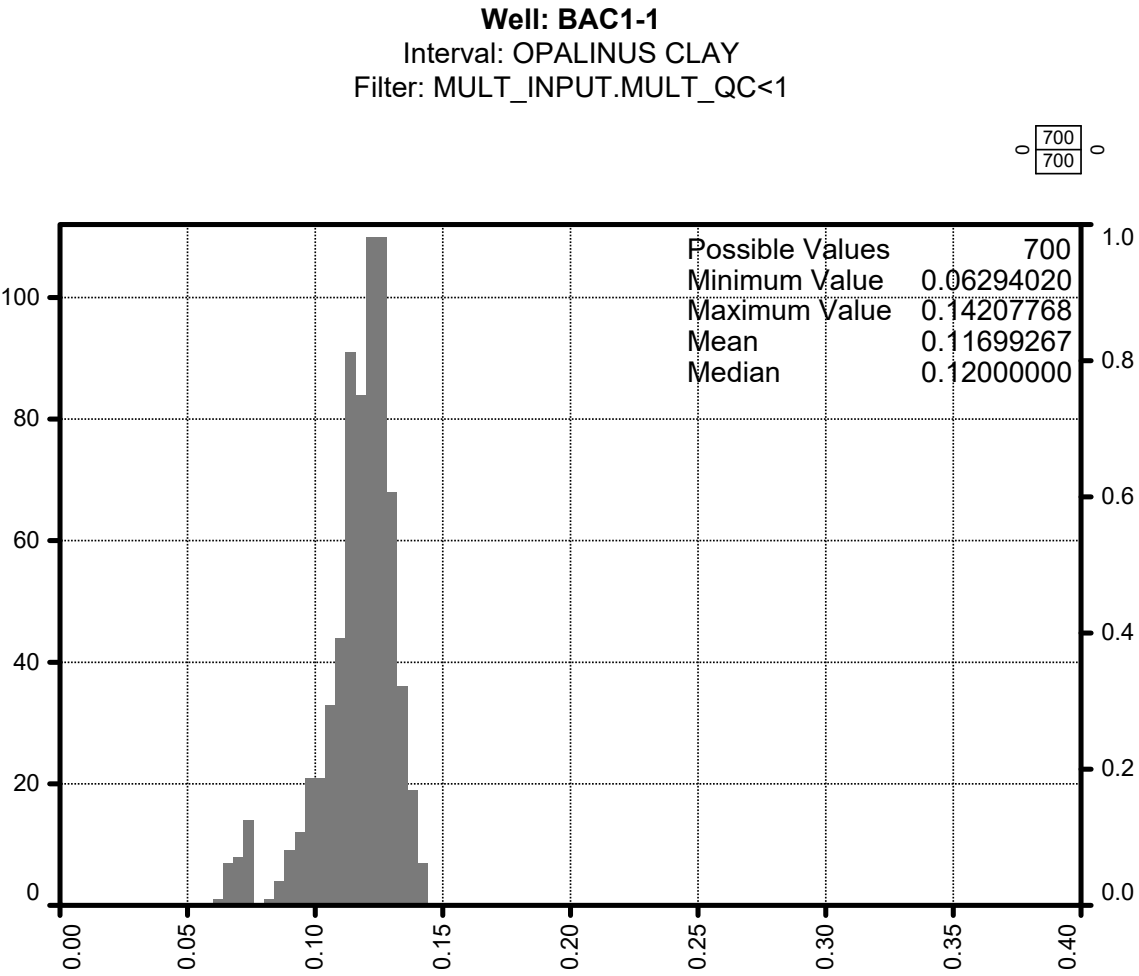
Fig. 4-14: Total porosity frequency histogram in the Opalinus Clay X-axis is the total porosity v/v from MultiMin, y-axis the number of points per bin (100 bins).
