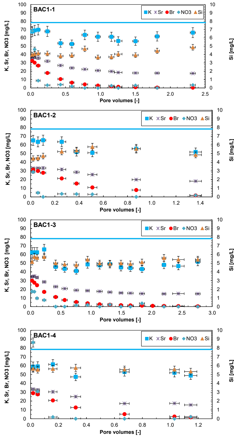
Fig. 4.7-10: Evolution of minor components during advective-displacement experiments
