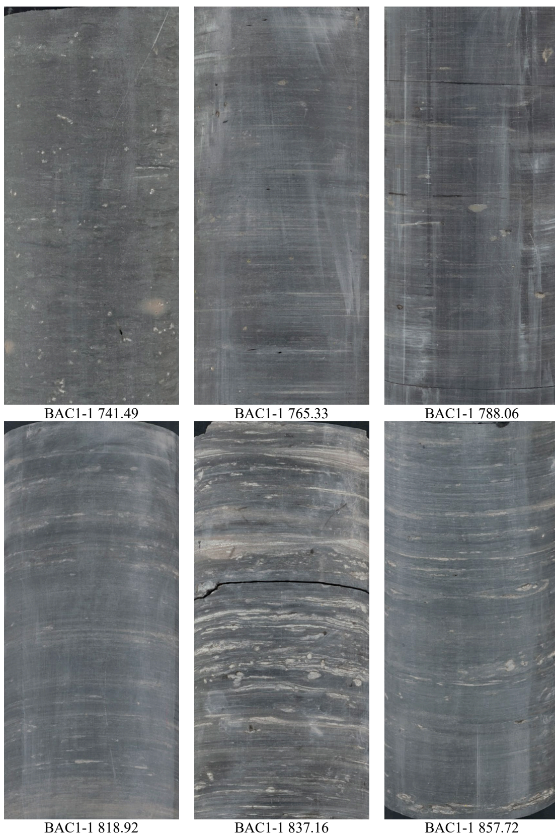
Fig. 4.6-1: Photographs of core samples subjected to squeezing Width of photographs = 9.5 cm.
