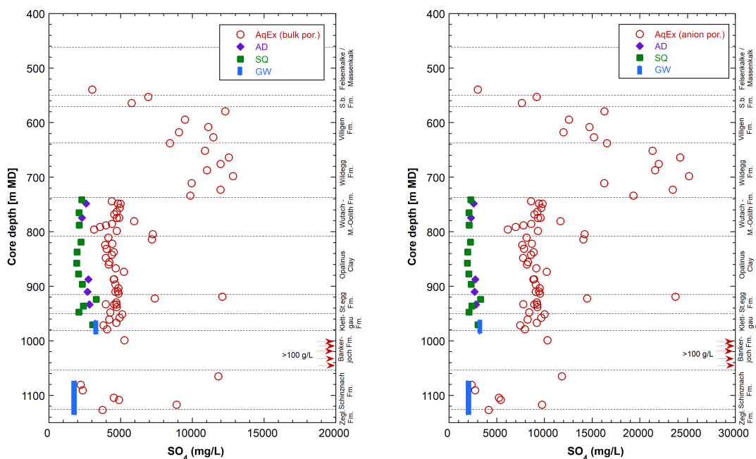
Fig. 5.3-1: SO 4 profiles with data from squeezing, advective displacement, aqueous extraction, and groundwater samples: left: AqEx data re-calculated to bulk porosity, right: AqEx data re-calculated to anion-accessible porosity
