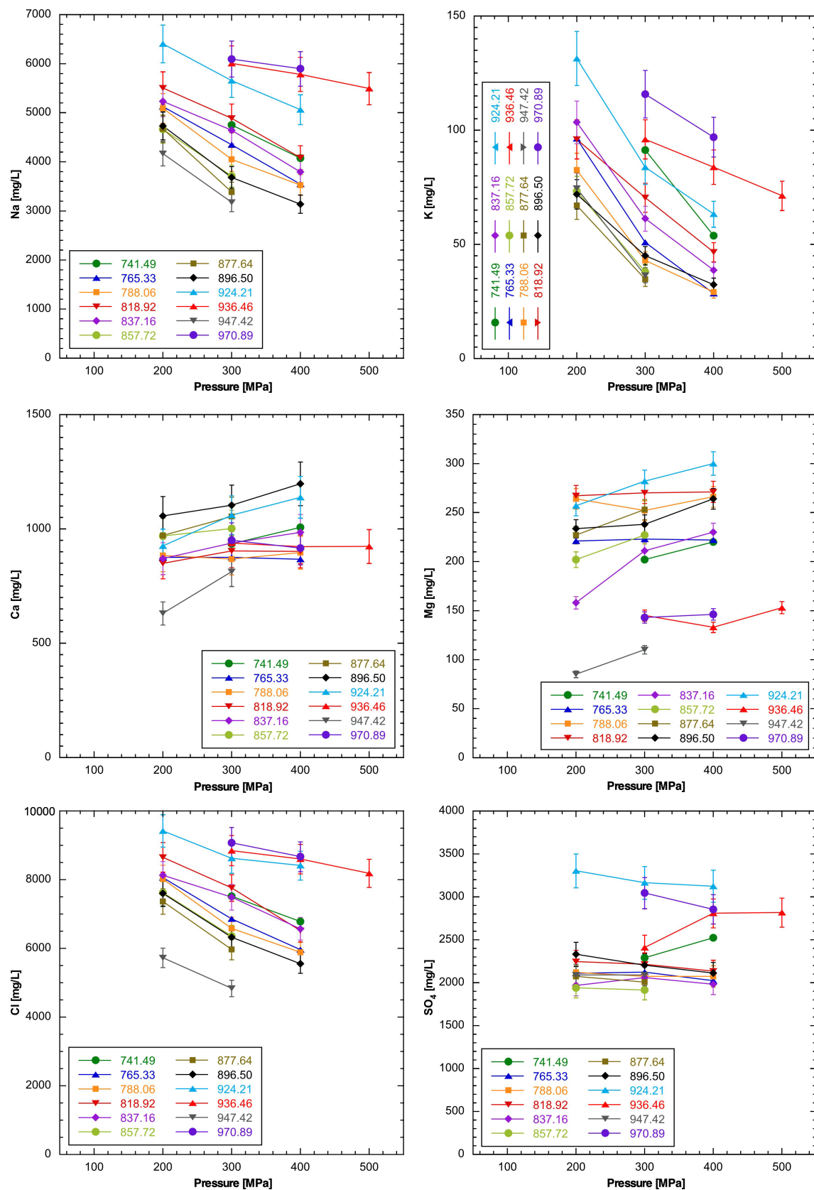
Fig. 4.6-4: Ion concentrations in squeezed waters as a function of squeezing pressure
