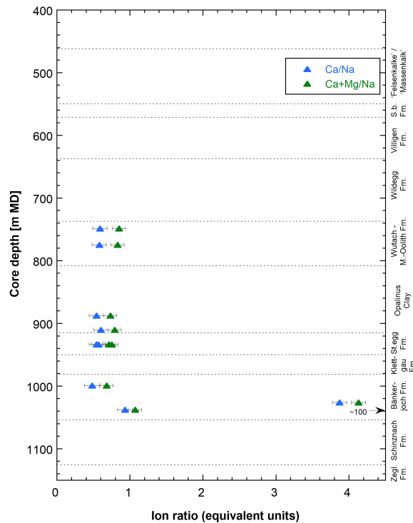
Fig. 4.5-3: Depth profiles of Ca/Na and (Ca+Mg)/Na ratios in Ni-en extracts (Uni Bern data)
