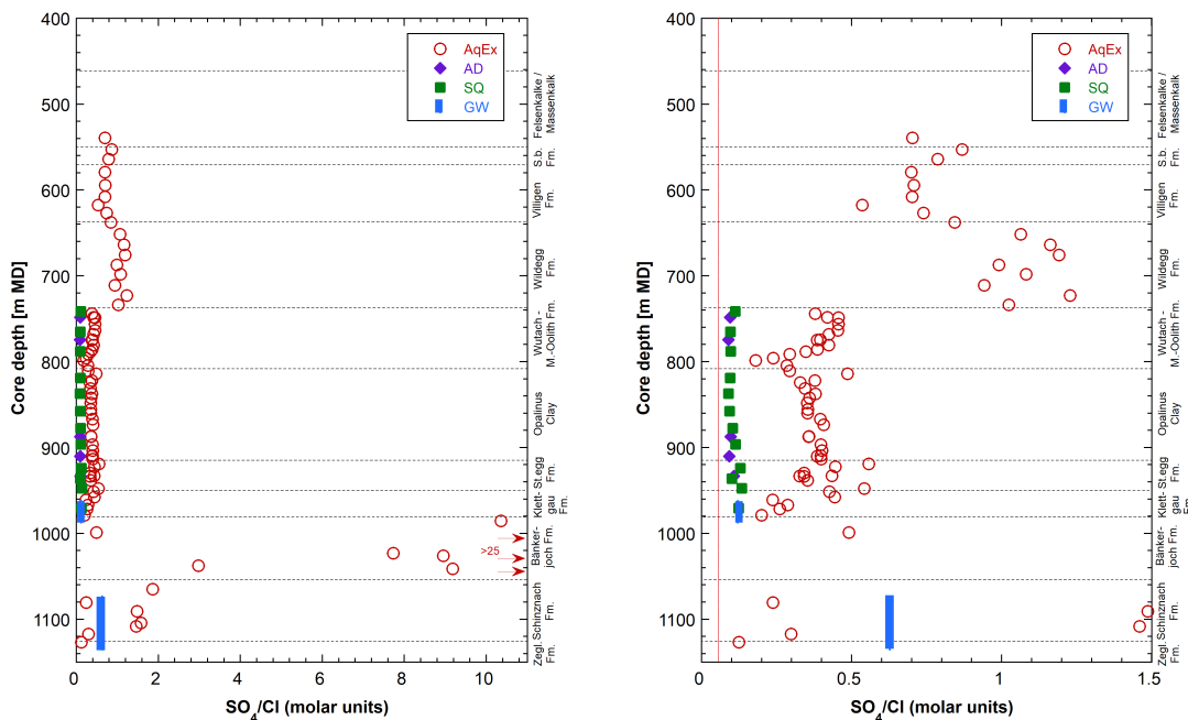
Fig. 5.3-2: Profiles showing molar \text{SO}_4/\text{Cl} ratios obtained from different methods
