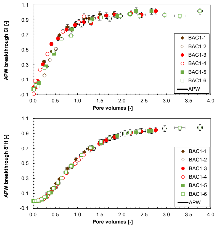
Fig. 4.7-18: Comparison of Cl and \delta^2\text{H} breakthrough during advective-displacement experiments
