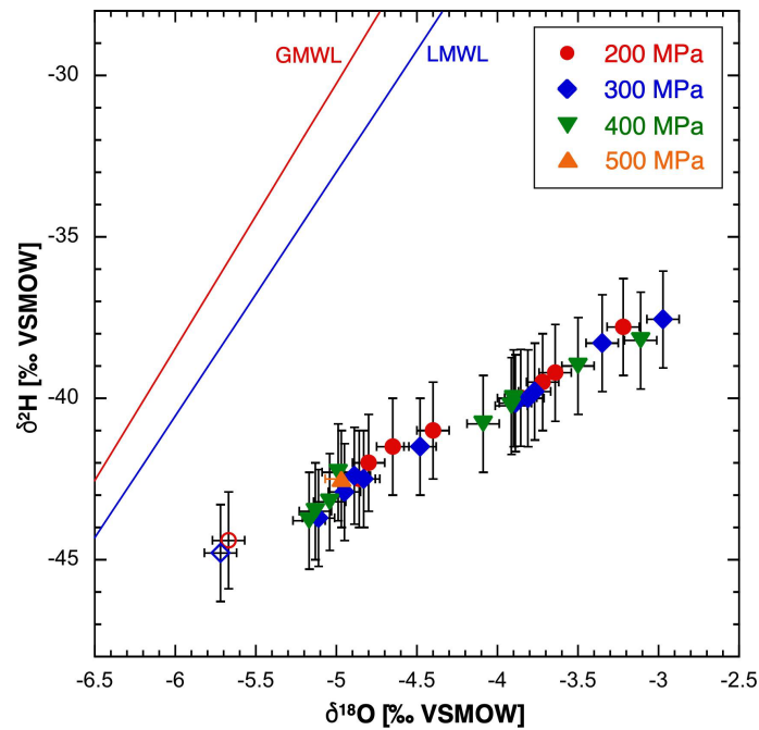
Fig. 4.6-8: Plot of \delta^{18}\text{O} vs. \delta^2\text{H} for squeezed waters
