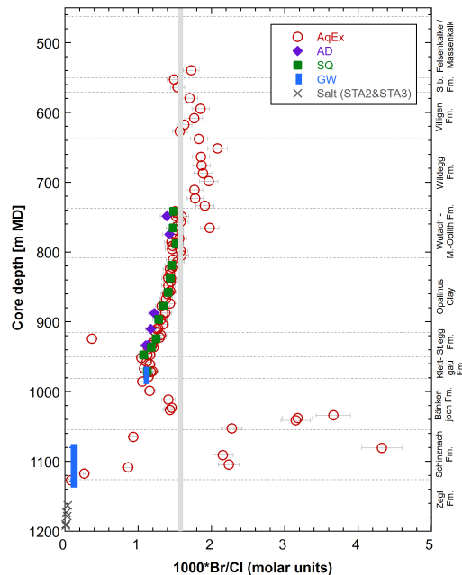
Fig. 5.2-4 1'000*Br/Cl (molar units) profile with data from squeezing, advective displacement, aqueous extraction, groundwater and halite samples
