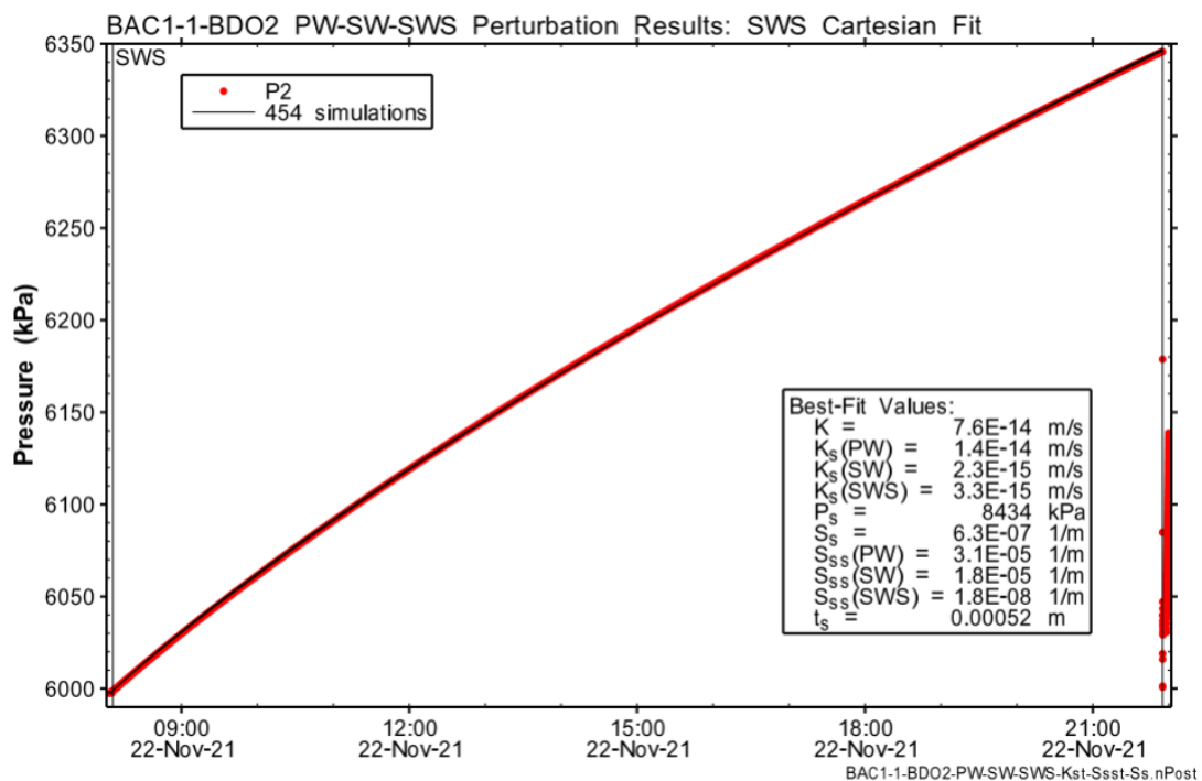
Fig. B-12: Hydraulic test BAC1-1-BDO2: Cartesian horsetail plot of the perturbation simulations on the SWS phase, accepting the fit discriminant
