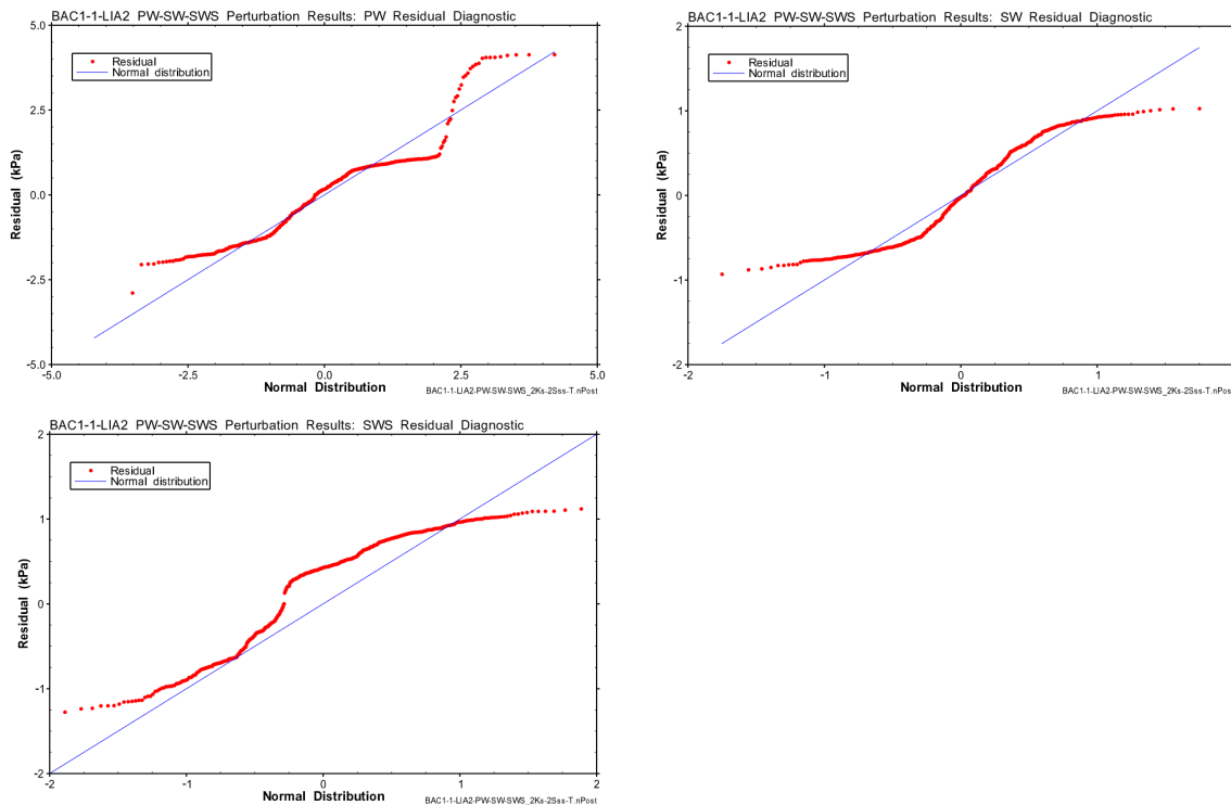
Fig. B-32: Hydraulic test BAC1-1-LIA2: Quantile-normal plot of residuals from the best Cartesian fit to PW phase (top left), SW phase (top right) and SWS phase data (bottom left)
