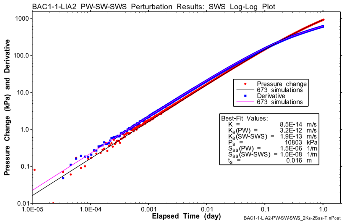
Fig. B-30: Hydraulic test BAC1-1-LIA2: Log-log horsetail plot of the perturbation simulations on the SWS phase, accepting the fit discriminant
