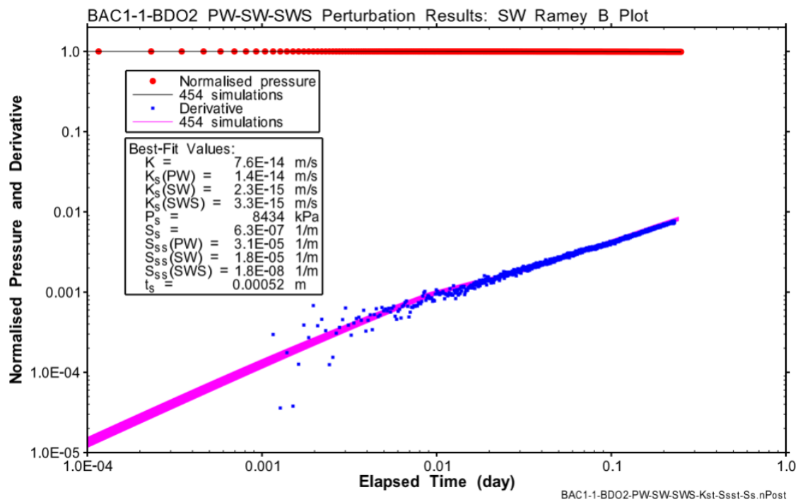
Fig. B-11: Hydraulic test BAC1-1-BDO2: Ramey B horsetail plot of the perturbation simulations on the SW phase, accepting the fit discriminant
