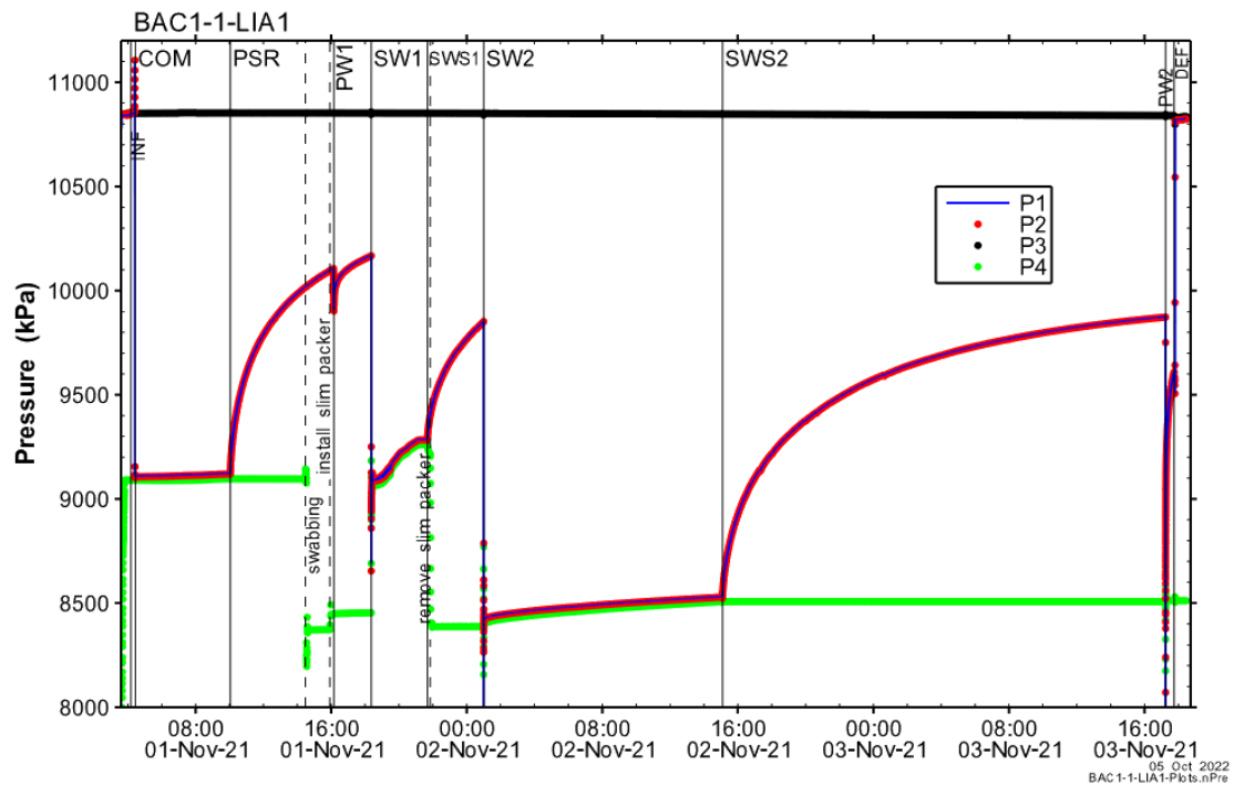
Fig. 4-16: Hydraulic packer test BAC1-1-LIA1: Overview plot of pressure vs. time and date
