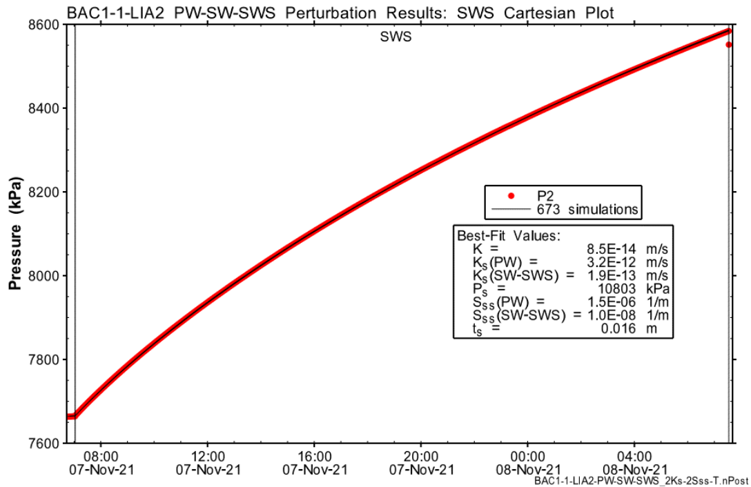
Fig. B-29: Hydraulic test BAC1-1-LIA2: Cartesian horsetail plot of the perturbation simulations on the SWS phase, accepting the fit discriminant
