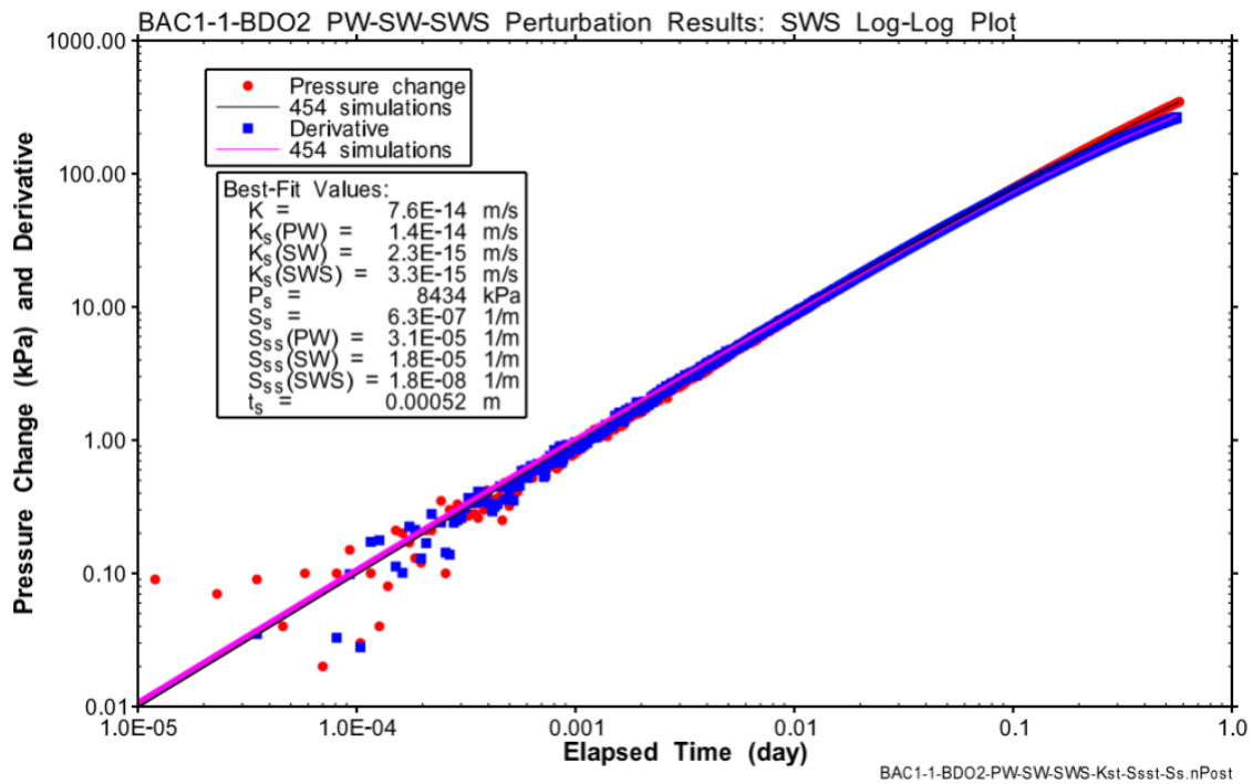
Fig. B-13: Hydraulic test BAC1-1-BDO2: Log-log horsetail plot of the perturbation simulations on the SWS phase, accepting the fit discriminant
