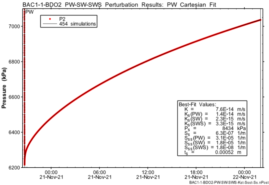
Fig. B-8: Hydraulic test BAC1-1-BDO2: Cartesian horsetail plot of the perturbation simulations on the PW phase, accepting the fit discriminant 454 / 1'000 results with a normalised objective function value less than 1.35.
