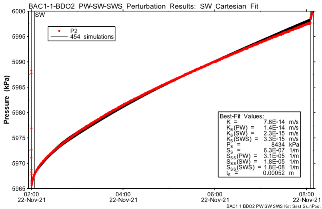
Fig. B-10: Hydraulic test BAC1-1-BDO2: Cartesian horsetail plot of the perturbation simulations on the SW phase, accepting the fit discriminant
