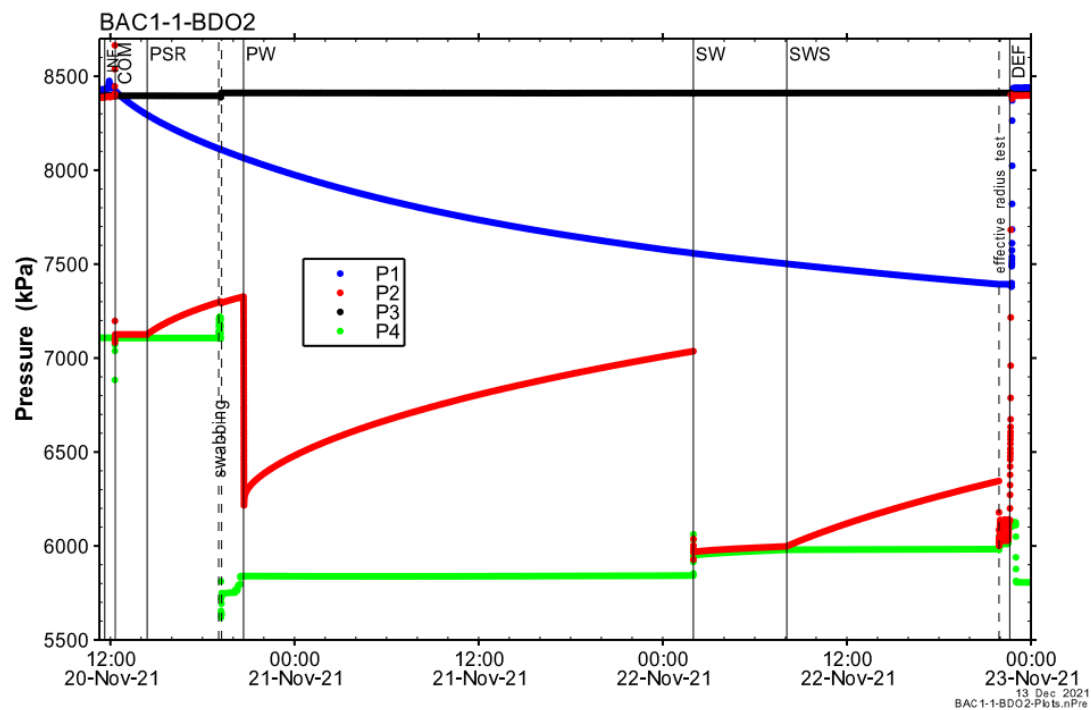
Fig. 4-8: Hydraulic packer test BAC1-1-BDO2: Overview plot of pressure vs. time and date
