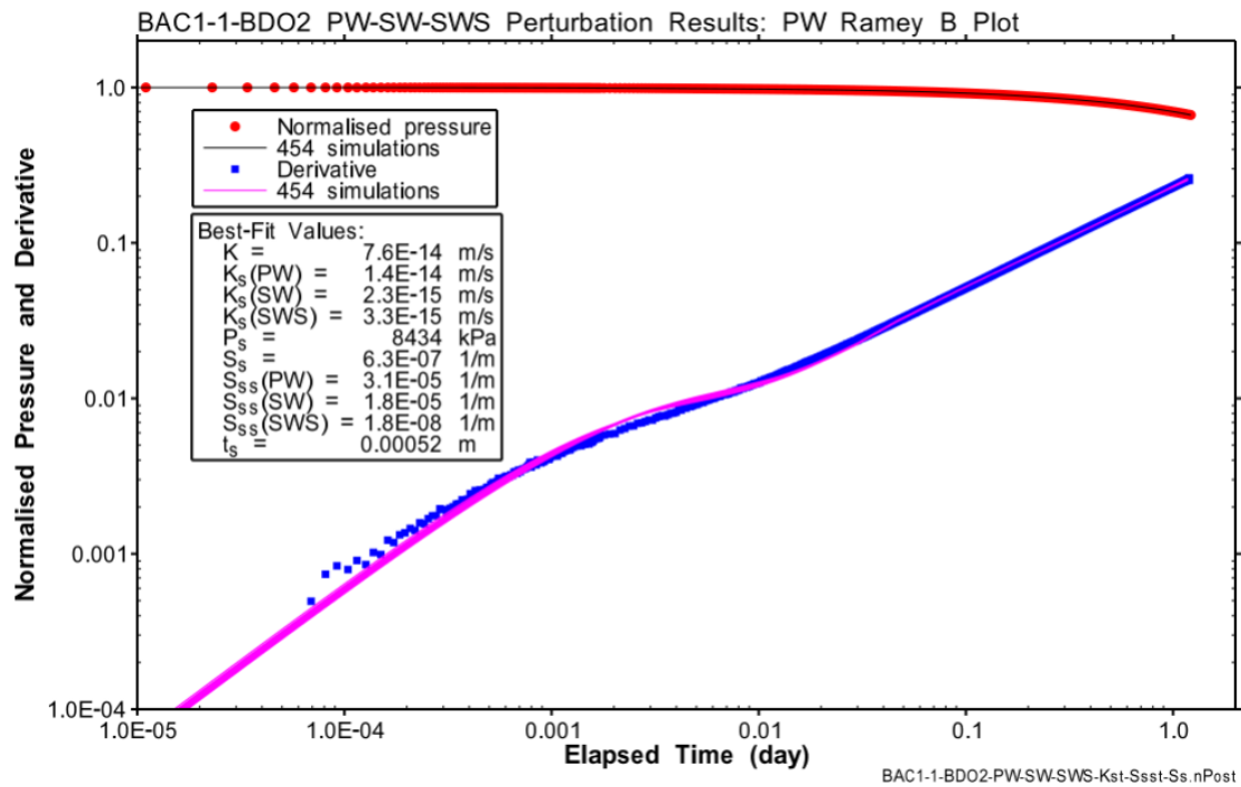
Fig. B-9: Hydraulic test BAC1-1-BDO2: Ramey B horsetail plot of the perturbation simulations on the PW phase, accepting the fit discriminant
