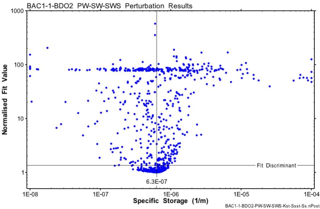
Fig. B-7: Hydraulic test BAC1-1-BDO2: Distribution of the normalised objective function value over S_s for the perturbation result of the PW-SW-SWS test sequence 994 / 1'000 results with a normalised objective function value less than 1'000.
