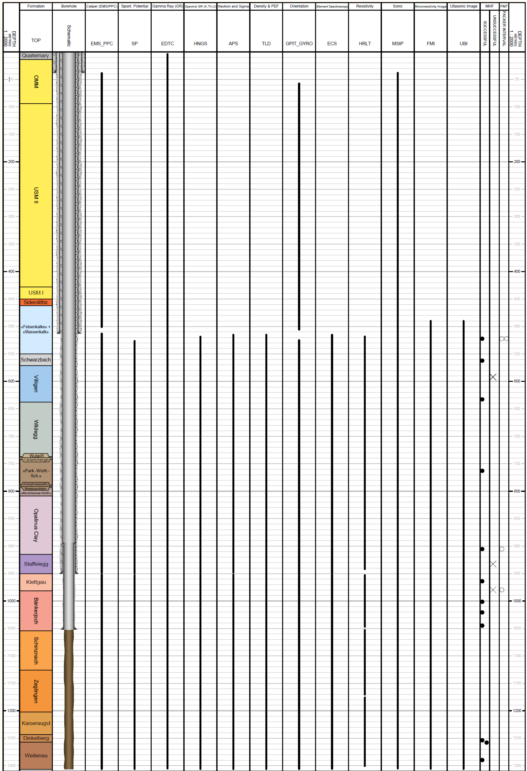
Fig. 2-1: Petrophysical log, MHF and PMT testing coverage at BAC1-1 (scale of 1:2'000)
