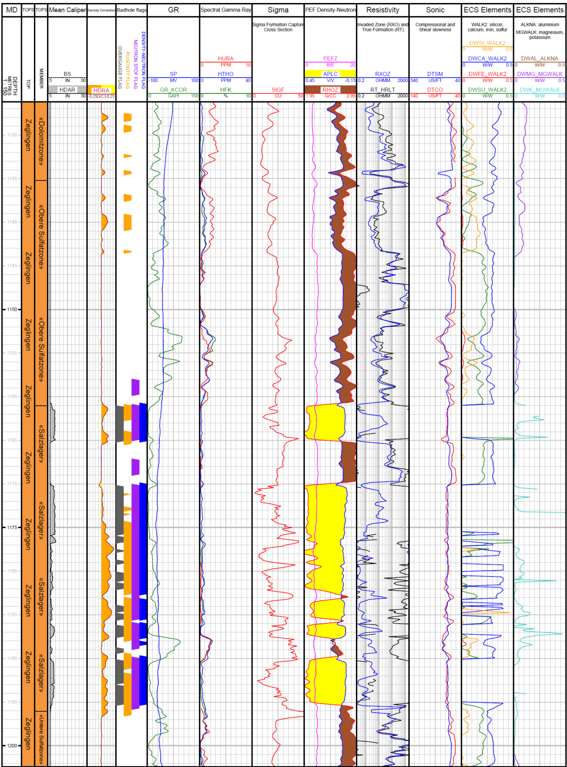
Fig. 3-8: Main logs of the composite dataset in the Zeglingen Formation
