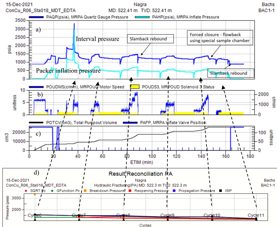
Fig. 5-2: Example of pressure record for MHF test from BAC1-1 (Station 4-1, Run 2.4.2)
