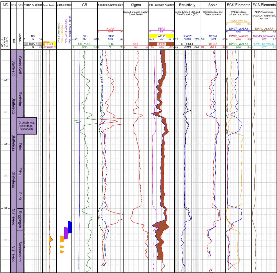
Fig. 3-4: Main logs of the composite dataset in the Staffelegg Formation
