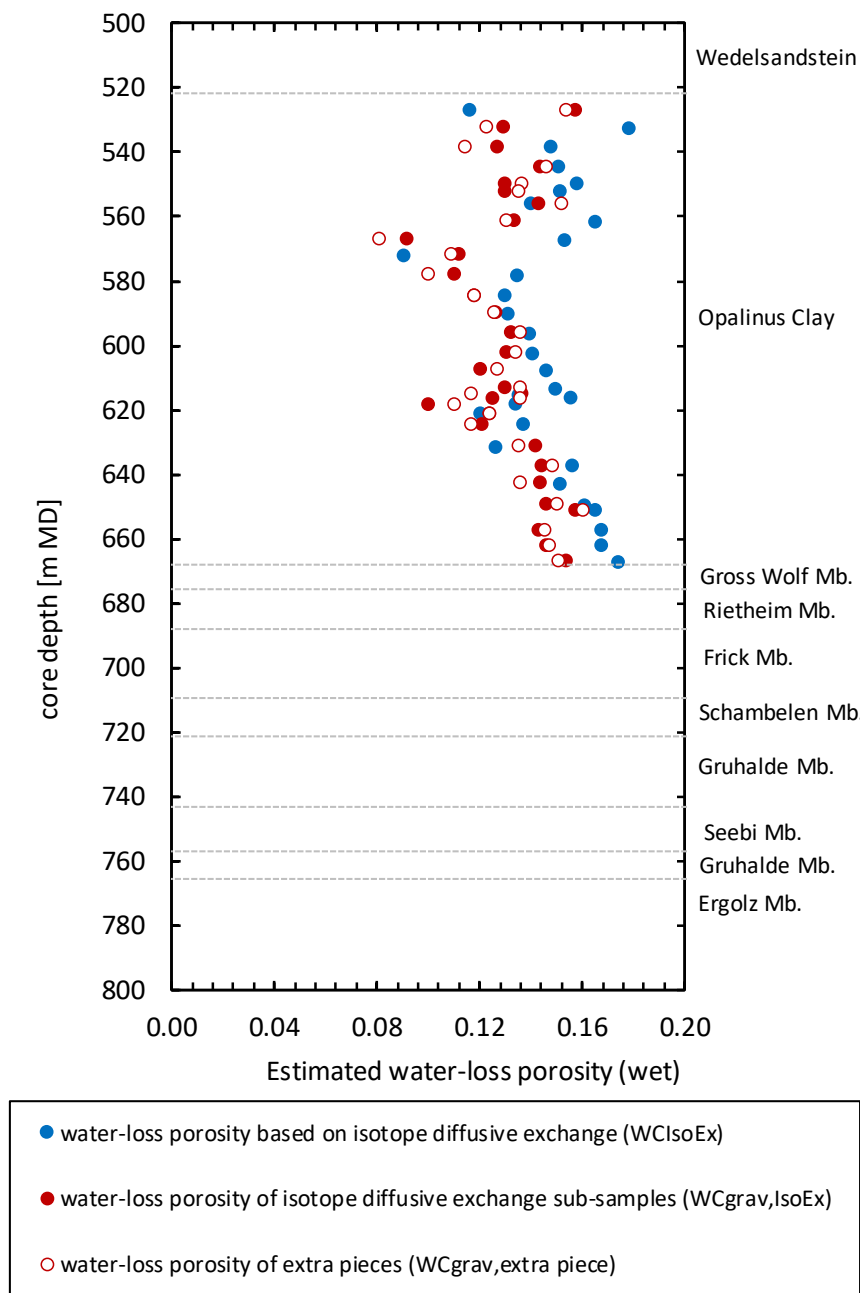
Fig. 3-3: Estimated water-loss porosity as a function of depth
