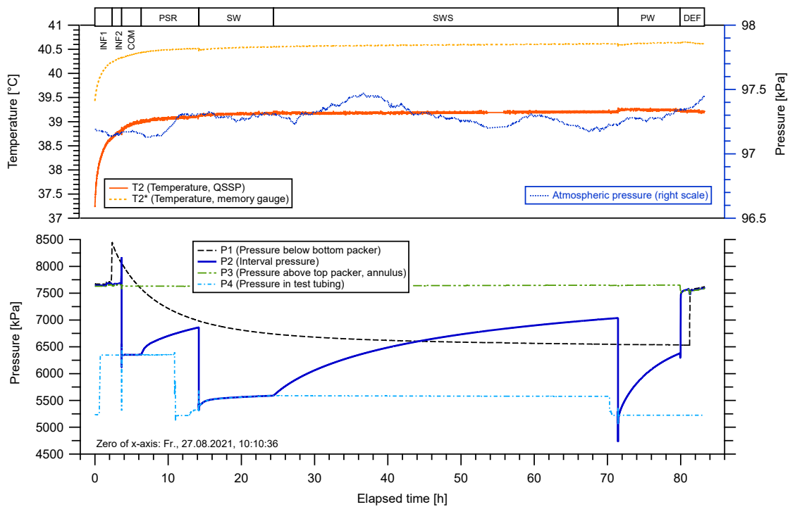
Fig. B-3: Hydraulic test RHE1-1-LIA1: Interval temperature ( T2^* memory gauge sensor), atmospheric pressure and downhole pressures of QSSP sensors (P1, P2, P3, P4) as well as temperature measurement at the QSSP ( T2 sensor)
