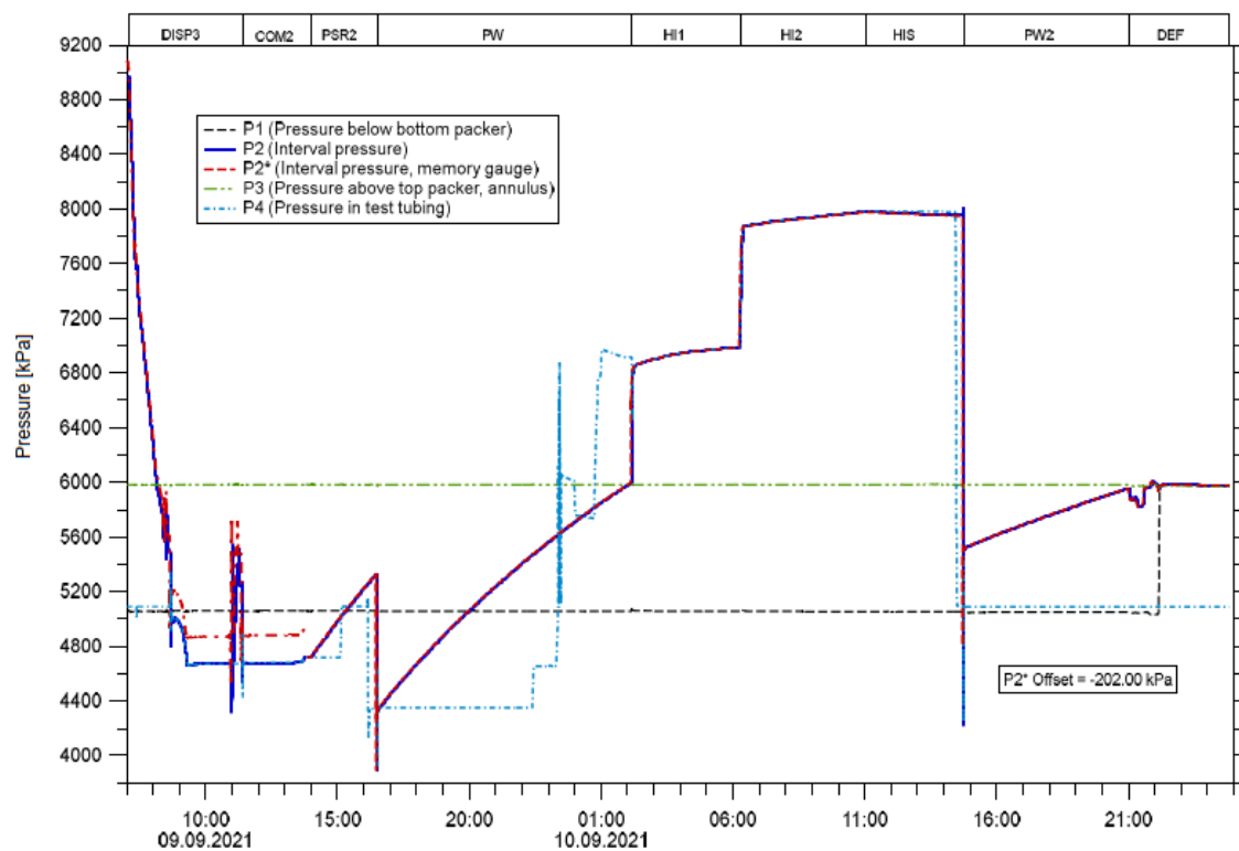
Fig. 3-11: Hydraulic packer test RHE1-1-OPA1c: Overview plot of pressure vs. time and date
