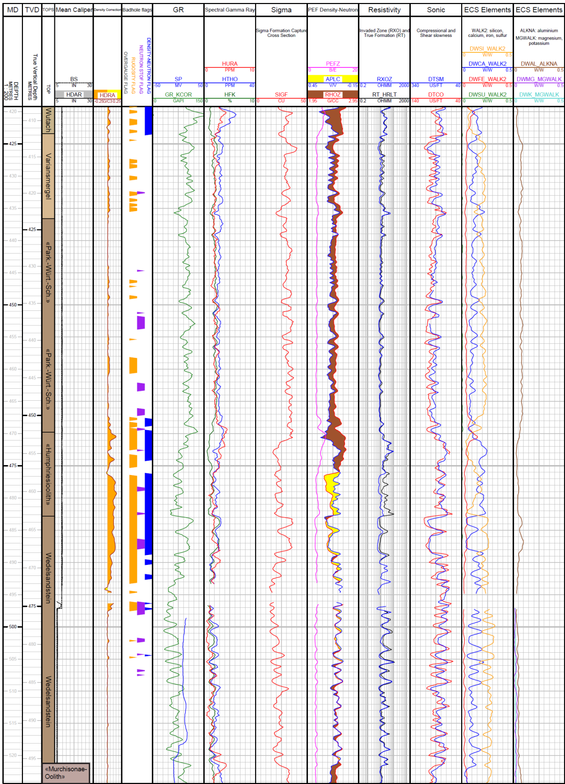
Fig. 3-3: Main logs of the composite dataset in the Wutach Formation to «Murchisonae-Oolith Formation»
