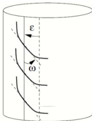
Fig. 5-2: Angles characterising 'en-échelon' fracture geometry at the wall of a deviated borehole
