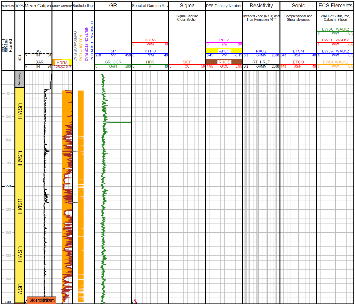
Fig. 3-1: Main logs of the composite dataset in the Cenozoic units
