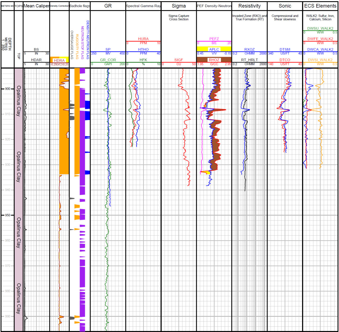
Fig. 3-4: Main logs of the composite dataset in the Opalinus Clay
