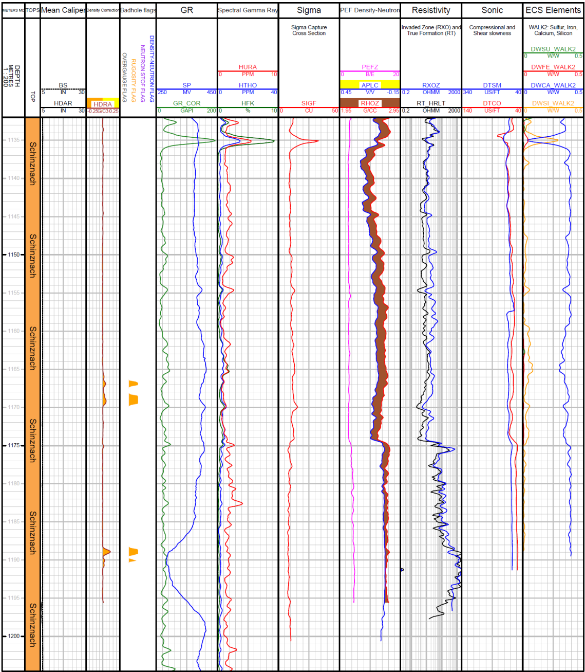
Fig. 3-7: Main logs of the composite dataset in the Schinznach Formation
