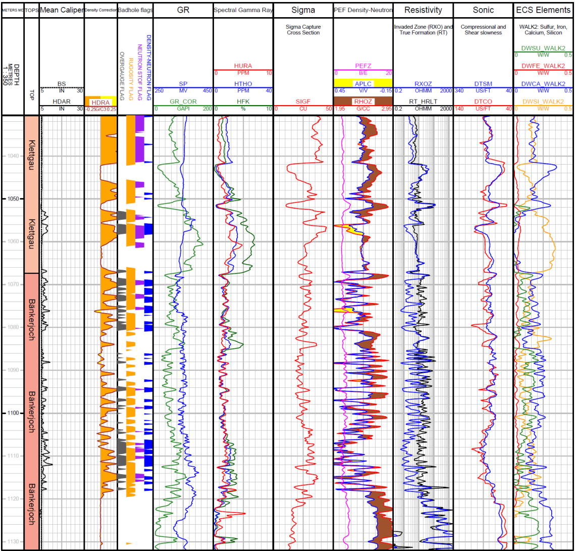
Fig. 3-6: Main logs of the composite dataset in the Klettgau and Bänkerjoch Formations
