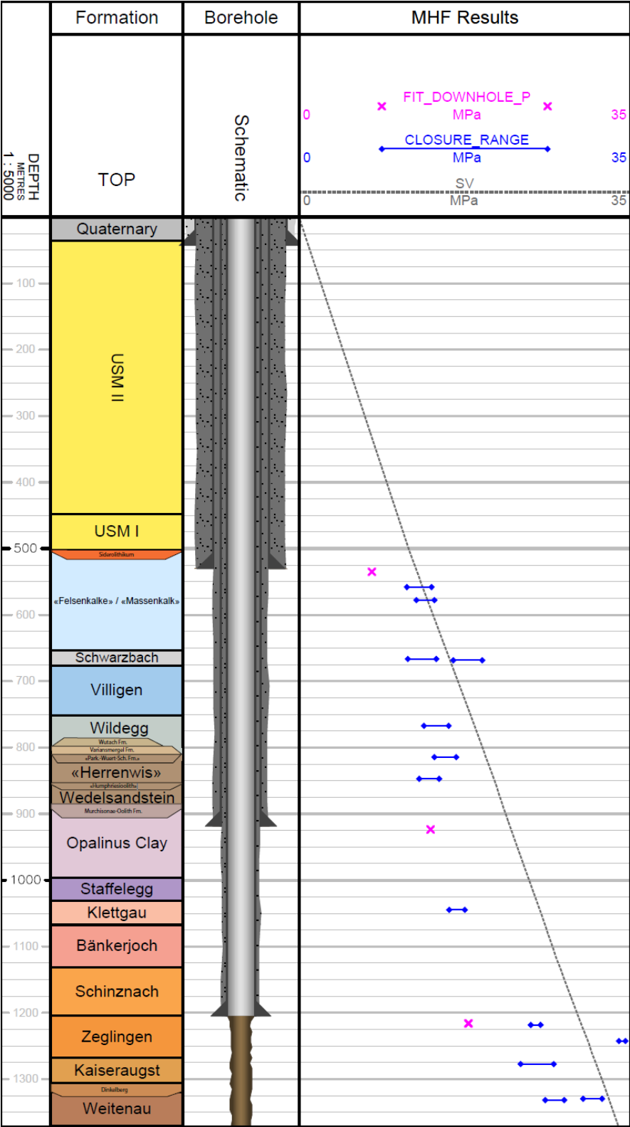
Fig. 5-4: Comparison of the quicklook closure stress range obtained from the MHF tests with the overburden vertical stress (Sv) from the integration of density over depth and the maximum pressures attained during the formation integrity tests (FIT)
