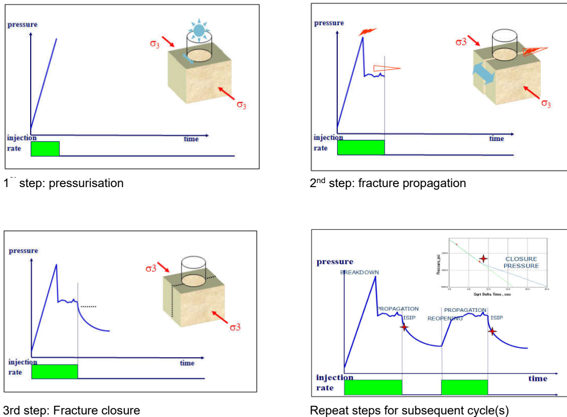
Fig. 5-1: Schematic showing the response of the interval pressure to fluid injection in the interval as a function of time during an MHF test, and associated formation response
