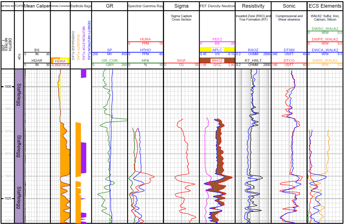
Fig. 3-5: Main logs of the composite dataset in the Staffelegg Formation
