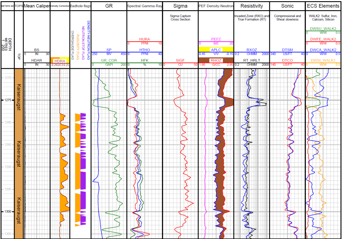
Fig. 3-9: Main logs of the composite dataset in the Kaiseraugst Formation
