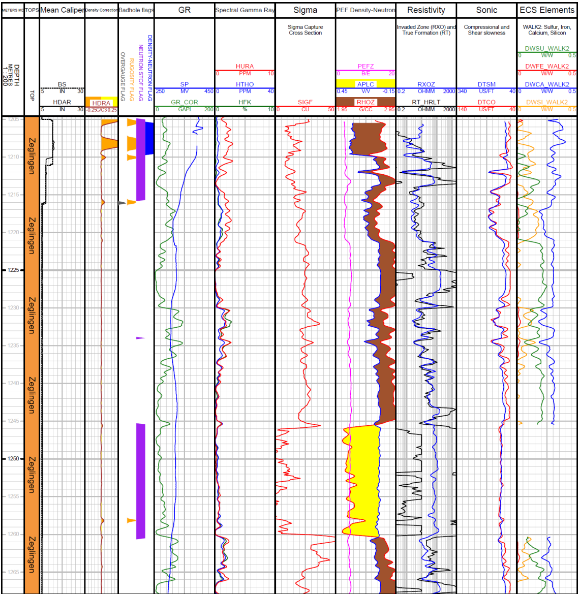
Fig. 3-8: Main logs of the composite dataset in the Zeglingen Formation
