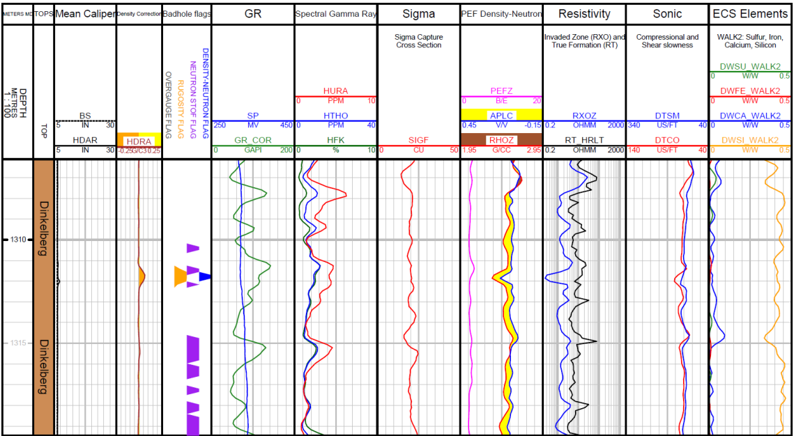
Fig. 3-10: Main logs of the composite dataset in the Dinkelberg Formation
