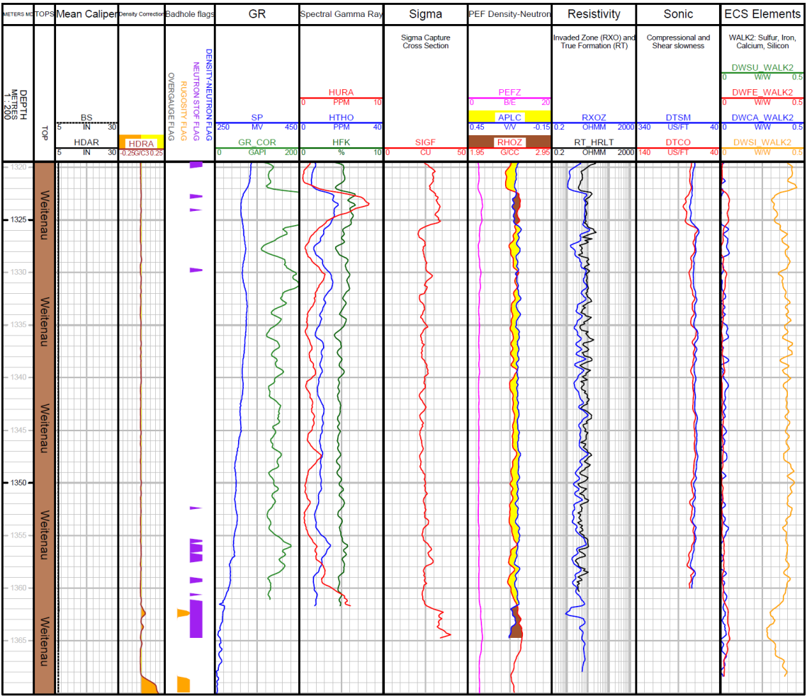
Fig. 3-11: Main logs of the composite dataset in the Weitenau Formation
