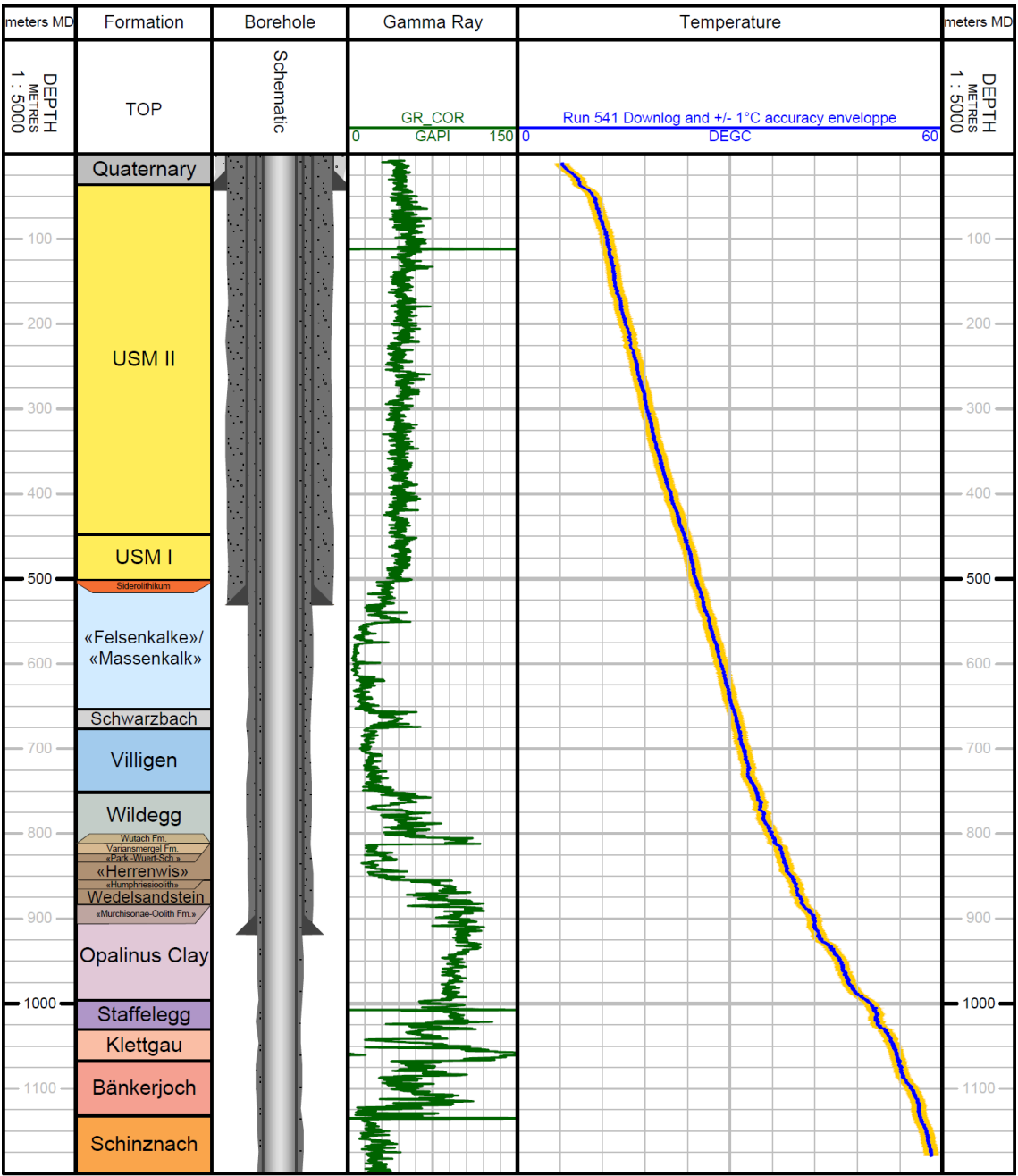
Fig. 3-12: Post-completion temperature log from the downlog pass of Run 5.4.1 (20.03.2021) A \pm 1^\circ\text{C} accuracy envelope is drawn in orange around the temperature log
