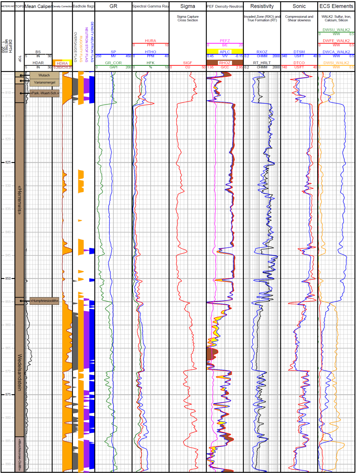
Fig. 3-3: Main logs of the composite dataset in the Wutach Formation to «Murchisonae-Oolith» unit
