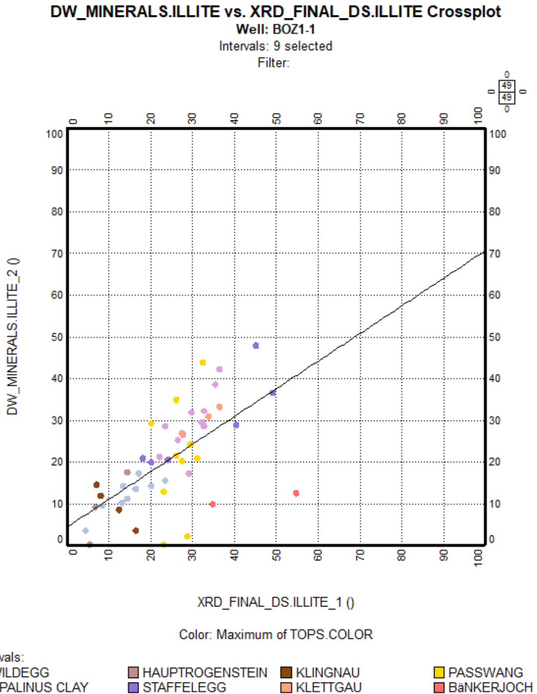
Fig. 4-3: Weight of illite (y-axis) compared to core XRD data (x-axis), XRD data in the Wildegg to Bänkerjoch Formation
