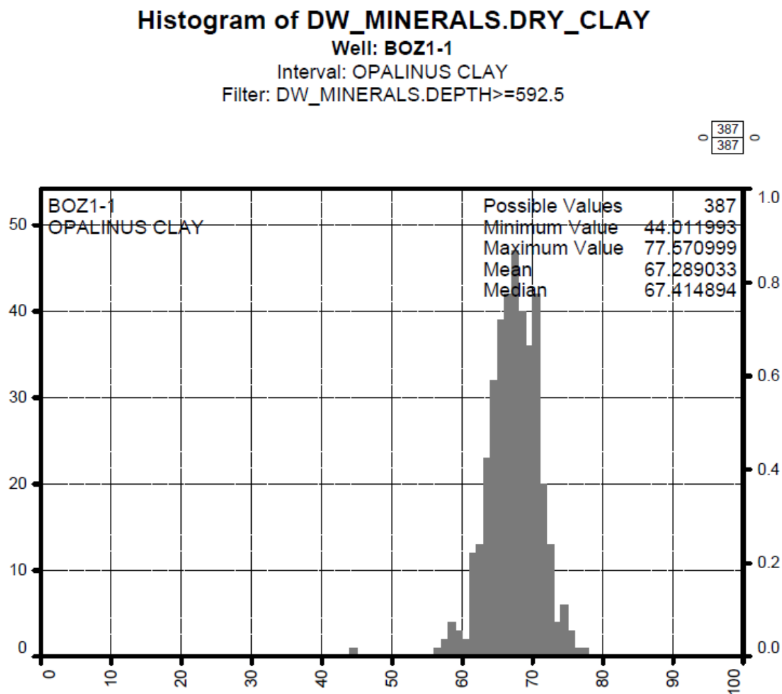
Fig. 4-10: Dry clay weight percentage frequency histogram in the lower section of Opalinus Clay (below 592.5 m)
