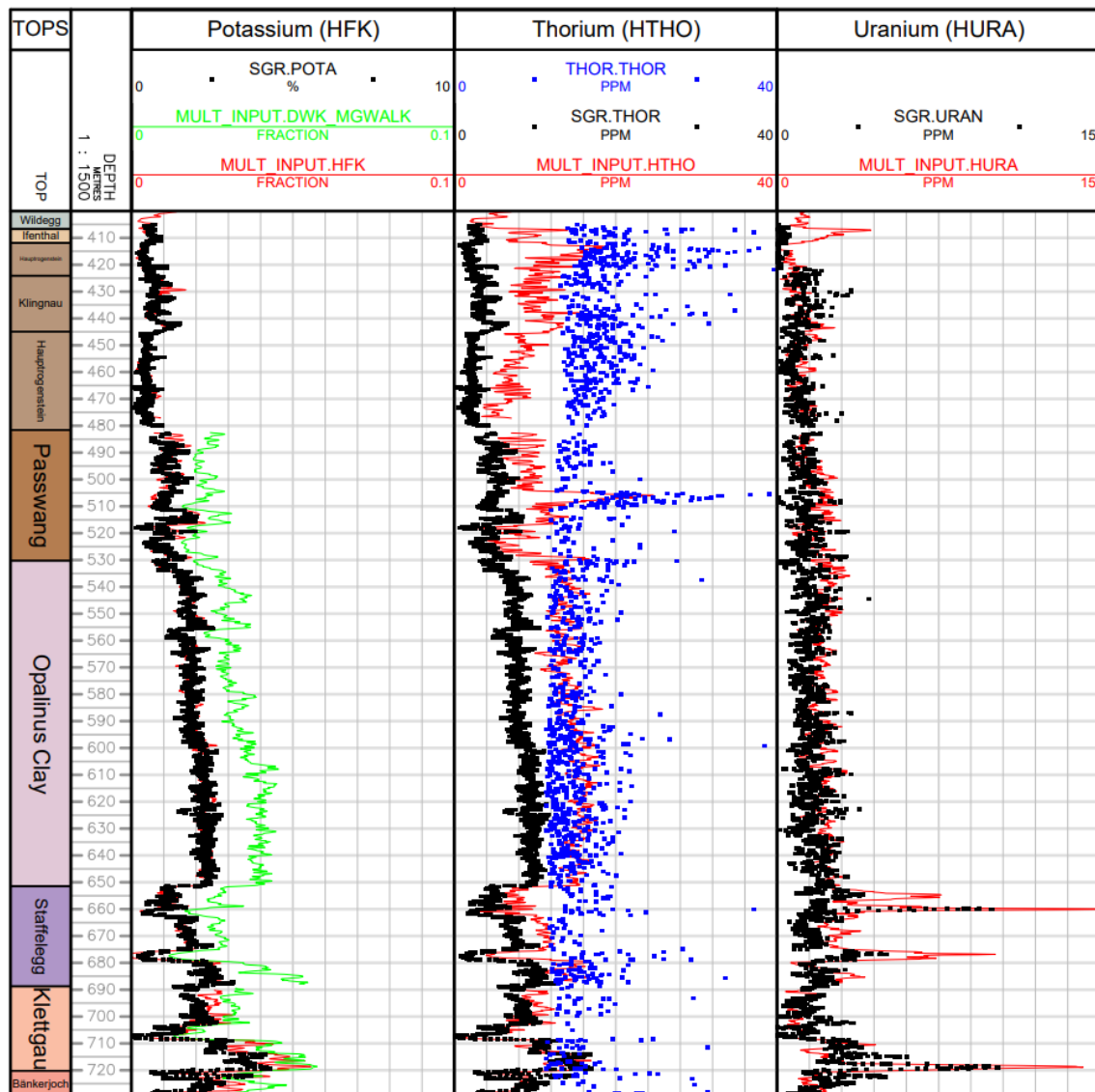
Fig. 2-3: Core (black dots: spectral gamma ray, blue dots XRF Thorium) and wireline HNGS (red curves) spectral gamma ray elements comparison
