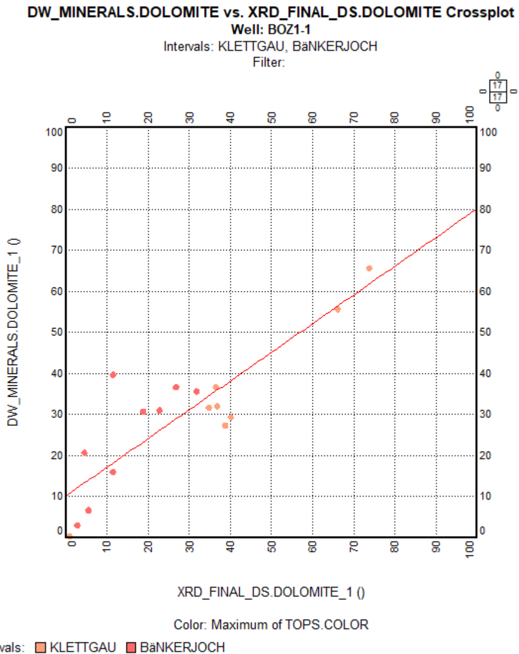
Fig. 4-6: Weight % of dolomite (y-axis) compared to core XRD data (x-axis), Klettgau and Bänkerjoch Formations
