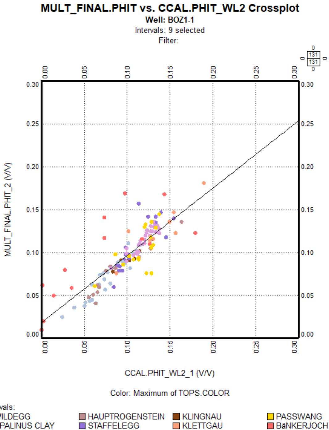
Fig. 4-7: Total porosity (v/v, y-axis) compared to core data (x-axis), Wildegg to Bänkerjoch Formation
