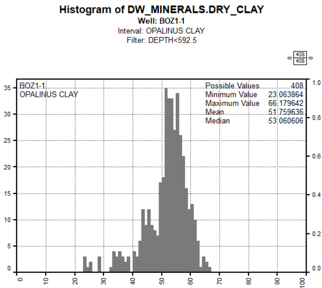
Fig. 4-9: Dry clay weight percentage frequency histogram in the upper section of Opalinus Clay (above 592.5 m)
