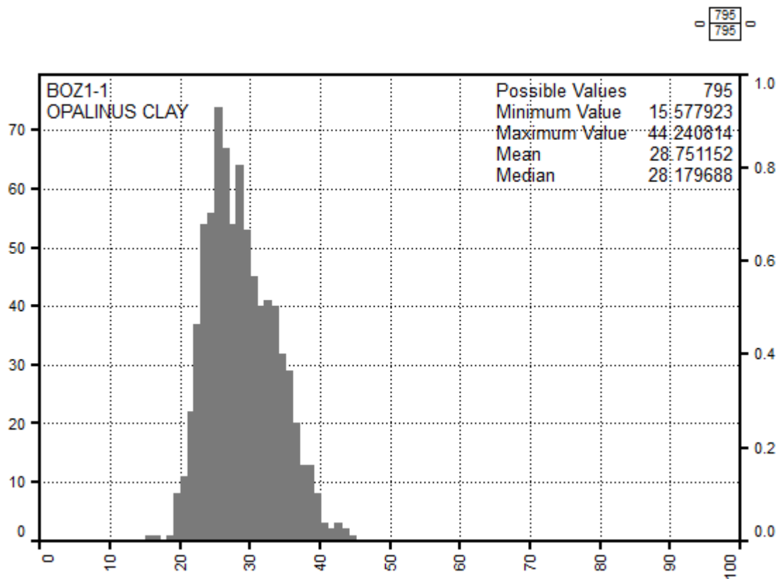
Fig. 4-13: QF-silicates (quartz and feldspars) weight percentage frequency histogram in the Opalinus Clay X-axis is the QF-silicates wt.-% from MultiMin, y-axis the number of points per bin (100 bins).
