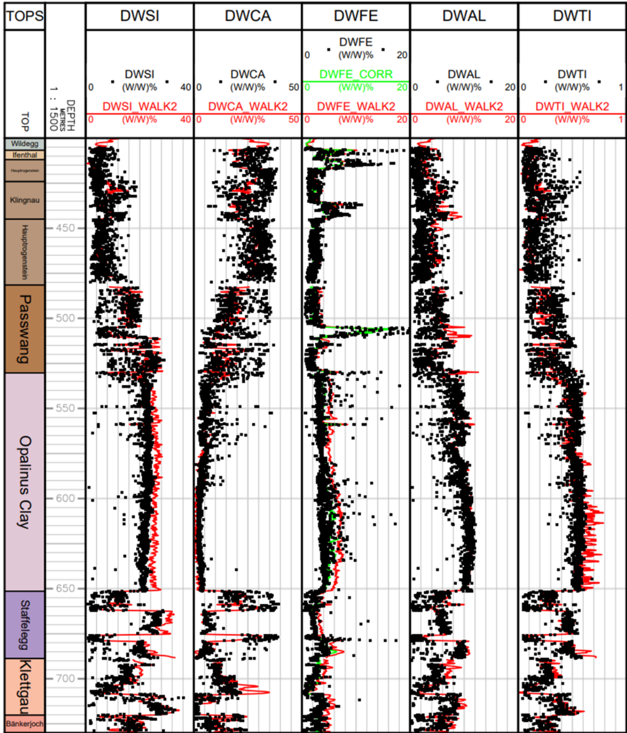
Fig. 2-2: XRF (black dots) and ECS WALK2 (red curves) elements comparison in BOZ1-1
