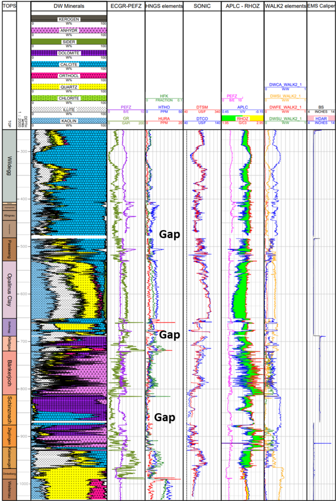
Fig. 2-1: Petrophysical log availability and gaps in the borehole BOZ1-1 Please note that ECS elements are displayed as measured (in weight/weight, 0 – 1 w/w range) and are not converted to wt.-% (weight percentage) here.
