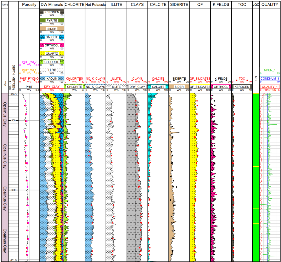
Fig. 4-15: Main log and core results in the Opalinus Clay The back line in the clay minerals track represents a 40% baseline. The wireline log quality was good in all the Opalinus Clay, as shown by the green LQC flag. The MultiMin quality curve always remains low, generally below 1.00, indicating an overall good curve prediction. The total porosity and the main minerals dry weight are well calibrated to the core XRD measurements. The siderite, K feldspars, chlorite endmembers and TOC calibration are less accurate. The whole Opalinus Clay is very argillaceous, almost always above 40 wt.-% (black line in the "Clay" minerals track in Fig. 4-15).
