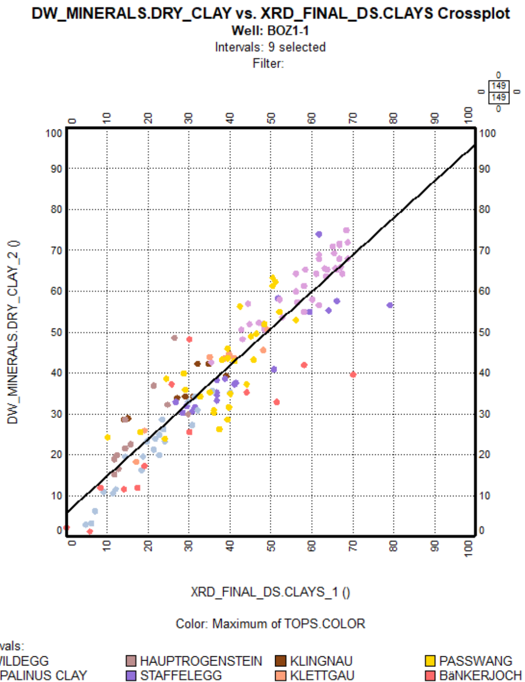
Fig. 4-1: Weight % of dry clay (y-axis) compared to core XRD data (x-axis), Wildegg to Bänkerjoch Formation
