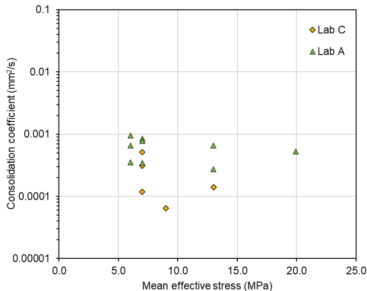
Fig. 6-5: Consolidation coefficient for Opalinus Clay specimens (all geometries)
