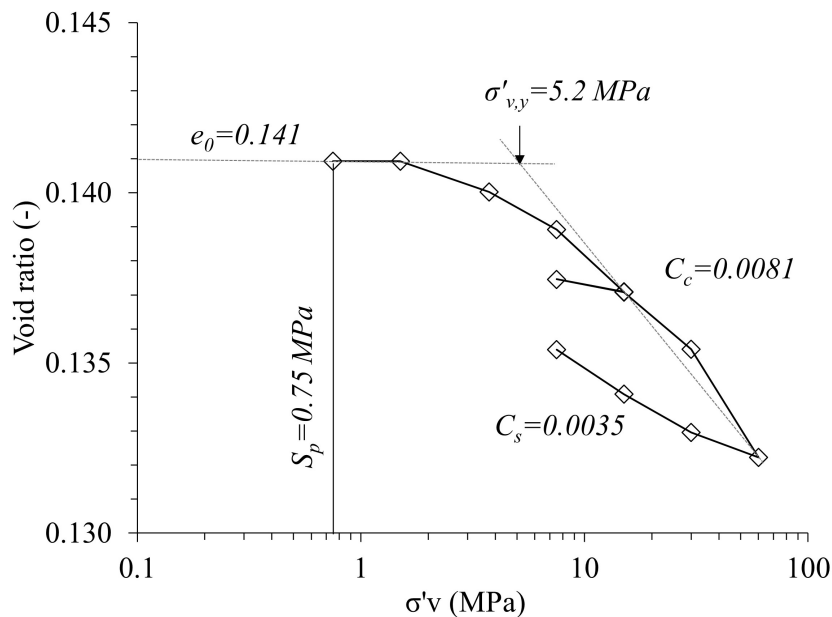
Fig. 6-19: Oedometric curve in void ratio versus vertical effective stress plane
