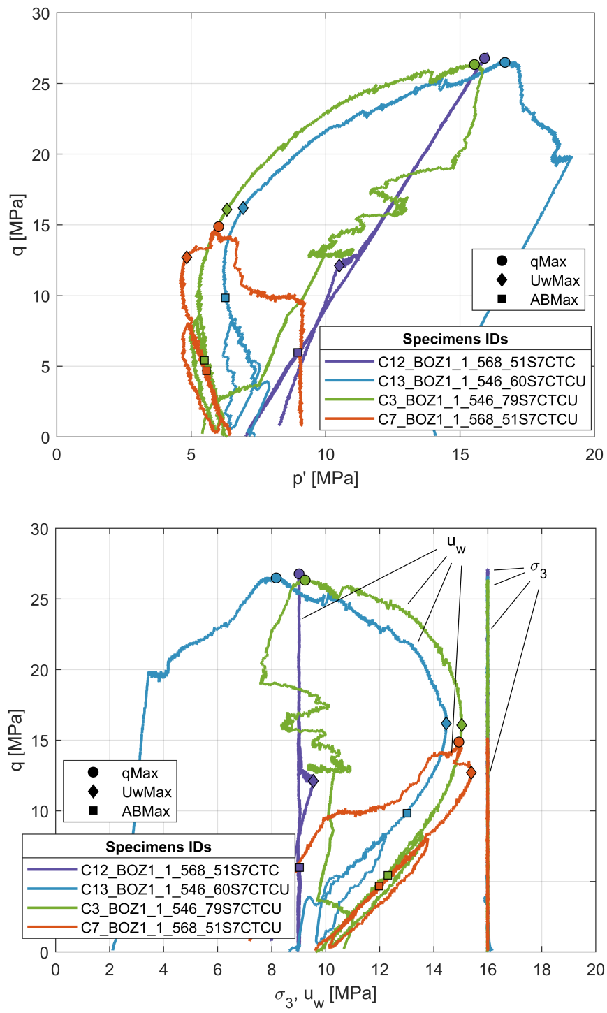
Fig. 6-18: Stress path (top), pore pressure and radial stress (bottom) of test C7_BOZ1_1_568_51S7CTCU: comparison with other test results
