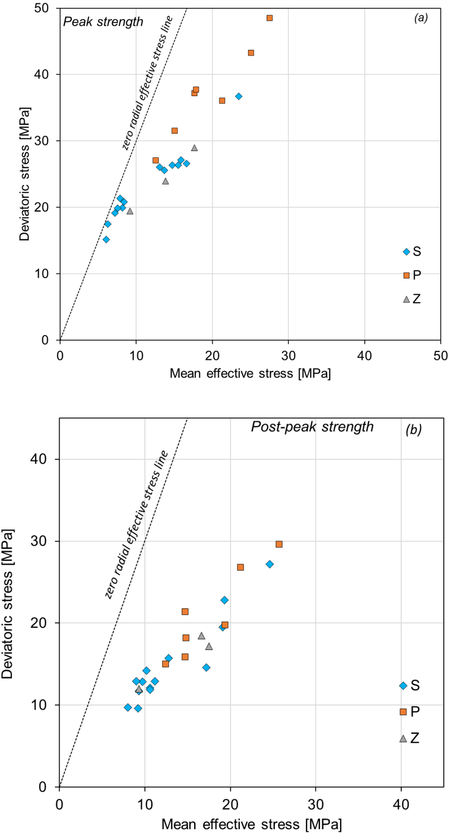
Fig. 6-13: Peak (a) and post-peak (b) shear strength of Opalinus Clay BOZ1-1 specimens Results divided by geometry.
