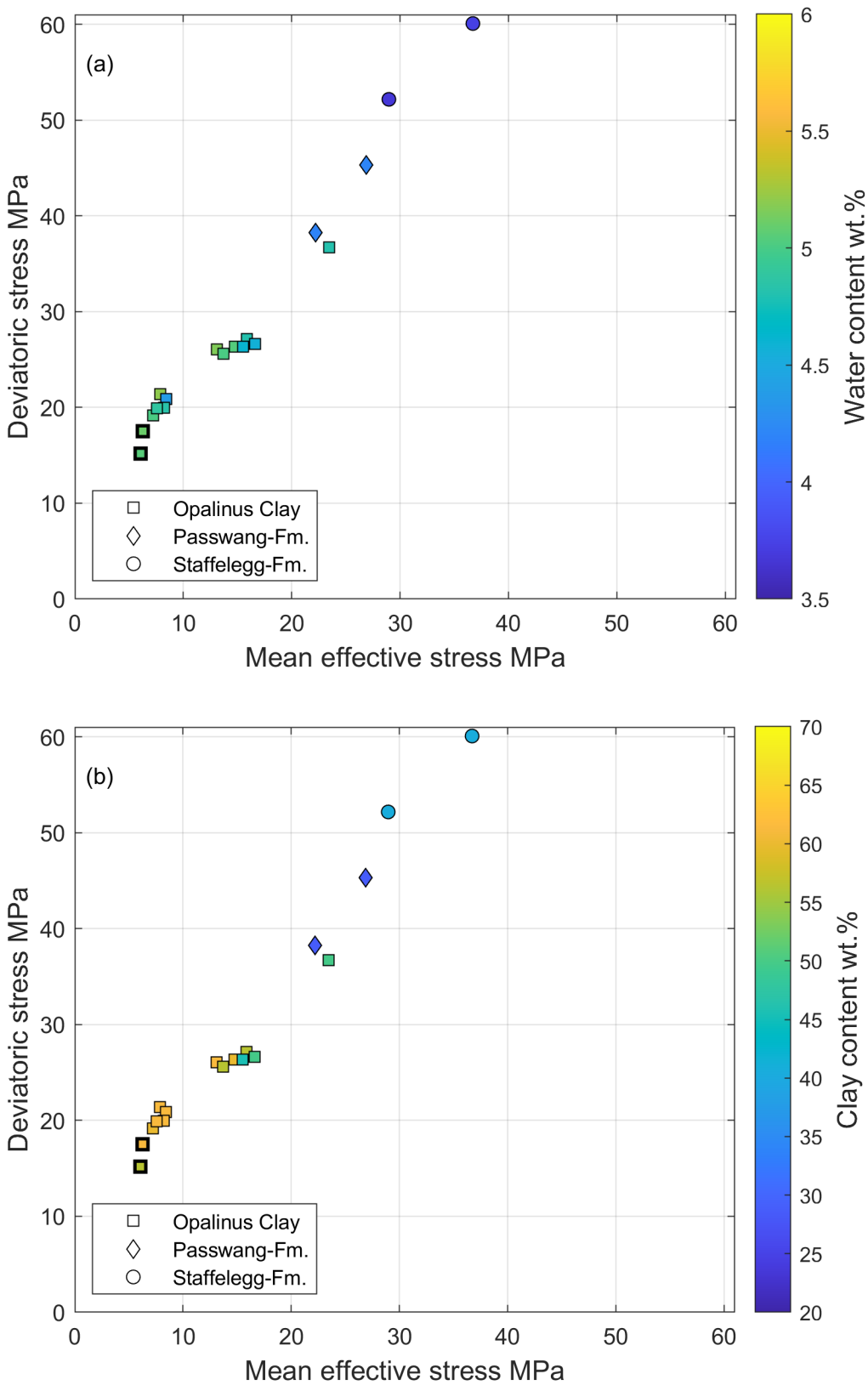
Fig. 6-14: Peak shear strength of specimens, Opalinus Clay and confining units
