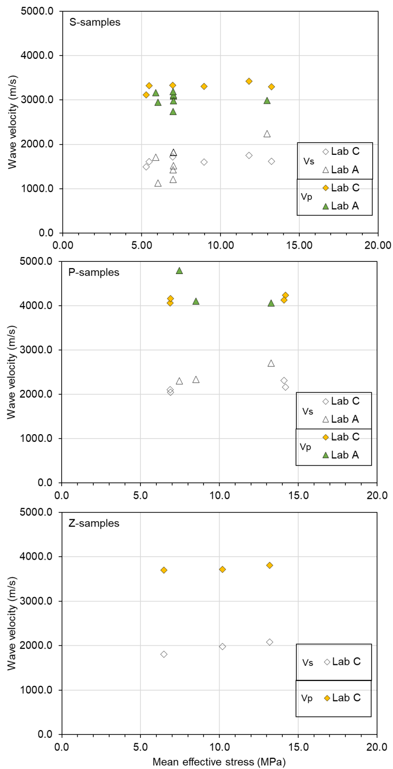
Fig. 6-11: Wave velocities at the beginning of the shearing phase Results are divided by specimen geometry (data in Appendix E).
