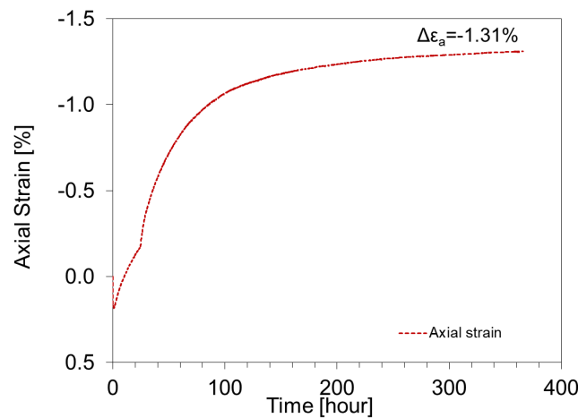
Fig. 6-21: One-dimensional swelling test, evolution of the axial strain in time Results obtained on specimen A01OS_BOZ1_1, constant axial stress of 0.1 MPa applied.
