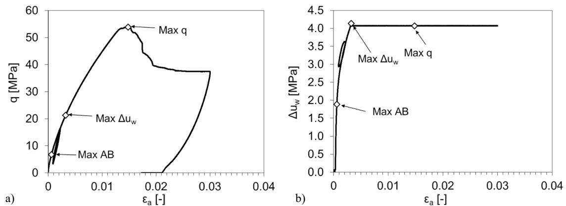
Fig. 5-2: Examples of problematic pore pressure during testing
