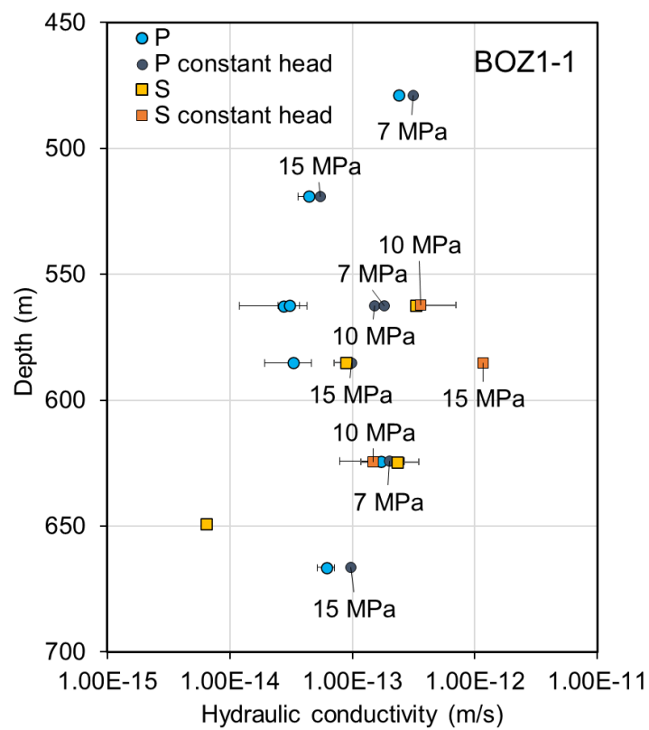
Fig. 6-20: Hydraulic conductivity versus depth
