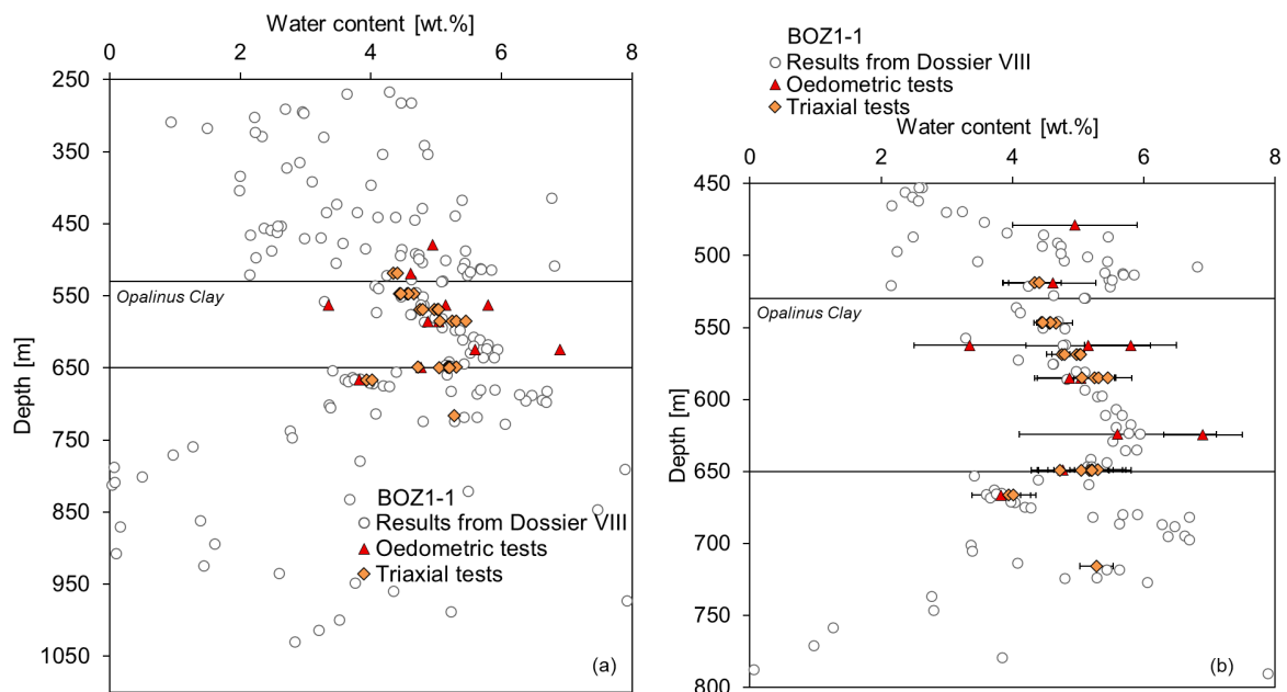
Fig. 7-2: Water content vs. depth from the large database and from specimens tested in this report
