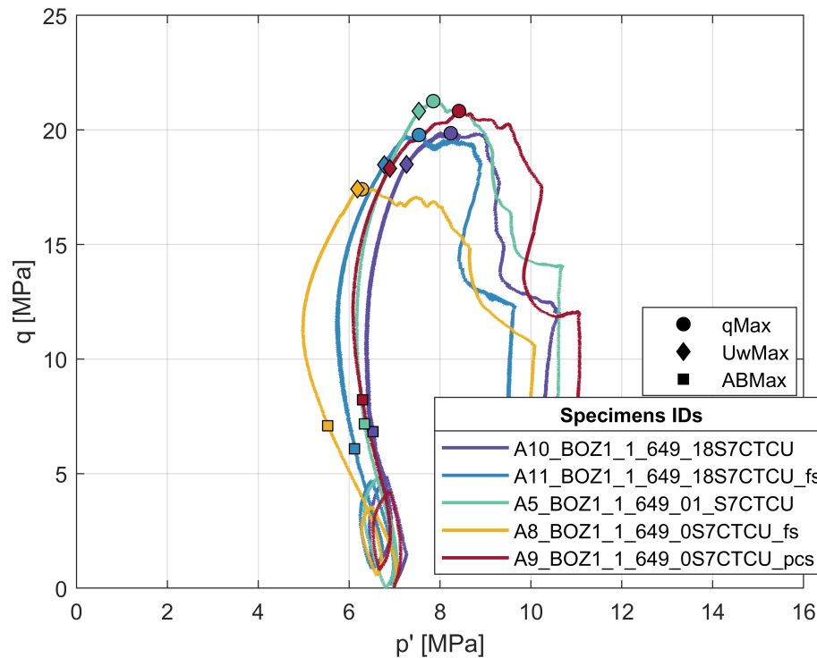
Fig. 6-17: Stress paths of samples from lab A, with various saturation procedures
