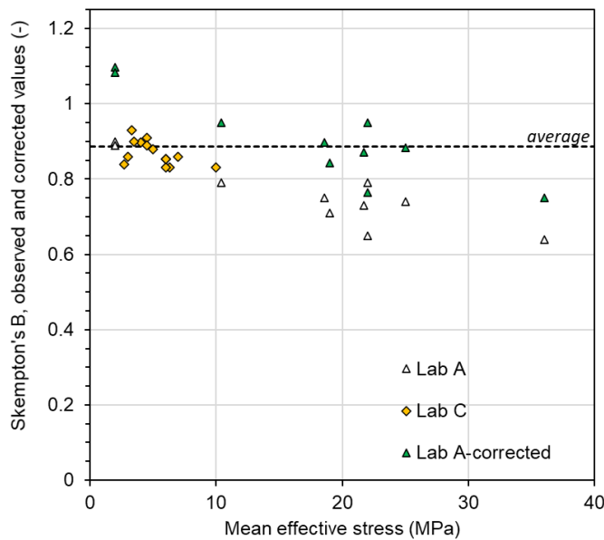
Fig. 6-4: Average Skempton's B values
