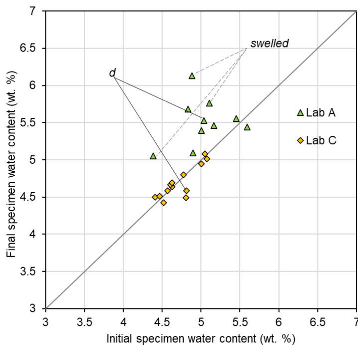
Fig. 6-1: Initial versus final water content of triaxial specimens (Opalinus Clay)
