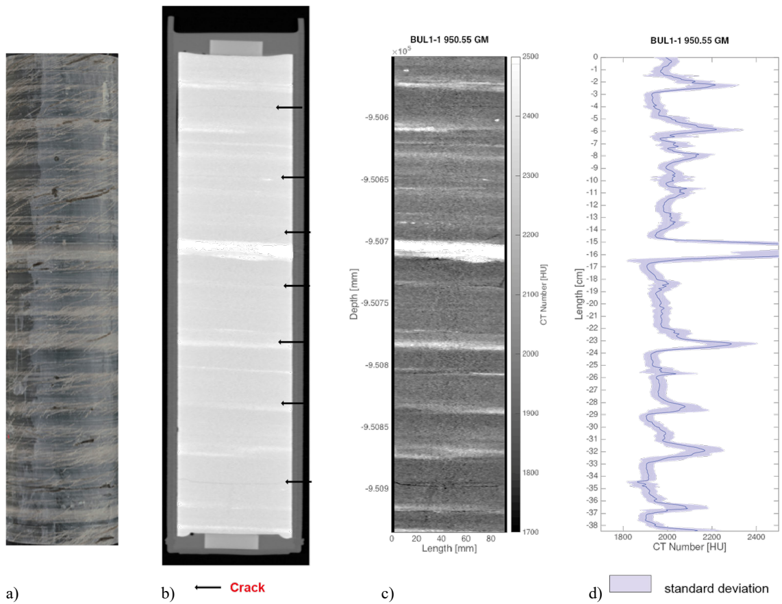
Fig. 3-2: Cross-section of XCT stack
