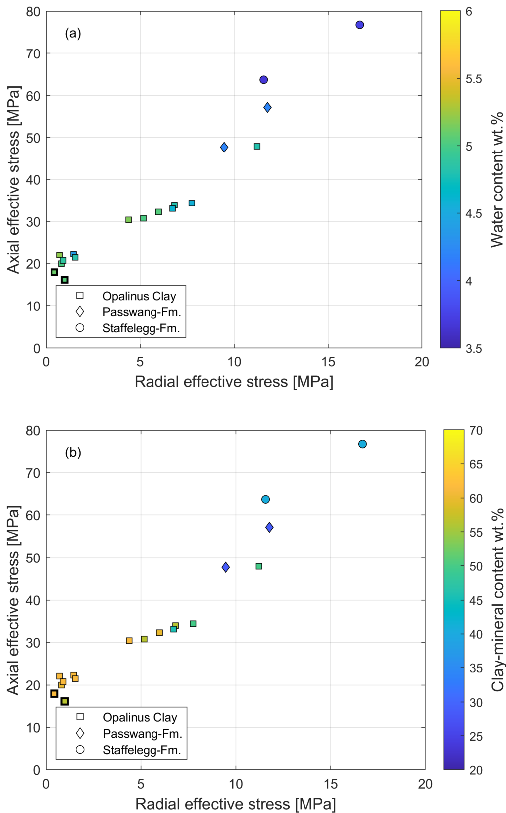
Fig. 6-15: Peak shear strength of specimens, Opalinus Clay and confining units
