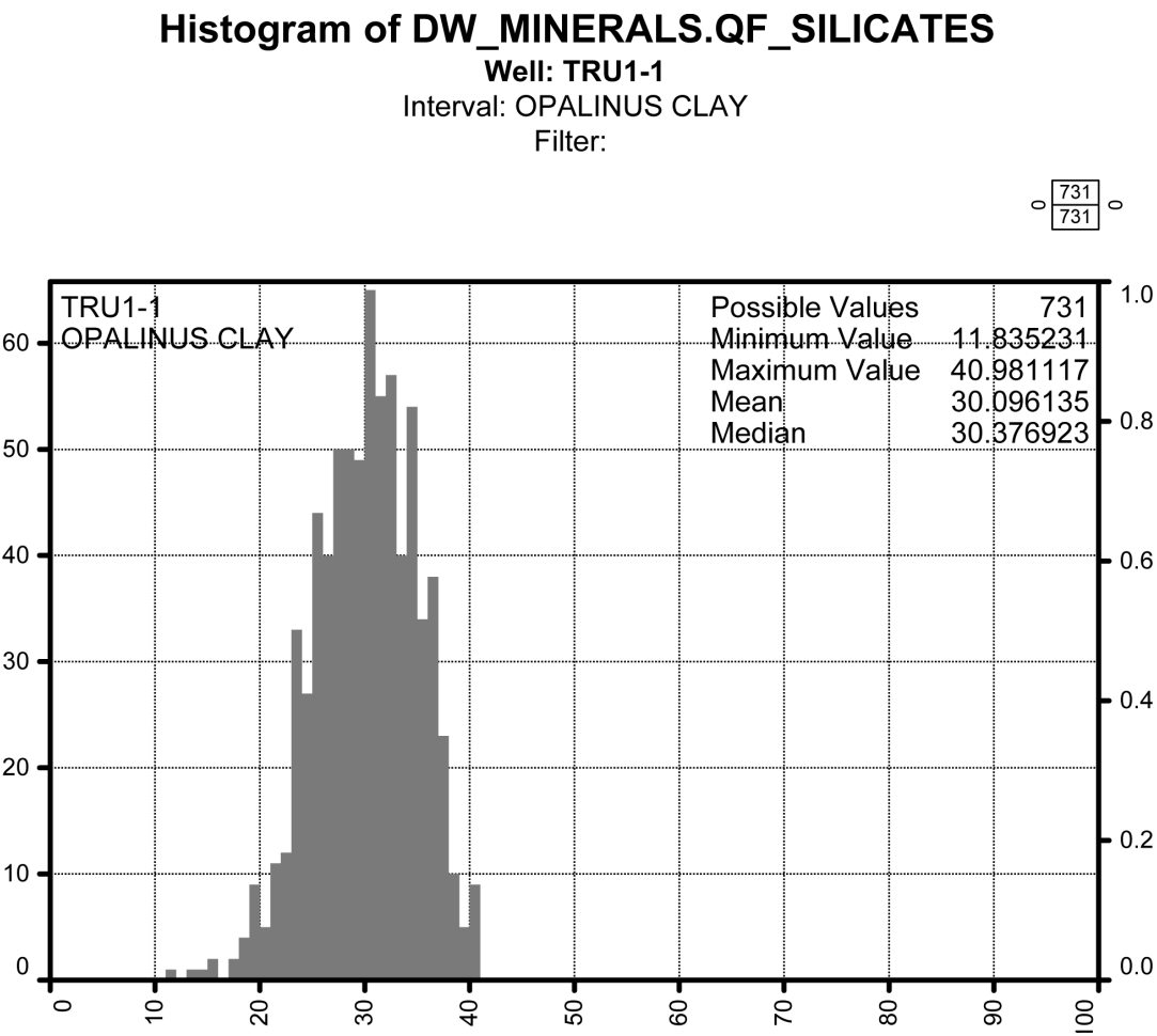
Fig. 4-13: QF-silicates (quartz and feldspars) weight percentage frequency histogram in the Opalinus Clay X axis is the QF-silicates wt.-% from MultiMin, y axis the number of points per bin (100 bins).
