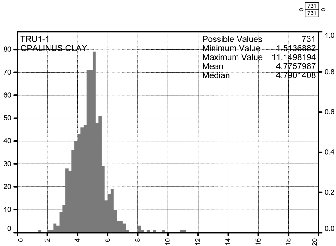
Fig. 4-12: Siderite weight percentage frequency histogram in the Opalinus Clay
