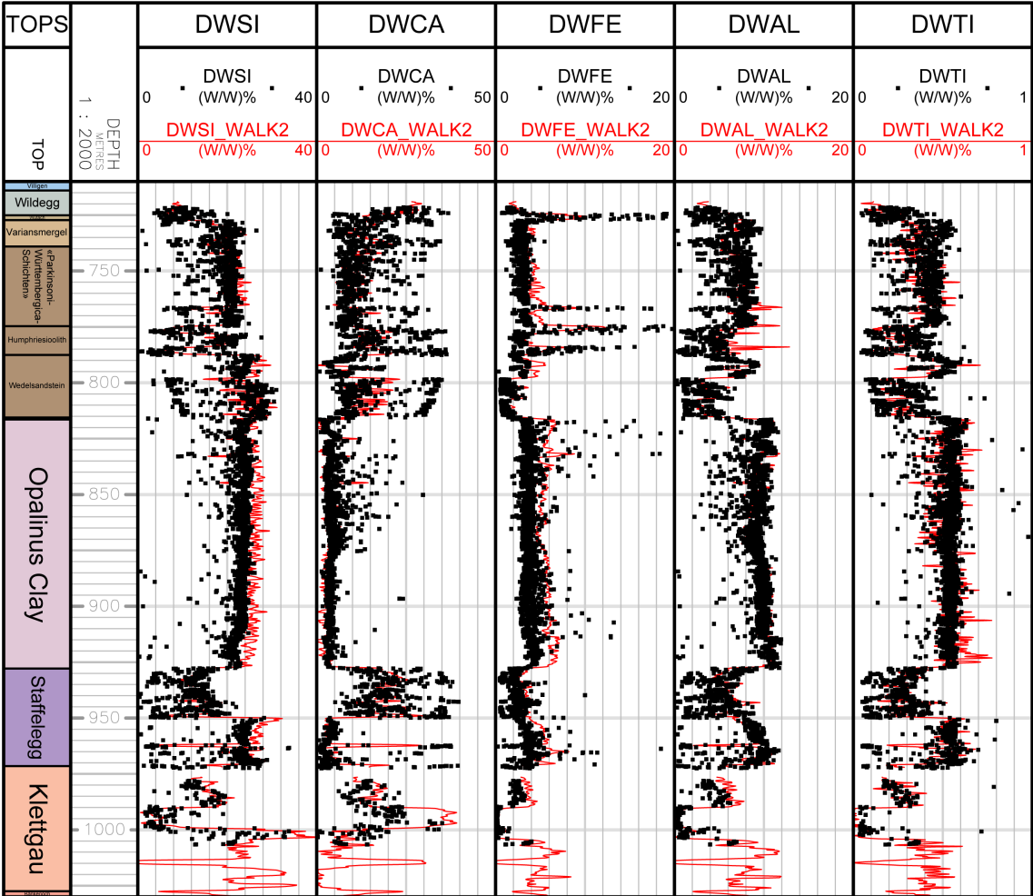
Fig. 2-2: XRF (black dots) and ECS (red curves) elements comparison
