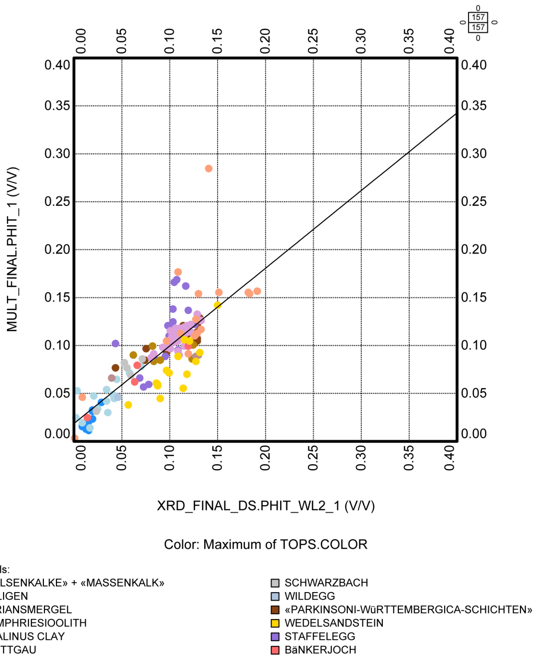
Fig. 4-7: Total porosity (v/v, y axis) compared to core data (x axis) («Felsenkalke» + «Massenkalk» to the Bänkerjoch Formation)
