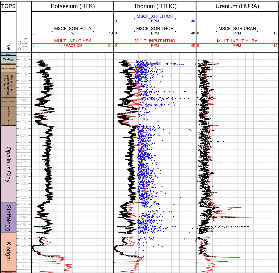
Fig. 2-3: Core (black dots: spectral gamma ray, blue dots XRF Thorium) and wireline HNGS (red curves) spectral gamma ray elements comparison Uranium from the XRF scanner was not measured because it was below the detection limit of the scanner.
