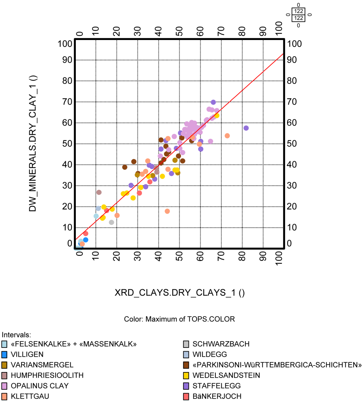
Fig. 4-1: Weight % of dry clay (y-axis) compared to core XRD data (x-axis) («Felsenkalke» + «Massenkalk» to the Schinznach Formation)
