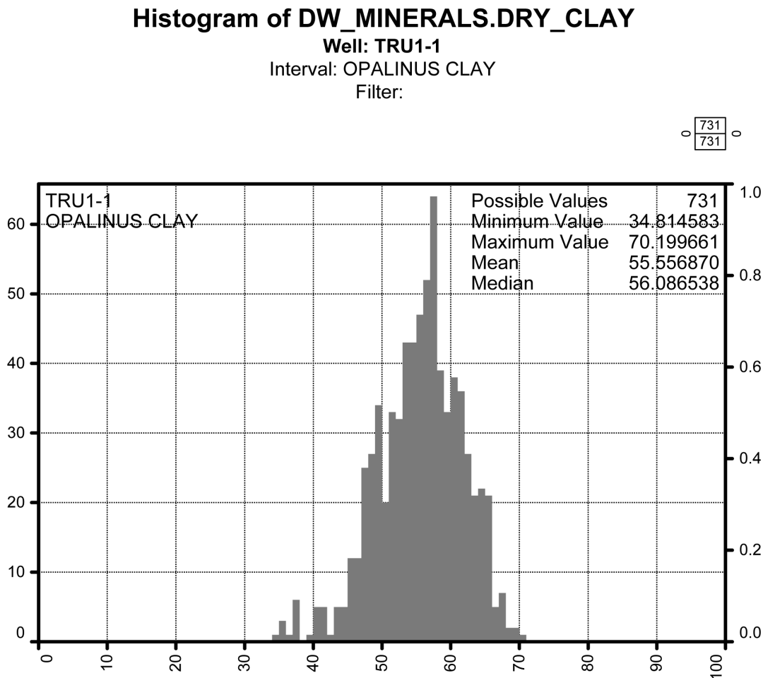
Fig. 4-8: Dry clay weight percentage frequency histogram in the Opalinus Clay X axis is the dry clay wt.-% from MultiMin, y axis the number of points per bin (100 bins).
