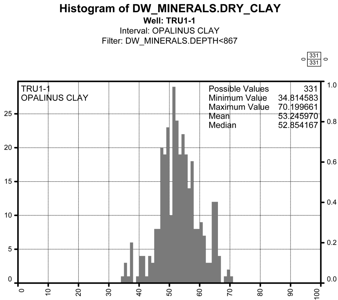
Fig. 4-9: Dry clay weight percentage frequency histogram in the upper section of Opalinus Clay (above 867 m) X axis is the dry clay wt.-% from MultiMin, y axis the number of points per bin (100 bins).
