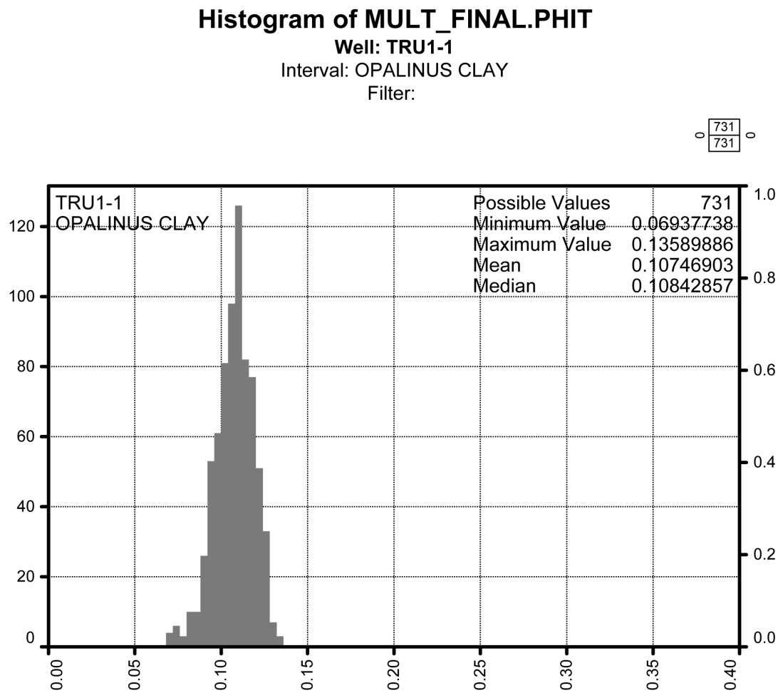
Fig. 4-14: Total porosity frequency histogram in the Opalinus Clay X axis is the total porosity v/v from MultiMin, y axis the number of points per bin (100 bins).
