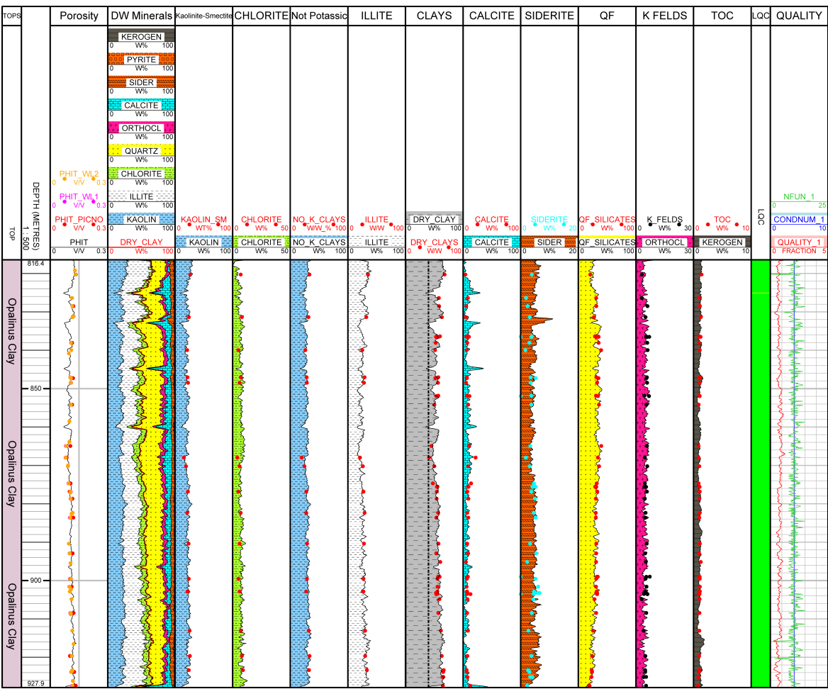
Fig. 4-15: Main log and core results in the Opalinus Clay
