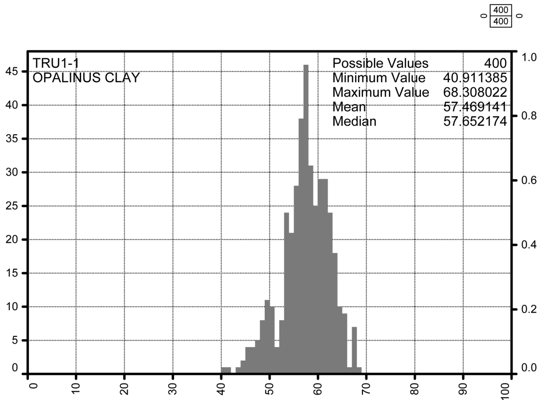
Fig. 4-10: Dry clay weight percentage frequency histogram in the lower section of Opalinus Clay (below 867 m)
