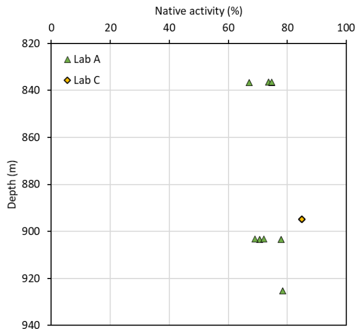
Fig. 6-2: Native activity of trimming versus depth of collection Results grouped by laboratory.
