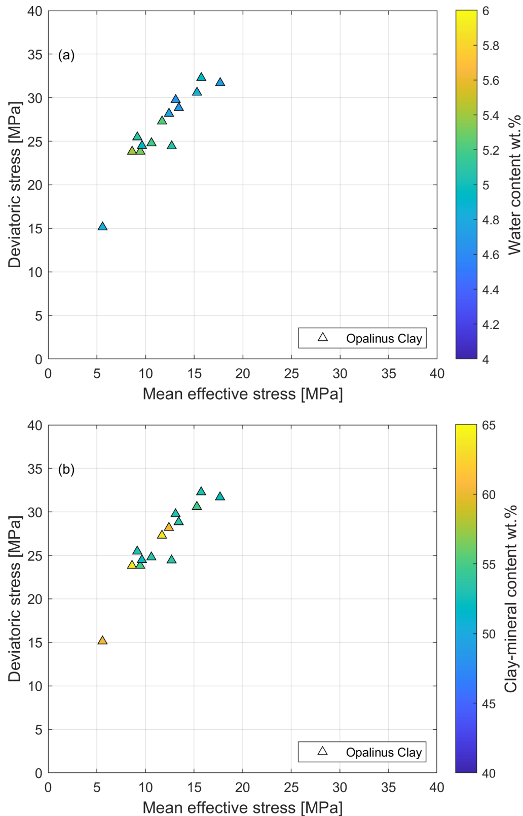
Fig. 6-14: Peak shear strength of specimens of Opalinus Clay and confining units
