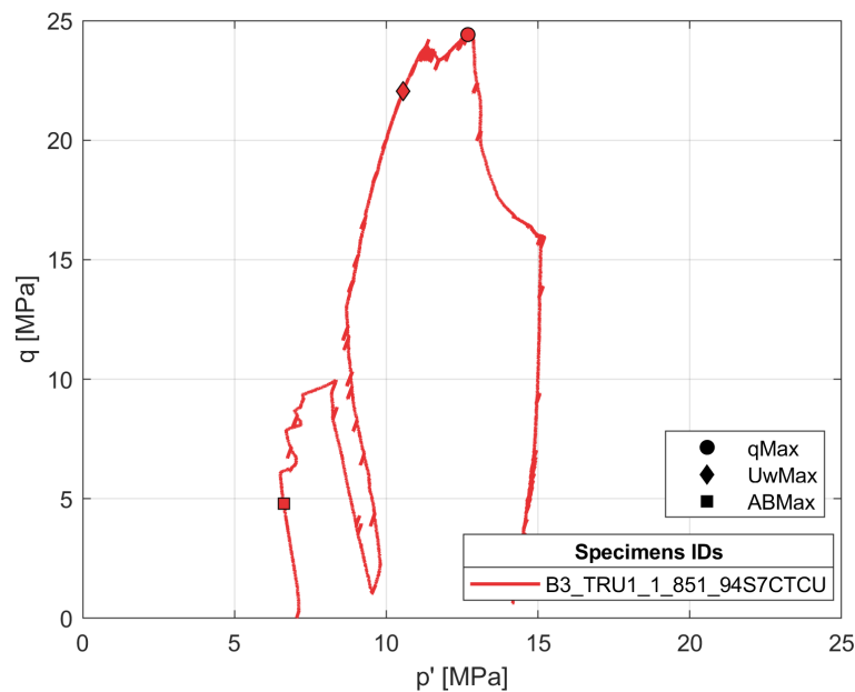
Fig. 6-20: Stress path of test B3_TRU1_1_851_94S7CTCU
