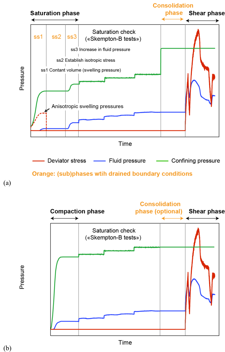
Fig. 4-6: Pressure-time sequences of triaxial deformation tests (specialised protocols) (a) conventional and (b) alternative testing procedures for undrained boundary conditions during the shear phase.
