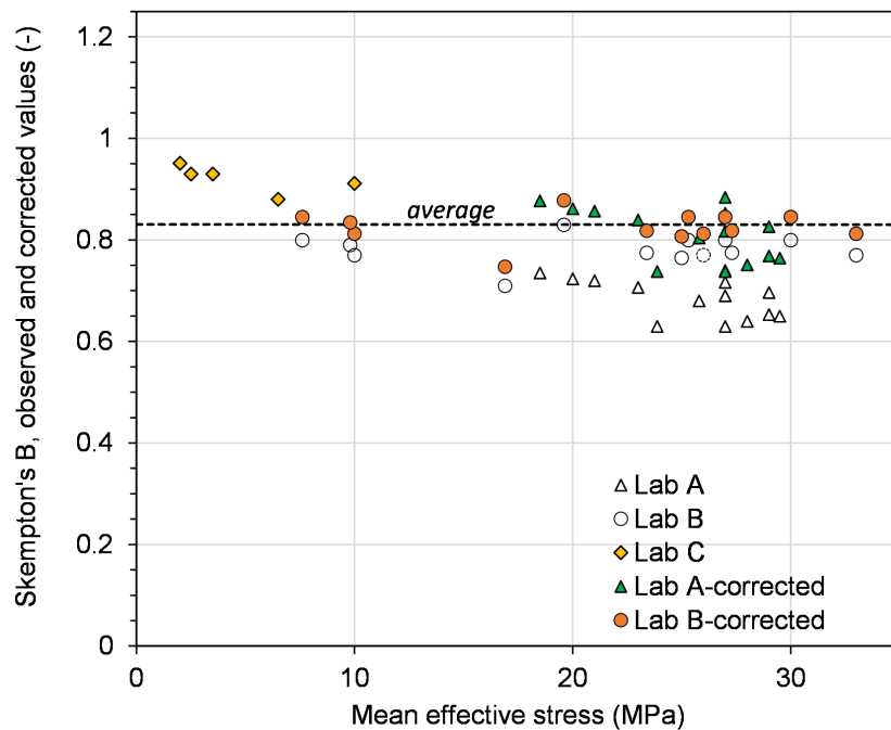
Fig. 6-4: Average Skempton's B values
