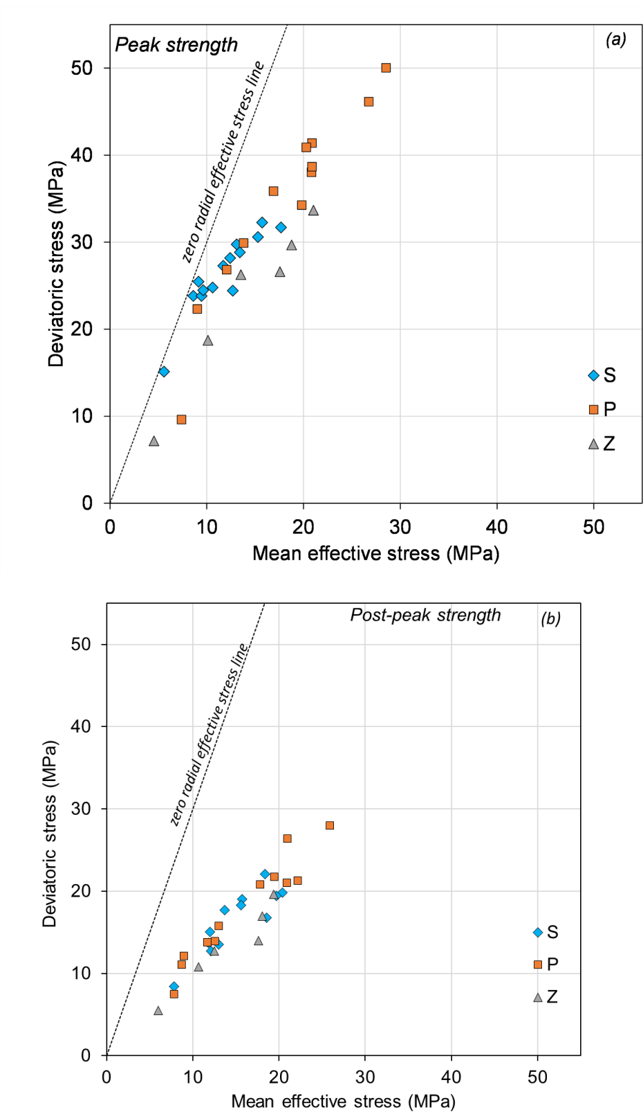
Fig. 6-13: Peak (a) and post-peak (b) shear strength of Opalinus Clay TRU1-1 specimens Results divided by geometry.
