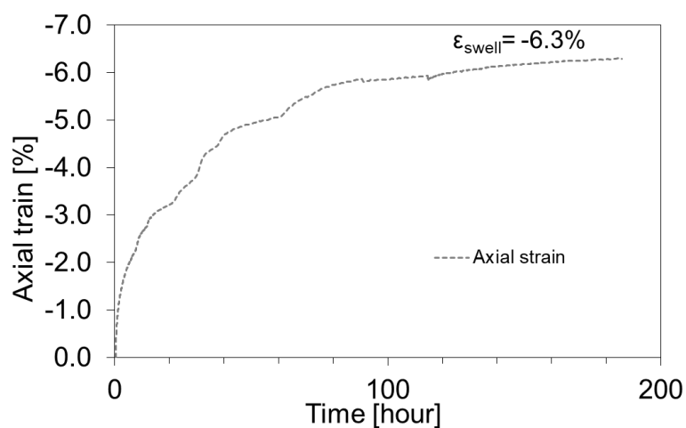
Fig. 6-26: One-dimensional swelling test, evolution of the axial strain in time Results obtained on specimen D01OS_TRU11.
