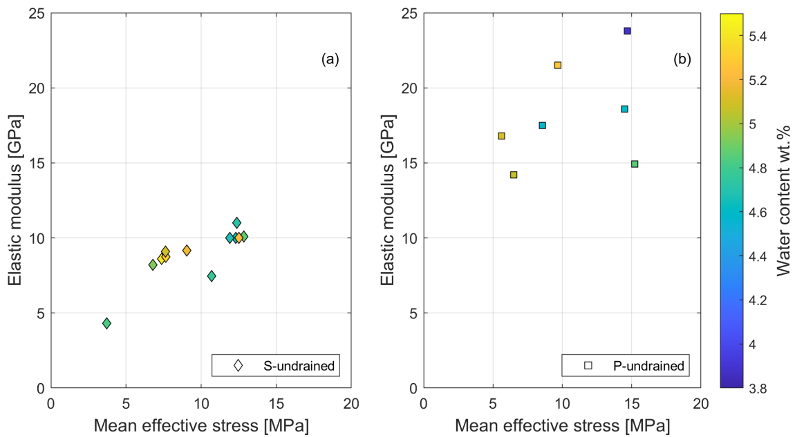
Fig. 6-9: Elastic undrained moduli, sorted by specimen final water content
