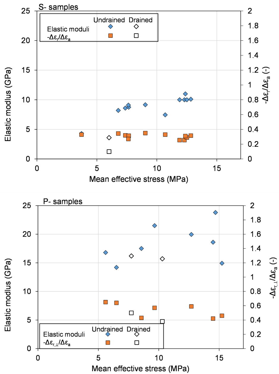
Fig. 6-10: Elastic drained and undrained properties
