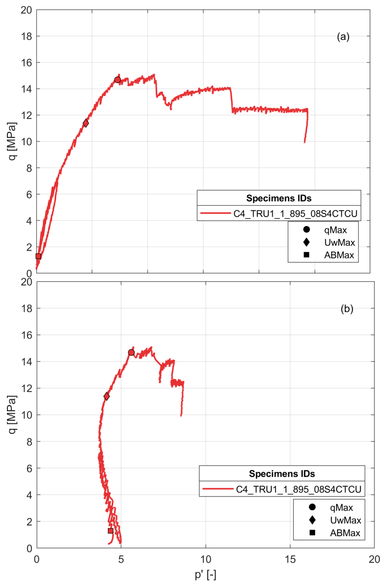
Fig. 6-22: Test C4_TRU1_1_895_08S4CTCU results
