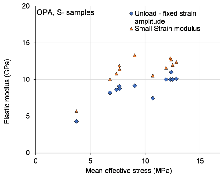
Fig. 6-8: Elastic undrained moduli calculated over an unloading (UL) path: modulus of a fixed strain interval and small strain extrapolation
