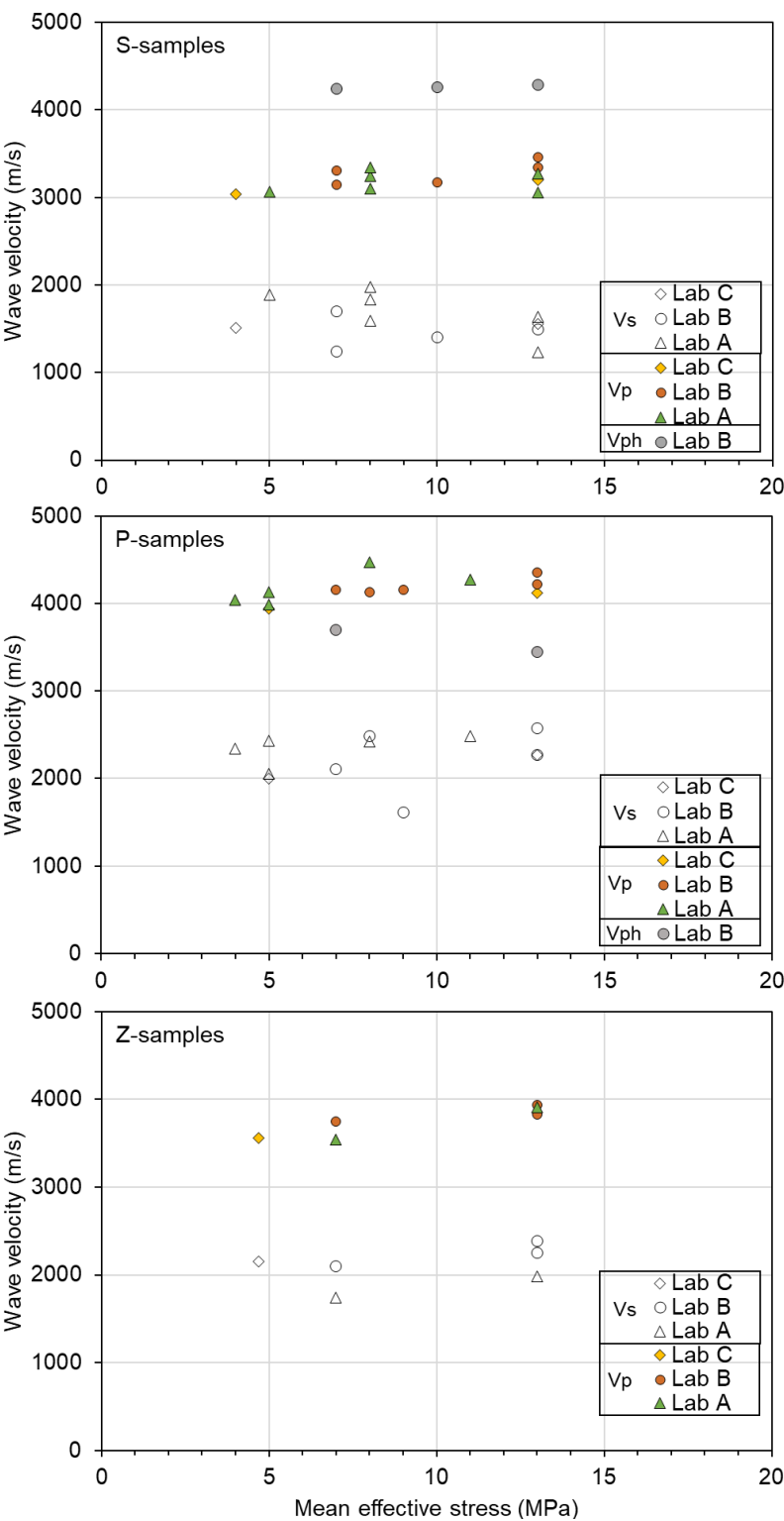
Fig. 6-11: Wave velocities at the beginning of the shearing phase Results are divided by specimen geometry. Lab C measured wave velocities after starting shearing, at a few MPa of deviatoric stress (data in Appendix E).
