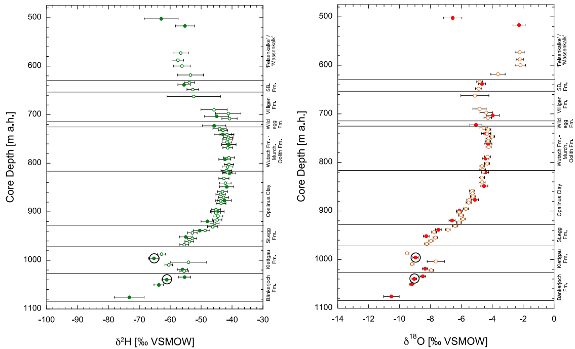
Fig. 4.8-4: Depth distribution of approved porewater \delta^{18}\text{O} - and \delta^2\text{H} -values obtained from isotope diffusive-exchange experiments
