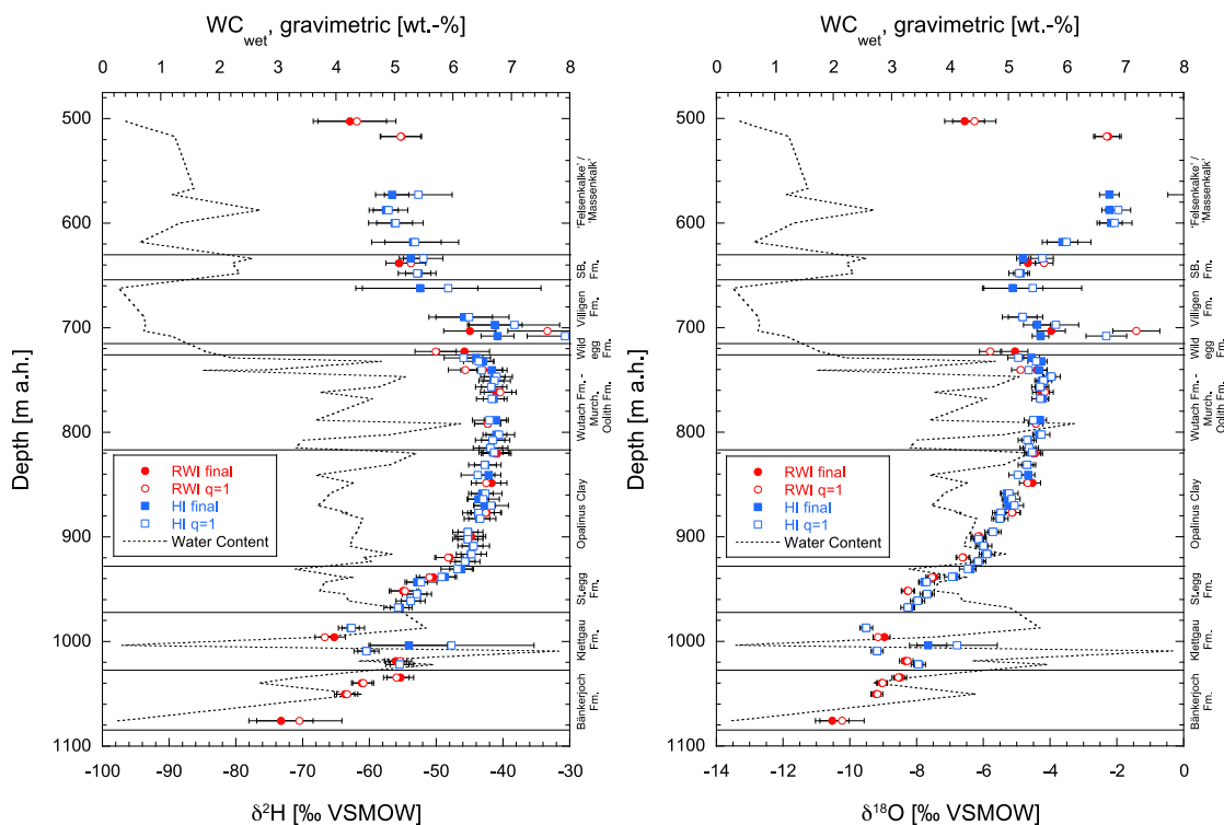
Fig. 4.8-1: Comparison of all porewater \delta^{18}\text{O} - and \delta^2\text{H} -values derived by isotope-diffusive exchange experiments and calculated by isotope mass balance based on the individual water contents (closed symbols, final) and based on assuming equal water contents (open symbols, q = 1 ) for the rock in both experiments
