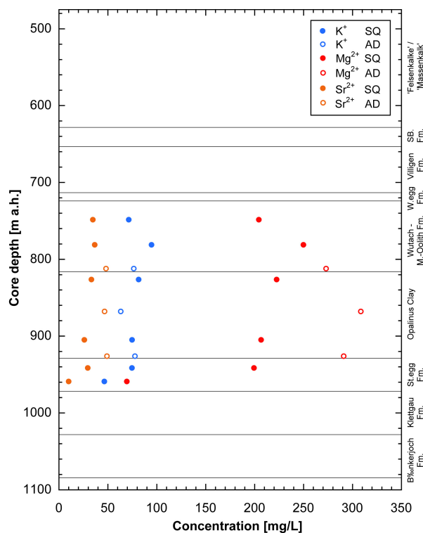
Fig. 5.4-2: Concentrations of K, Mg and Sr in aliquots from squeezing experiments and advective displacement experiments
