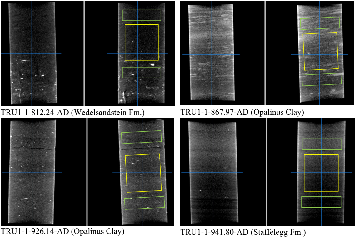
Fig. 4.7-2: X-ray CT images of AD samples
