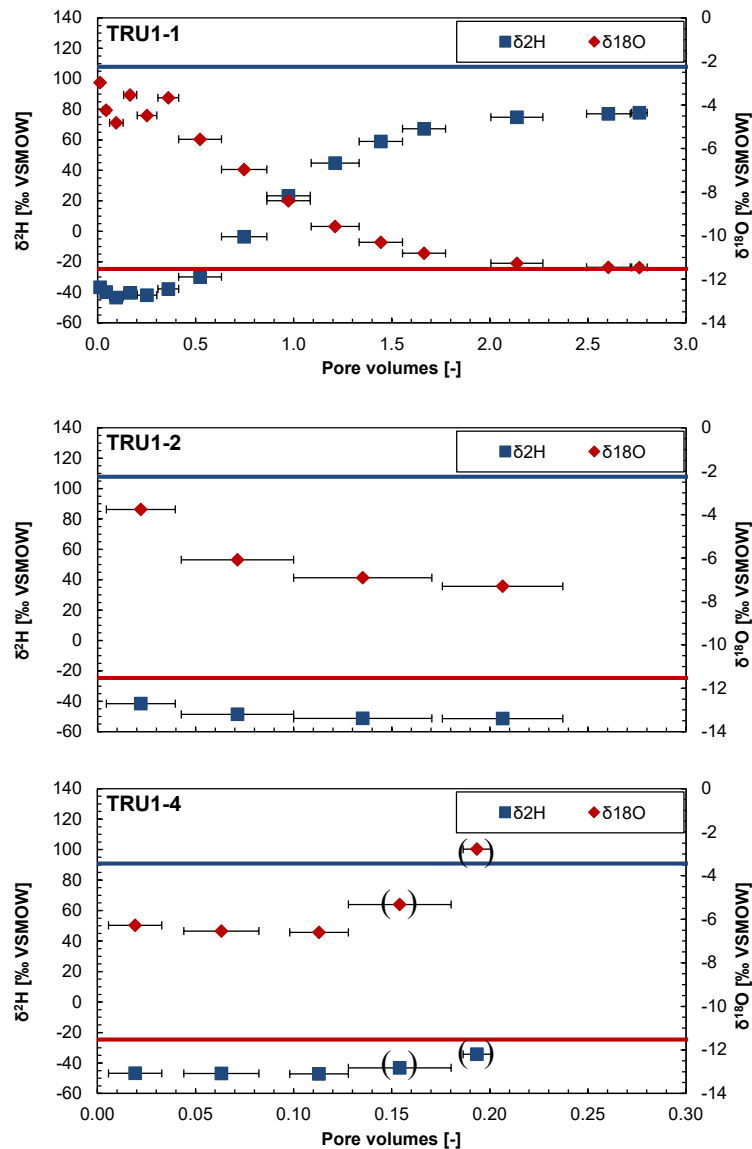
Fig. 4.7-15: Evolution of \delta^2\text{H} and \delta^{18}\text{O} during advective displacement experiments
