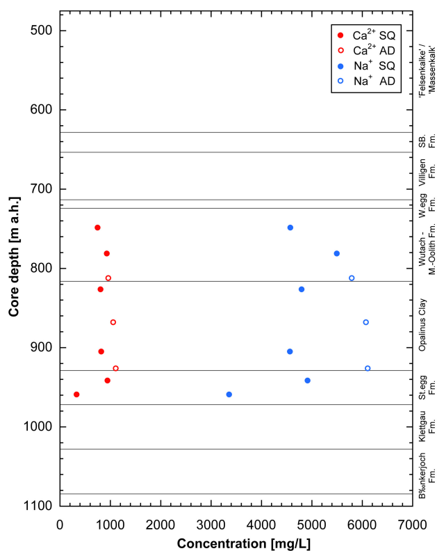
Fig. 5.4-1: Concentrations of Na and Ca in aliquots from squeezing experiments and advective displacement experiments
