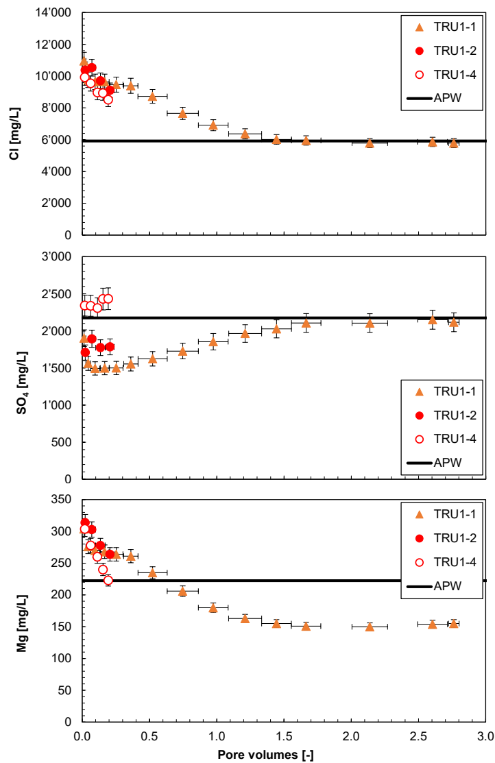
Fig. 4.7-9: Evolution of selected major components during advective displacement experiments
