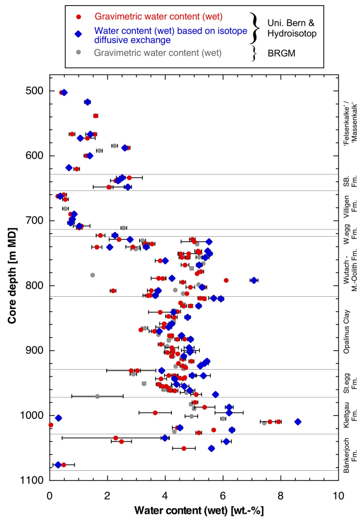
Fig. 4.3-1: Water content as a function of depth
