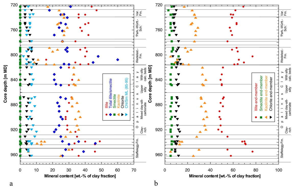
Fig. 4.2-5: Mineralogical composition of the clay fraction as a function of depth in the Lias – Dogger interval
