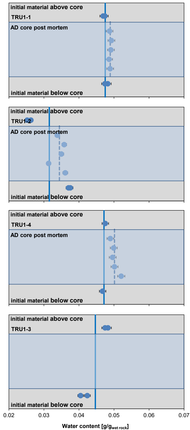
Fig. 4.7-3: Details of water content measurements before and after AD experiments
