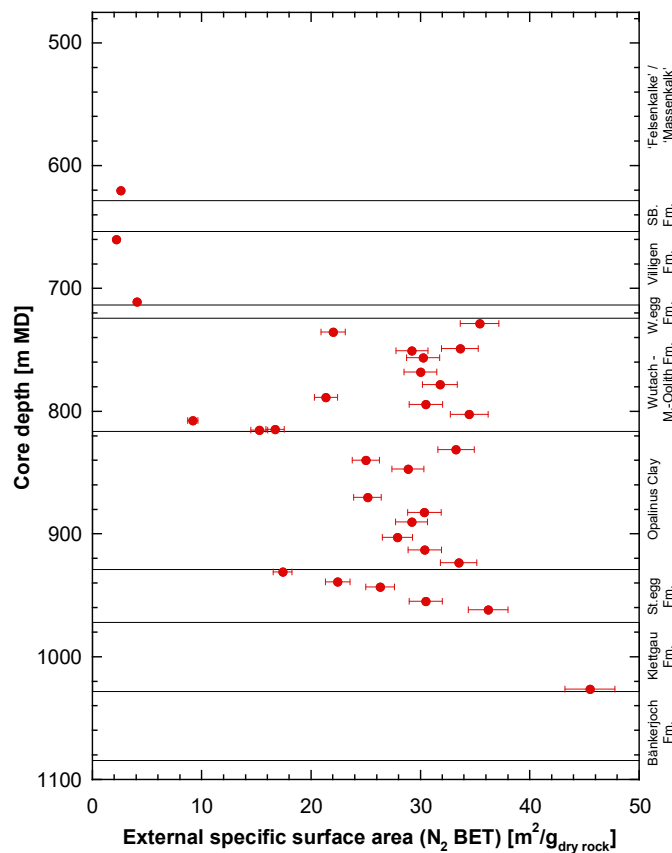
Fig. 4.3-13: Depth profile of specific surface area ( S_{\text{BET}} ) derived from \text{N}_2 adsorption
