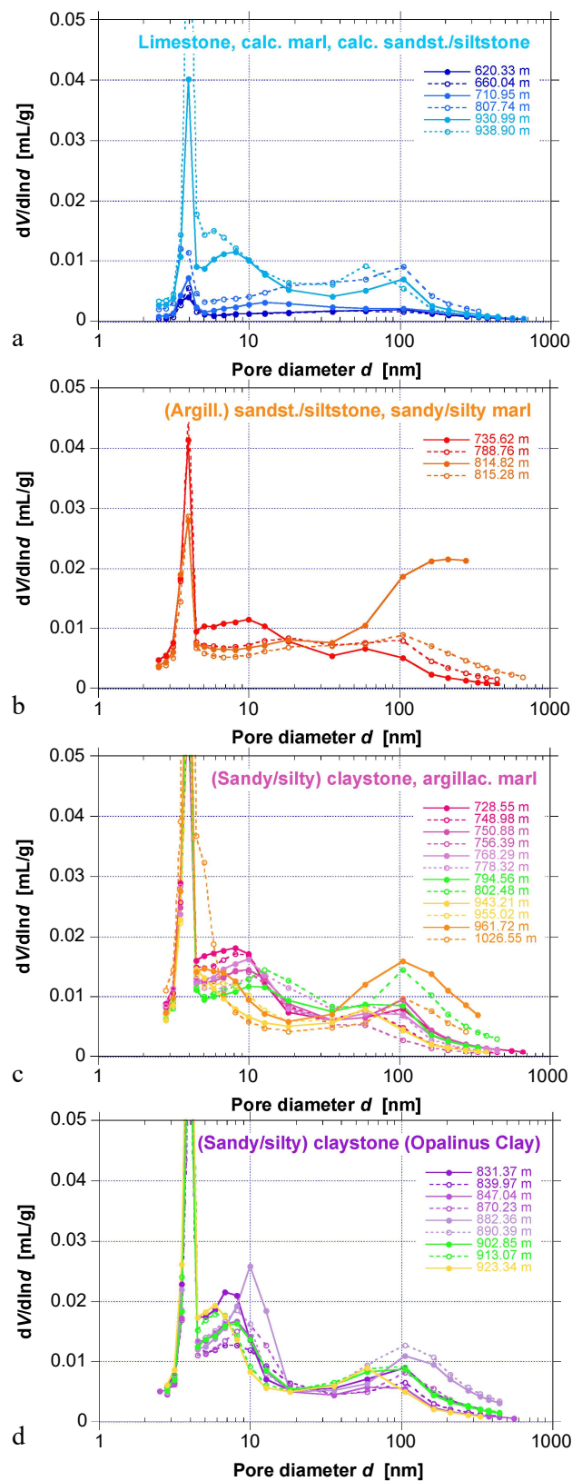
Fig. 4.3-18: Distribution of (external) pore sizes derived from N_2 desorption
