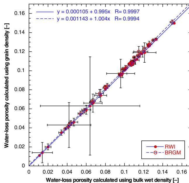
Fig. 4.3-7: Water-loss porosity calculated from gravimetric water content using either bulk wet or grain density
