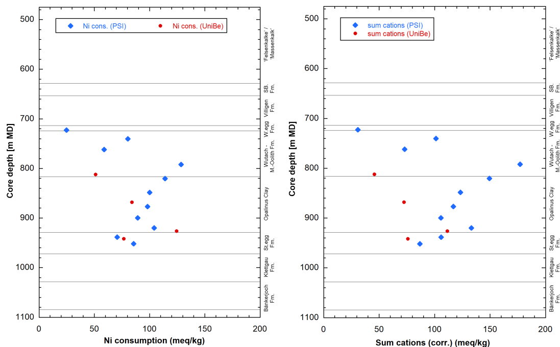
Fig. 5.6-3: Comparison of CEC data from University of Bern and from PSI
