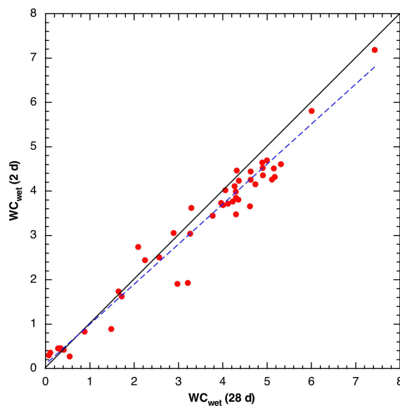
Fig. 3.4-1: Comparison of water contents obtained by BRGM by drying at 105 °C over 2 and 28 d
