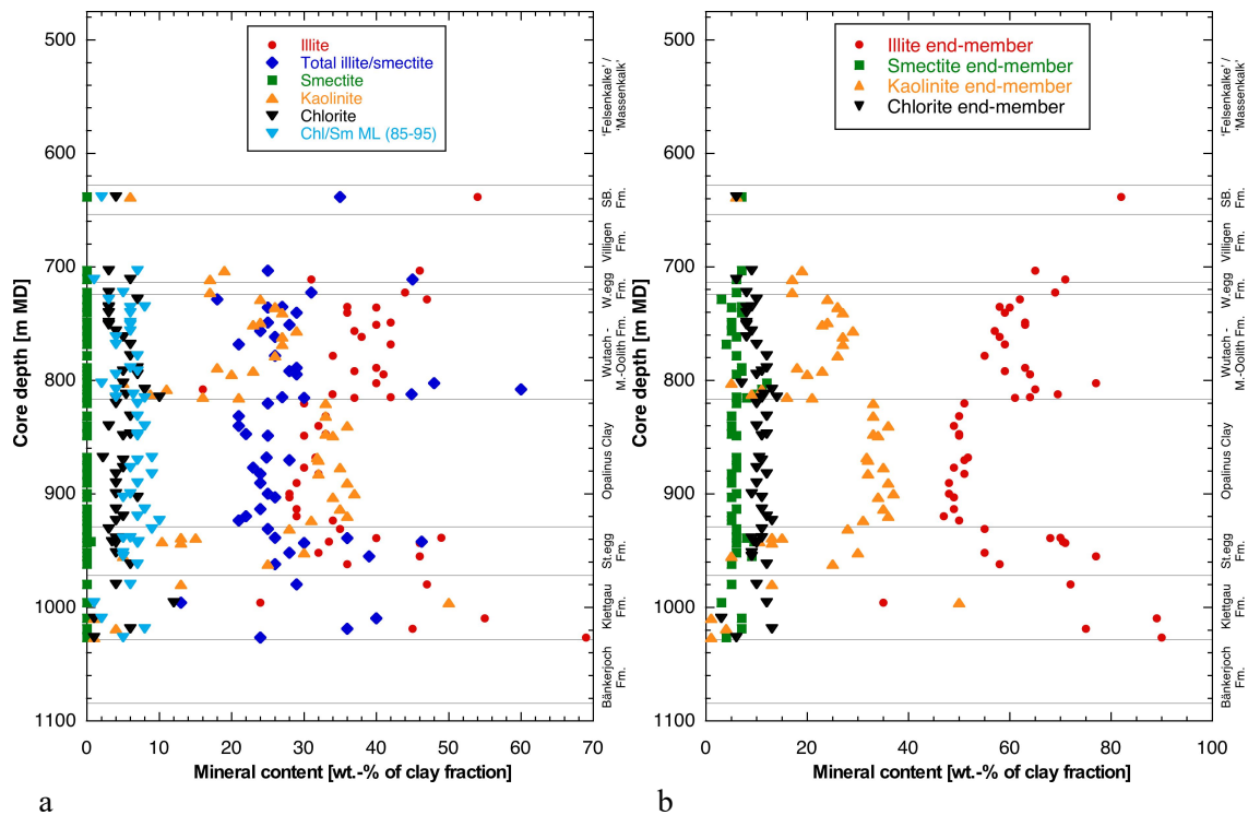
Fig. 4.2-4: Mineralogical composition of the clay fraction as a function of depth
