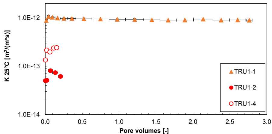
Fig. 4.7-4: Evolution of hydraulic conductivity during advective displacement experiments
