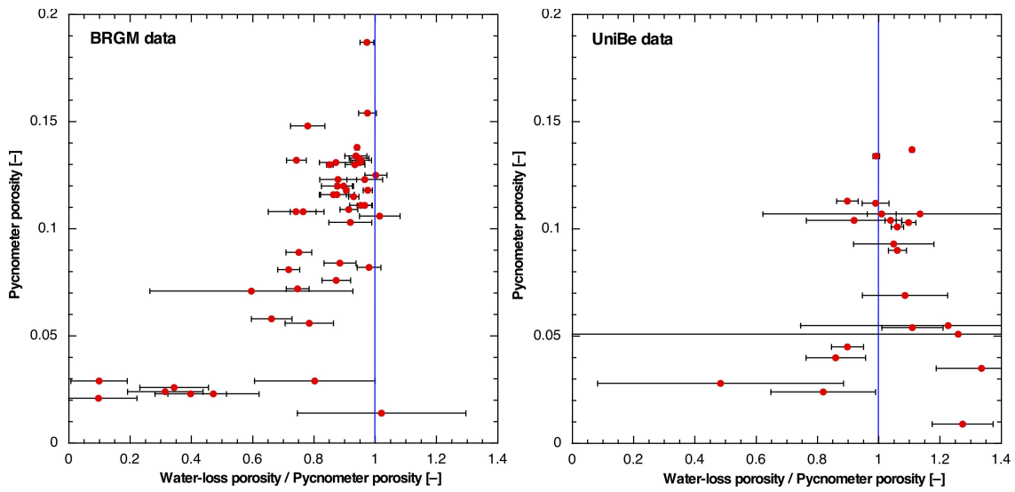
Fig. 3.4-2: Ratio of water-loss porosity (calculated from WC_{28d} in the case of BRGM) and pycnometer porosity obtained from measurements at BRGM and at the University of Bern
