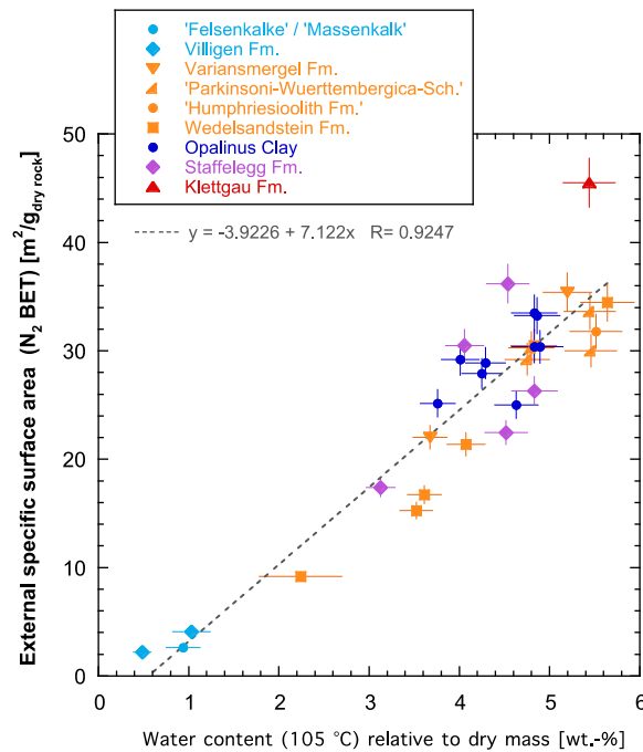
Fig. 4.3-14: Specific surface area ( S_{\text{BET}} ) derived from N_2 adsorption plotted against the gravimetric water content relative to the dry mass of the samples
