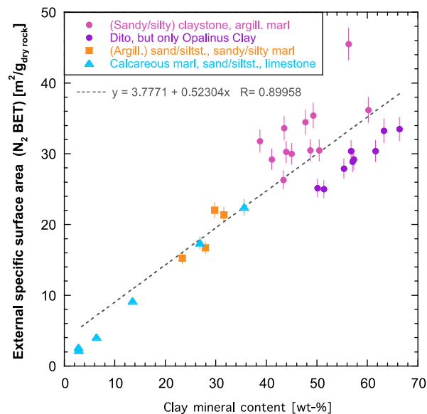
Fig. 4.3-15: Relation between external specific surface area ( S_{\text{BET}} ) derived from N_2 adsorption and content of clay minerals
