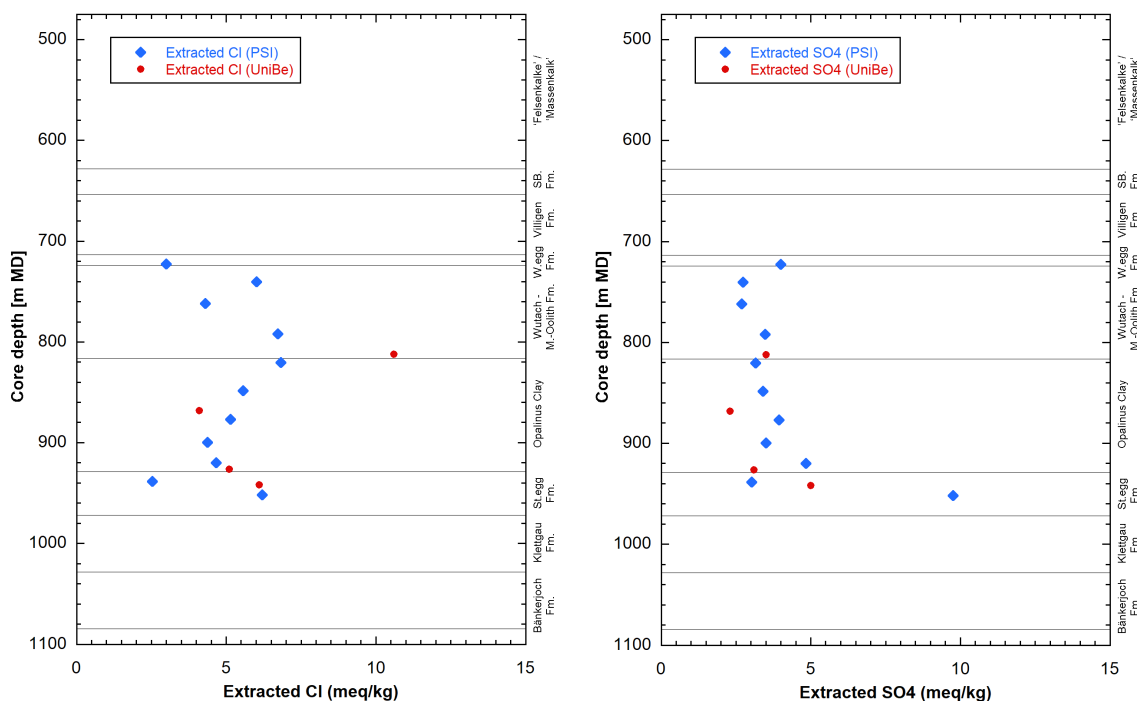
Fig. 5.6-9: Extracted Cl (left) and SO 4 (right) according to University of Bern and PSI data
