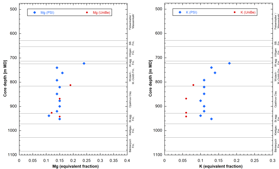
Fig. 5.6-6: Mg (left) and K (right) fractional occupancies according to University of Bern and PSI data
