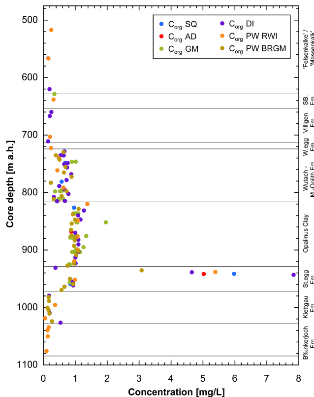
Fig. 5.5-1: Organic carbon in rock samples
