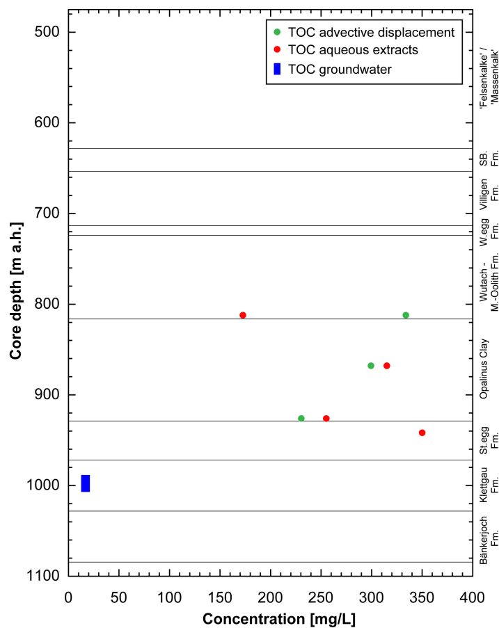
Fig. 5.5-2: TOC in aliquots from AD, upscaled from aqueous extracts, and the Keuper aquifer
