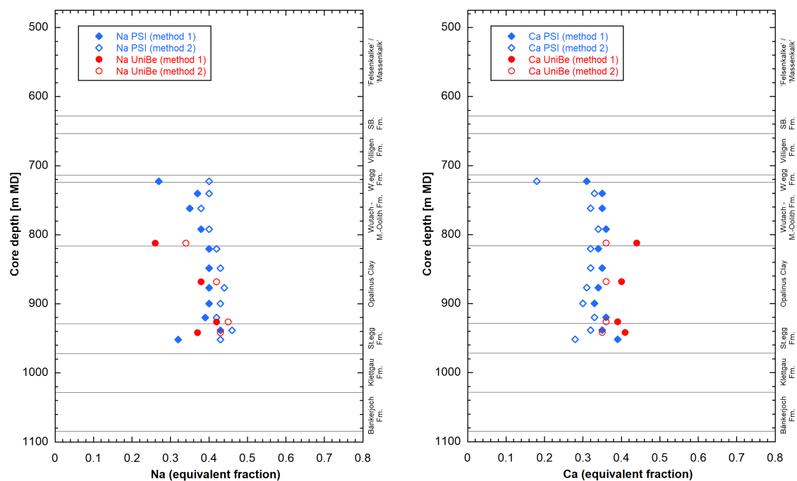
Fig. 5.6-5: Na (left) and Ca (right) fractional occupancies according to University of Bern and PSI data
