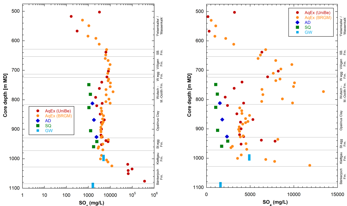
Fig. 5.3-1: SO 4 profile with data from squeezing, advective displacement, aqueous extraction, and groundwater samples
