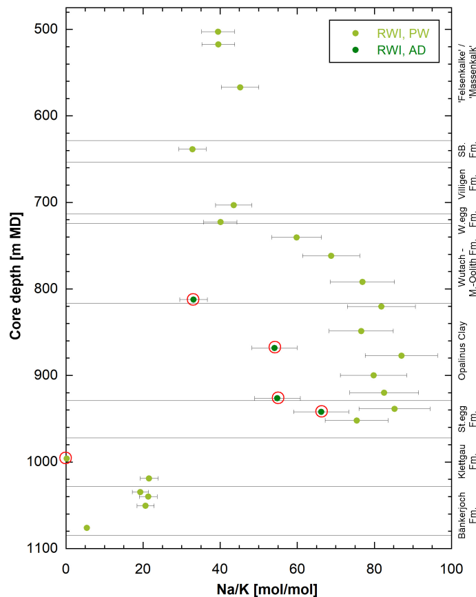
Fig. 4.4-8: Depth versus Na/K molar concentration ratio in aqueous extracts at a S/L ratio of 1
