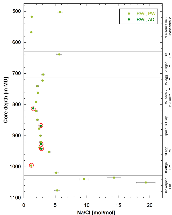
Fig. 4.4-7: Depth profile of the Na/Cl molar concentration ratio in aqueous extracts at a S/L ratio of 1
