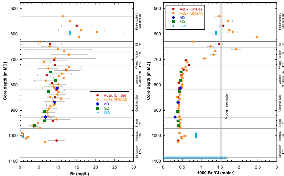
Fig. 5.2-2: Br and Br/Cl profiles with data from squeezing, advective displacement, aqueous extraction and groundwater samples
