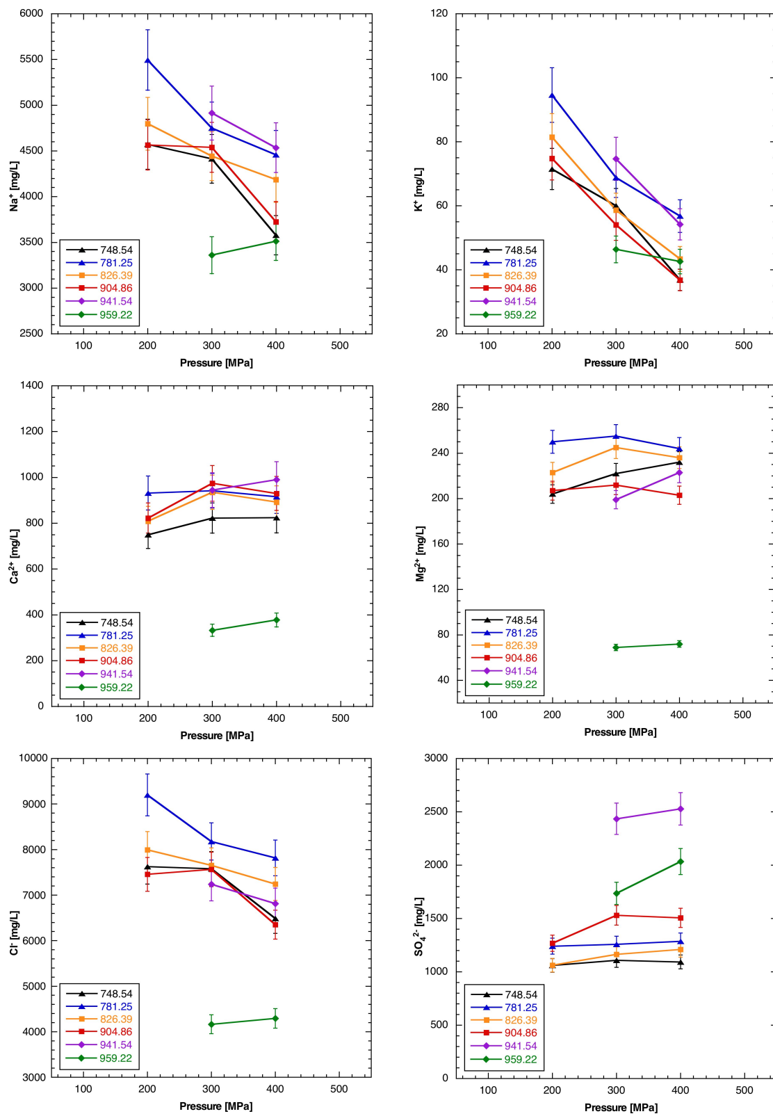
Fig. 4.6-3: Ion concentrations in squeezed waters as a function of squeezing pressure Bars indicate analytical errors of ion-chromatography analysis.
