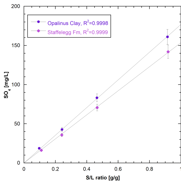
Fig. 4.4-2: SO 4 concentrations versus S/L ratios in aqueous extract solutions from the Opalinus Clay and the Staffelegg Formation
