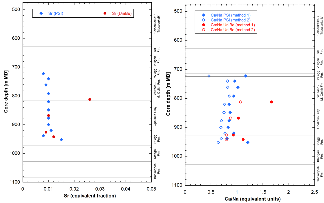
Fig. 5.6-7: Sr fractional occupancies (left) and Ca/Na ratios (right) according to University of Bern and PSI data
