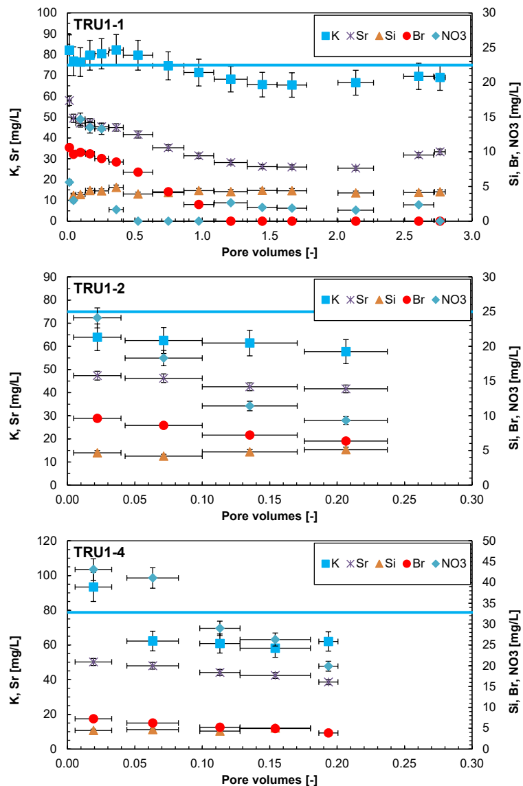
Fig. 4.7-10: Evolution of minor components during advective displacement experiments
