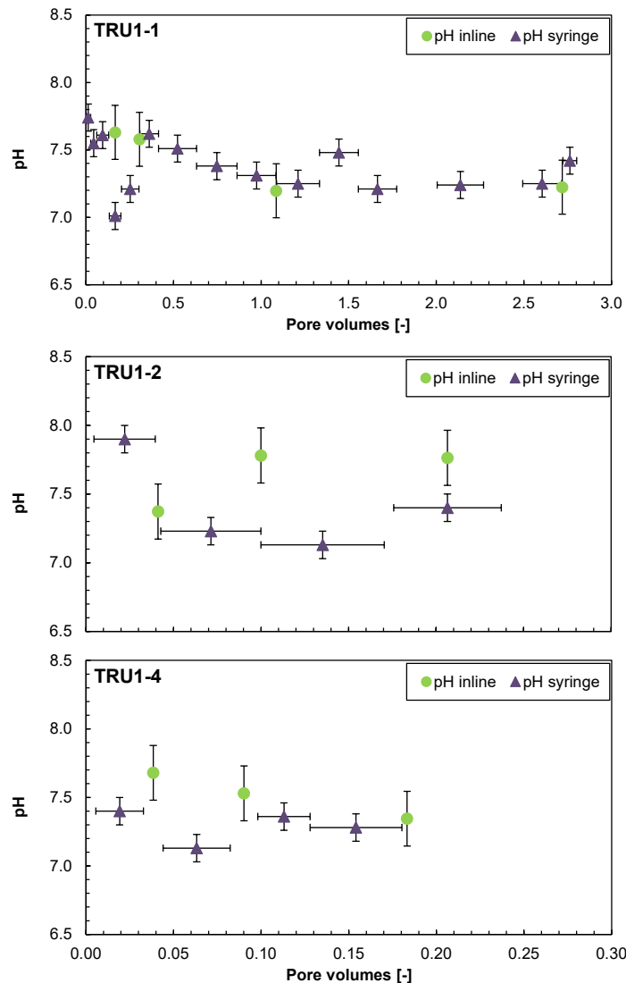
Fig. 4.7-14: Evolution of pH during advective displacement experiments
