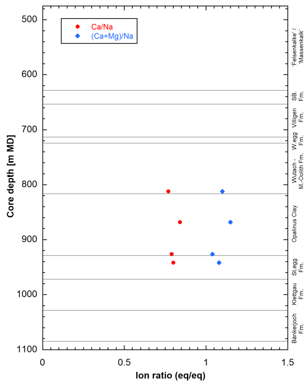
Fig. 4.5-3: Depth profiles of Ca/Na and (Ca+Mg)/Na ratios in Ni-en extracts
