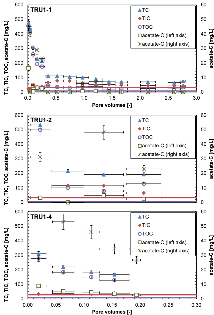
Fig. 4.7-12: Evolution of carbon system during advective displacement experiments
