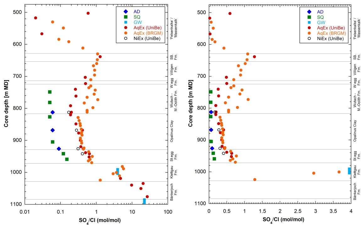
Fig. 5.3-3: Profiles showing molar \text{SO}_4/\text{Cl} ratios obtained from different methods in logarithmic and linear scales
