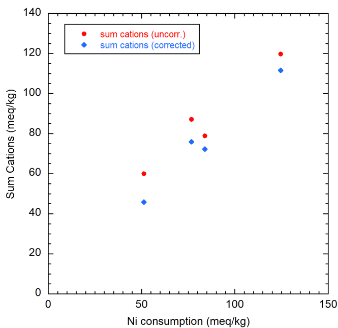
Fig. 5.6-1: Ni consumption vs. sum of cations (data of University of Bern)
