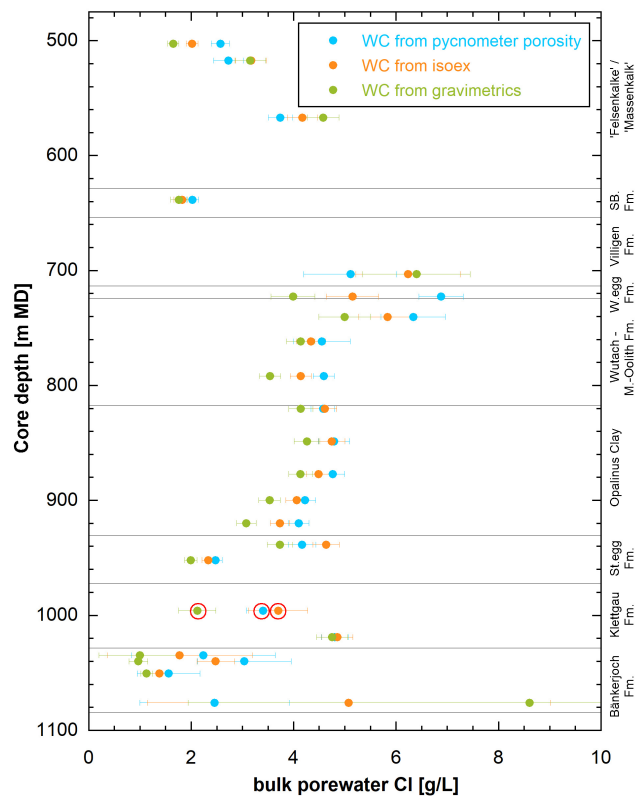
Fig. 4.4-11: Bulk porewater Cl of RWI data calculated with three different derived water contents: gravimetrically, from diffusive-exchange experiments and from pycnometer porosity
