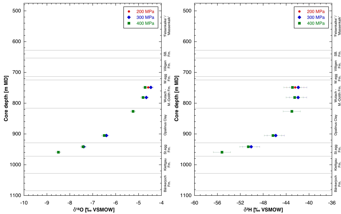
Fig. 4.6-6: Depth trends of \delta^{18}\text{O} and \delta^2\text{H} in squeezed waters
