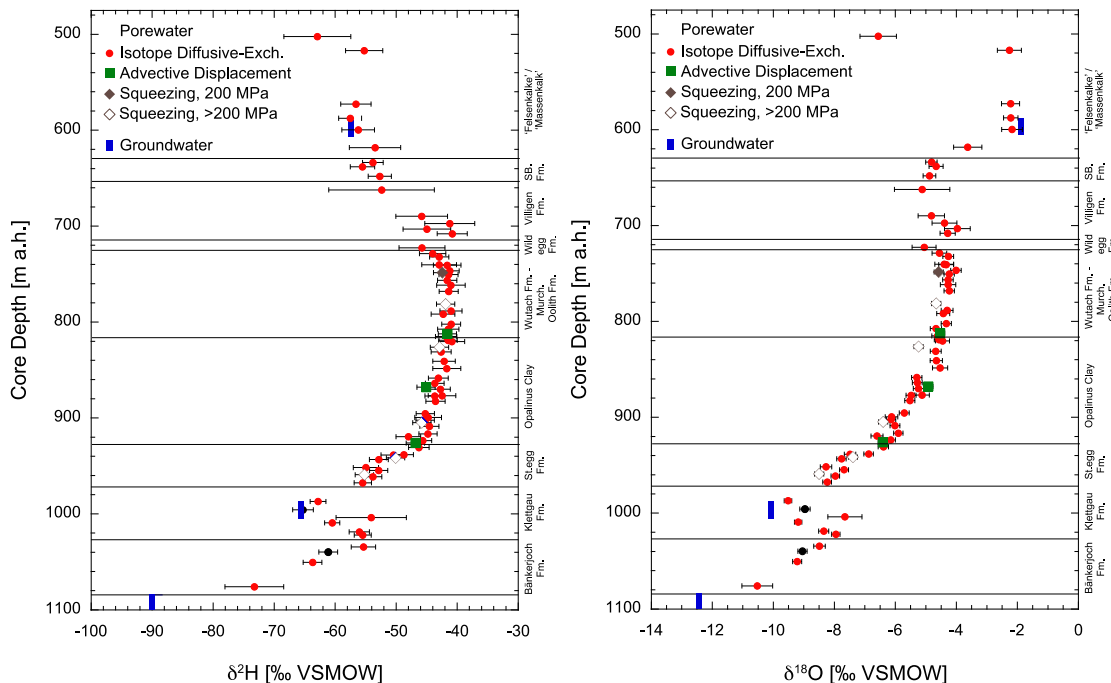
Fig. 5.7-1: Depth trends of \delta^{18}\text{O} and \delta^2\text{H} in groundwater and porewater derived by all techniques
