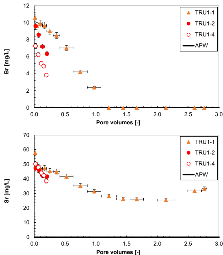
Fig. 4.7-11: Evolution of selected minor components during advective displacement experiments
