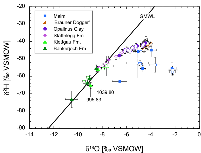
Fig. 4.8-5: \delta^{18}\text{O} vs. \delta^2\text{H} -values of porewater obtained from isotope diffusive-exchange experiments
