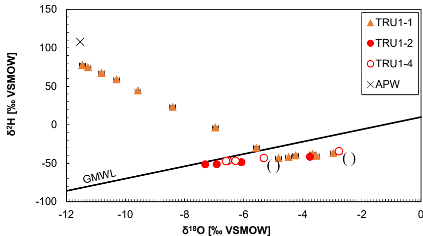
Fig. 4.7-16: Stable isotope composition of aliquots from advective displacement experiments
