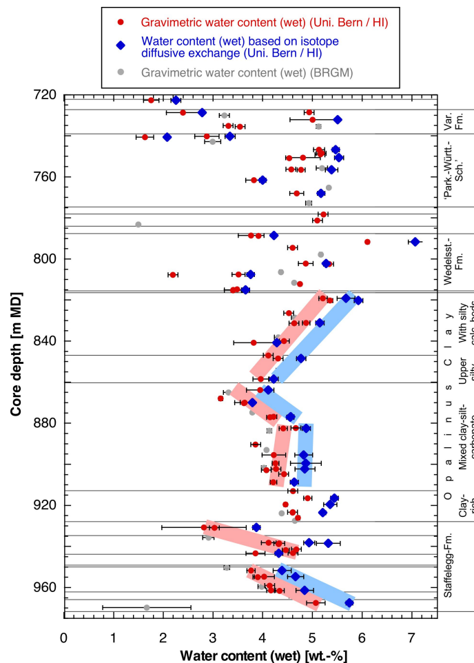
Fig. 4.3-4: Water content (wet) as a function of depth in the Lias-Dogger interval
