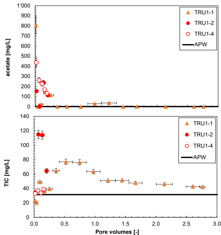
Fig. 4.7-13: Evolution of selected carbon components during advective displacement experiments
