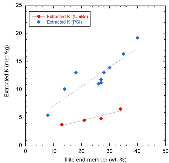
Fig. 5.6-8: Content of the illite end-member vs. extracted K
