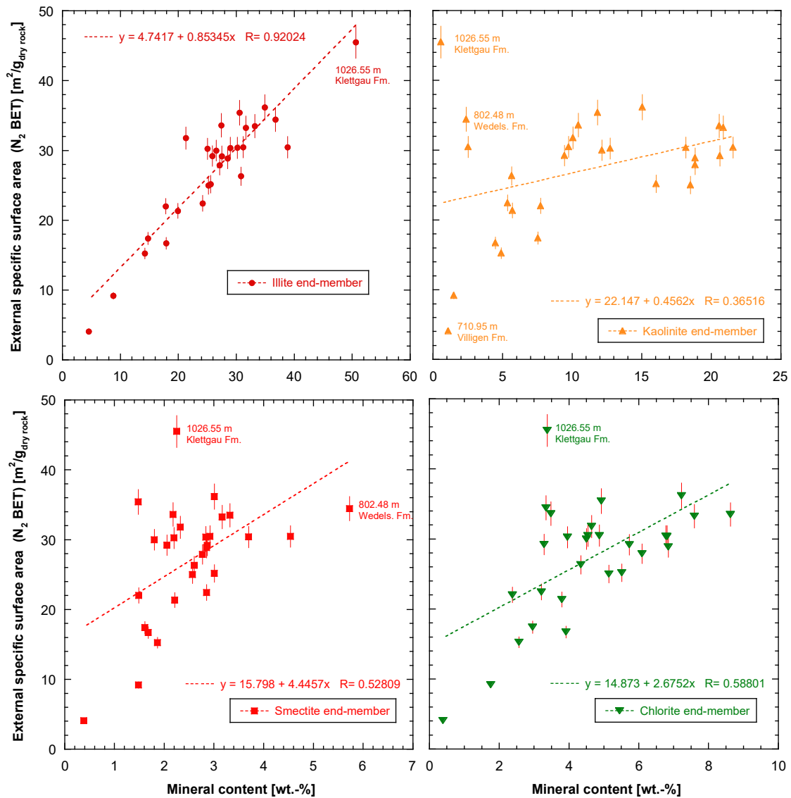
Fig. 4.3-16: Relation between external specific surface area ( S_{\text{BET}} ) derived from N_2 adsorption and contents of specific clay mineral end-members
