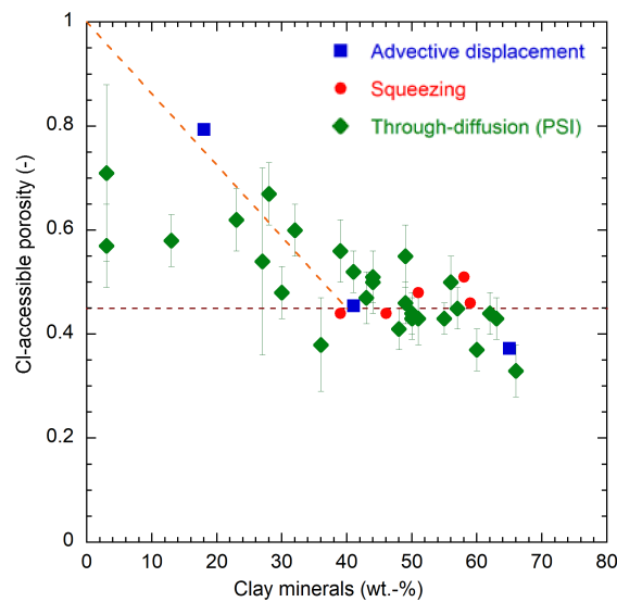
Fig. 5.1-1: Cl-accessible porosity fraction as a function of the clay-mineral content
