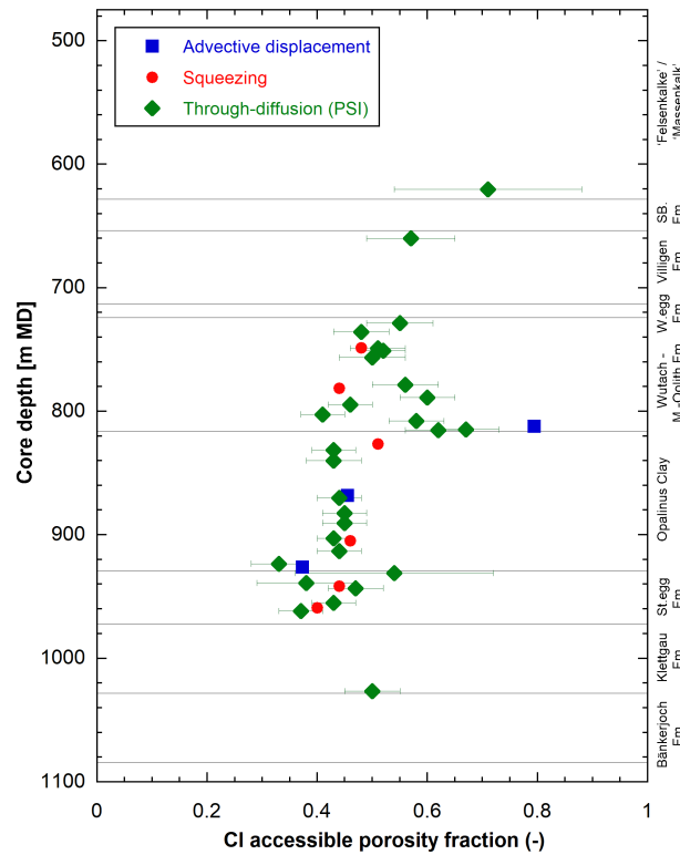
Fig. 5.1-2: Cl-accessible porosity fraction ( f_{Cl} ) as a function of depth
