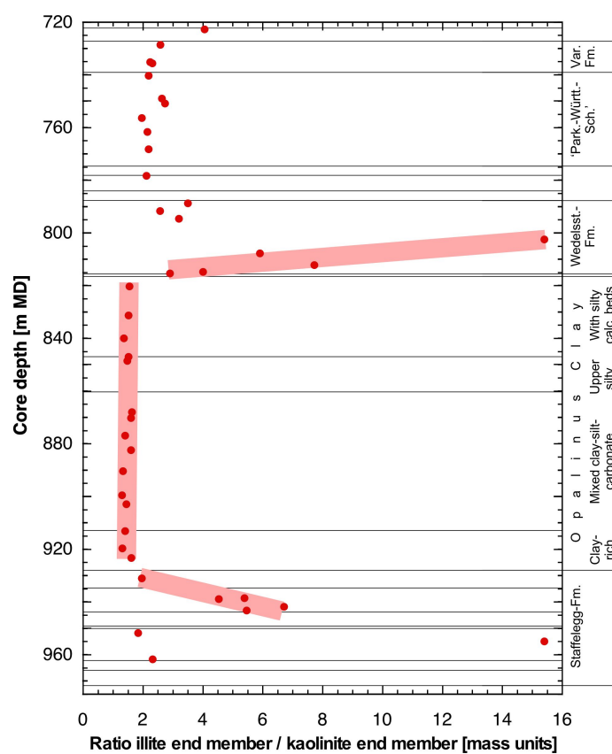
Fig. 4.2-6: Ratio of the illite to kaolinite end-member clays as a function of depth
