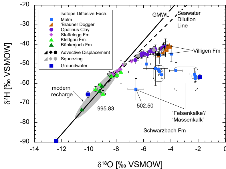
Fig. 5.7-2: \delta^{18}\text{O} vs. \delta^2\text{H} for groundwater and porewater derived by all techniques
