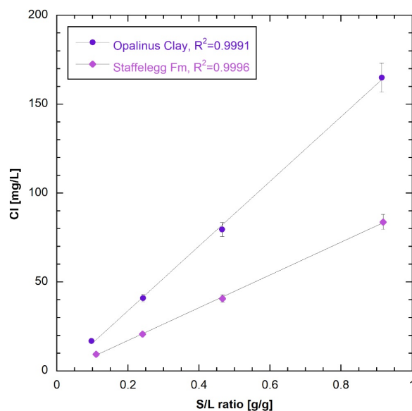
Fig. 4.4-1: Cl concentrations versus S/L ratios in aqueous extract solutions from the Opalinus Clay and the Staffelegg Formation
