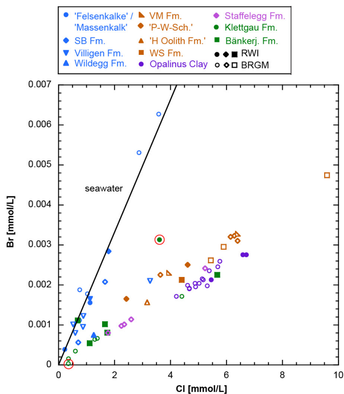
Fig. 4.4-4: Br versus Cl molar concentrations in aqueous extracts at a S/L ratio of 1
