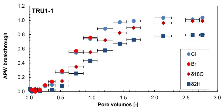
Fig. 4.7-17: Breakthrough of Cl, Br, \delta^2\text{H} and \delta^{18}\text{O} during advective displacement experiments
