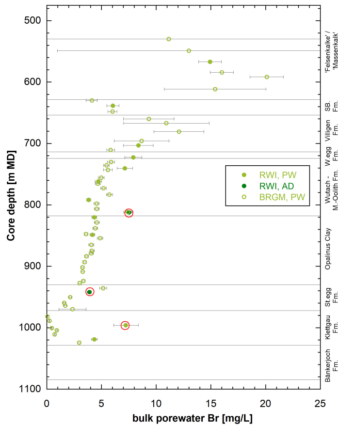
Fig. 4.4-10: Bulk porewater Br concentrations versus depth from aqueous extracts
