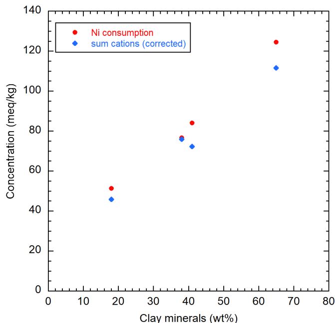
Fig. 5.6-2: CEC parameters as a function of clay-mineral content (data of University of Bern)
