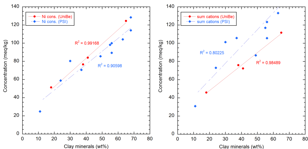
Fig. 5.6-4: CEC data as function of the clay-mineral content
