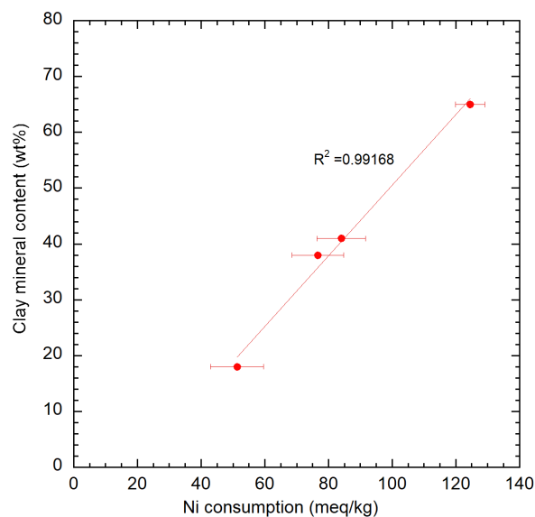
Fig. 4.5-2: Ni consumption vs. clay-mineral content
