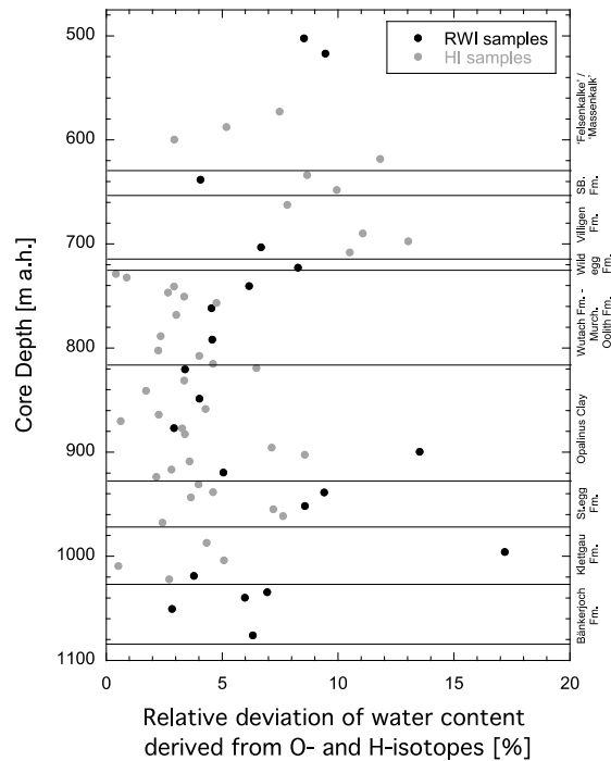
Fig. 4.8-2: Relative deviation of water contents obtained from \delta^{18}\text{O} and \delta^2\text{H} mass balance
