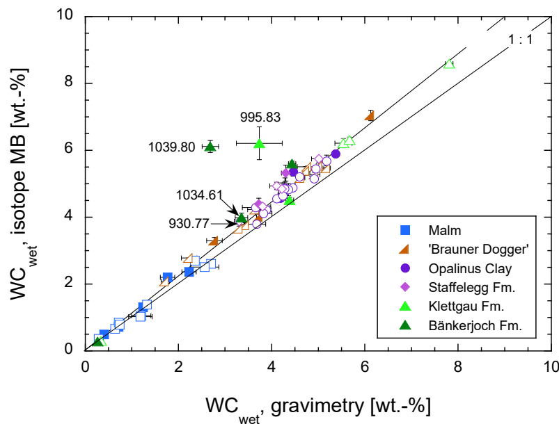
Fig. 4.8-3: Average water content obtained by water-loss at 105 °C ( WC_{wet} gravimetry) of the subsamples LAB and NGW/ICE used in isotope diffusive-exchange experiments vs. the average water content calculated from \delta^{18}O and \delta^2H mass balance from the NGW/ICE samples ( WC_{wet} isotope MB)
