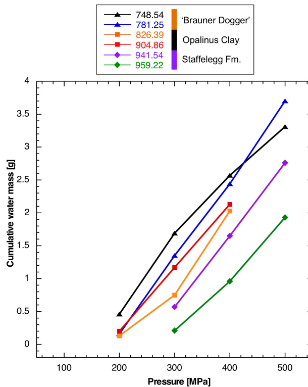
Fig. 4.6-1: Cumulative water mass obtained by squeezing as a function of the squeezing pressure
