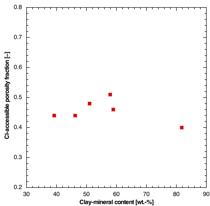
Fig. 4.6-5: Cl-accessible porosity fractions derived from squeezing experiments as a function of the clay-mineral content
