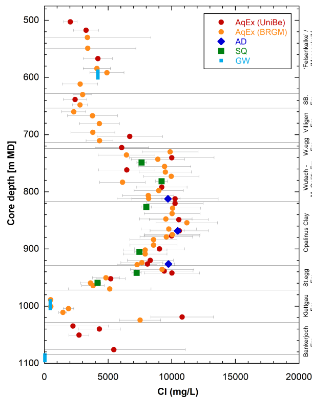
Fig. 5.2-1: Cl profile with data from squeezing, advective displacement, aqueous extraction, and groundwater samples
