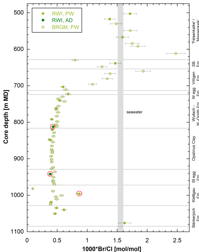
Fig. 4.4-5: Depth profile of the molar Br/Cl ratio in aqueous extracts at a S/L ratio of 1
