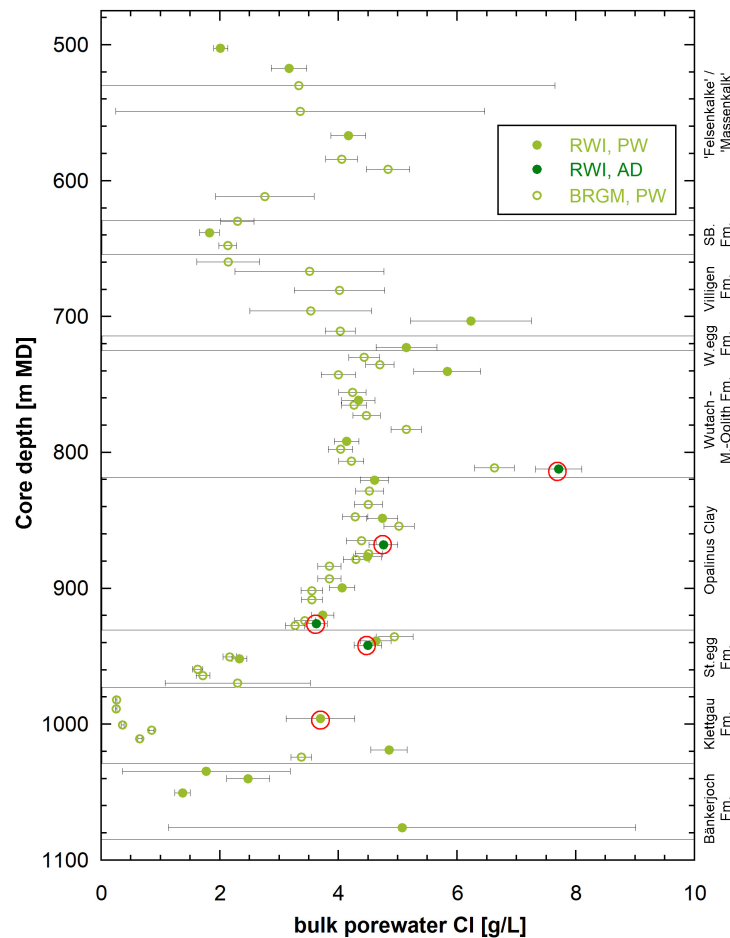
Fig. 4.4-9: Bulk porewater Cl concentrations versus depth from aqueous extracts
