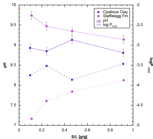
Fig. 4.4-3: pH and \log P_{\text{CO}_2} versus S/L ratio in aqueous extracts from the Opalinus Clay and the Staffelegg Formation
