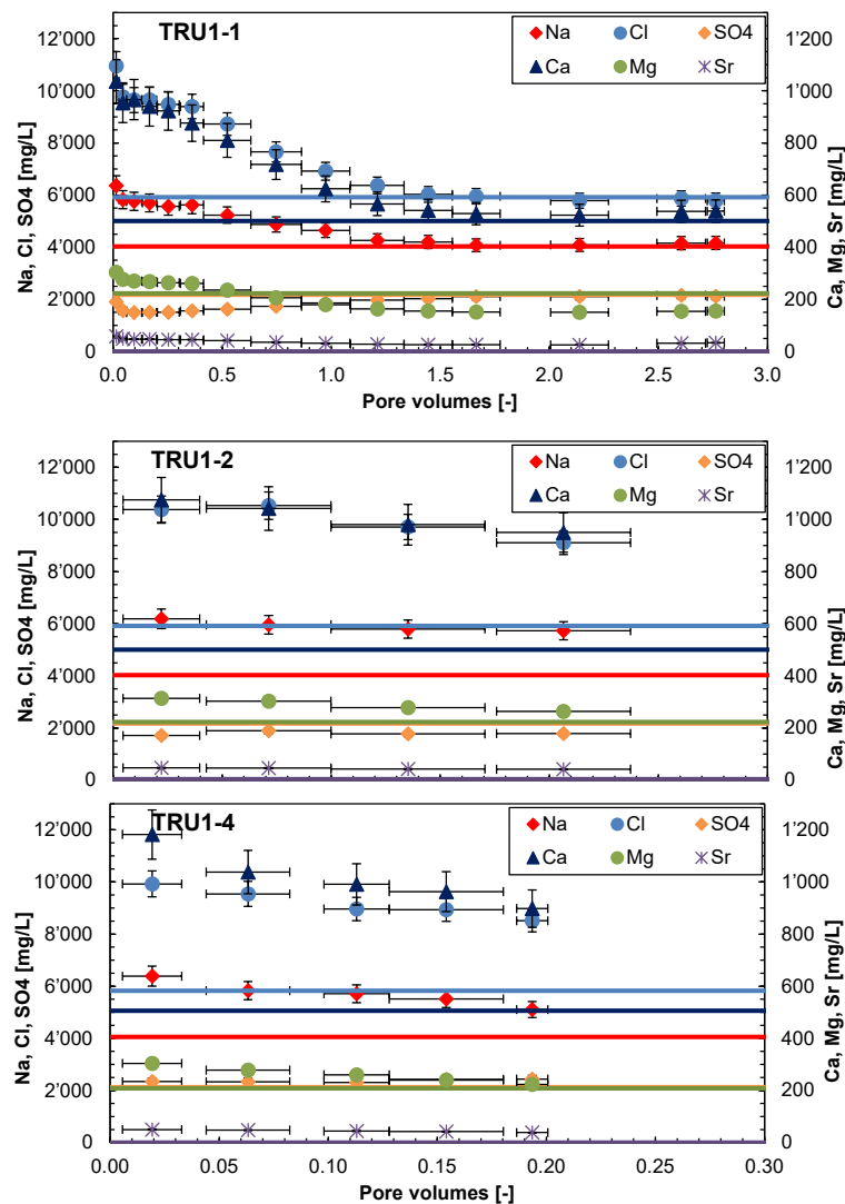
Fig. 4.7-8: Evolution of major components during advective displacement experiments
