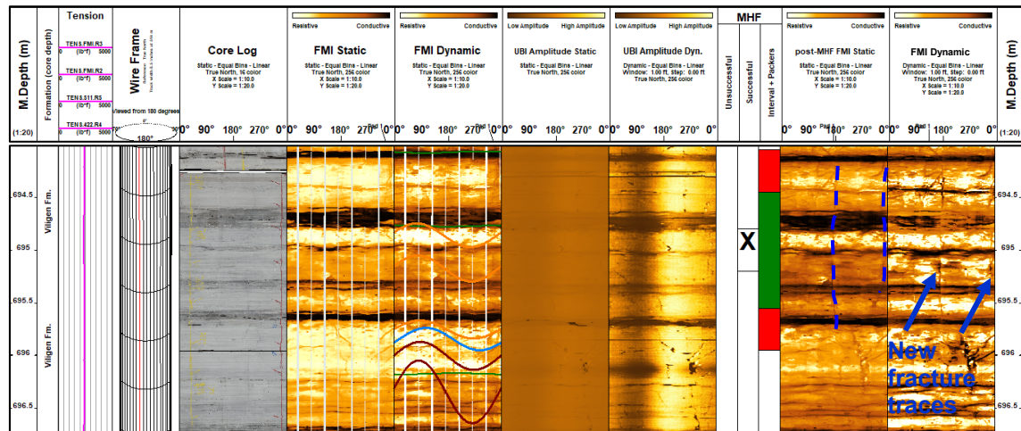
Fig. 5-19: Example of pre- vs. post-MHF images from TRU1-1 (Station 1-3, Section II)
