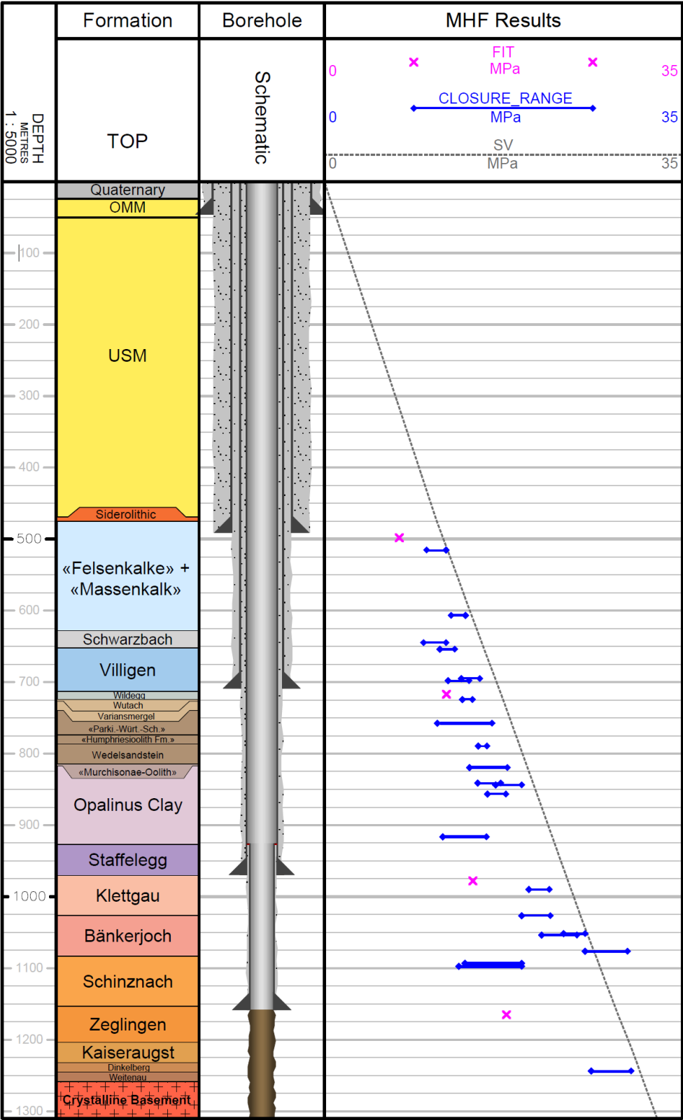
Fig. 5-20: Comparison of the quicklook closure stress range obtained from the TRU1-1 MHF tests with the overburden vertical stress (Sv) from the integration of density over depth and the maximum pressures attained during the formation integrity tests (FIT)
