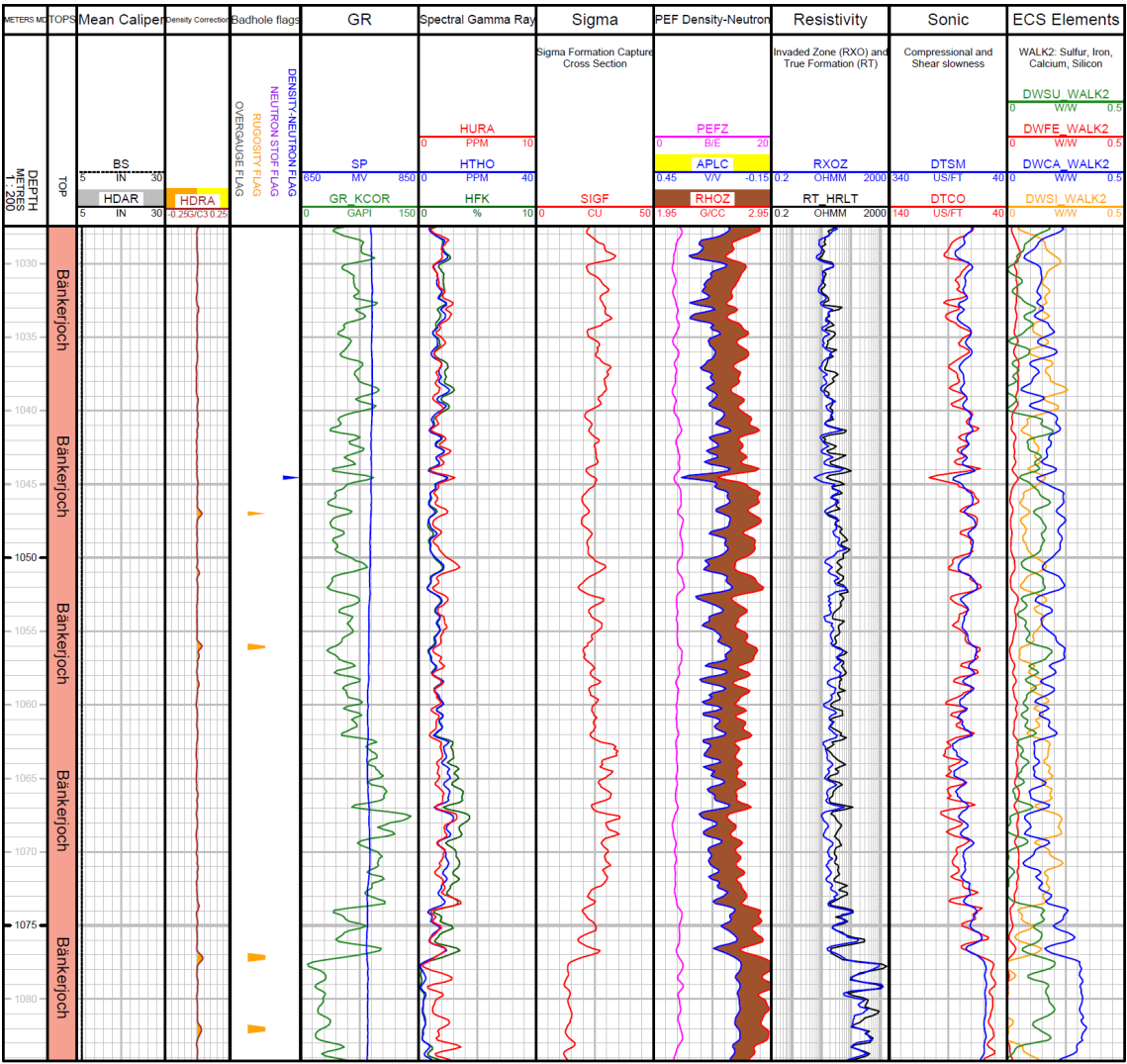
Fig. 3-8: Main logs of the composite dataset in the Bänkerjoch Formation
