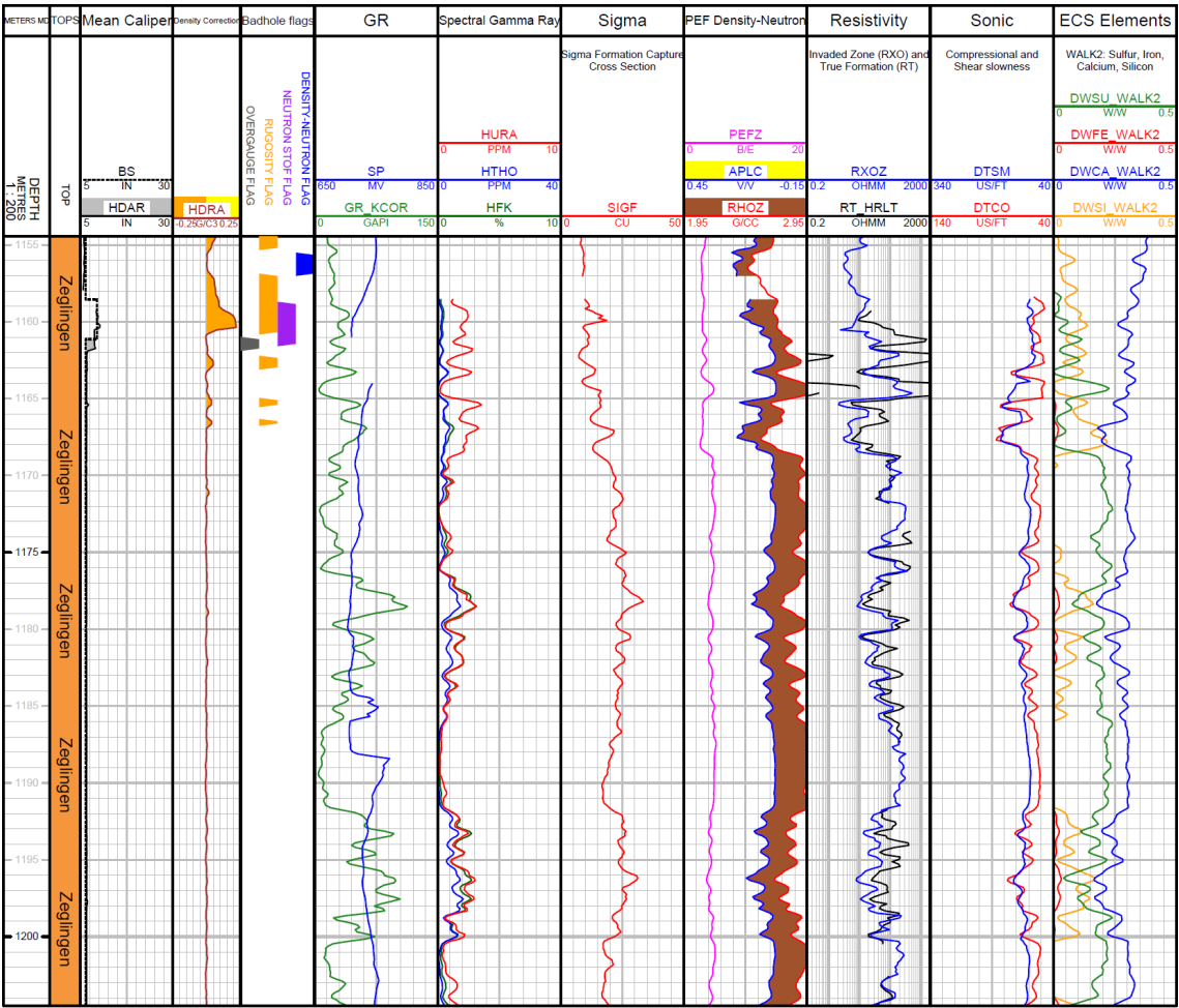
Fig. 3-10: Main logs of the composite dataset in the Zeglingen Formation
