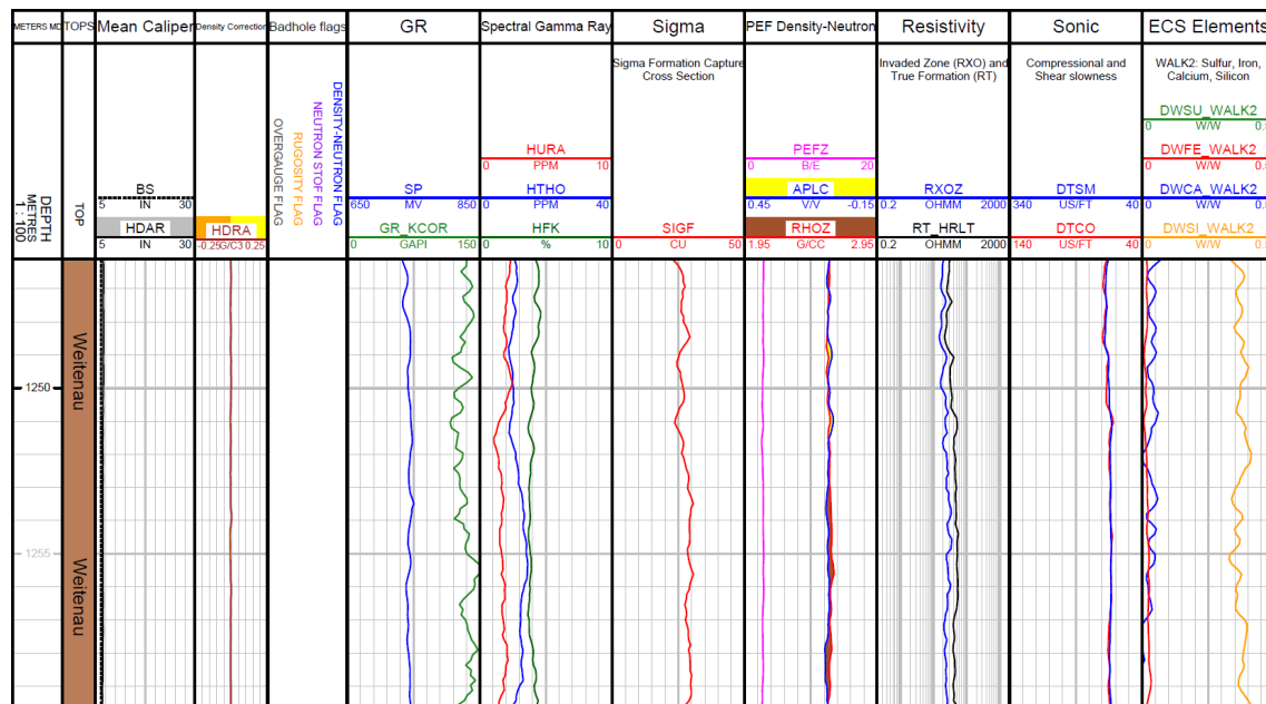
Fig. 3-13: Main logs of the composite dataset in the Weitenau Formation
