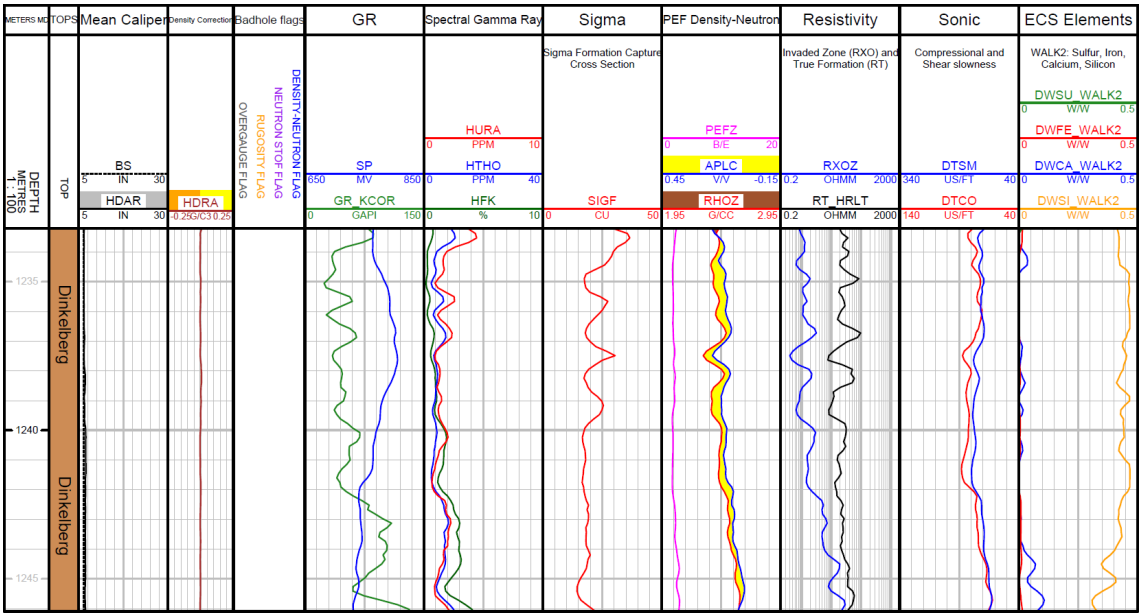
Fig. 3-12: Main logs of the composite dataset in the Dinkelberg Formation
