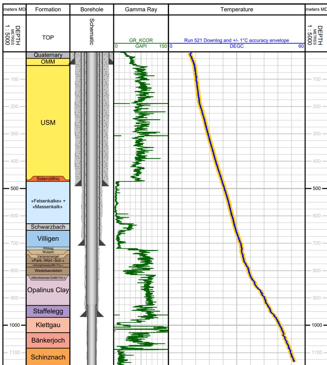
Fig. 3-15: Post-completion temperature log from the downlog pass of Run 5.2.1 (09.04.2021)
