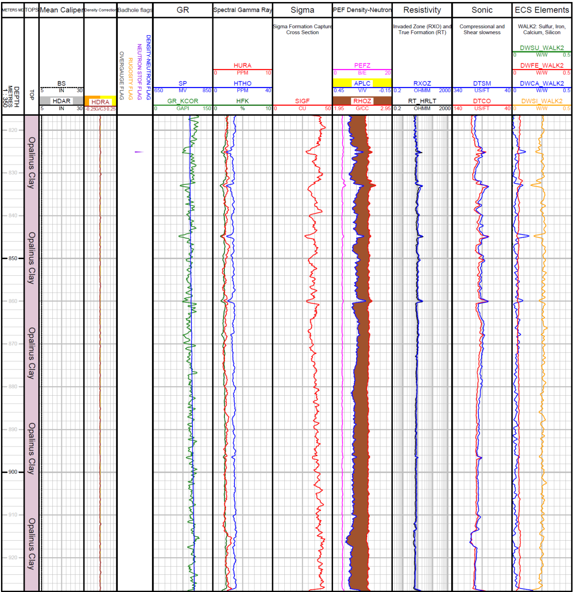
Fig. 3-5: Main logs of the composite dataset in the Opalinus Clay
