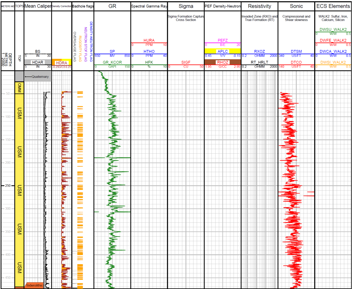
Fig. 3-2: Main logs of the composite dataset in the Cenozoic units
