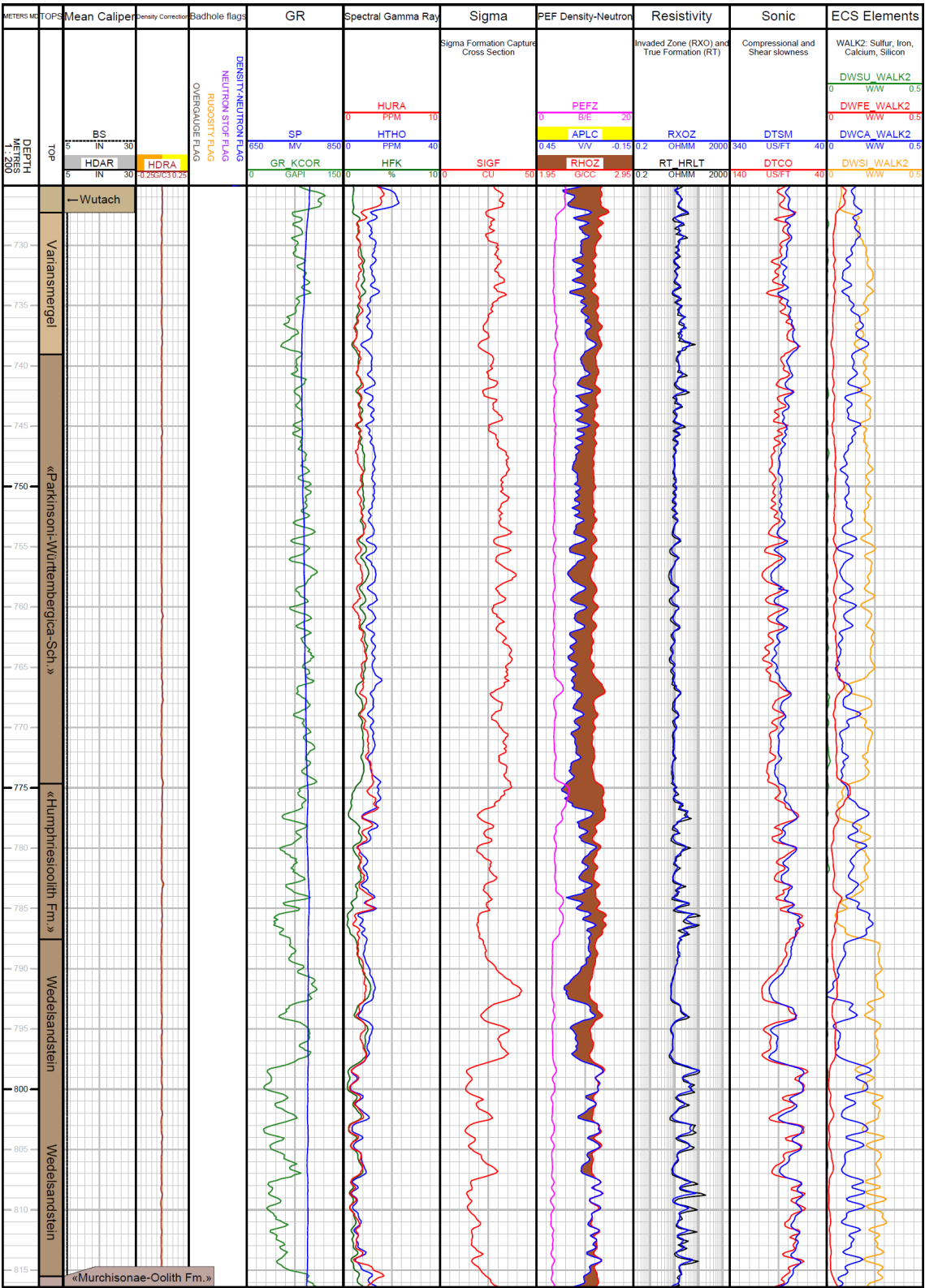
Fig. 3-4: Main logs of the composite dataset in the Wutach Formation to «Murchisonae-Oolith» unit
