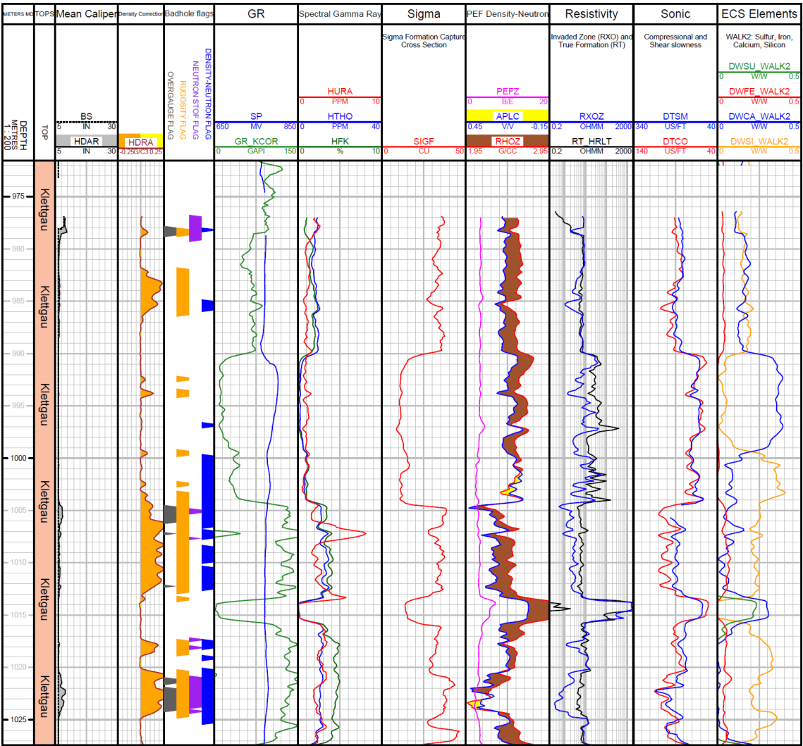
Fig. 3-7: Main logs of the composite dataset in the Klettgau Formation
