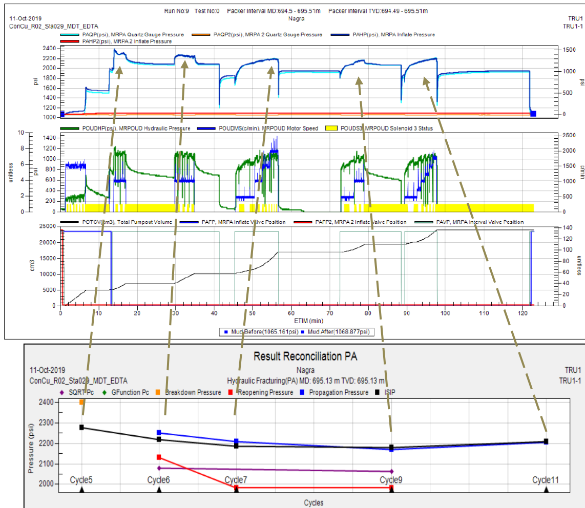
Fig. 5-18: Example of pressure record for MHF test from TRU1-1 (Station 1-3, Run 2.1.8)
