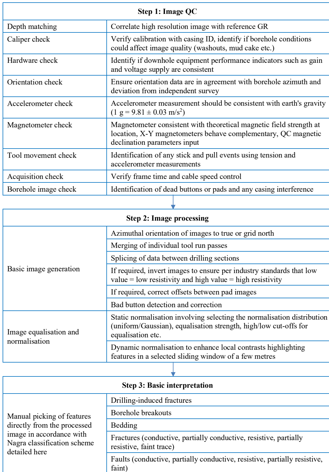
Fig. 4-16: Borehole image processing workflow
