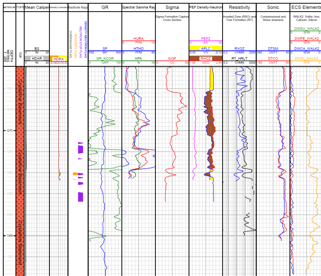
Fig. 3-14: Main logs of the composite dataset in the crystalline basement
