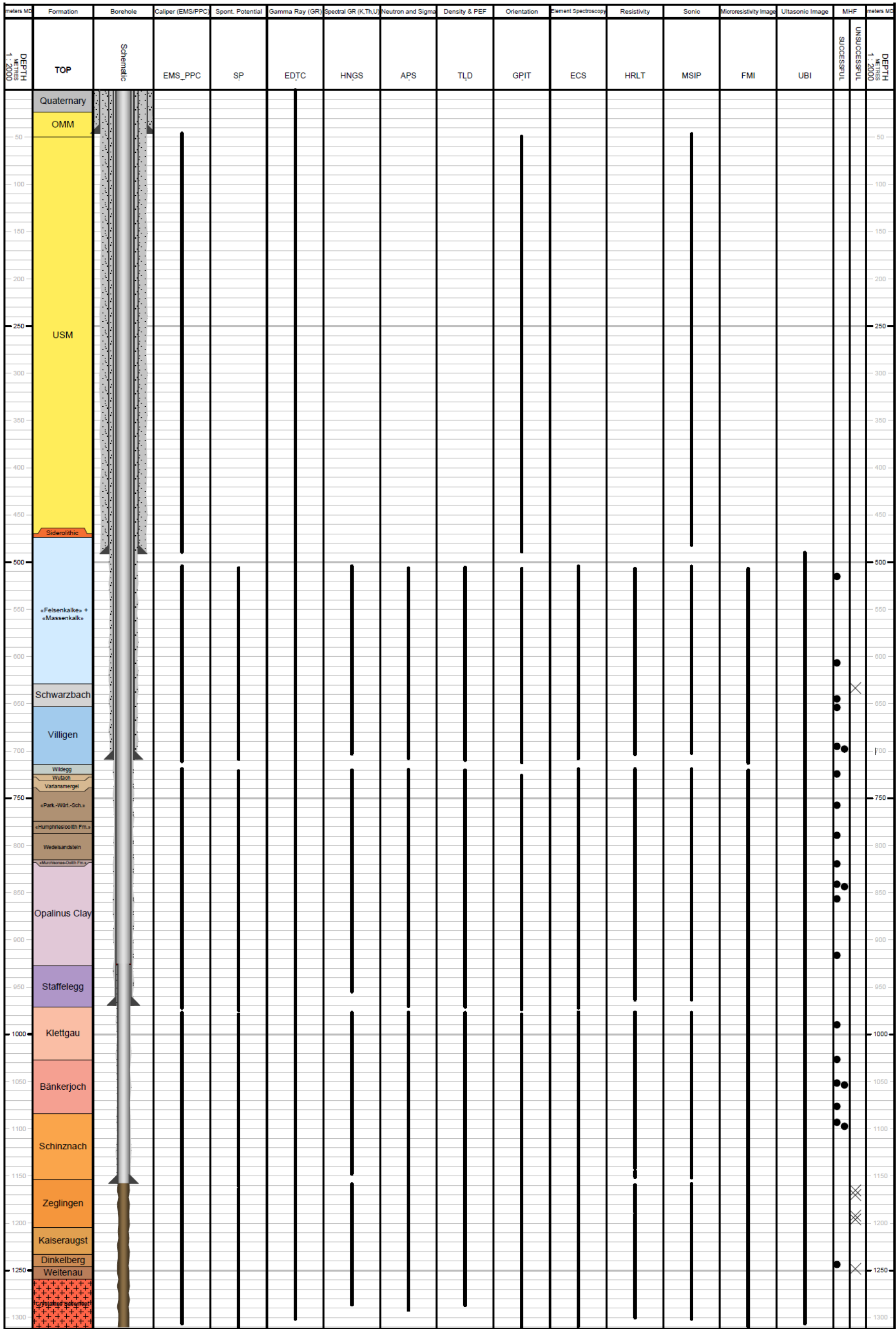
Fig. 2-1: Petrophysical log and MHF testing coverage at TRU1-1 (scale of 1:2'000)
