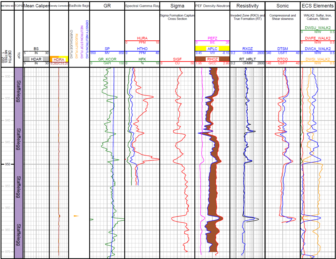
Fig. 3-6: Main logs of the composite dataset in the Staffelegg Formation
