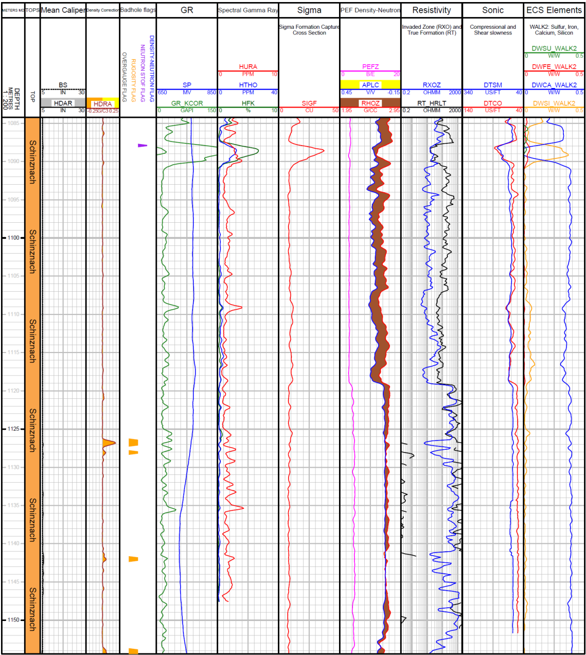
Fig. 3-9: Main logs of the composite dataset in the Schinznach Formation
