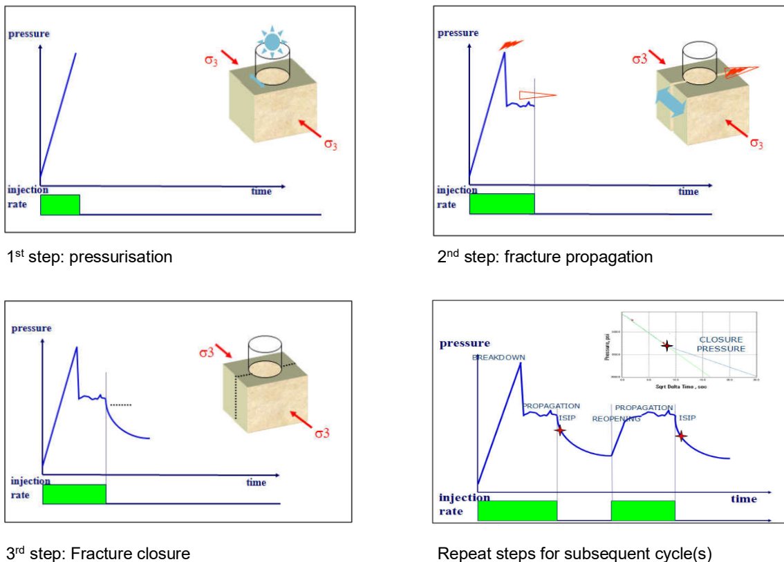
Fig. 5-17: Schematic showing the response of the interval pressure to fluid injection in the interval as a function of time during an MHF test and associated formation response (courtesy of SLB)
