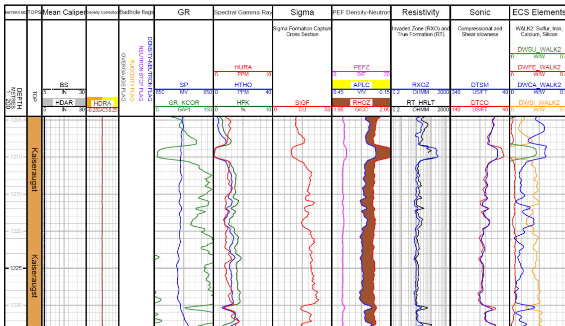
Fig. 3-11: Main logs of the composite dataset in the Kaiseraugst Formation
