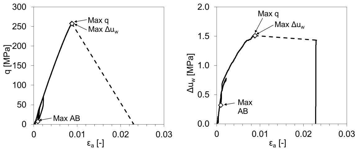
Fig. 5-2: Sample with strong deformation and a very sudden drop of strength post peak Test STA3-1_516_TRX_S1
