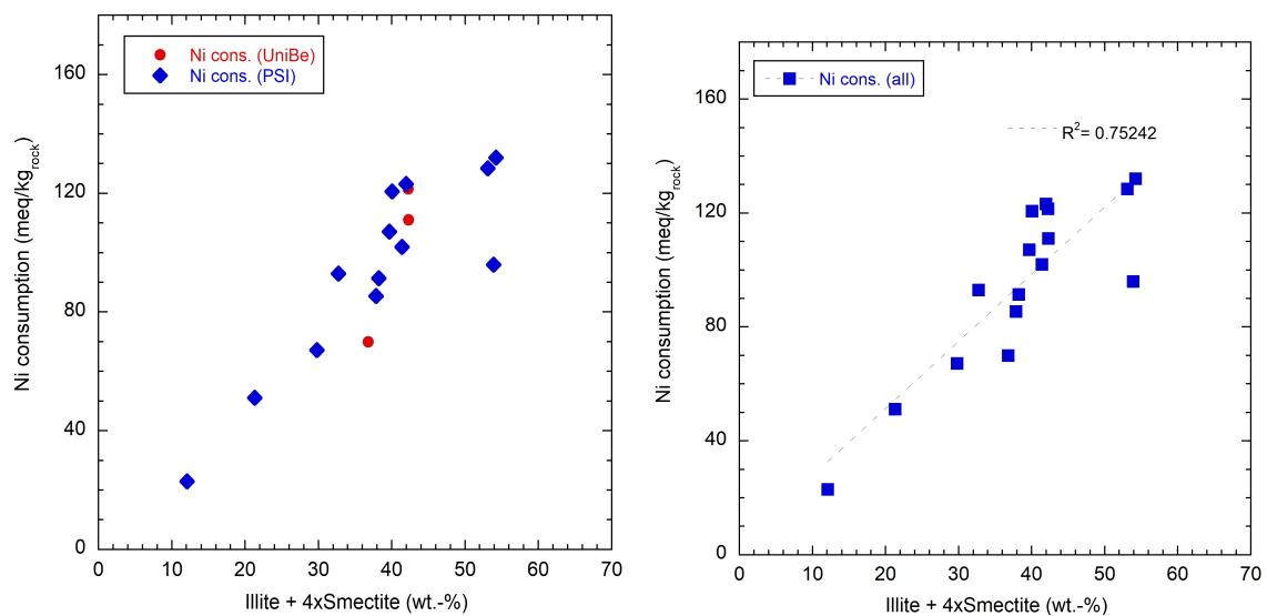
Fig. 5.6-4: Ni consumption as function of the sum of illite end-member content and 4×smectite end-member content
