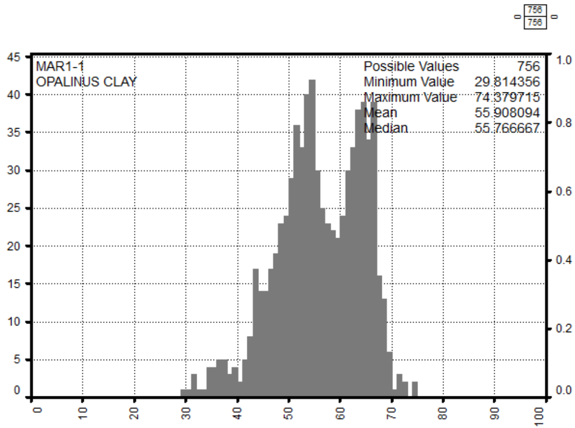
Fig. 4-9: Dry clay weight percentage frequency histogram in the Opalinus Clay X axis is the dry clay weight % from MultiMin, y axis the number of points per bin (100 bins).
