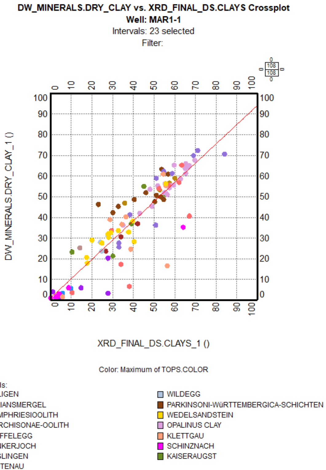
Fig. 4-1: Weight % of dry clay (y-axis) compared to core XRD data (x-axis), Villigen to Weitenau Formations
