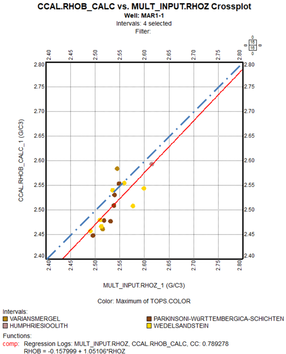
Fig. 4-8: Bulk density computed from core grain density and water loss porosity versus RHOZ in the «Brauner Dogger»
