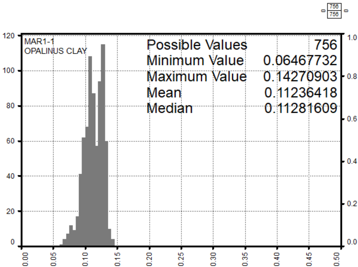
Fig. 4-15: Total porosity frequency histogram in the Opalinus Clay X axis is the total porosity v/v from MultiMin, y axis the number of points per bin (100 bins).
