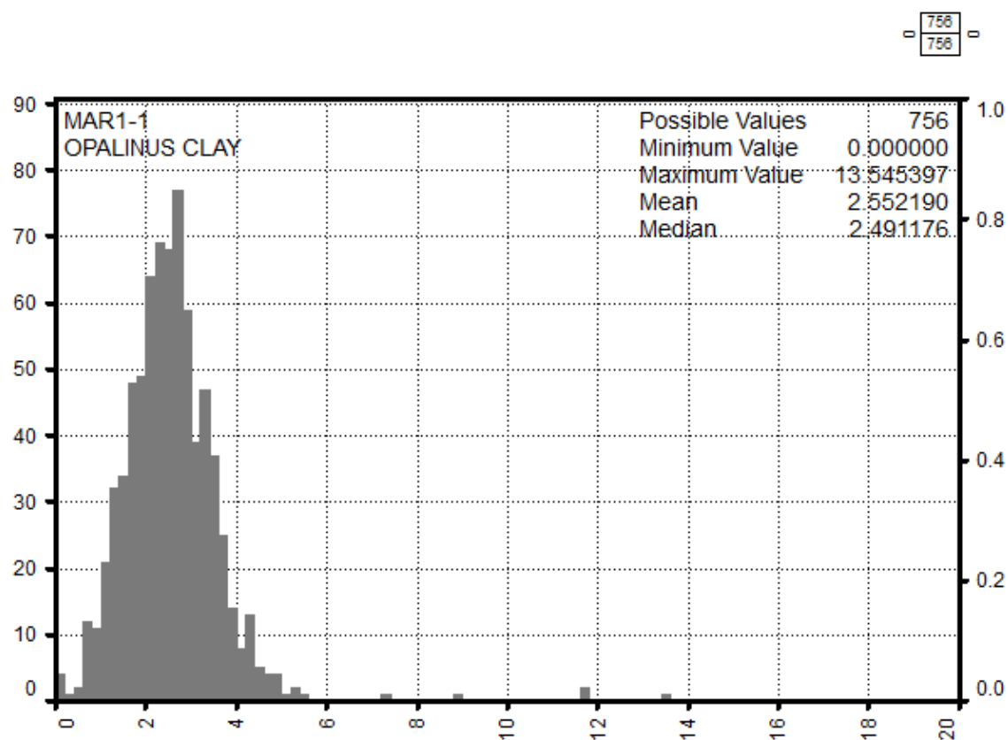
Fig. 4-13: Siderite weight percentage frequency histogram in the Opalinus Clay X axis is the siderite weight % from MultiMin, y axis the number of points per bin (100 bins).
