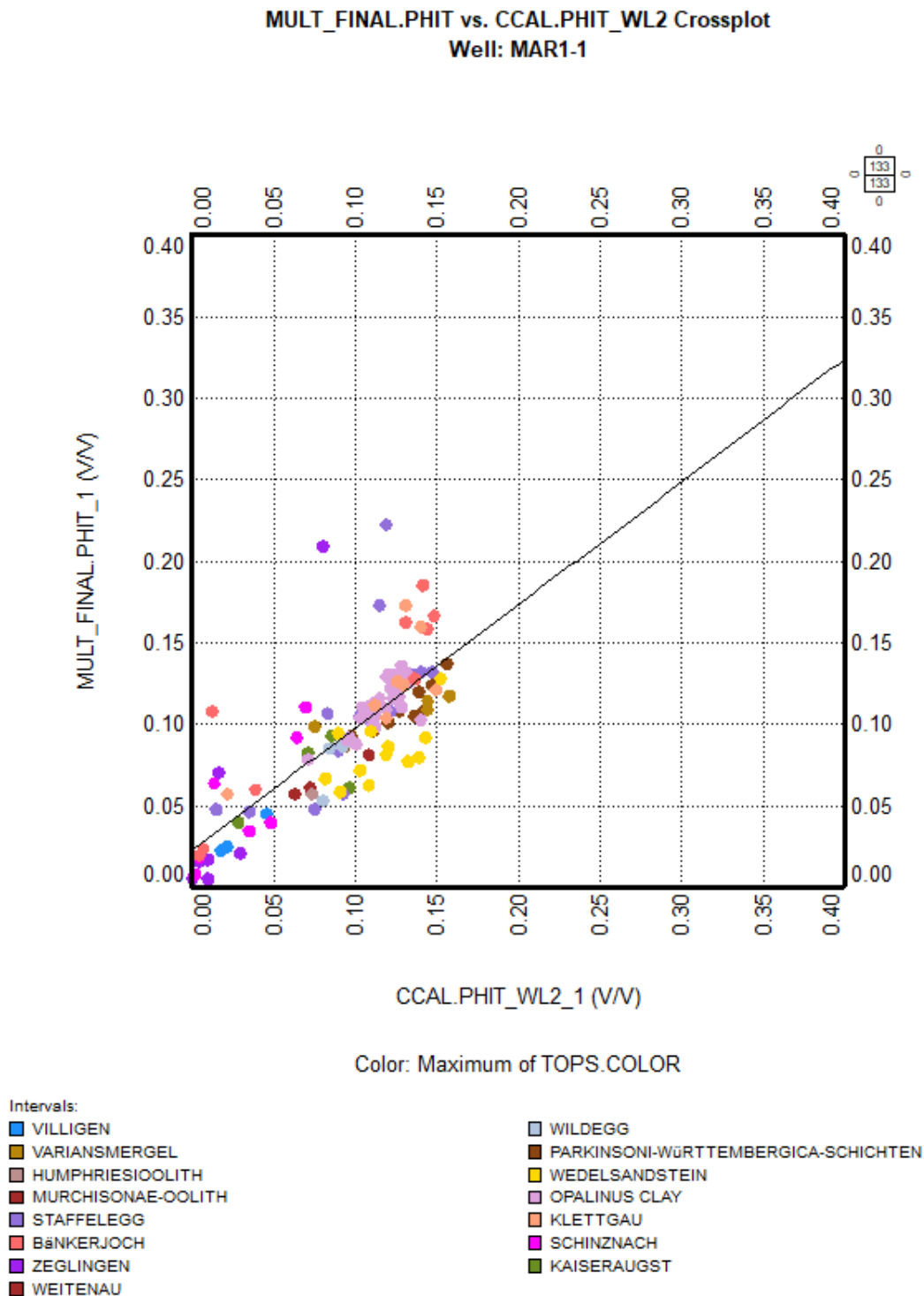
Fig. 4-7: Total porosity (v/v, y axis) compared to core data (x axis), Villigen to Weitenau Formations
