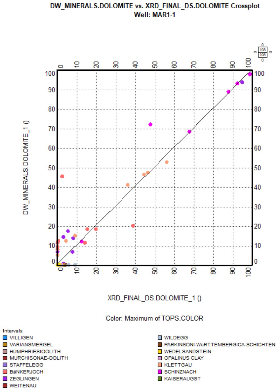
Fig. 4-6: Weight % of dolomite (x axis) compared to core XRD data (y axis), Villigen to Weitenau Formations
