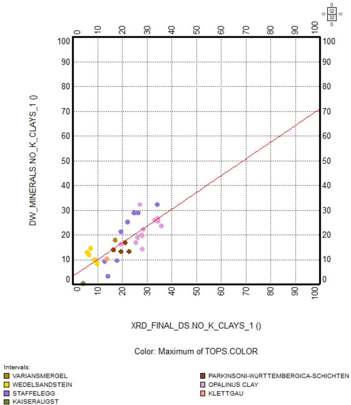
Fig. 4-2: Weight % of not potassic dry clay (y-axis) compared to core XRD data (x-axis), XRD data in the Variansmergel to the Kaiseraugst Formations
