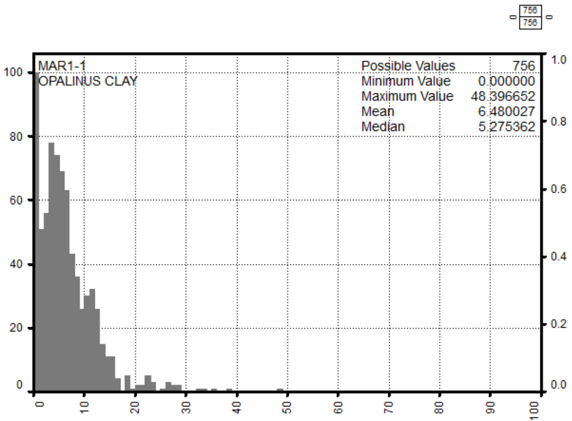
Fig. 4-12: Calcite weight percentage frequency histogram in the Opalinus Clay X axis is the calcite weight % from MultiMin, y axis the number of points per bin (100 bins).
