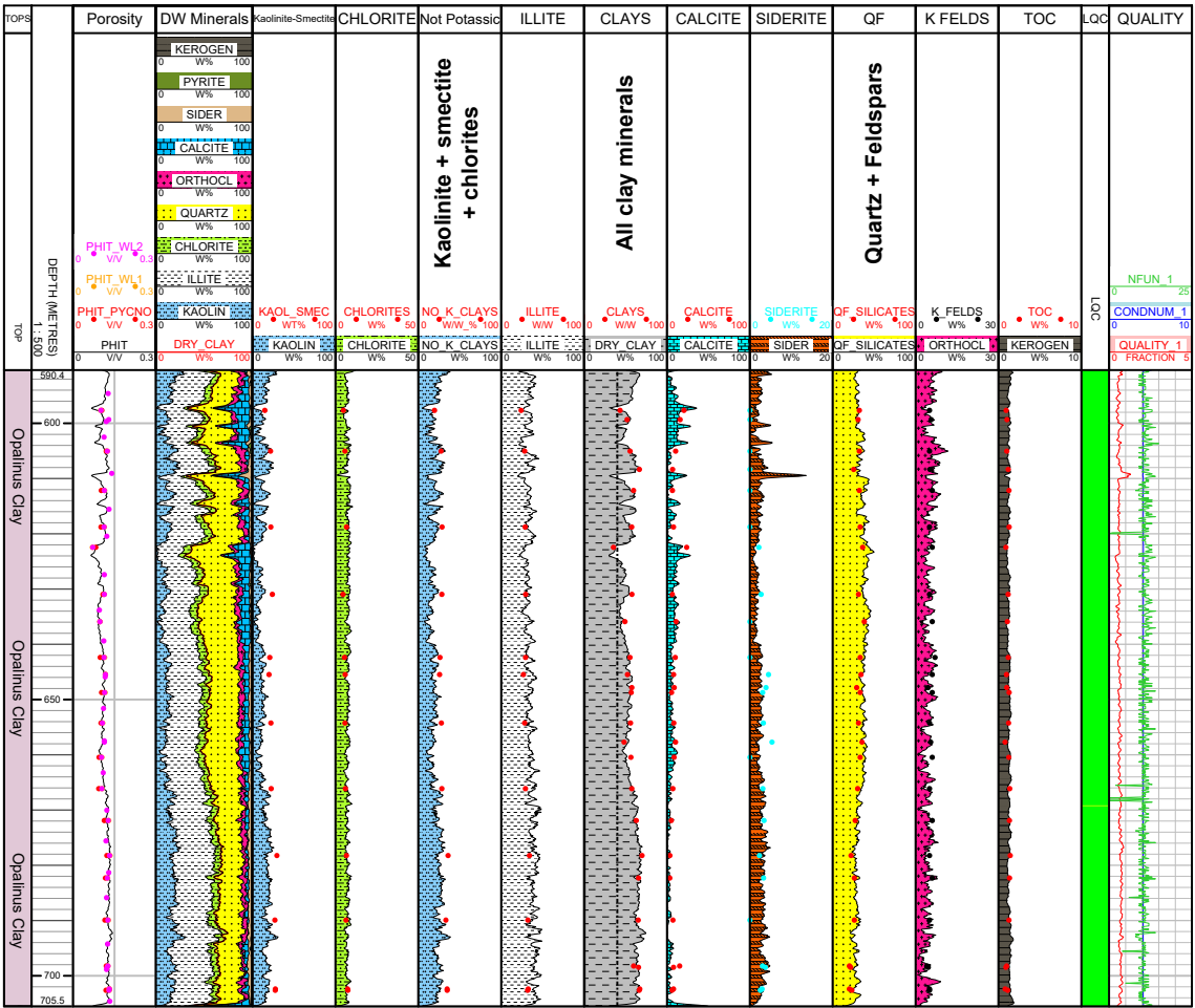
Fig. 4-16: Main log and core results in the Opalinus Clay The black line in the All clay minerals track represents a 40% baseline.
