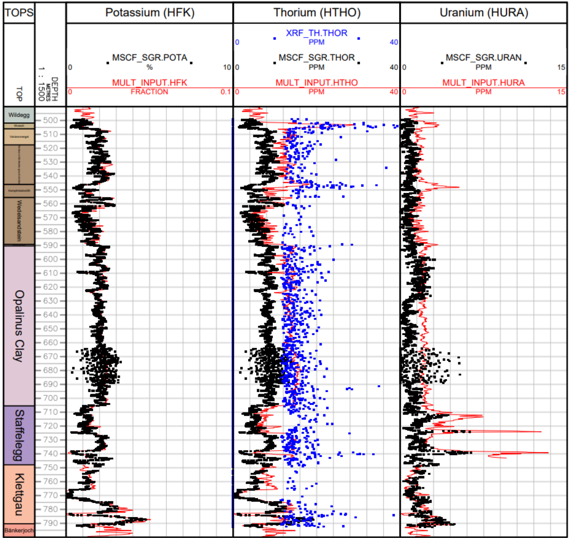
Fig. 2-3: Core (black dots: Spectral Gamma Ray, blue dots: XRF thorium) and wireline HNGS (red curves) Spectral Gamma Ray elements comparison Uranium from the XRF scanner was not measured because it was below the detection limit of the scanner.
