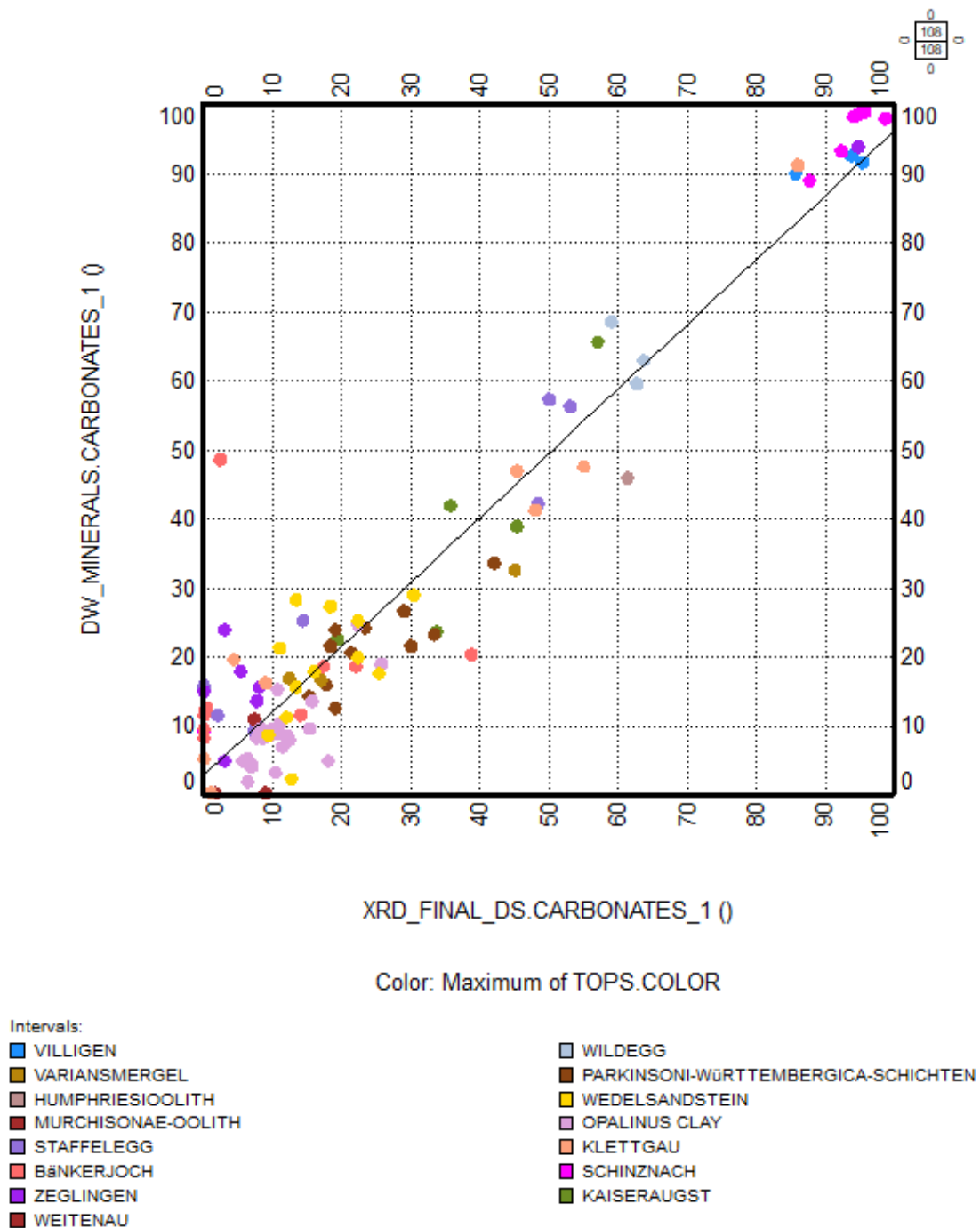
Fig. 4-5: Weight % of carbonates (x axis) compared to core XRD data (y axis), Villigen to Weitenau Formations
