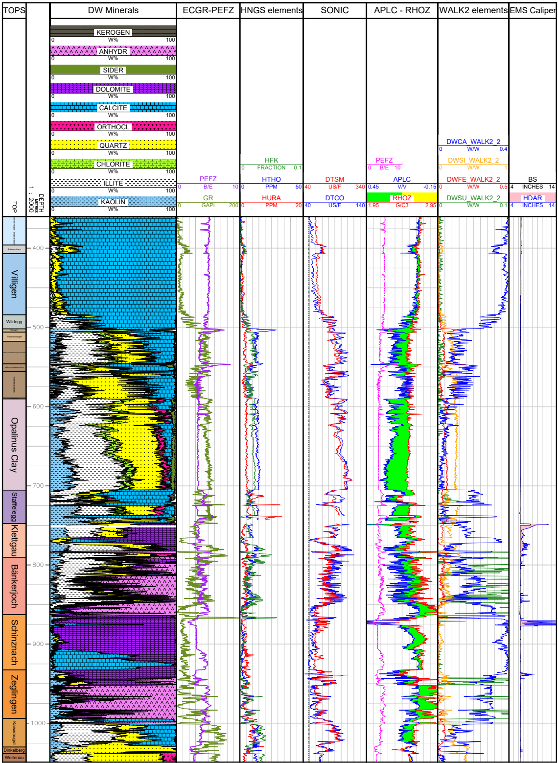
Fig. 2-1: Petrophysical log availability and gaps in the borehole MAR1-1 Please note that ECS elements are displayed as measured (in weight/weight, 0 – 1 w/w range) and are not converted to wt.-% (weight percentage) here.
