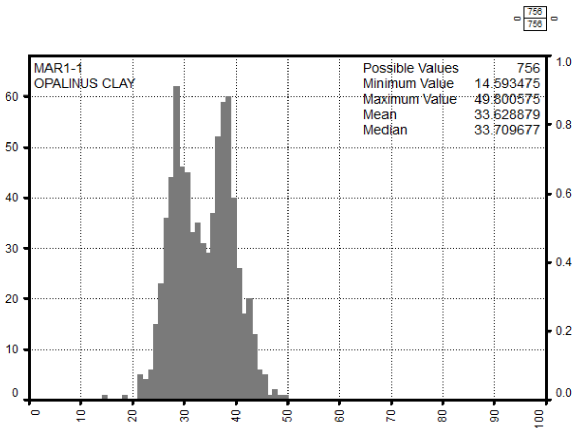
Fig. 4-14: QF-silicates (quartz and feldspars) weight percentage frequency histogram in the Opalinus Clay X axis is the QF-silicates weight % from MultiMin, y axis the number of points per bin (100 bins).
