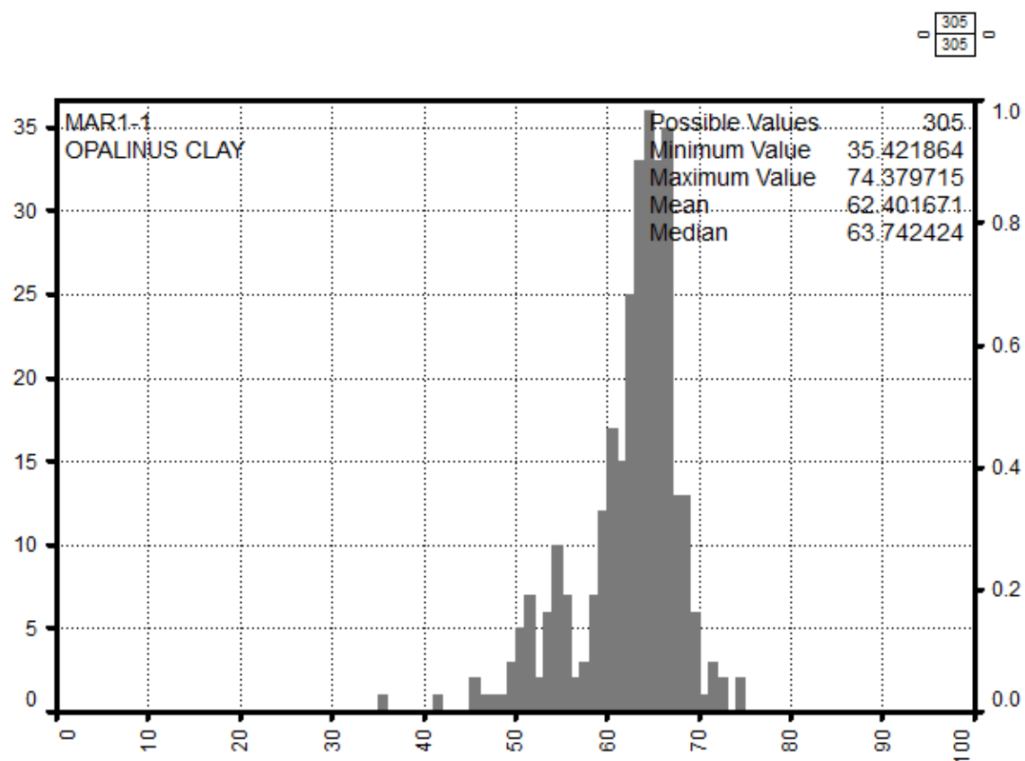
Fig. 4-11: Dry clay weight percentage frequency histogram in the lower section of the Opalinus Clay (below 659 m)
