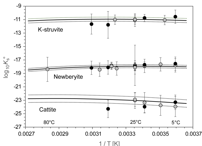
Fig. 4.1-7: The equilibrium constants \log_{10}K_s^\circ for K-struvite, newberyite and cattite (Tab. 4.1-2) as a function of reciprocal absolute temperature in the range 5 – 80 °C
