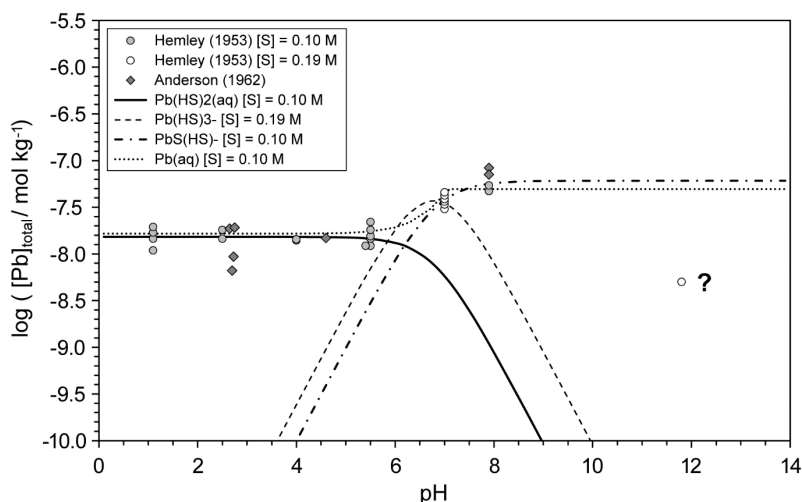
Fig. 12-2: Solubility of PbS(s) in water as a function of pH at different total dissolved sulphide concentrations, [S]_{total}
