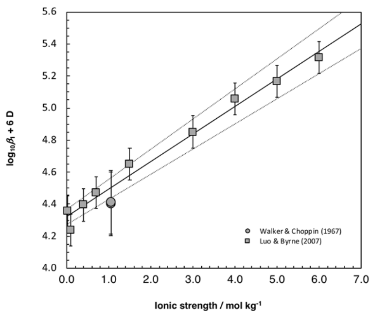
Fig. 23.2.5-2: SIT-plot of the equilibrium \text{Eu}^{3+} + \text{F}^- \rightleftharpoons \text{EuF}^{2+} in \text{NaClO}_4 using the experimental data by Walker & Choppin (1967) and Luo & Byrne (2007)
