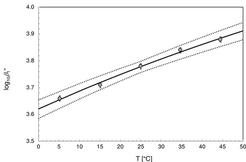
Fig. 23.3.5-4: Stability constants \log_{10}\beta_1^\circ of \text{Ho}^{3+} + \text{F}^- \rightleftharpoons \text{HoF}_2^+ measured by Luo & Millero (2004) in 0.025 M \text{HNO}_3 at various temperatures
