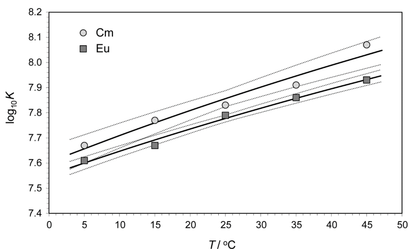
Fig. 25-15: Temperature dependence of the stability constant for the equilibrium (Cm, Eu) 3+ + SiO(OH) 3 - ⇌ (Cm, Eu)SiO(OH) 3 2+
