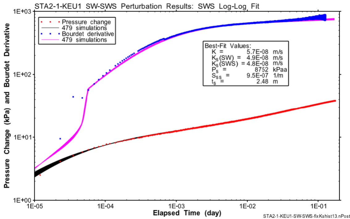
Fig. B-27: Hydraulic test STA2-1-KEU1: Log-log horsetail plot of the SWS of the SW-SWS simulations accepting the fit discriminant 479 / 750 results with a normalised objective function value less than 1.07.
