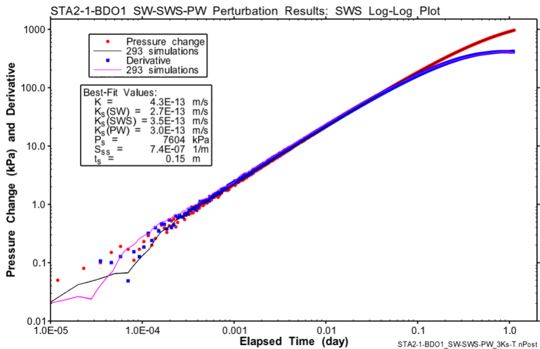
Fig. B-10: Hydraulic test STA2-1-BDO1: Log-log horsetail plot of SWS accepting the fit discriminant
