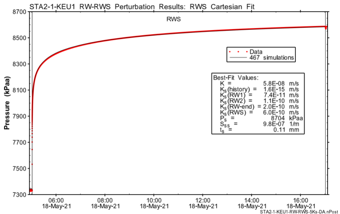
Fig. B-32: Hydraulic test STA2-1-KEU1: Cartesian horsetail plot of the perturbation simulations of the RWS on the RW-RWS accepting the fit discriminant
