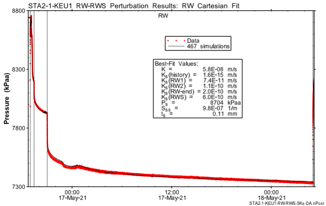
Fig. B-31: Hydraulic test STA2-1-KEU1: Cartesian horsetail plot of the perturbation simulations of the RW on the RW-RWS accepting the fit discriminant
