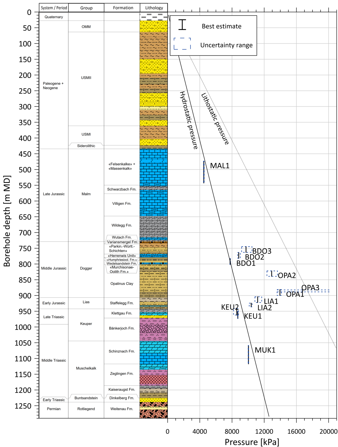
Fig. 4-26: Summary of hydraulic testing in borehole STA2-1: Static formation pressure profile The lithostatic pressure is based on the assumption of a mean density of 2'000 \text{ kg m}^{-3} . Tests STA2-1-OPA2 and STA2-1-OPA4 were performed in comparable test intervals. Due to artificially induced overpressures, test STA2-1-OPA4 did not provide representative hydraulic parameters.
