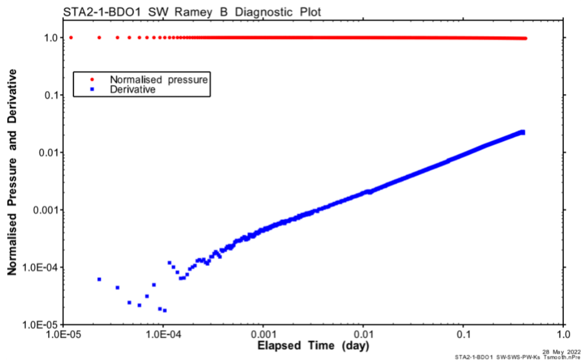
Fig. B-2: Hydraulic test STA2-1-BDO1: Ramey B diagnostic plot of the SW phase
