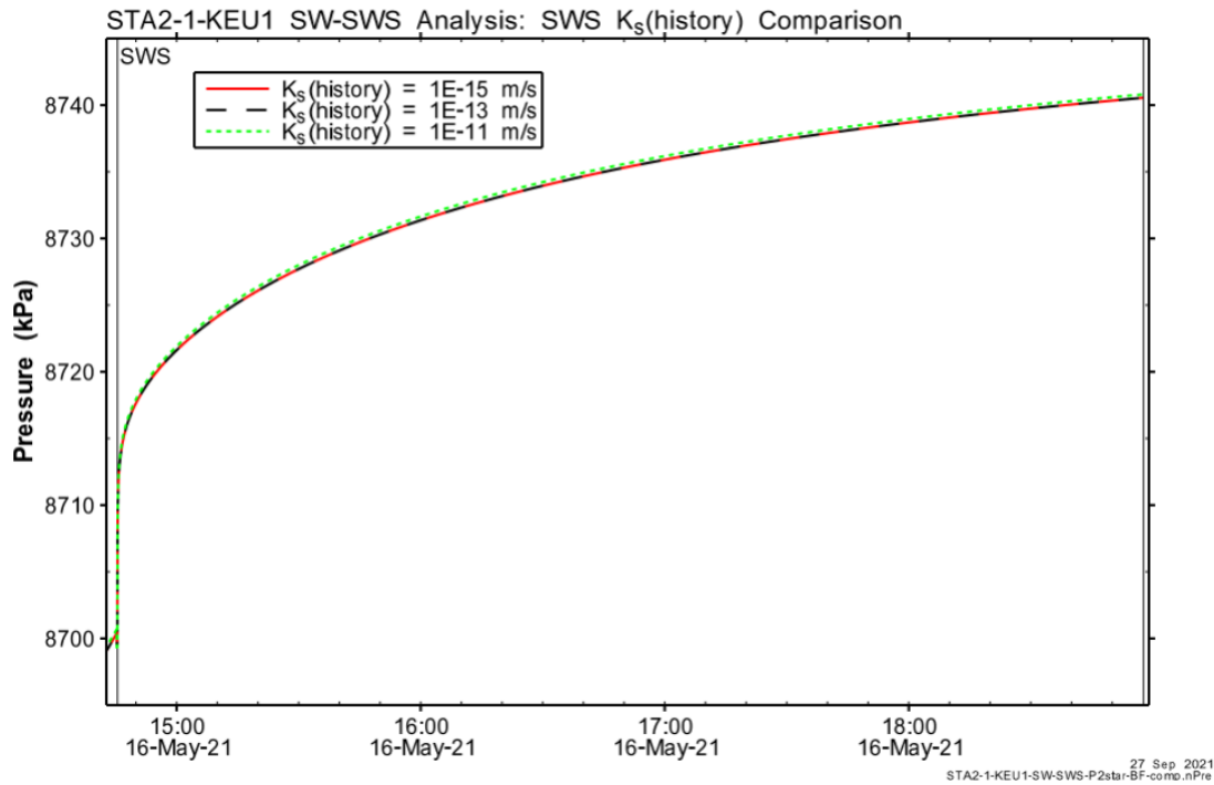
Fig. B-35: Hydraulic test STA2-1-KEU1: SWS phase of simulations of the SW-SWS with different values of K_s (history)
