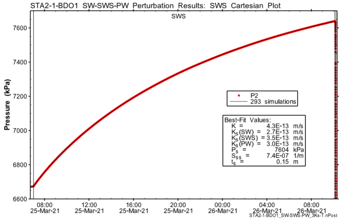
Fig. B-9: Hydraulic test STA2-1-BDO1: Cartesian horsetail plot of the perturbation simulations on SWS accepting the fit discriminant
