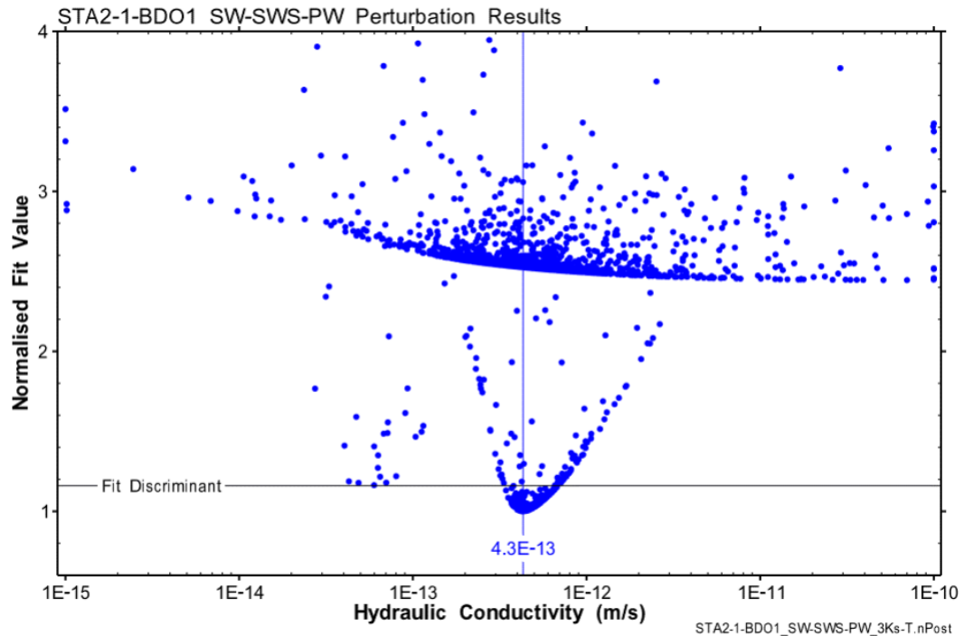
Fig. B-5: Hydraulic test STA2-1-BDO1: Distribution of the normalised objective function value over K for the numerical simulation of the SW-SWS-PW
