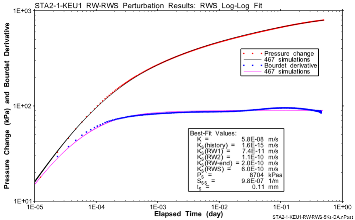
Fig. B-33: Hydraulic test STA2-1-KEU1: Log-log horsetail plot of RWS of the RW-RWS simulations accepting the fit discriminant
