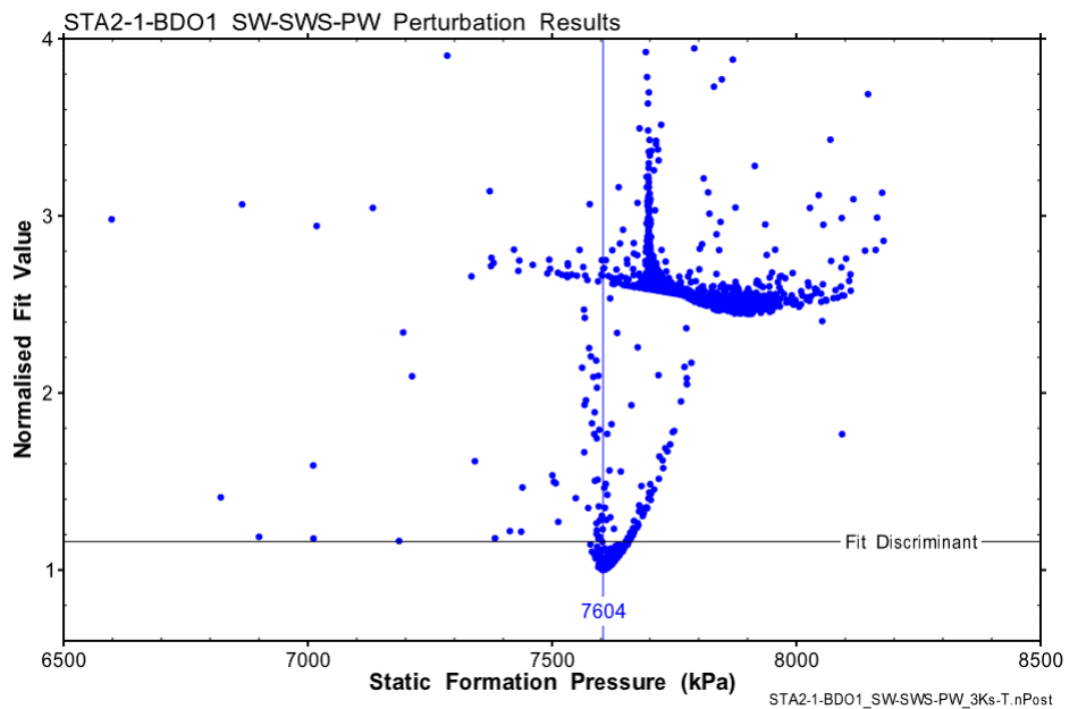
Fig. B-6: Hydraulic test STA2-1-BDO1: Distribution of the normalised objective function value over P_f for the numerical simulation of the SW-SWS-PW
