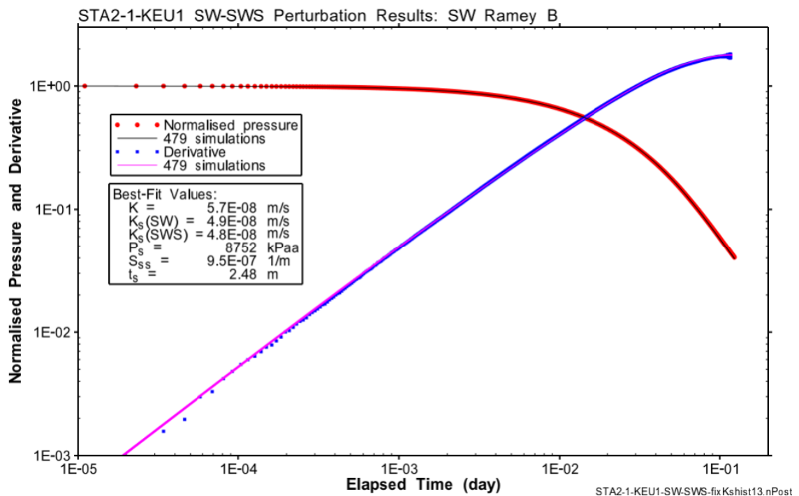
Fig. B-26: Hydraulic test STA2-1-KEU1: Ramey B horsetail plot of the SW of the SW-SWS simulations accepting the fit discriminant
