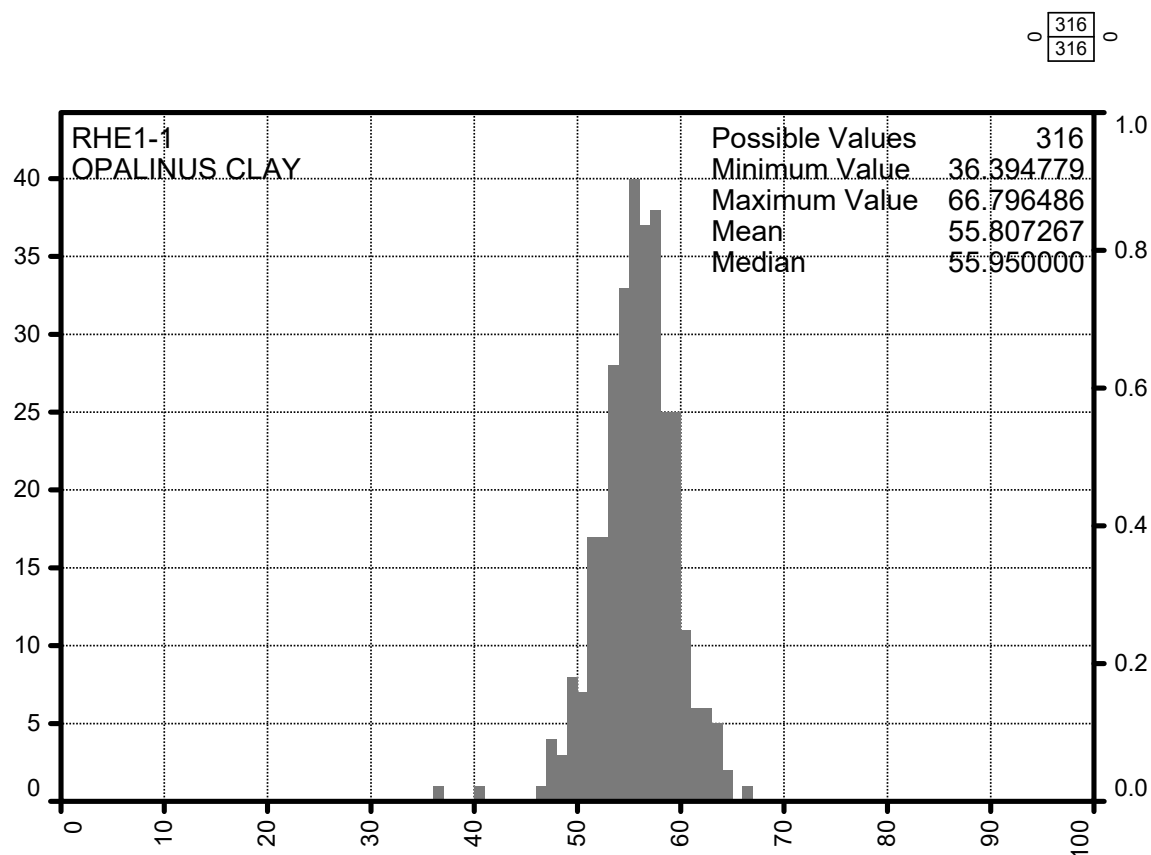
Fig. 4-3: Dry clay weight-percentage frequency histogram in the lower section of the Opalinus Clay (below 620 m) X-axis is the dry clay wt.-% from MultiMin, y-axis the number of points per bin (100 bins).
