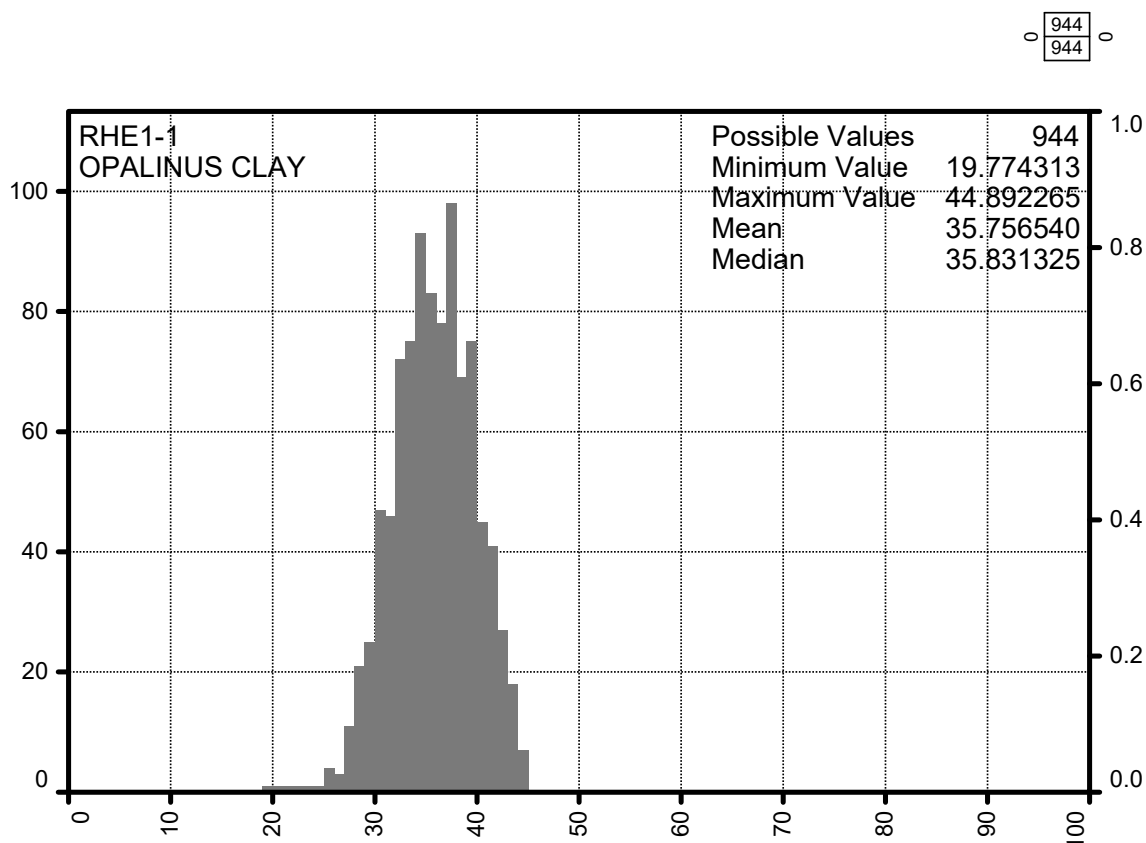
Fig. 4-6: QF-silicates (quartz and feldspars) weight percentage frequency histogram in the Opalinus Clay
