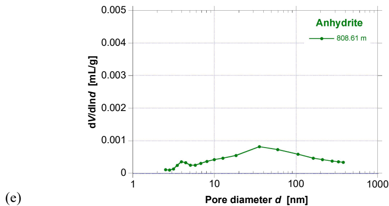
Fig. 4.3-19: Distribution of (external) pore sizes derived from N_2 desorption
