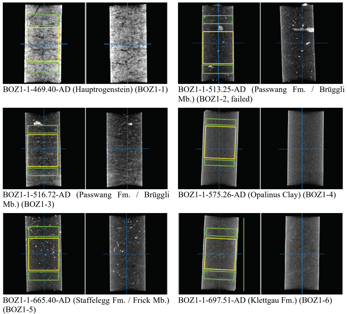
Fig. 4.7-2: X-ray CT images of AD samples
