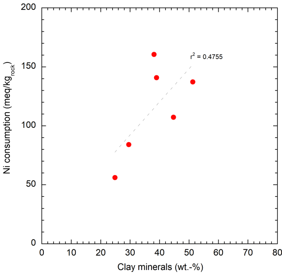
Fig. 4.5-2: Ni consumption vs. clay-mineral content
