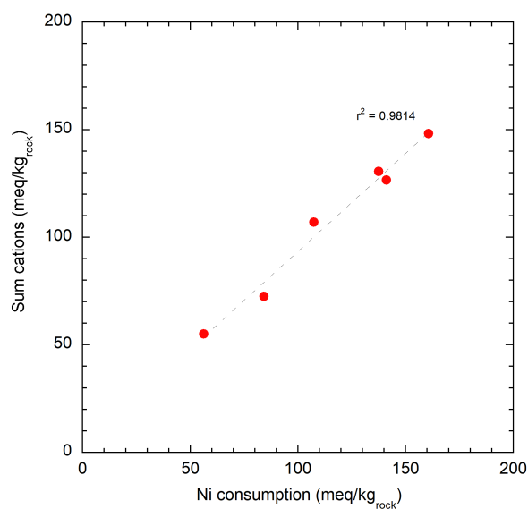
Fig. 5.6-1: Ni consumption vs. corrected sum of cations (data of Uni Bern)
