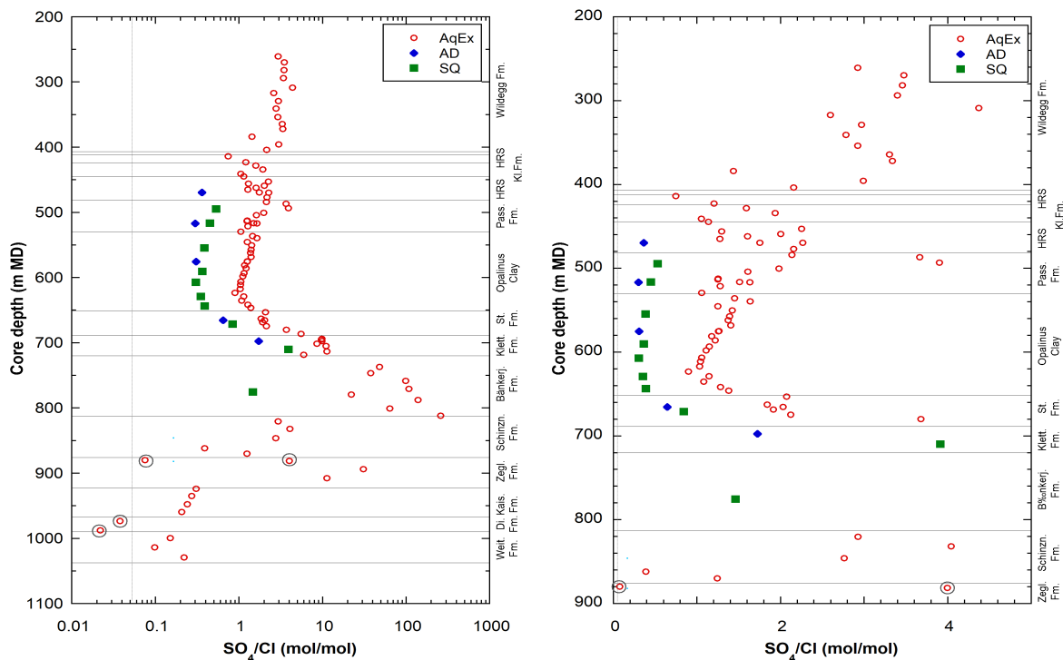
Fig. 5.3-3: Profiles showing molar \text{SO}_4/\text{Cl} ratios obtained from different methods in logarithmic and linear concentration scales
