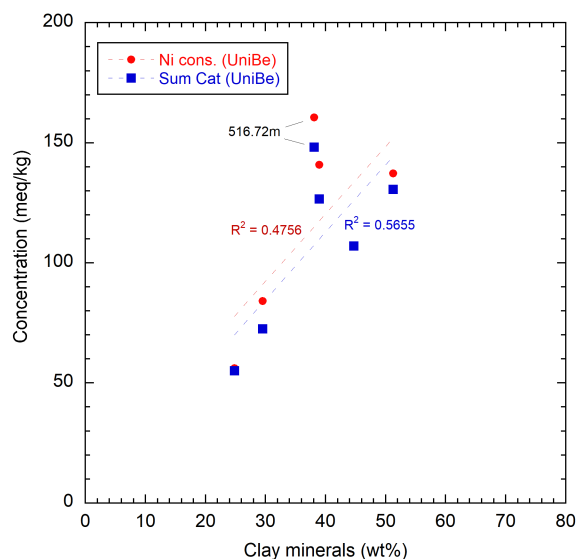
Fig. 5.6-2: Cation exchange capacity (Ni consumption and corrected sum of cations) as a function of the clay-mineral content (data of Uni Bern)
