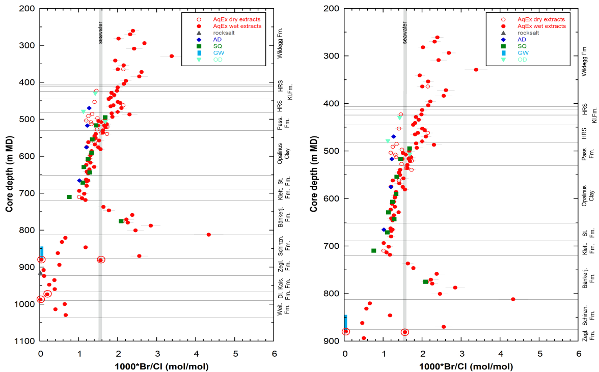
Fig. 5.2-5: Br*1000/Cl ratios (mol/mol) at two different depth scales with data from squeezing, advective displacement, aqueous extraction, out-diffusion and rock salt (from BUL1-1) samples
