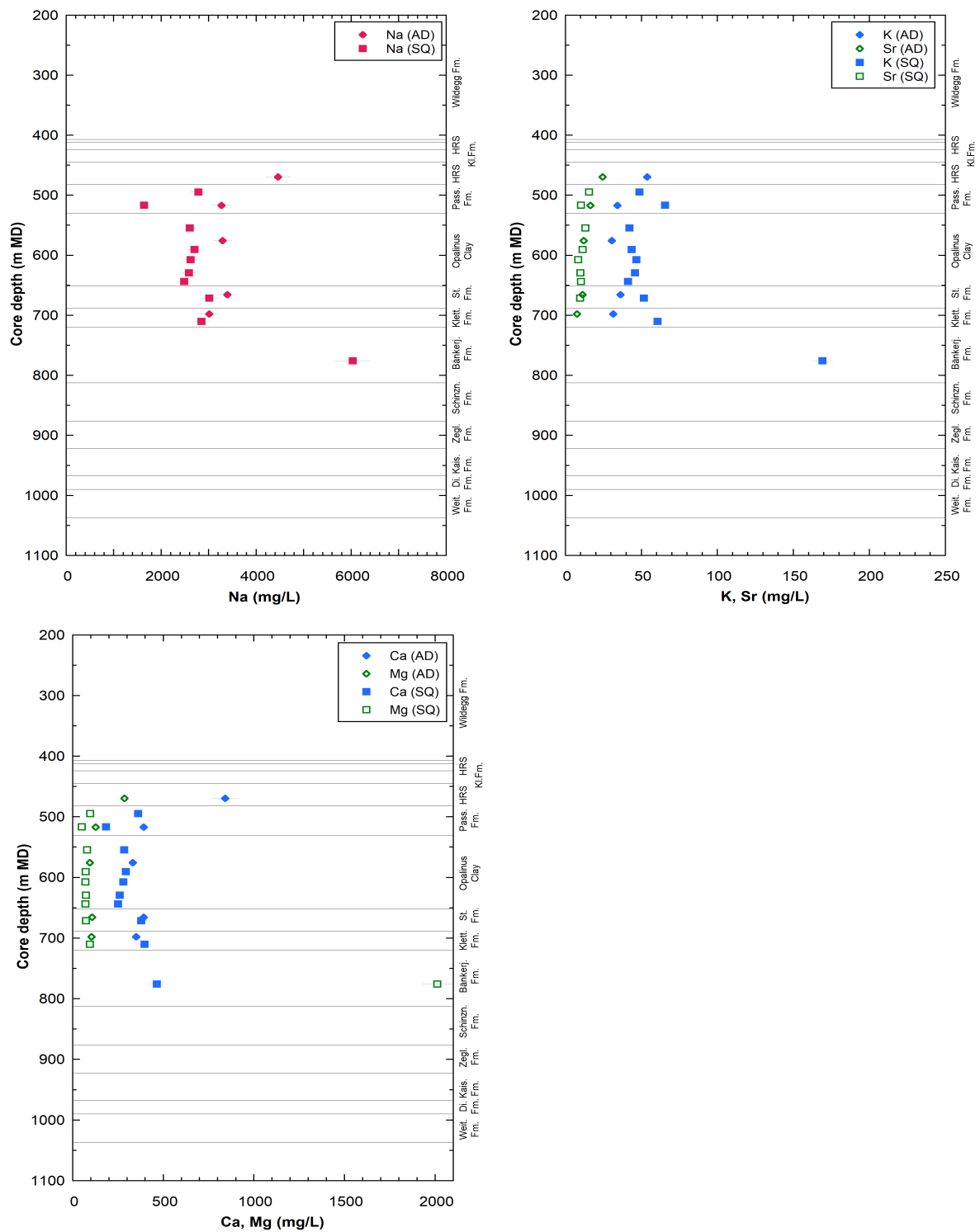
Fig. 5.4-1: Profiles for Na, Ca, Mg, K and Sr in porewater with data from squeezing, advective displacement
