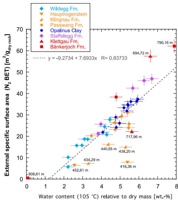
Fig. 4.3-15: Specific surface area ( S_{\text{BET}} ) derived from \text{N}_2 adsorption plotted against the gravimetric water content relative to the dry mass of the samples
