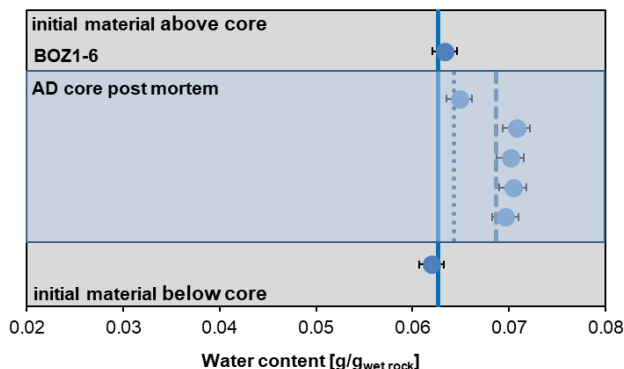
Fig. 4.7-3: Details of water content measurements before and after AD experiments
