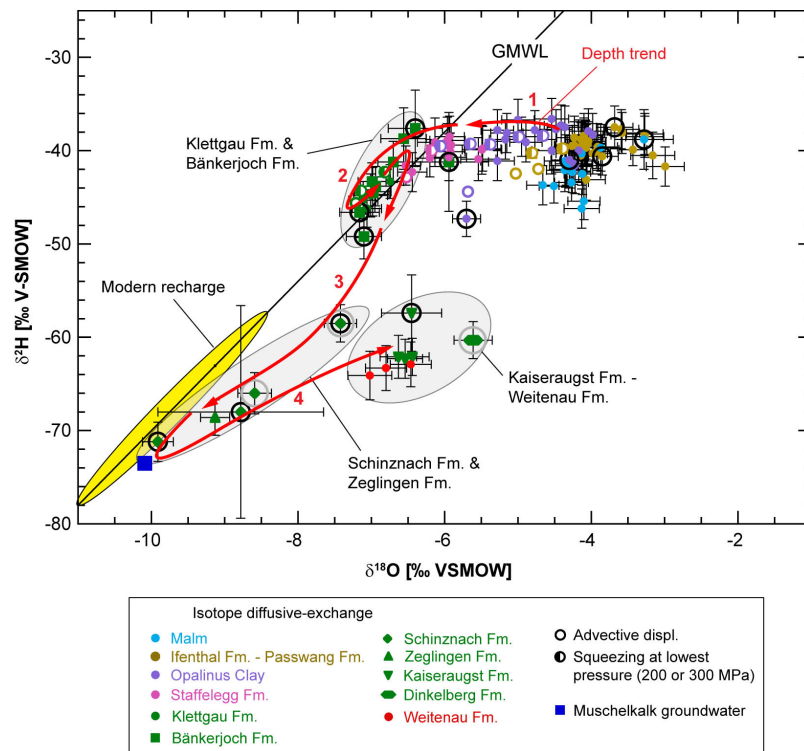
Fig. 5.7-2: \delta^2\text{H} vs. \delta^{18}\text{O} for groundwater and porewater derived by all techniques
