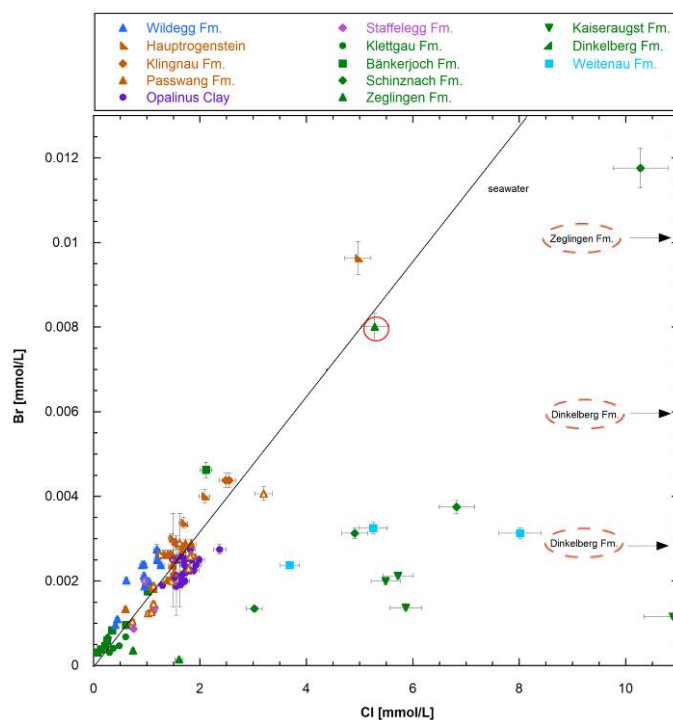
Fig. 4.4-1: Molar Br versus Cl concentrations in aqueous extracts at a S/L ratio of about 1
