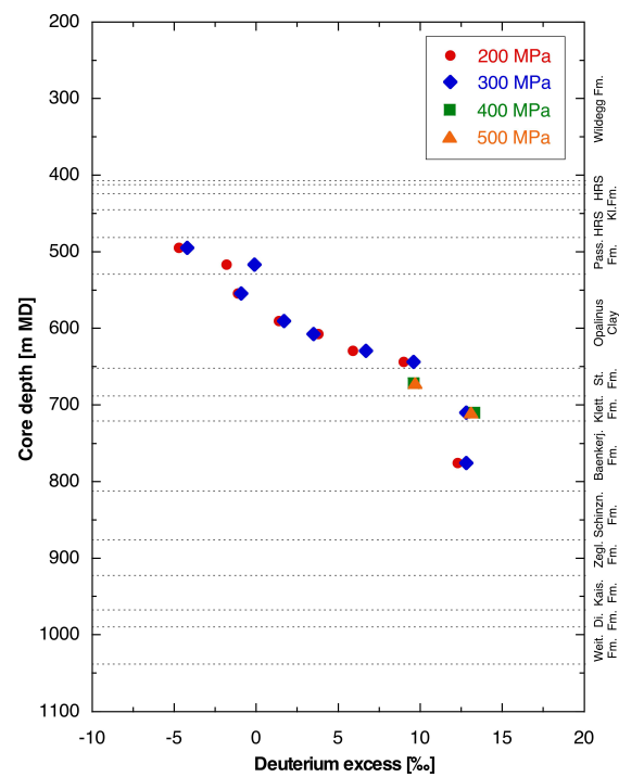
Fig. 4.6-8: Depth trend of deuterium excess in squeezed waters
