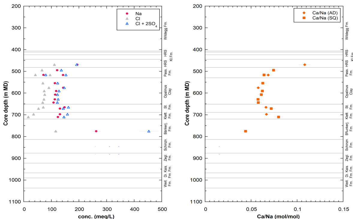
Fig. 5.4-2: Profiles for Na, Cl and \Sigma\text{Cl}+\text{SO}_4 in porewater (SQ and AD samples) in meq/L (left), Ca/Na ratio (molar units) for SQ and AD samples (right)
