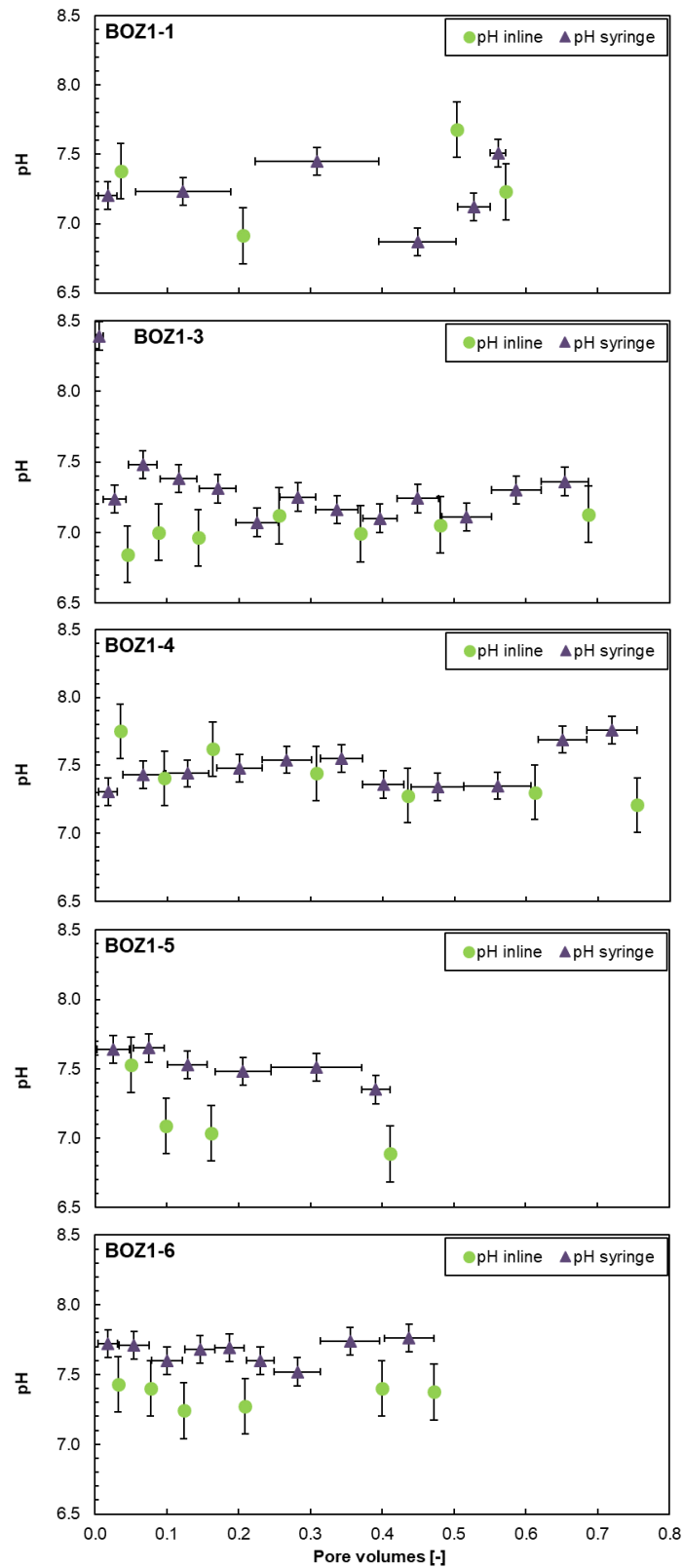
Fig. 4.7-14: Evolution of pH during advective displacement experiments
