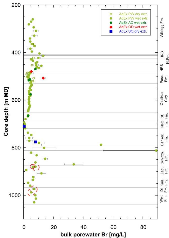
Fig. 4.4-8: Bulk porewater Br concentrations versus depth from aqueous extracts
