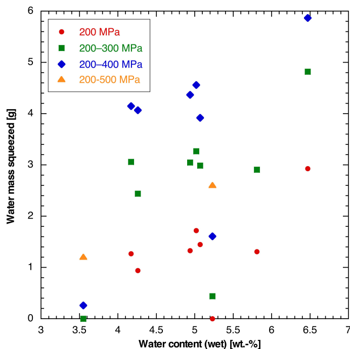
Fig. 4.6-2: Correlation of the original water content and the cumulative water mass obtained by squeezing
