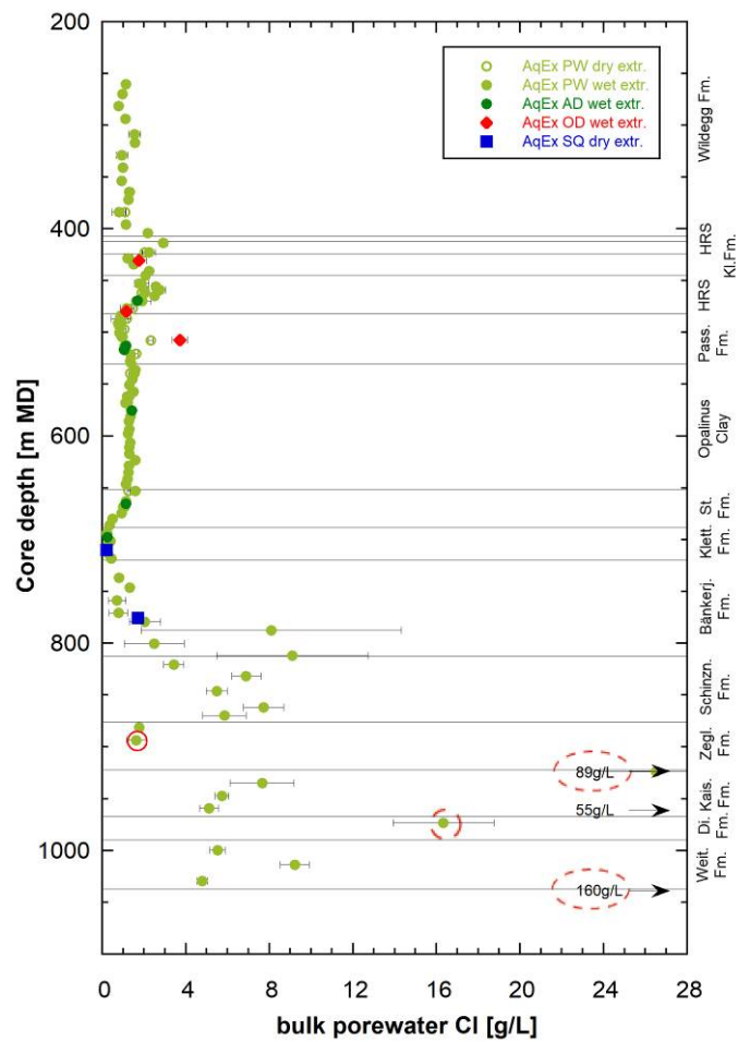
Fig. 4.4-6: Bulk porewater Cl concentrations versus depth from aqueous extracts
