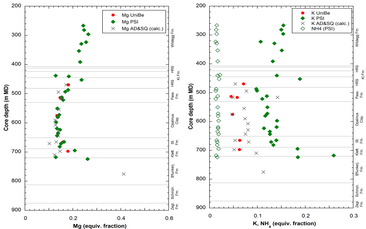
Fig. 5.6-7: Mg (left) and K, NH 4 (right) occupancies according to Uni Bern and PSI data and values calculated from AD/SQ data
