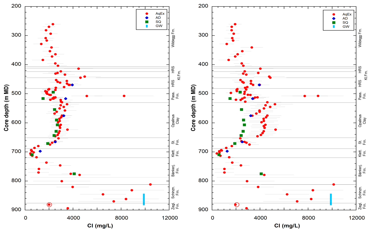
Fig. 5.2-2: Alternative Cl profiles based on f_{Cl} from squeezing data (left) and from diffusion data (right) (see text)
