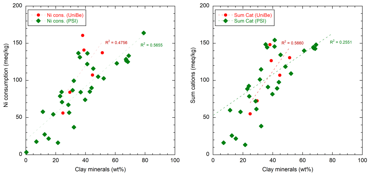
Fig. 5.6-4: CEC data as function of the clay-mineral content; left: Ni consumption data; right: Corrected sum of cations
