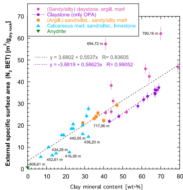
Fig. 4.3-16: Relation between external specific surface area ( S_{\text{BET}} ) derived from \text{N}_2 adsorption and content of clay minerals
