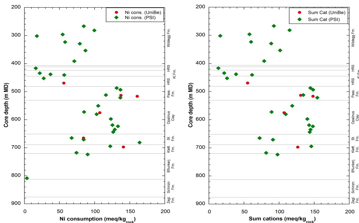
Fig. 5.6-3: Comparison of CEC data from Uni Bern and from PSI; Ni consumption data (left) and (corrected) sum of cations data (right)
