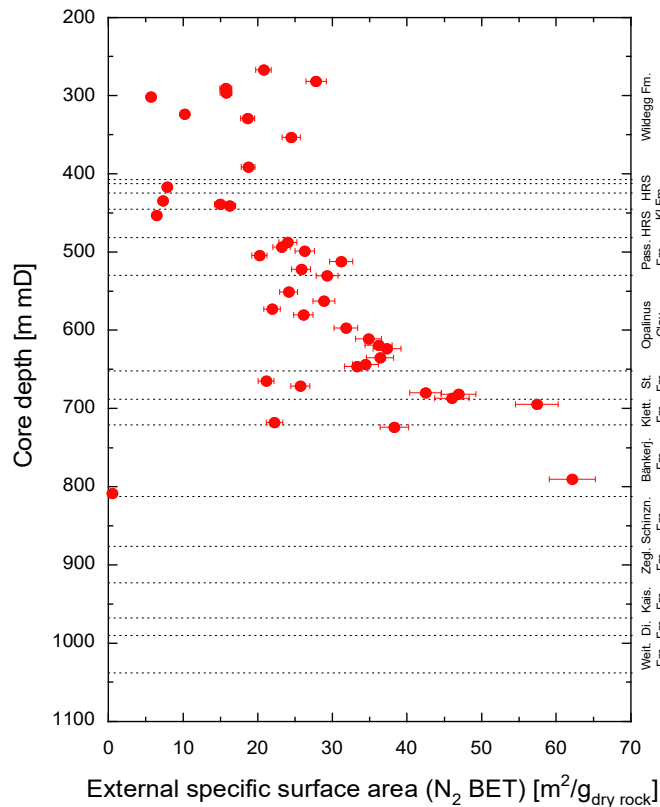
Fig. 4.3-14: Depth profile of specific surface area ( S_{\text{BET}} ) derived from \text{N}_2 adsorption
