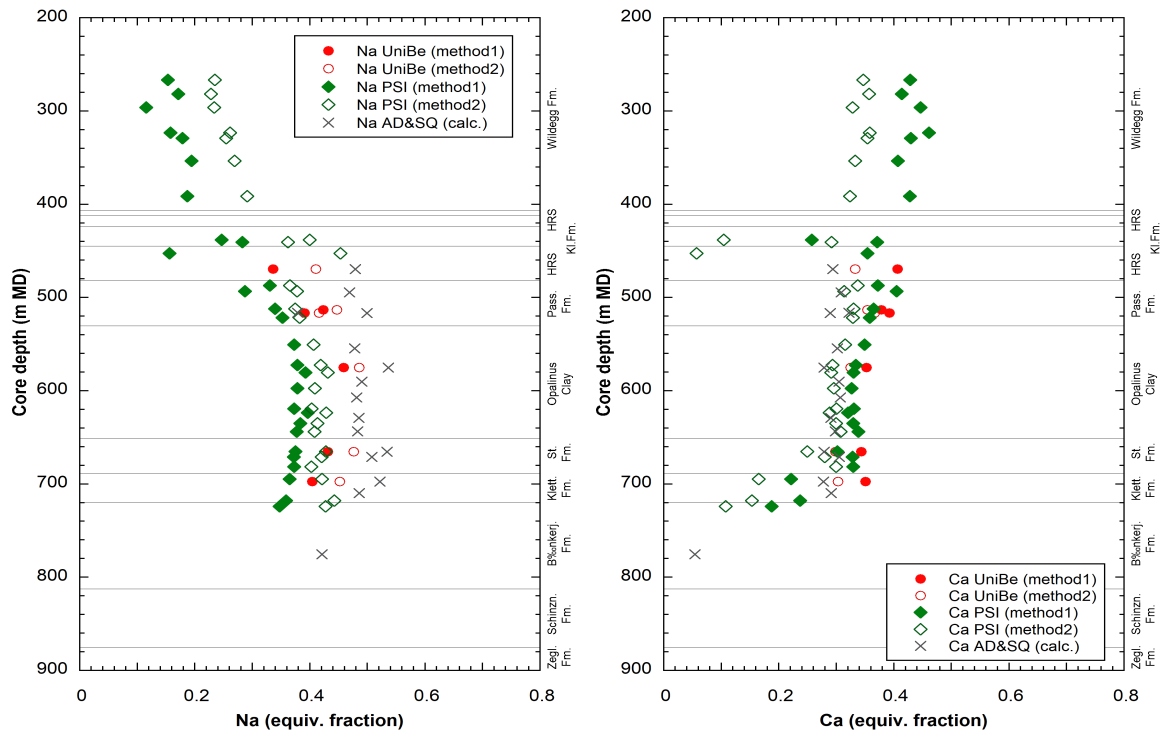
Fig. 5.6-6: Na (left) and Ca (right) occupancies according to Uni Bern and PSI data and calculated from AD/SQ data
