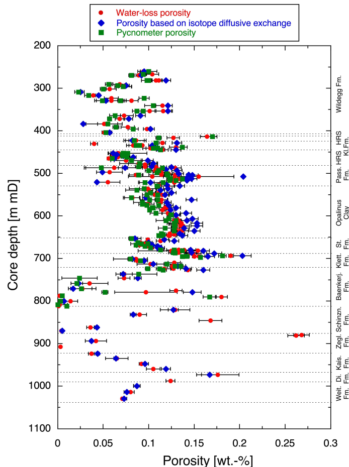
Fig. 4.3-11: Depth trends of porosities obtained by different methods
