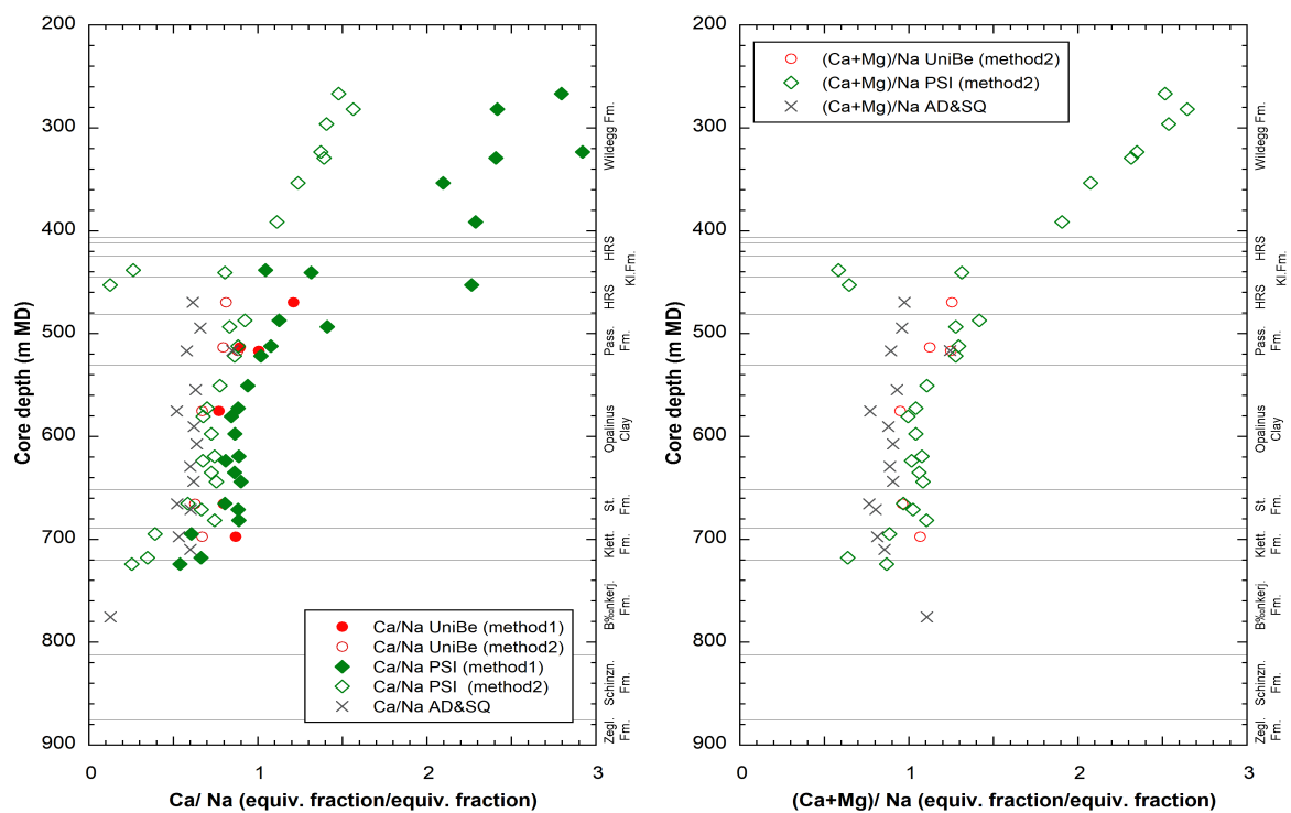
Fig. 5.6-9: Ca/Na ratios (left) and (Ca+Mg)/Na (right) according to Uni Bern and PSI data and calculated from AD/SQ data
