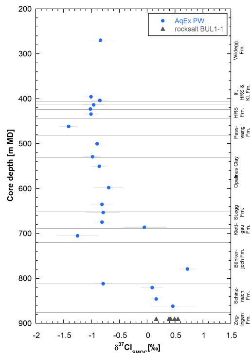
Fig. 5.2-3: Profile of \delta^{37}\text{Cl} with data from aqueous extraction
