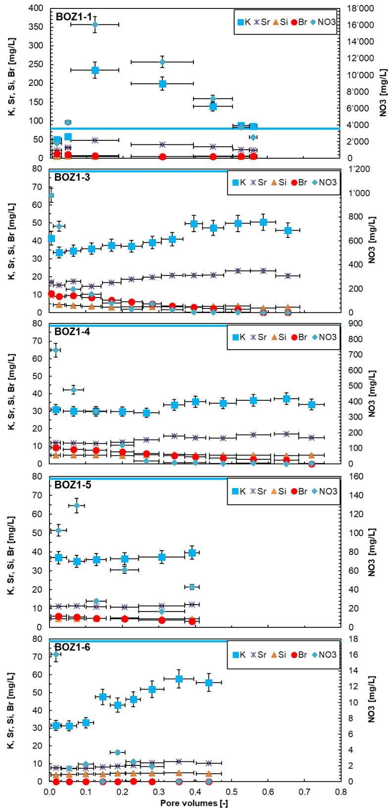
Fig. 4.7-10: Evolution of minor components during advective displacement experiments
