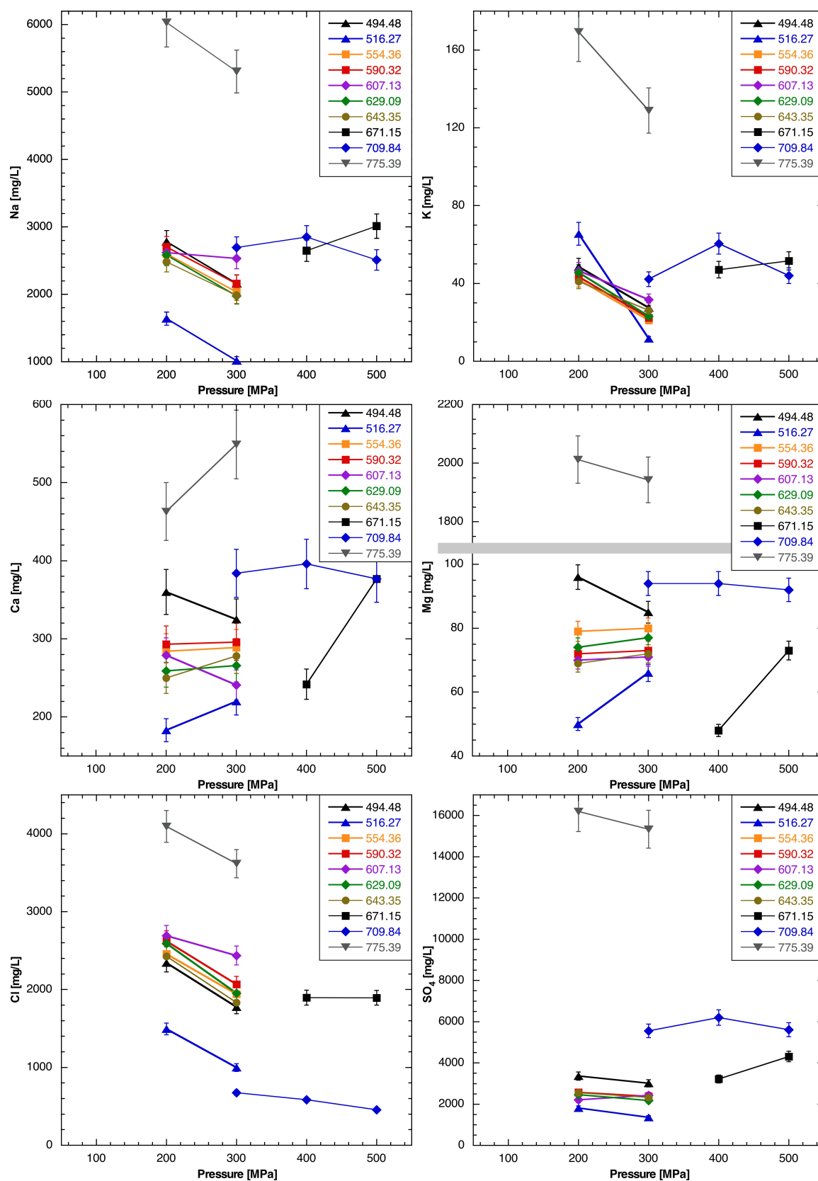
Fig. 4.6-3: Ion concentrations in squeezed waters as a function of squeezing pressure Bars indicate analytical errors of ion-chromatography analysis. Grey bar in the plot for Mg separates two y-axis ranges.
