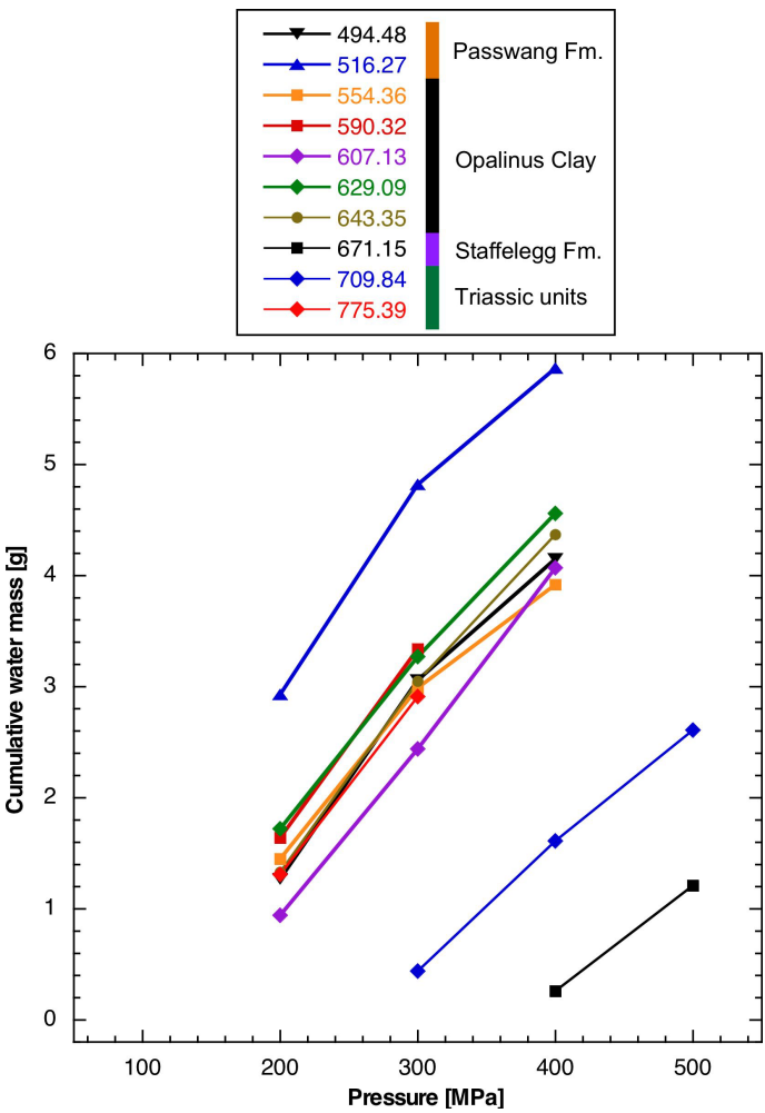
Fig. 4.6-1: Cumulative water masses obtained by squeezing as a function of the squeezing pressure
