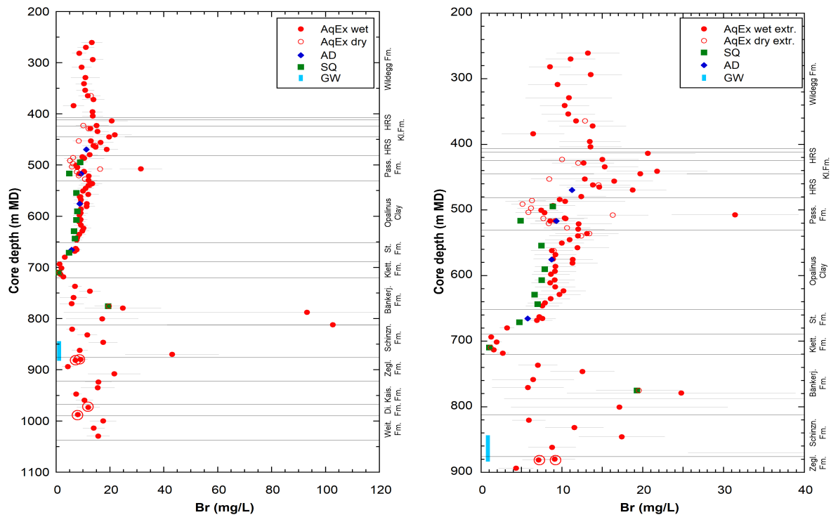
Fig. 5.2-4: Br with data at two different depth scales from squeezing, advective displacement, aqueous extraction and groundwater samples
