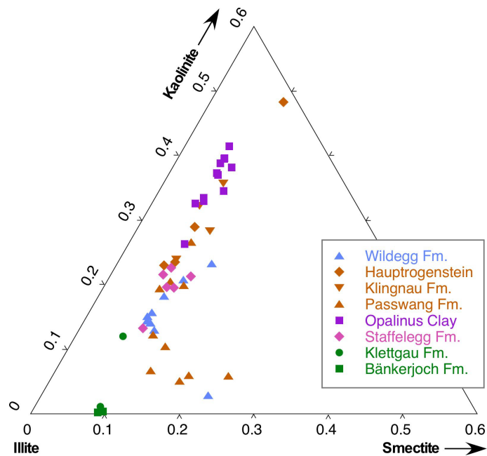
Fig. 4.2-6: Relative mass proportions of illite, smectite and kaolinite end-member clays
