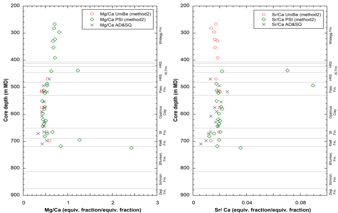
Fig. 5.6-10: Mg/Ca ratios (left) and Sr/Ca ratios (right) according to Uni Bern and PSI data and calculated from AD/SQ data
