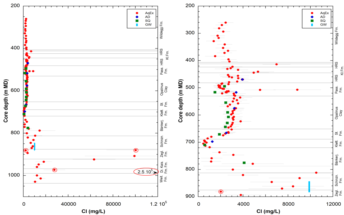
Fig. 5.2-1: Cl profiles at different scales (depth and concentration) with data from squeezing, advective displacement, aqueous extraction, and groundwater samples
