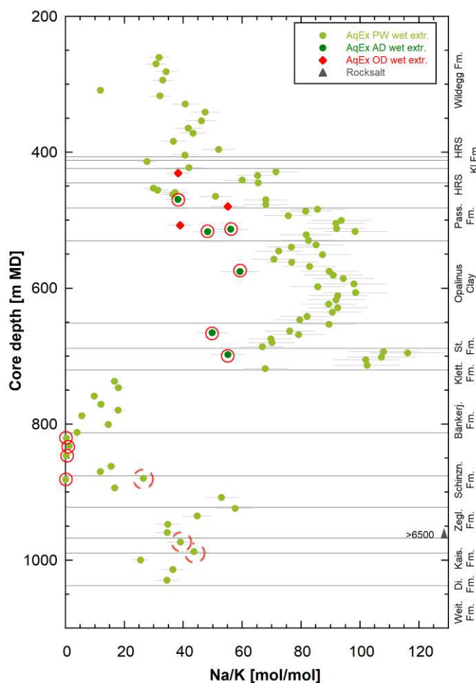
Fig. 4.4-5: Depth versus Na/K molar concentration ratio in aqueous extracts at a S/L ratio of about 1
