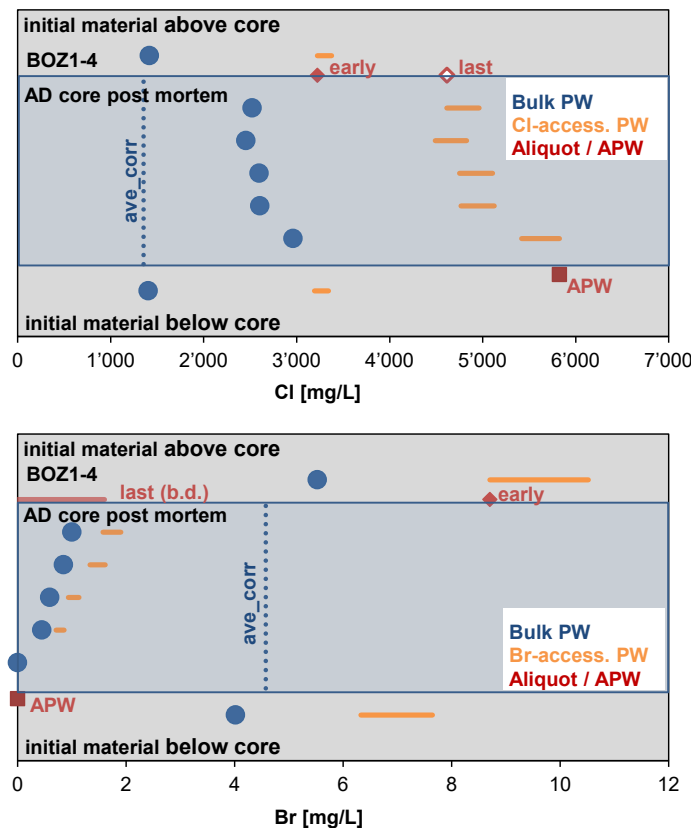
Fig. 4.7-17: Cl and Br concentrations from aqueous extracts up-scaled to bulk porewater and Cl/Br accessible porewater concentrations for the initial material and post-mortem profile of AD experiment BOZ1-4 (BOZ1-1-575.26-AD, Opalinus Clay)
