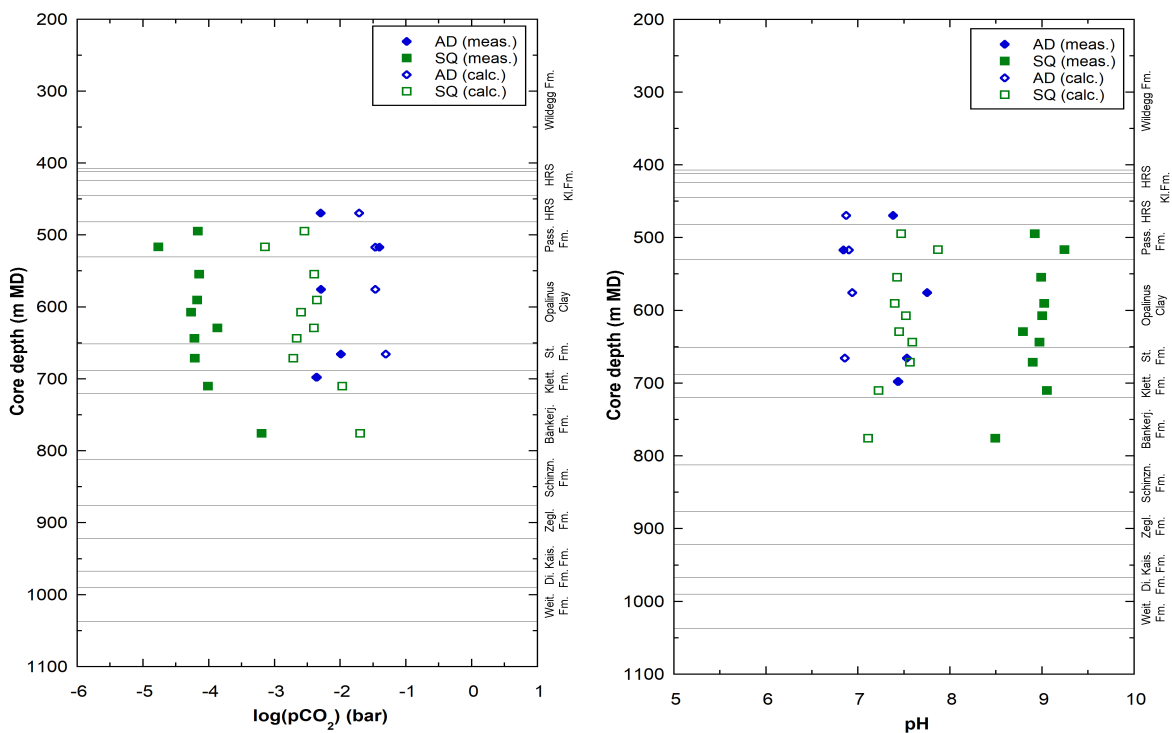
Fig. 5.5-1: pH (left) and calculated P_{CO_2} values from AD and SQ (see text)
