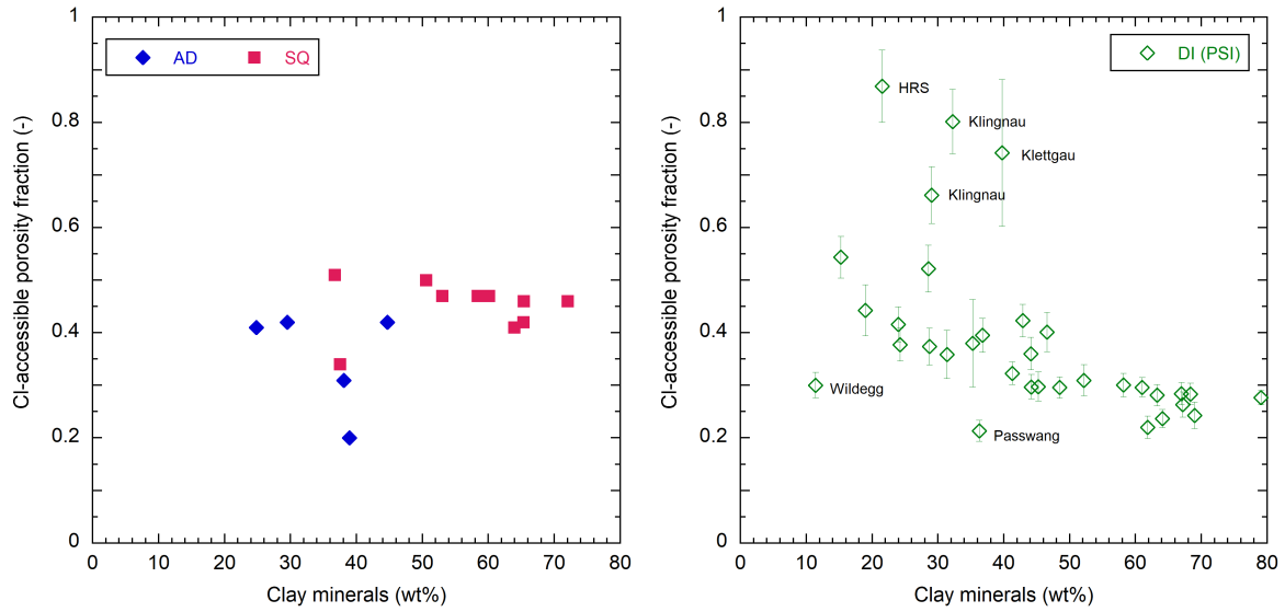
Fig. 5.1-1: Cl-accessible porosity fraction as a function of the clay-mineral content, left: AD and SQ data; right: diffusion data (PSI)
