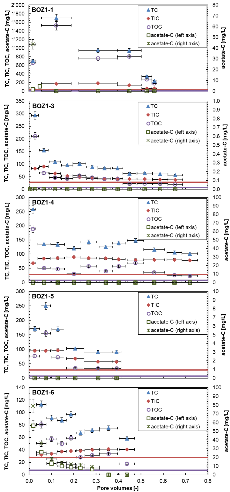
Fig. 4.7-12: Evolution of carbon system during advective displacement experiments
