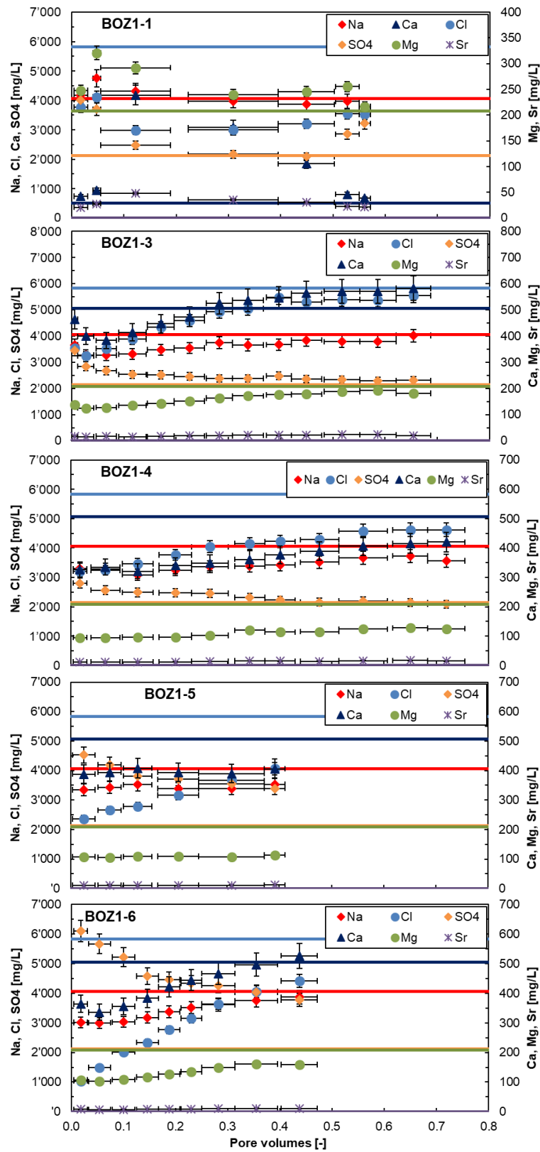
Fig. 4.7-8: Evolution of major components during advective displacement experiments
