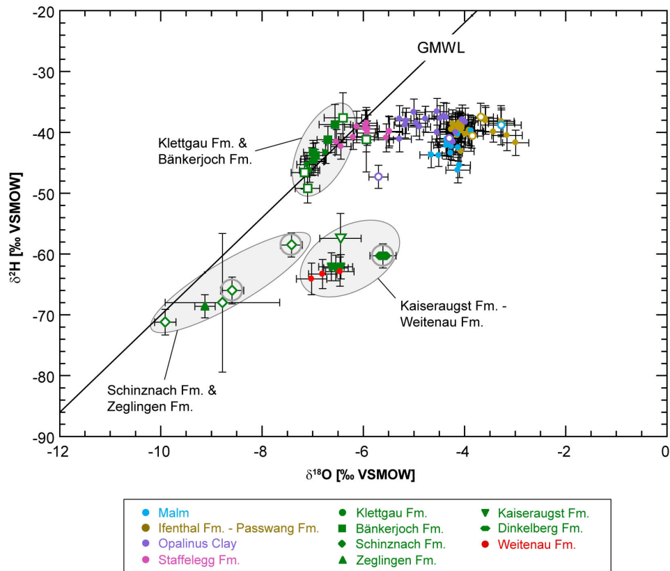
Fig. 4.8-5: \delta^2\text{H} vs. \delta^{18}\text{O} -values of porewater obtained from isotope diffusive-exchange experiments
