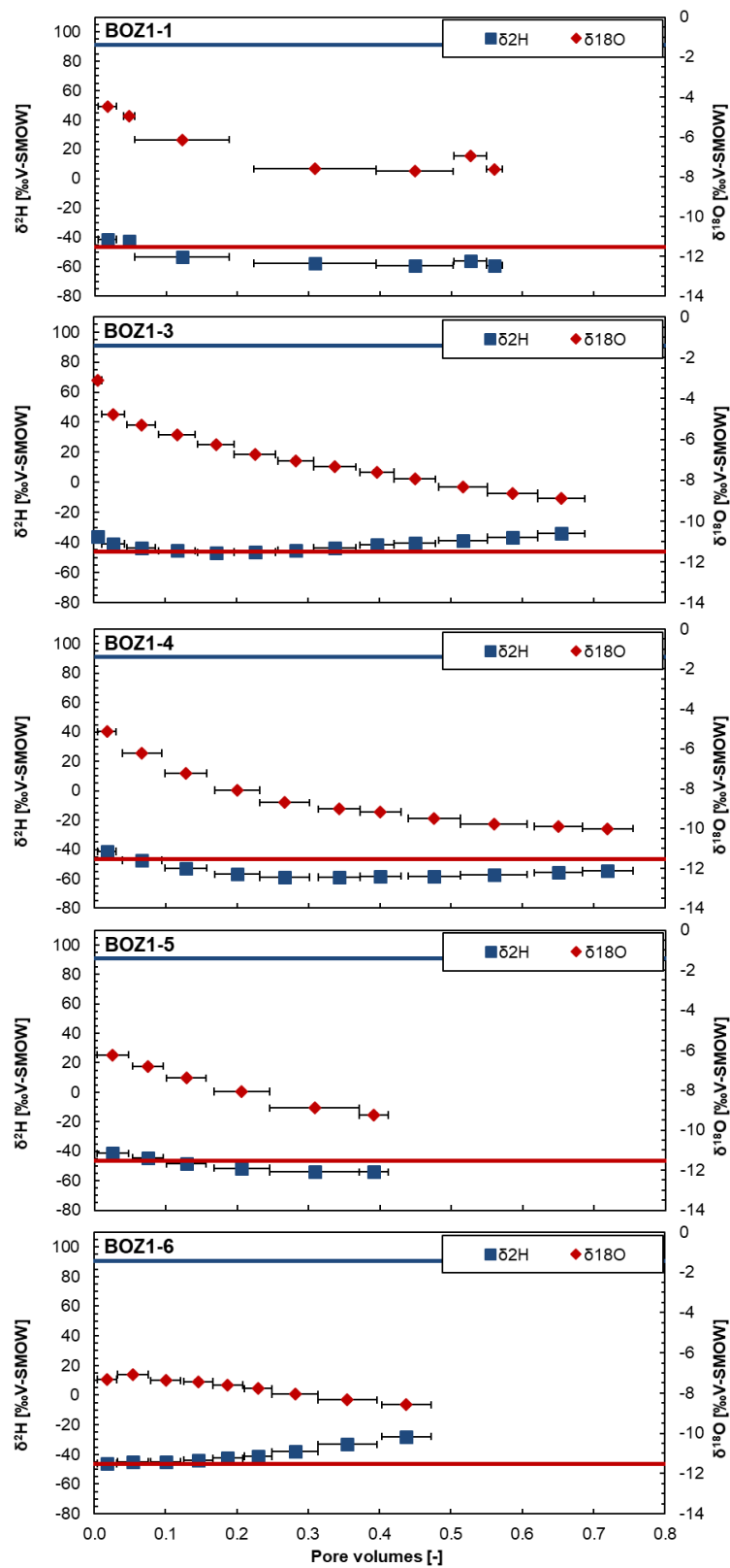
Fig. 4.7-15: Evolution of \delta^2\text{H} and \delta^{18}\text{O} during advective displacement experiments
