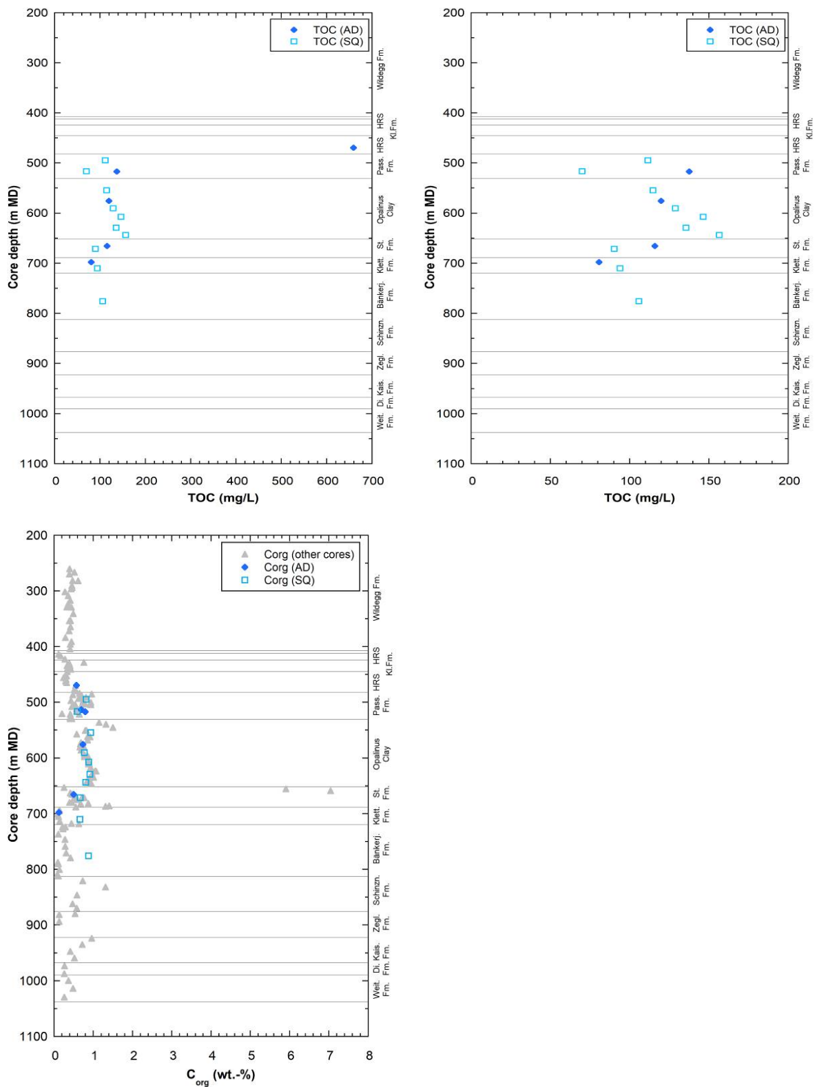
Fig. 5.5-2: TOC concentrations in porewater samples at different scales (pannels above) from AD and SQ and organic carbon content in rock (below)
