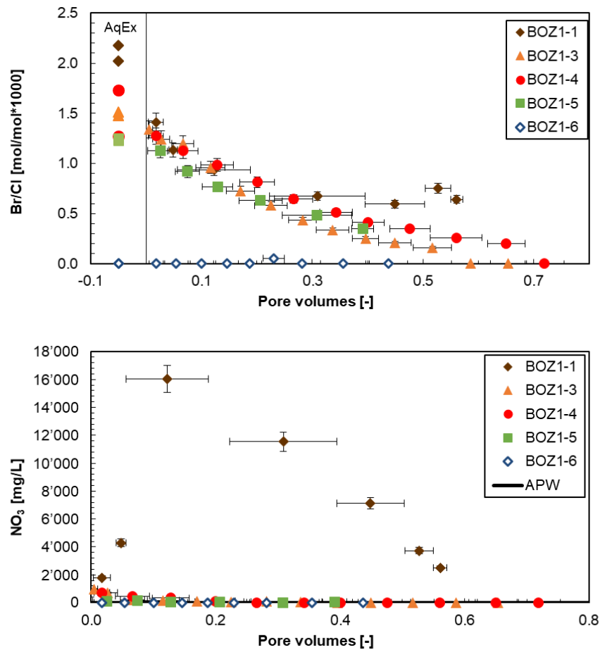
Fig. 4.7-19: Breakthrough of Cl/Br and NO 3 during advective displacement experiments
