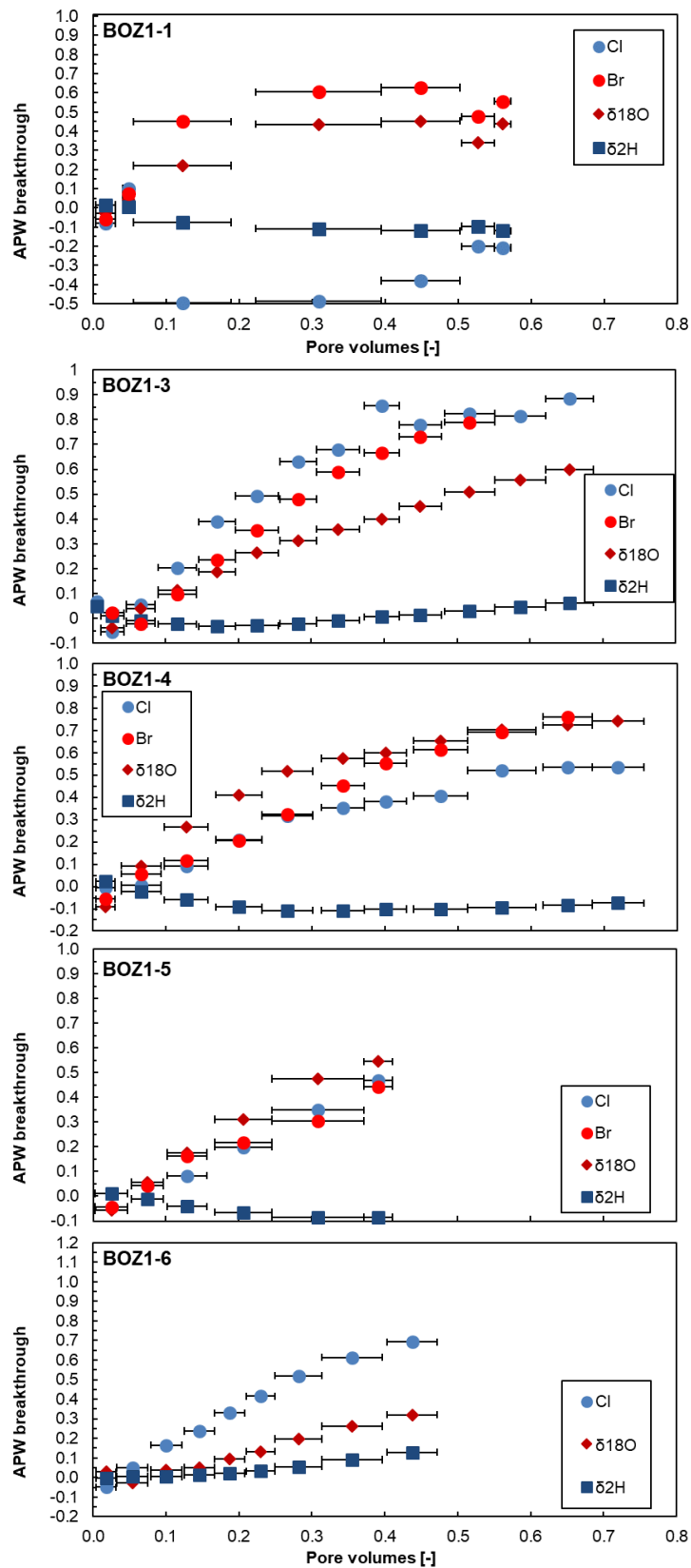
Fig. 4.7-18: Breakthrough of Cl, Br, \delta^2\text{H} and \delta^{18}\text{O} during advective displacement experiments
