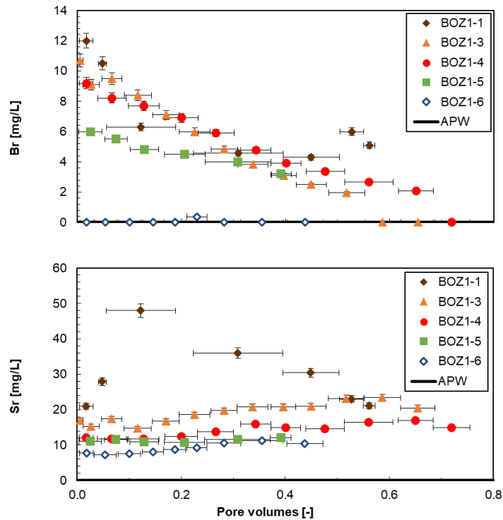
Fig. 4.7-11: Evolution of selected minor components during advective displacement experiments
