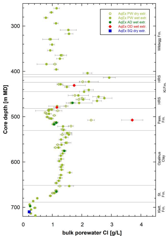
Fig. 4.4-7: Bulk porewater Cl concentrations versus depth from aqueous extracts from the Malm to the Klettgau Formation
