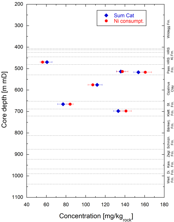
Fig. 4.5-1: Depth profile of Ni consumption and sum of cations (uncorrected) Errors reflect propagated analytical uncertainties.
