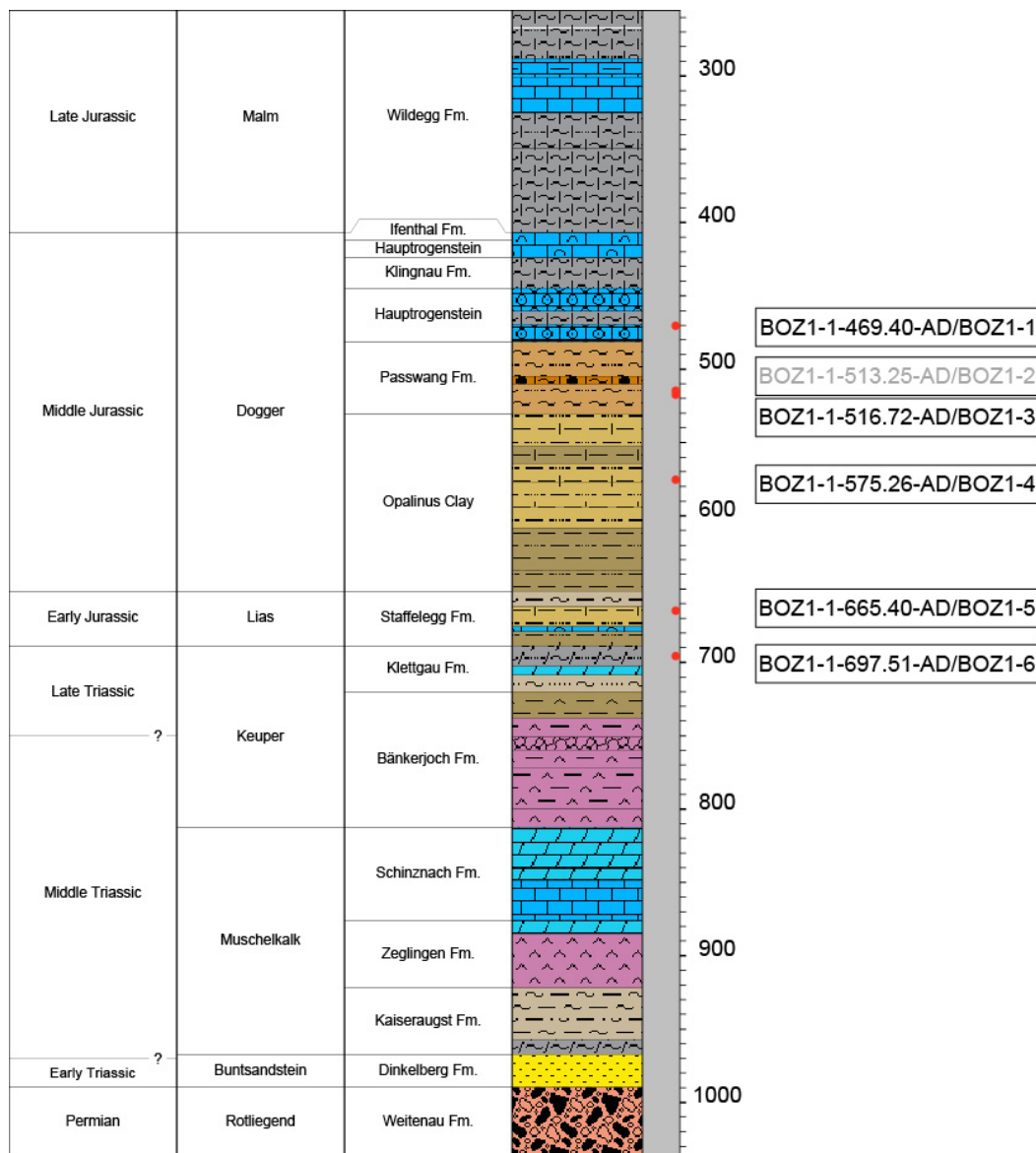
Fig. 4.7-1: Location of samples used for advective displacement experiments (red dots)
