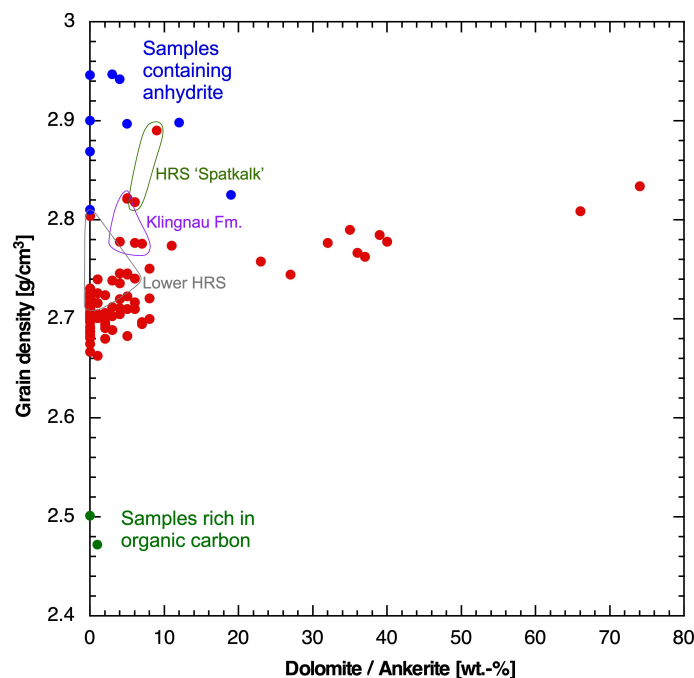
Fig. 4.3-5: Grain density as a function of the contents of dolomite/ankerite
