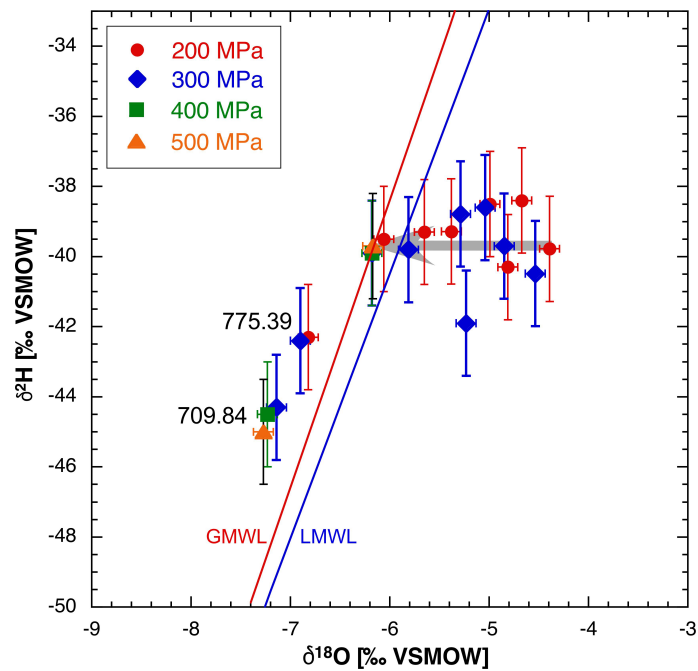
Fig. 4.6-7: Plot of \delta^{18}\text{O} vs. \delta^2\text{H} for squeezed waters
