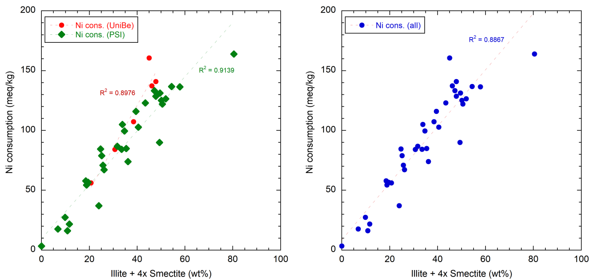
Fig. 5.6-5: Ni consumption as function of the sum of illite content and 4× smectite content
