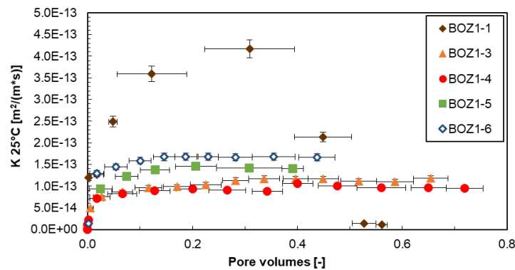
Fig. 4.7-4: Evolution of hydraulic conductivity during advective displacement experiments
