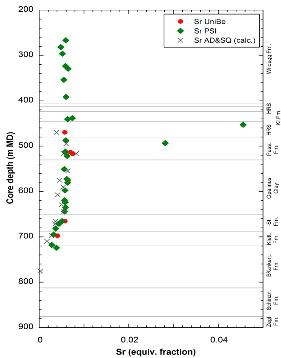
Fig. 5.6-8: Sr occupancies according to Uni Bern and PSI data and calculated from AD/SQ data
