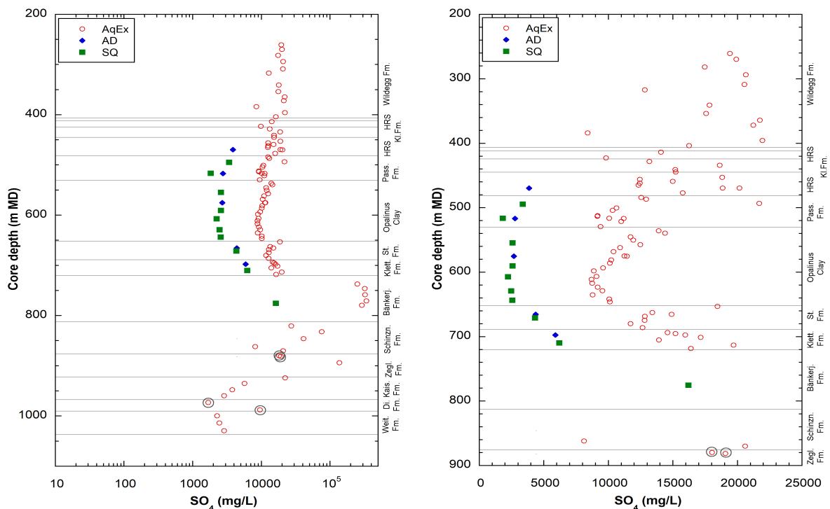
Fig. 5.3-1: \text{SO}_4 profiles (logarithmic and linear scales) with data from squeezing, advective displacement and aqueous extractions; left: entire data (logarithmic scale); right: data down to 900 m depth with \text{SO}_4 concentrations < 25 g/L (linear scale)
