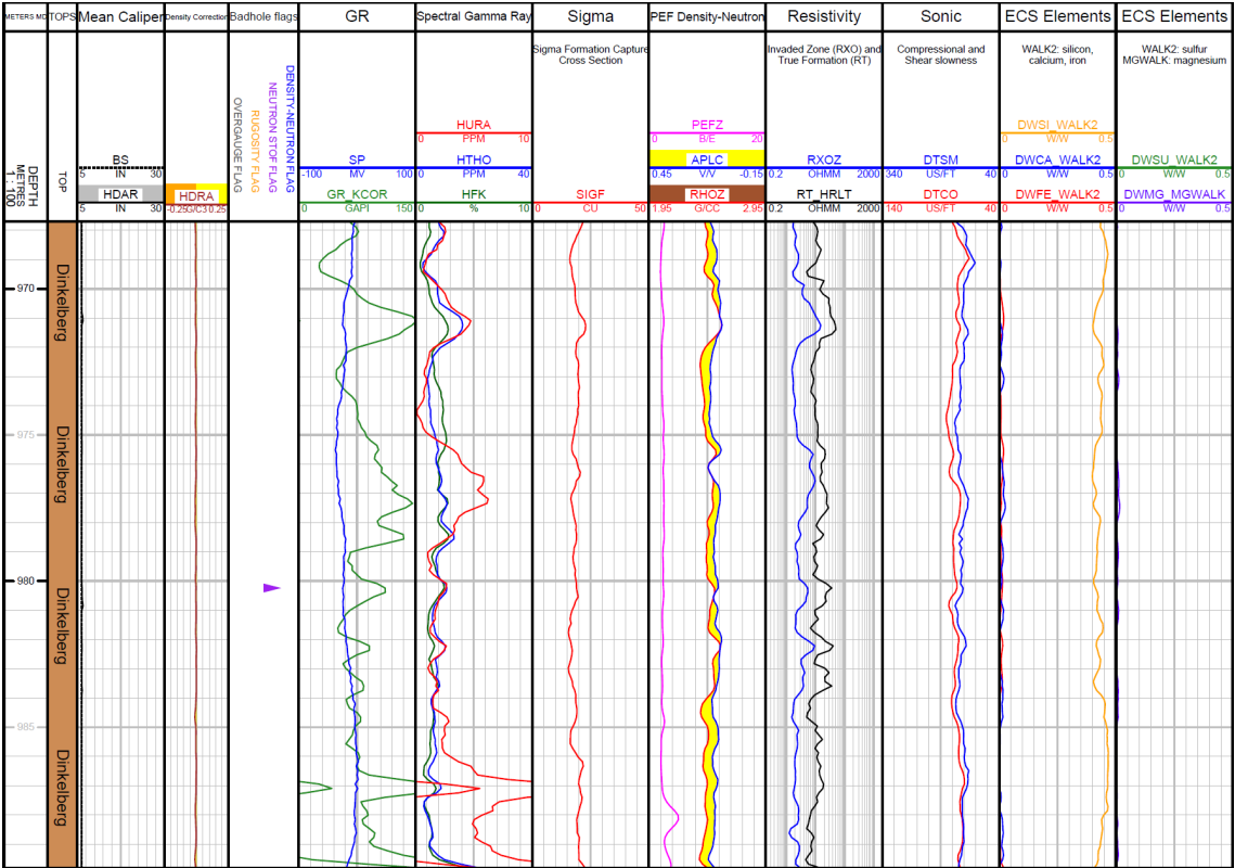
Fig. 3-10: Main logs of the composite dataset in the Dinkelberg Formation
