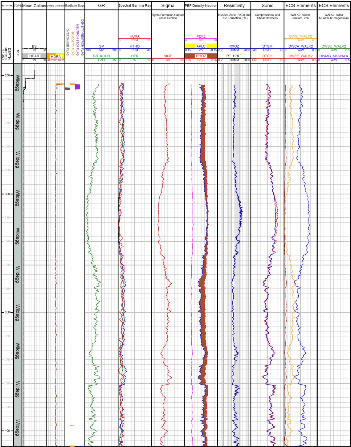
Fig. 3-1: Main logs of the composite dataset in the Wildegg Formation
