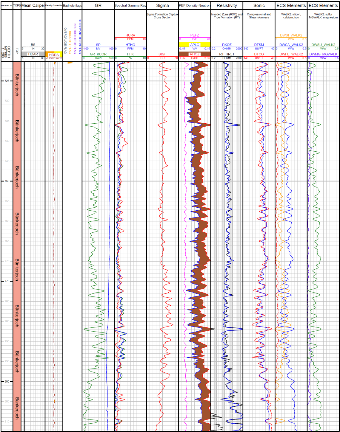
Fig. 3-6: Main logs of the composite dataset in the Bänkerjoch Formation
