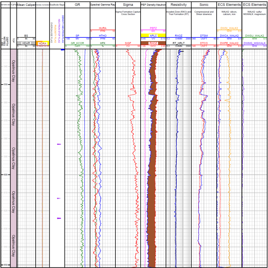
Fig. 3-3: Main logs of the composite dataset in the Opalinus Clay
