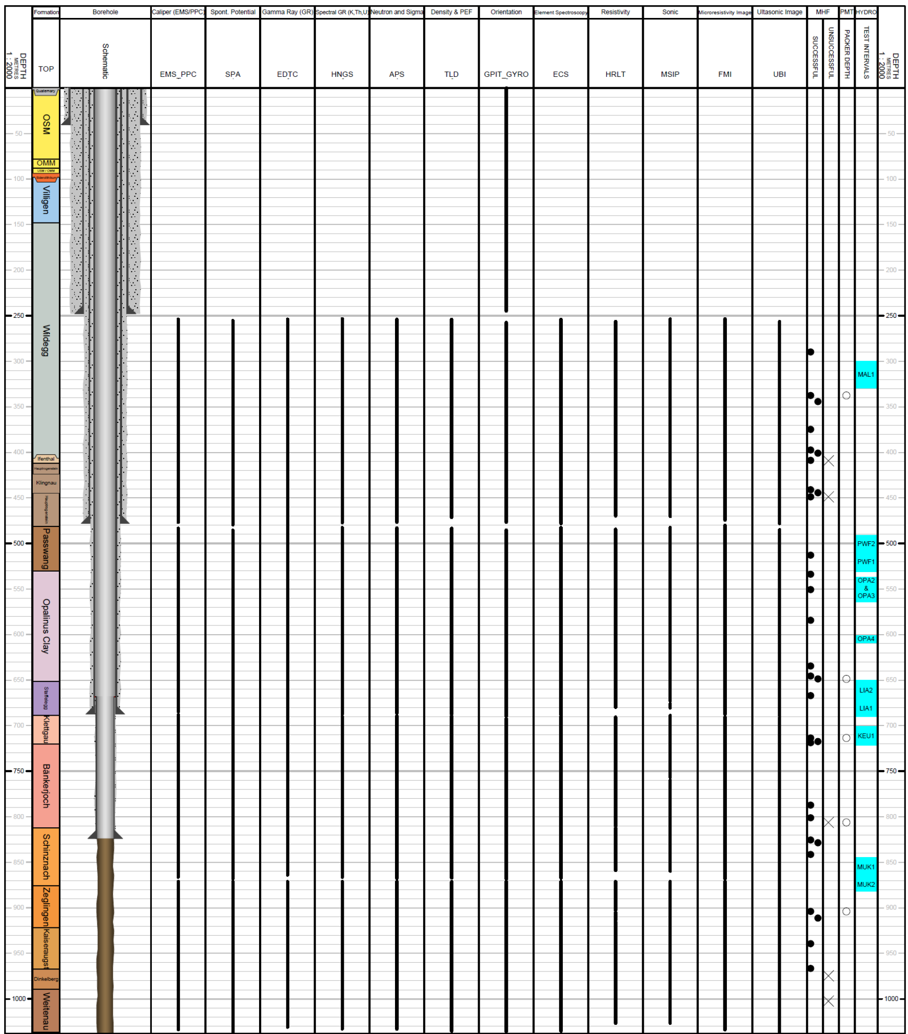
Fig. 2-1: Petrophysical log and MHF / PMT testing coverage at BOZ1-1 (scale of 1:2'000)
