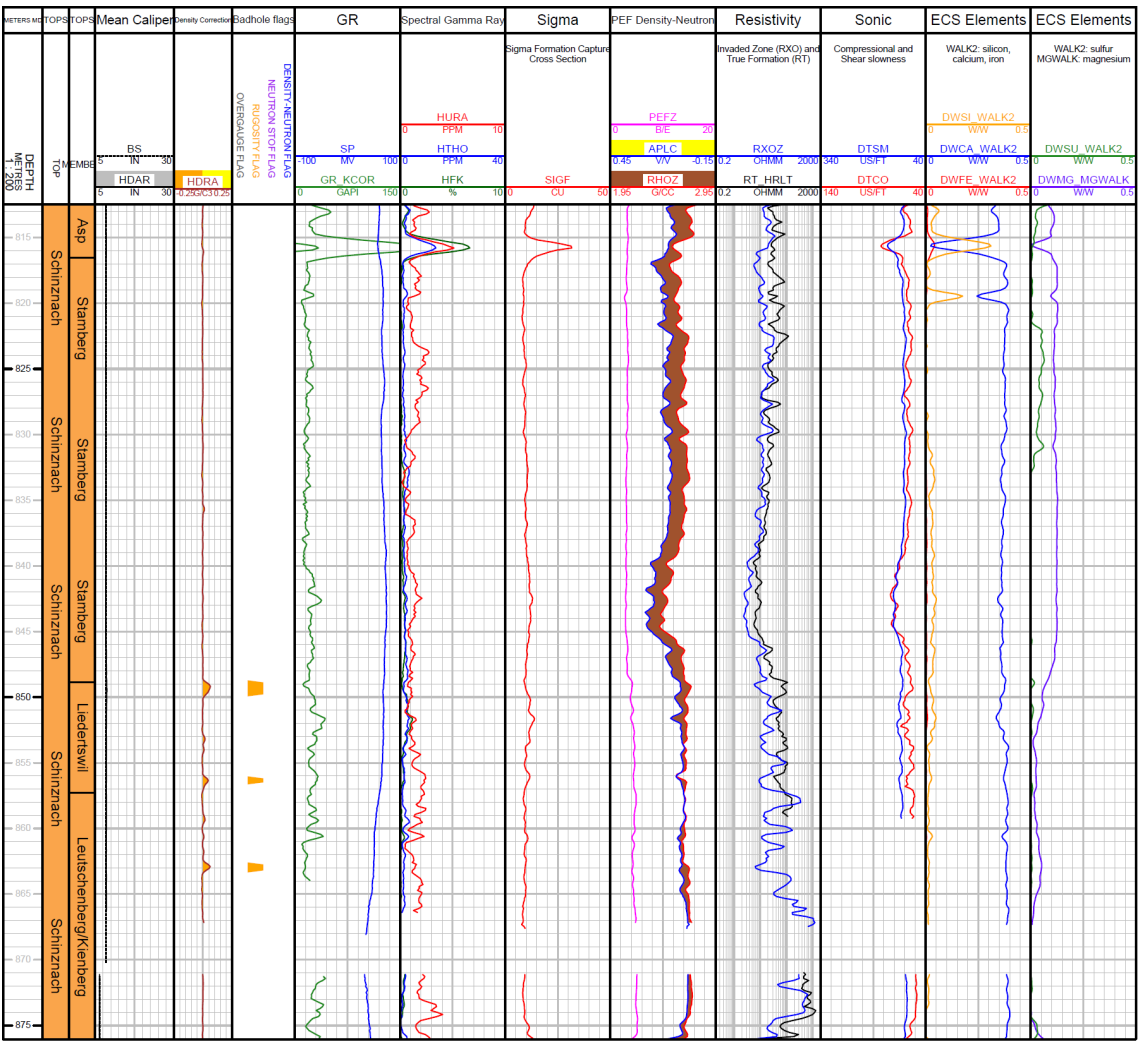
Fig. 3-7: Main logs of the composite dataset in the Schinznach Formation
