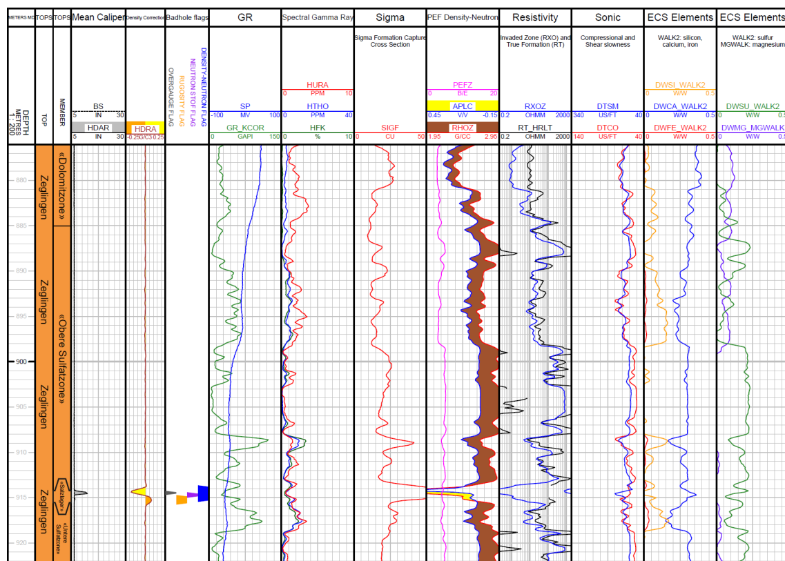
Fig. 3-8: Main logs of the composite dataset in the Zeglingen Formation
