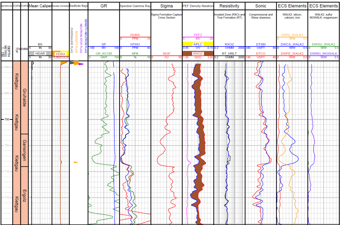
Fig. 3-5: Main logs of the composite dataset in the Klettgau Formation
