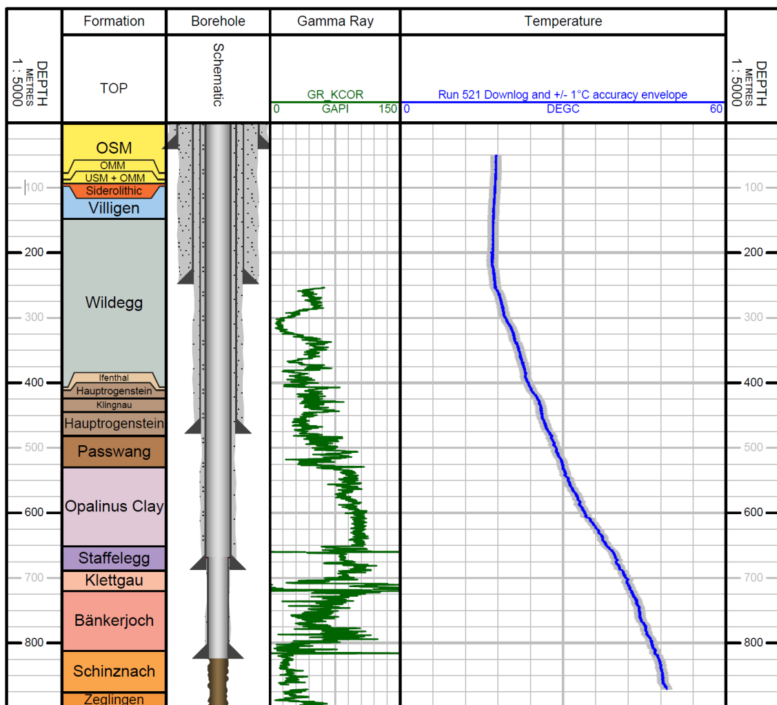
Fig. 3-12: Post-completion temperature log from the downlog pass of Run 5.2.1 (10.08.2021)
