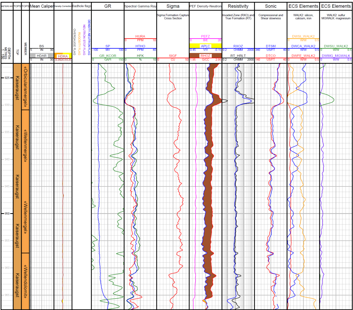
Fig. 3-9: Main logs of the composite dataset in the Kaiseraugst Formation
