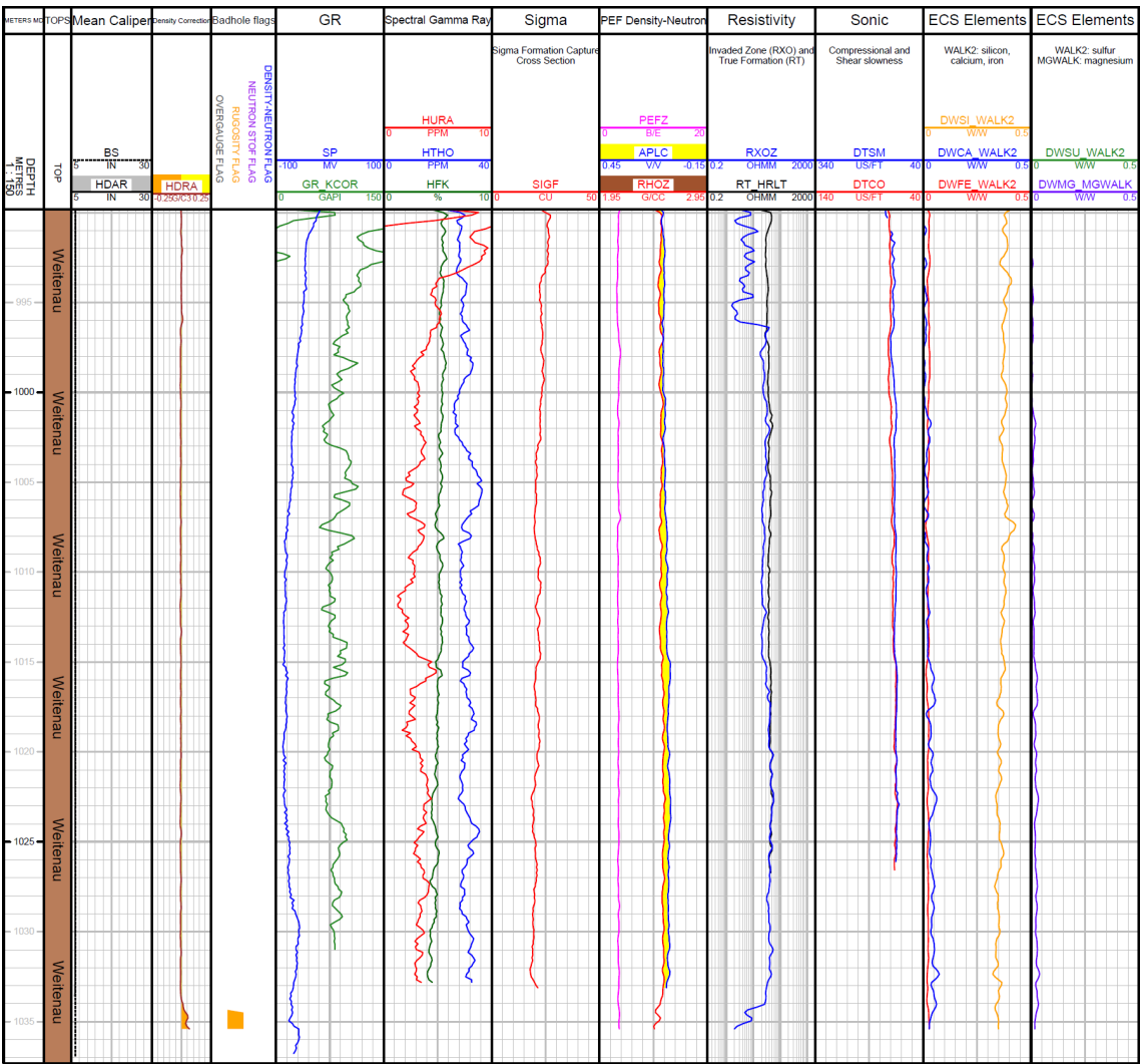
Fig. 3-11: Main logs of the composite dataset in the Weitenau Formation
