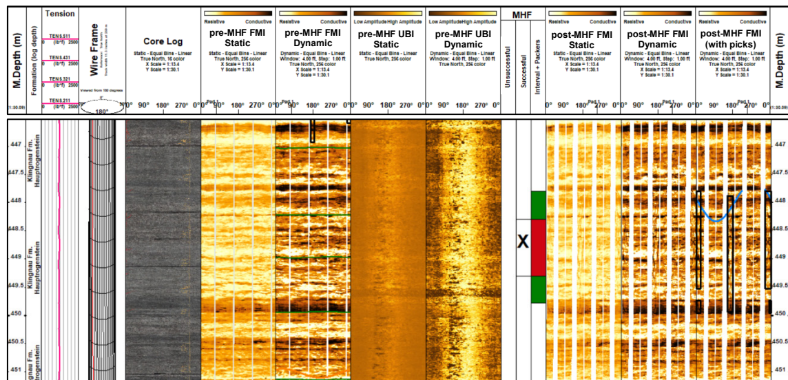
Fig. 5-4: Example of pre- vs. post-MHF images from BOZ1-1 (Station 1-4 from run 2.6.3, Section II)
