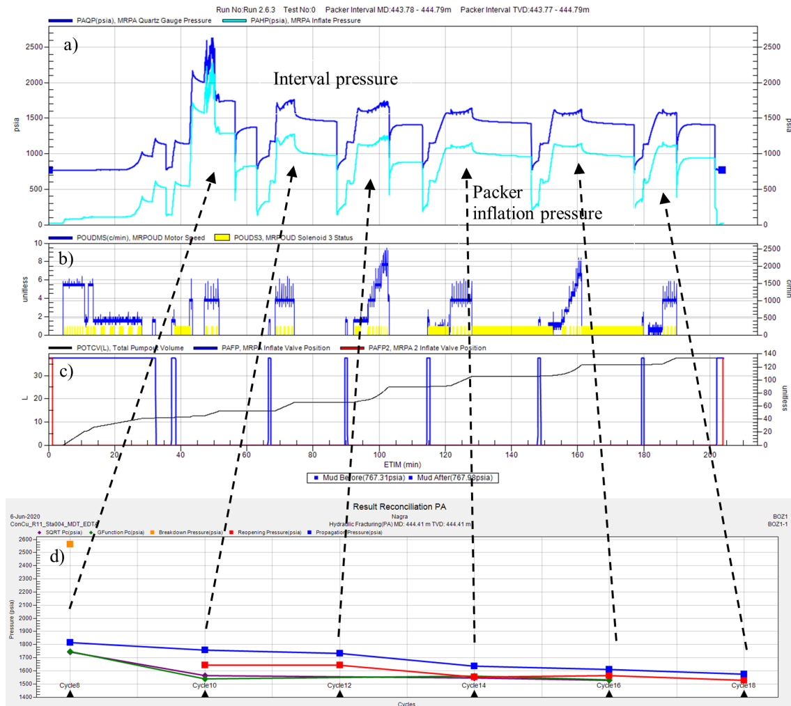
Fig. 5-2: Example of pressure record for MHF test from BOZ1-1 (Station 1-3, Run 2.6.3) Pc stands for closure pressure, ISIP stands for Instantaneous Shut-in Pressure.
