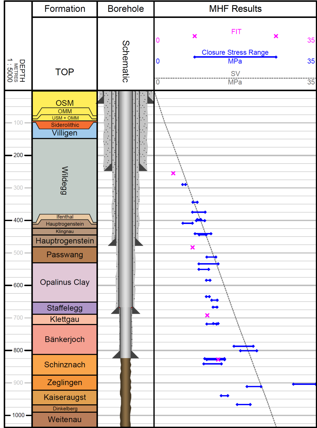
Fig. 5-3: Comparison of the quicklook closure stress range obtained from the BOZ1-1 MHF tests with the overburden vertical stress (Sv) from the integration of density over depth and the maximum pressures attained during the formation integrity tests (FIT)
