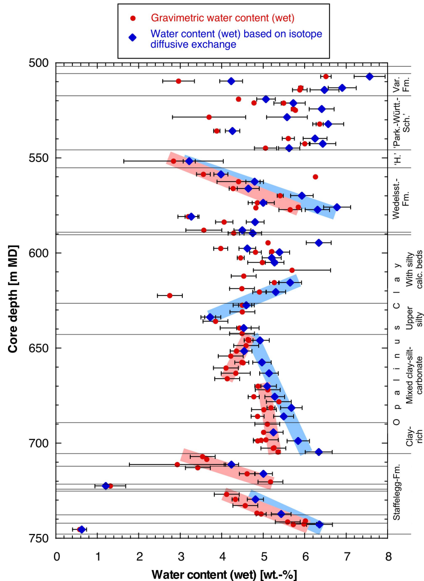
Fig. 4.3-3: Water content (wet) as a function of depth in the Lias – Dogger interval
