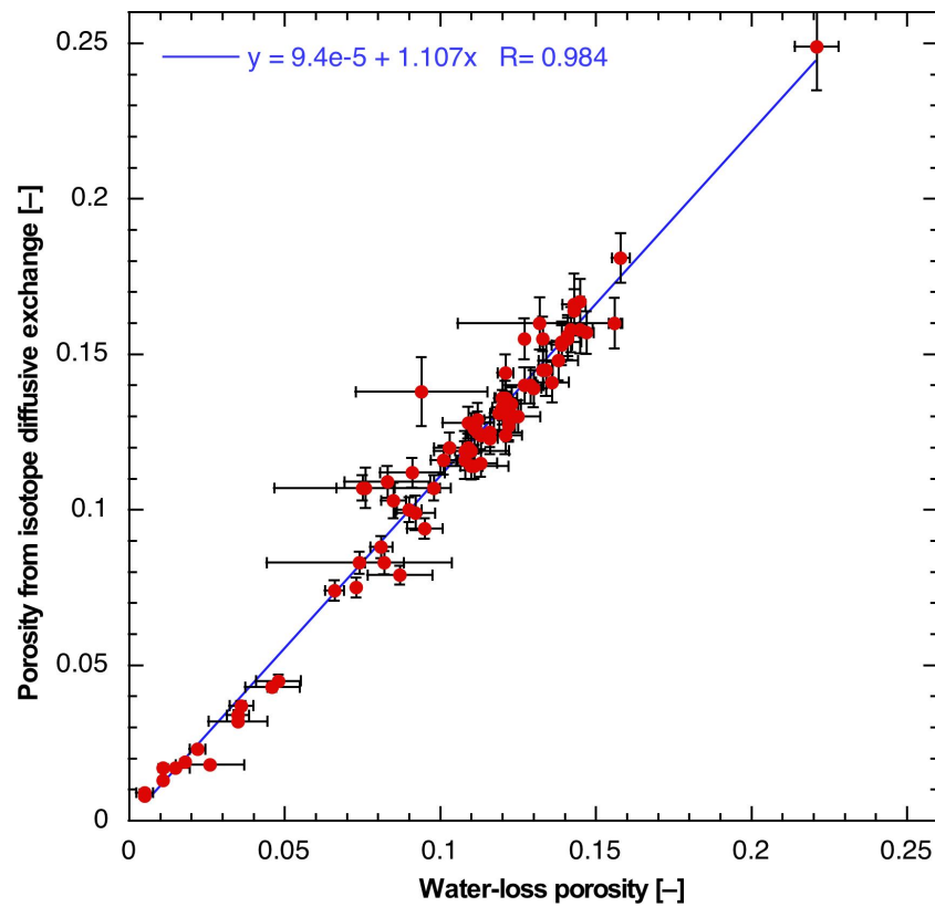
Fig. 4.3-7: Correlation of water-loss porosity and porosity from isotope diffusive exchange
