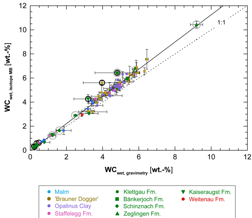
Fig. 4.8-2: Average water content obtained by water-loss at 105 °C ( WC_{\text{wet, gravimetry}} ) of sub-samples LAB and NGW/ICE vs. average water content calculated from \delta^{18}\text{O} and \delta^2\text{H} mass balance from NGW/ICE diffusive-exchange experiments ( WC_{\text{wet, isotope MB}} )
