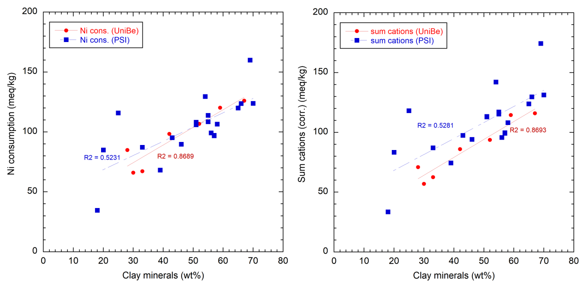
Fig. 5.7-4: CEC data as function of the clay-mineral content; left: Ni consumption data; right: Corrected sum of cations
