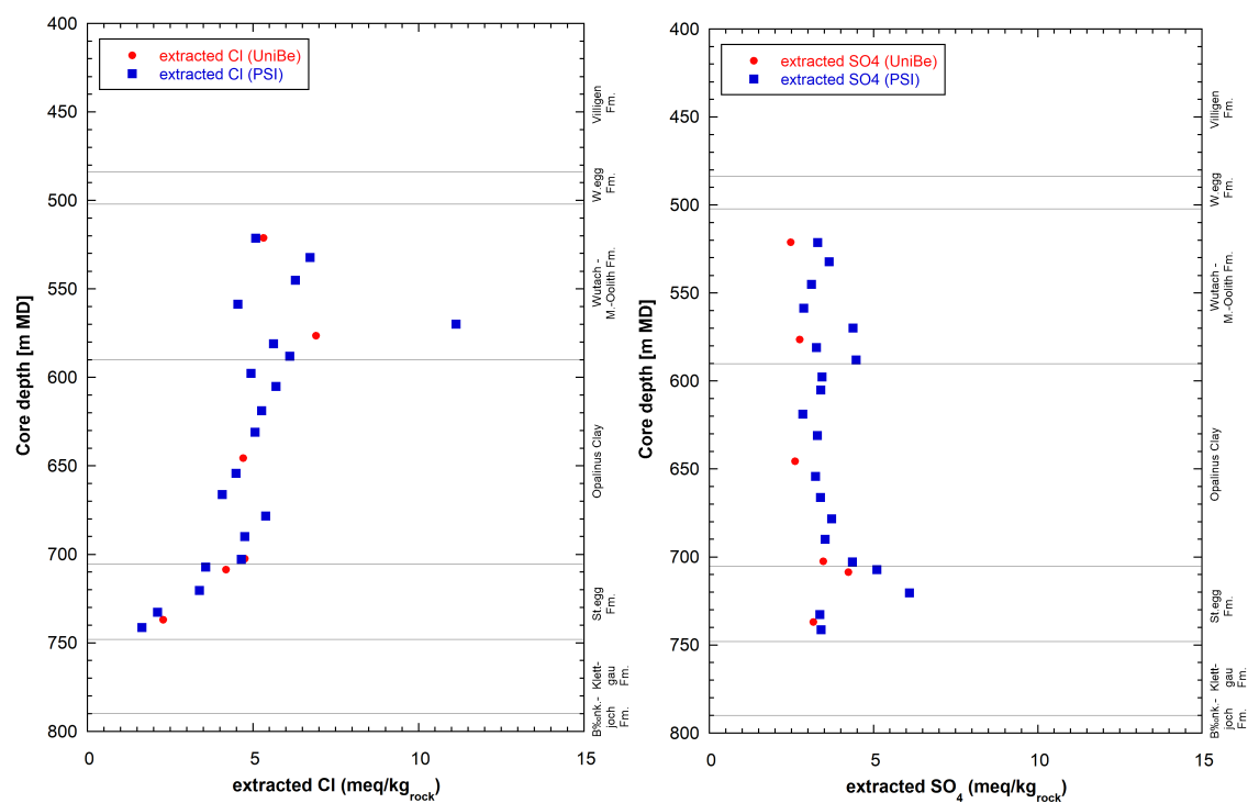
Fig. 5.7-9: Extracted Cl (left) and SO 4 (right) according to Uni Bern and PSI data
