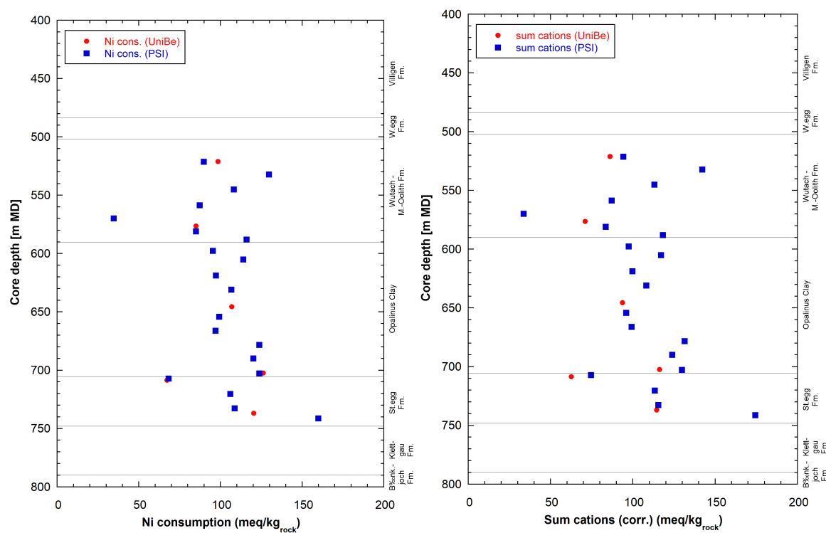
Fig. 5.7-3: Comparison of CEC data from Uni Bern and from PSI; Ni consumption data (left) and (corrected) sum of cations data (right)
