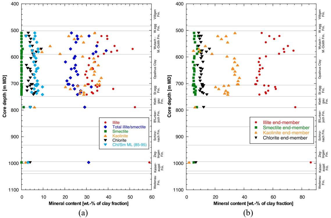
Fig. 4.2-5: Mineralogical composition of the clay fraction as a function of depth; (a) individual clay minerals, (b) end-member clays Detailed lithostratigraphic subdivision according to Dossier III.
