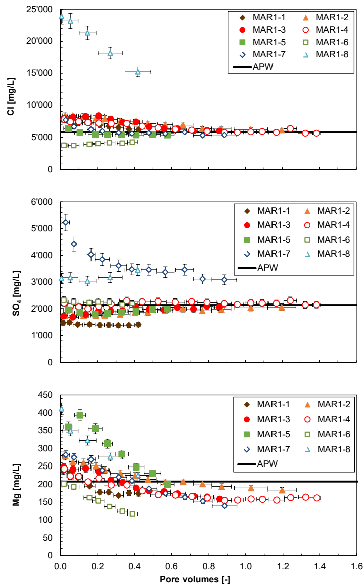
Fig. 4.7-9: Evolution of Cl, SO 4 and Mg during advective displacement experiments
