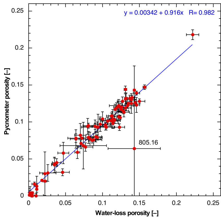
Fig. 4.3-10: Correlation of water-loss and pycnometer porosity
