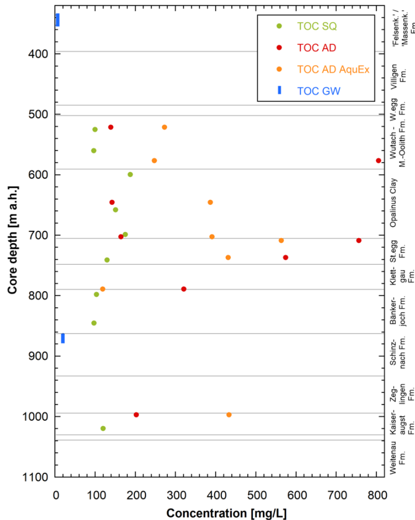
Fig. 5.5-2: TOC in aliquots from AD, upscaled from aqueous extracts, and aquifers
