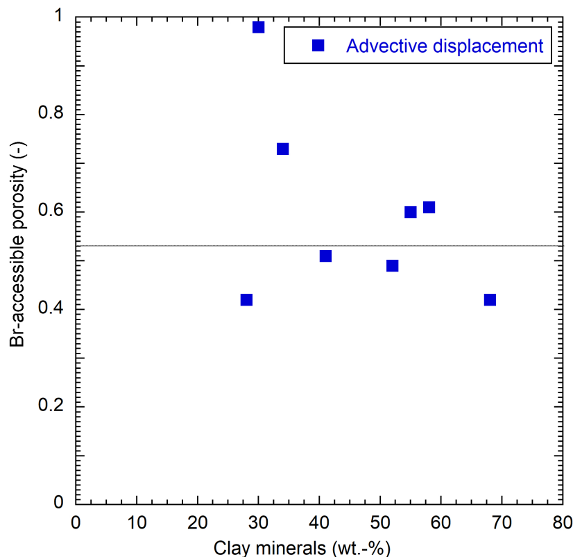
Fig. 5.1-2: Br-accessible porosity fraction as a function of the clay-mineral content
