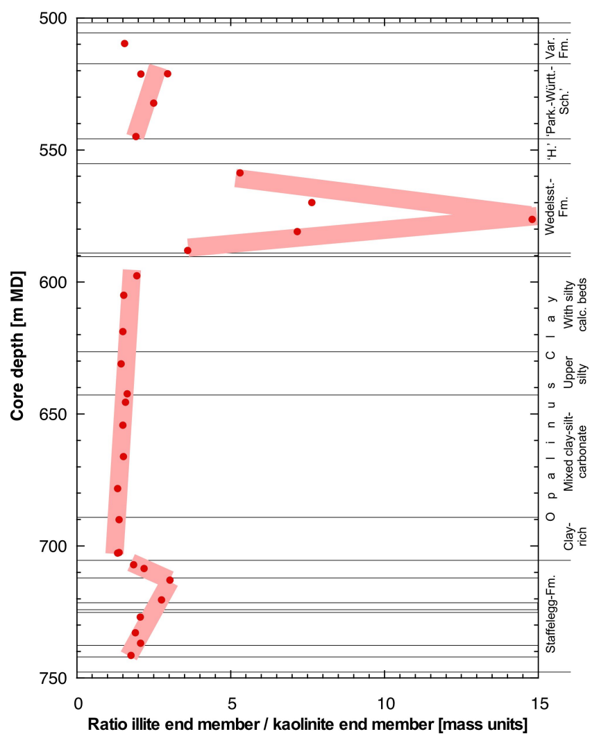
Fig. 4.2-7: Ratio of the illite to kaolinite end-member clays as a function of depth
