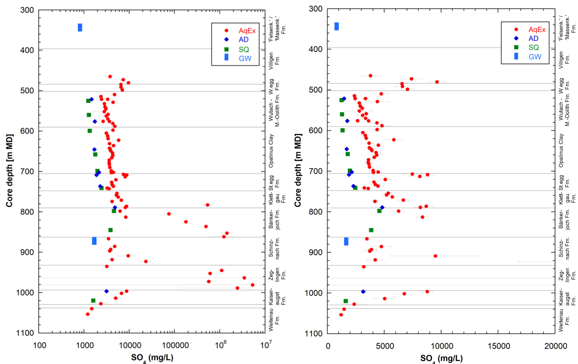
Fig. 5.3-1: \text{SO}_4 profiles (logarithmic and linear scales) with data from squeezing, advective displacement, aqueous extraction, Ni-en extraction and groundwater samples; left: entire data (logarithmic scale); right: data with \text{SO}_4 concentrations < 20 g/L (linear scale)
