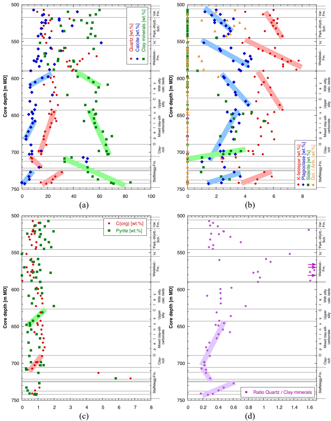
Fig. 4.2-4: Depth trends of mineral contents in the bulk rock in the Lias – Dogger interval
