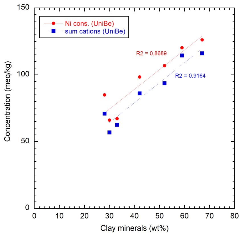
Fig. 5.7-2: CEC parameters as a function of the clay-mineral content (data of Uni Bern)
