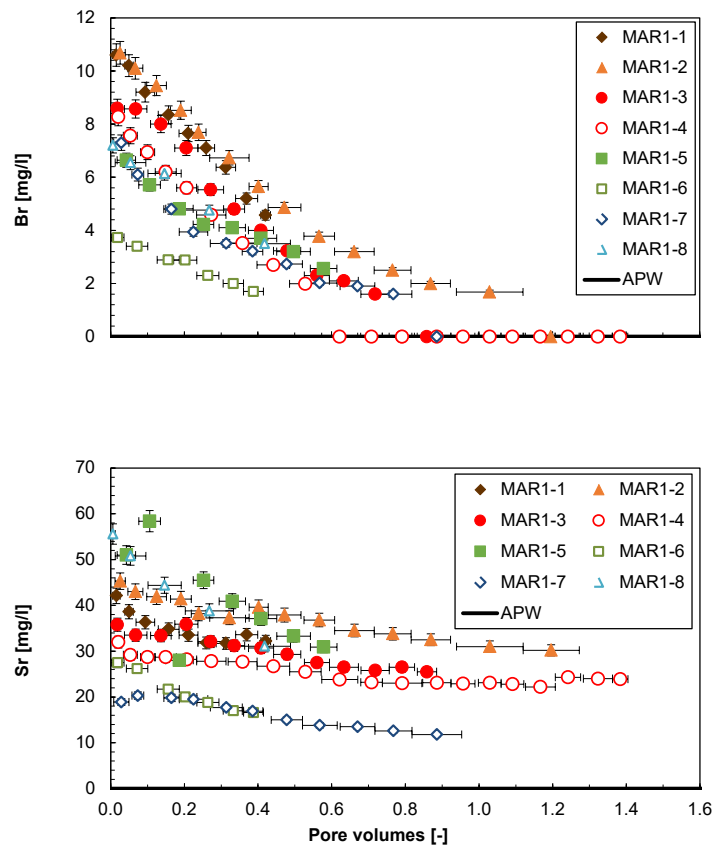
Fig. 4.7-11: Evolution of select minor components during advective displacement experiments
