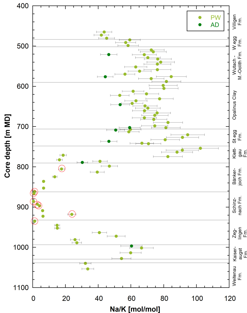
Fig. 4.4-5: Depth versus Na/K molar concentration ratio in aqueous extracts at a S/L ratio of about 1
