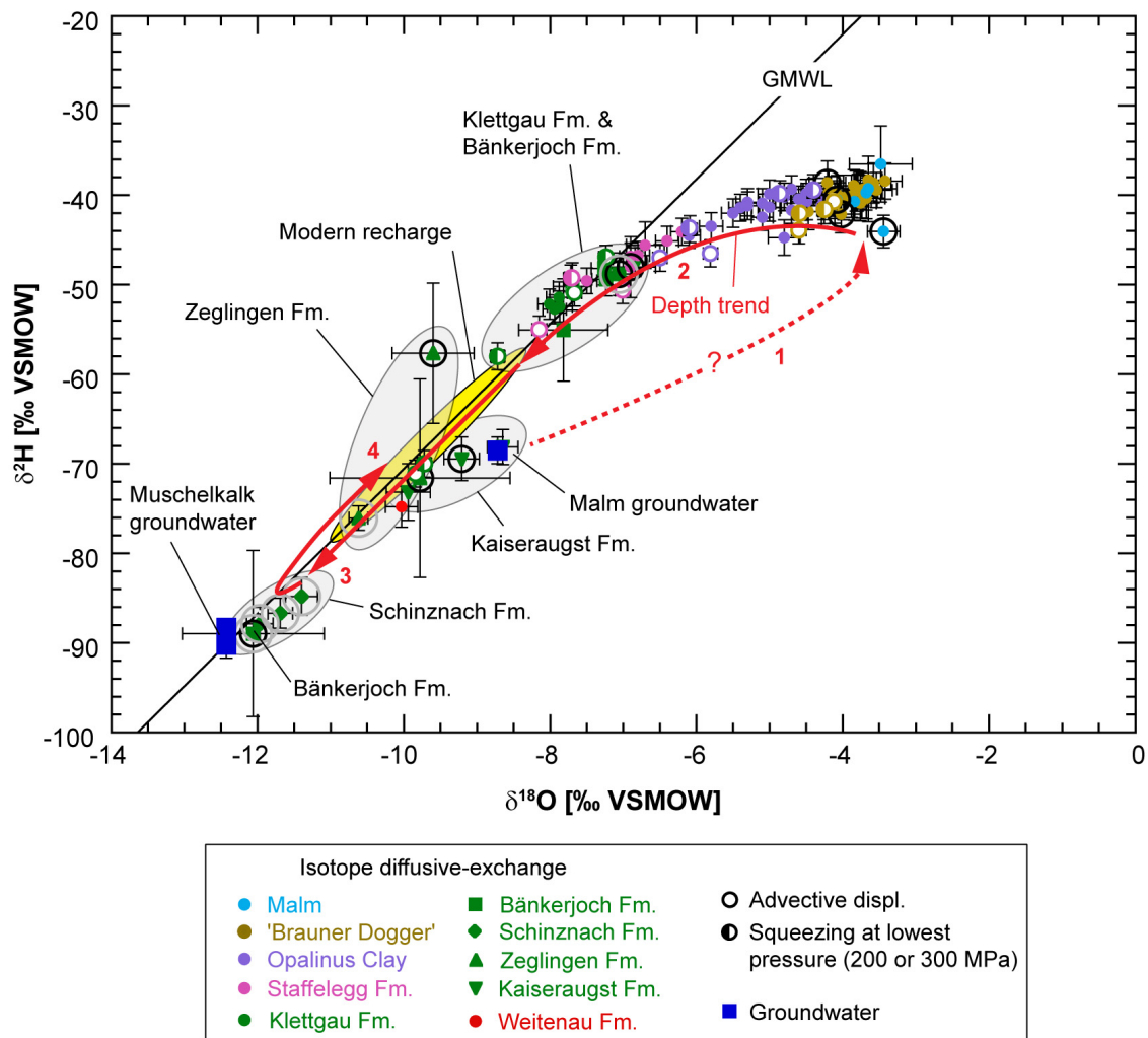
Fig. 5.8-2: \delta^{18}\text{O} vs. \delta^2\text{H} for groundwater and porewater derived by all techniques
