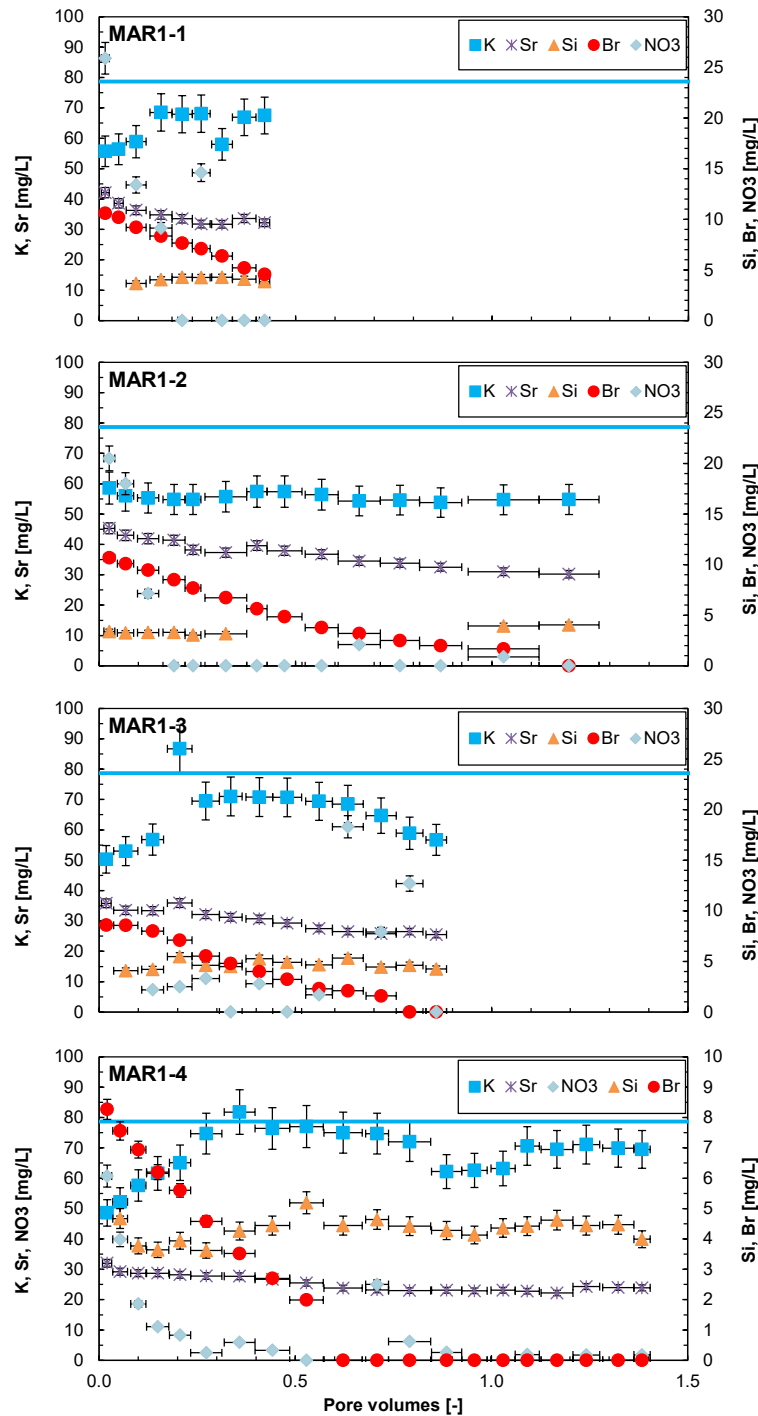
Fig. 4.7-10: Evolution of minor components during advective displacement experiments
