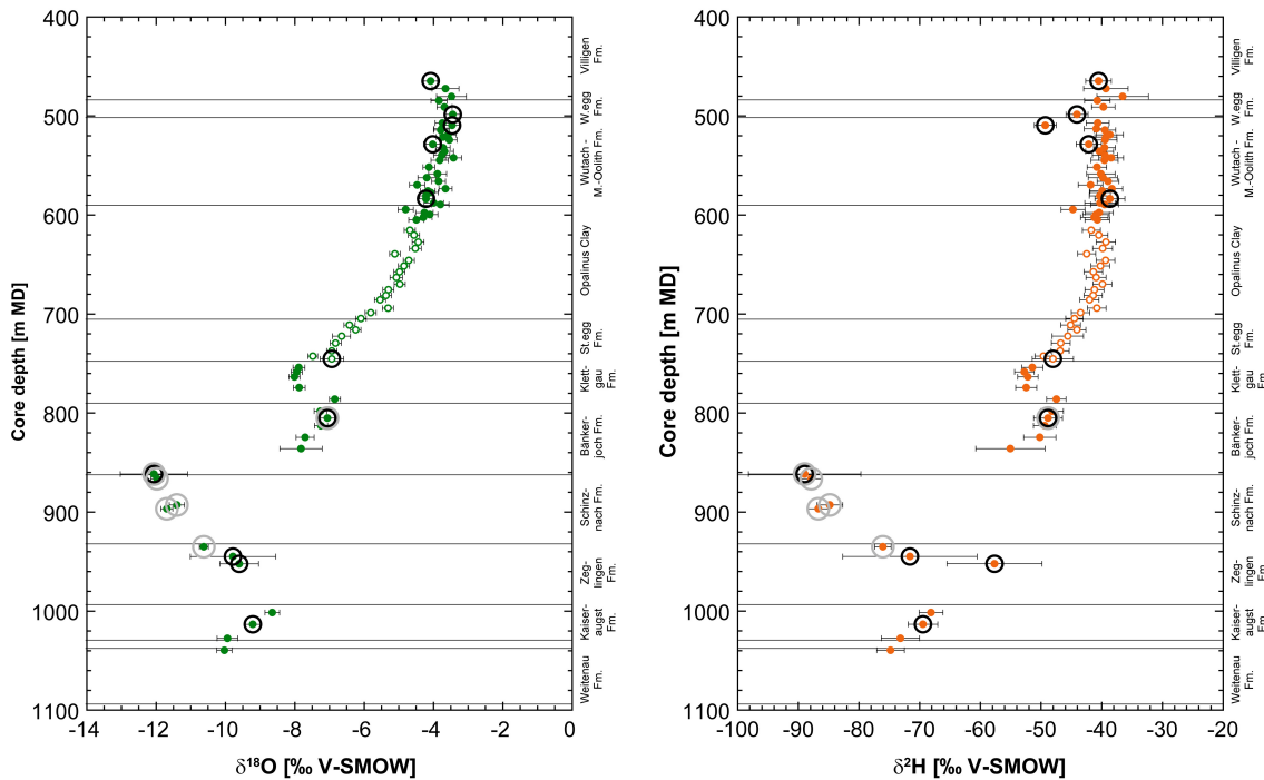
Fig. 4.8-3: Depth distribution of accepted porewater \delta^{18}\text{O} and \delta^2\text{H} values obtained from isotope diffusive-exchange experiments
