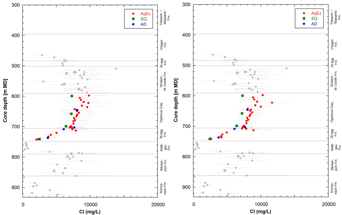
Fig. 5.2-2: Cl profiles using 'standard' procedure (left) and alternative approach (right), see text
