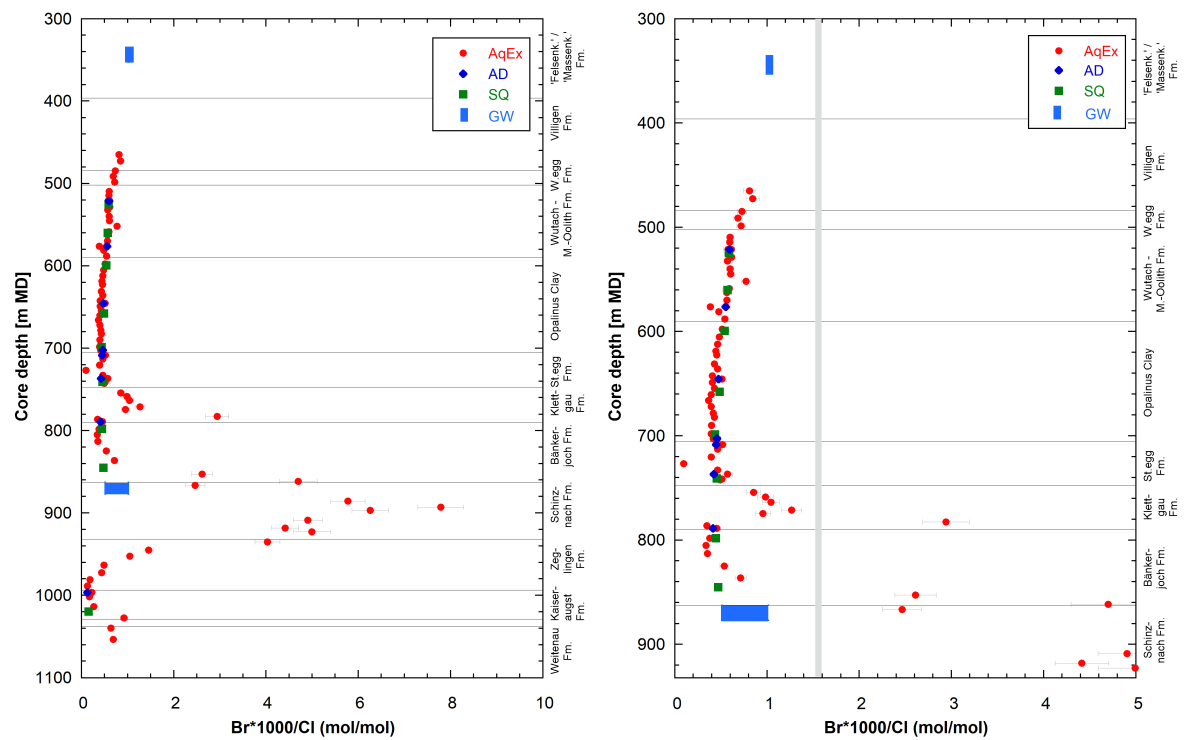
Fig. 5.2-4: Br*1000/Cl ratios (mol/ mol) at two different depth scales with data from squeezing, advective displacement, aqueous extraction and groundwater samples
