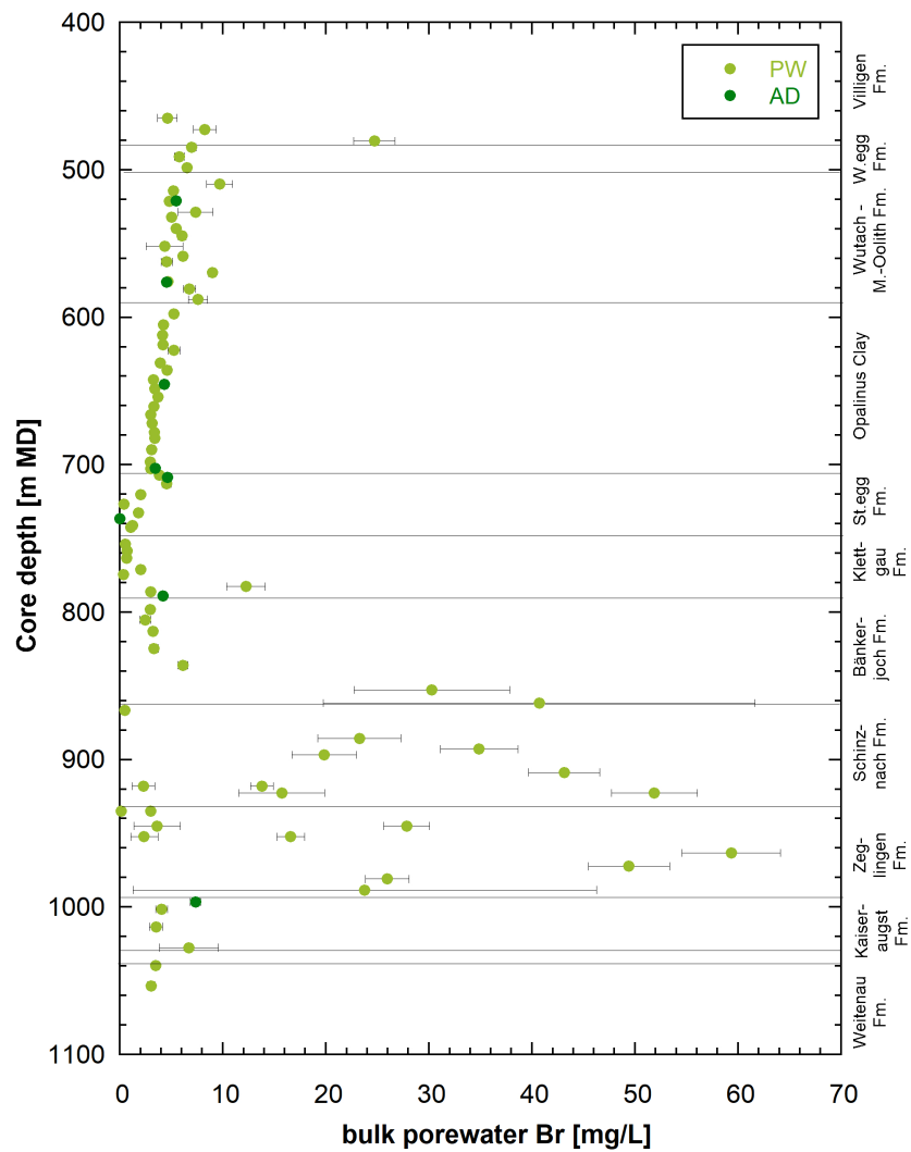
Fig. 4.4-7: Bulk porewater Br concentrations versus depth from aqueous extracts
