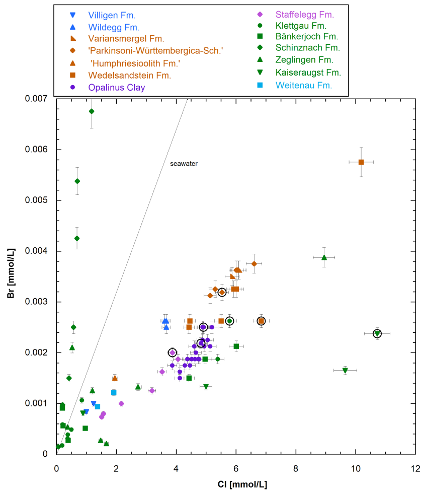
Fig. 4.4-1: Molar Br versus Cl concentrations in aqueous extracts at a S/L ratio of about 1 AD samples are marked with black circles.
