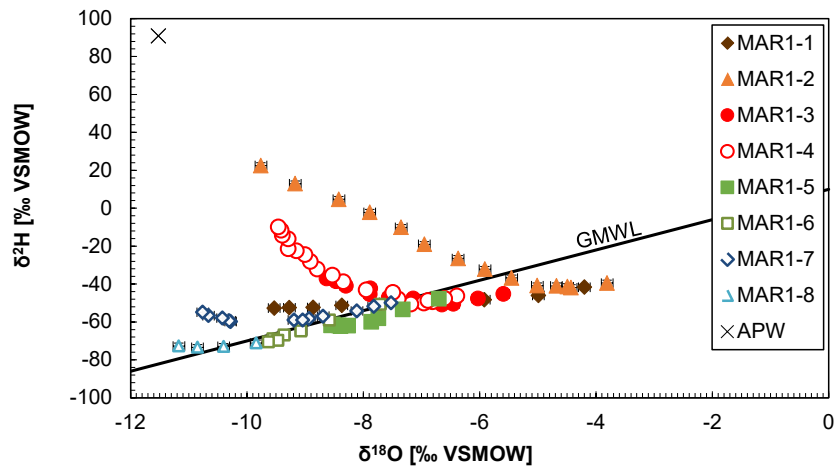
Fig. 4.7-16: Composition stable isotopes of aliquots from advective displacement experiments
