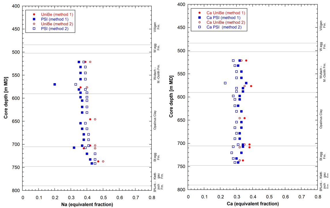
Fig. 5.7-6: Na (left) and Ca (right) occupancies according to Uni Bern and PSI data
