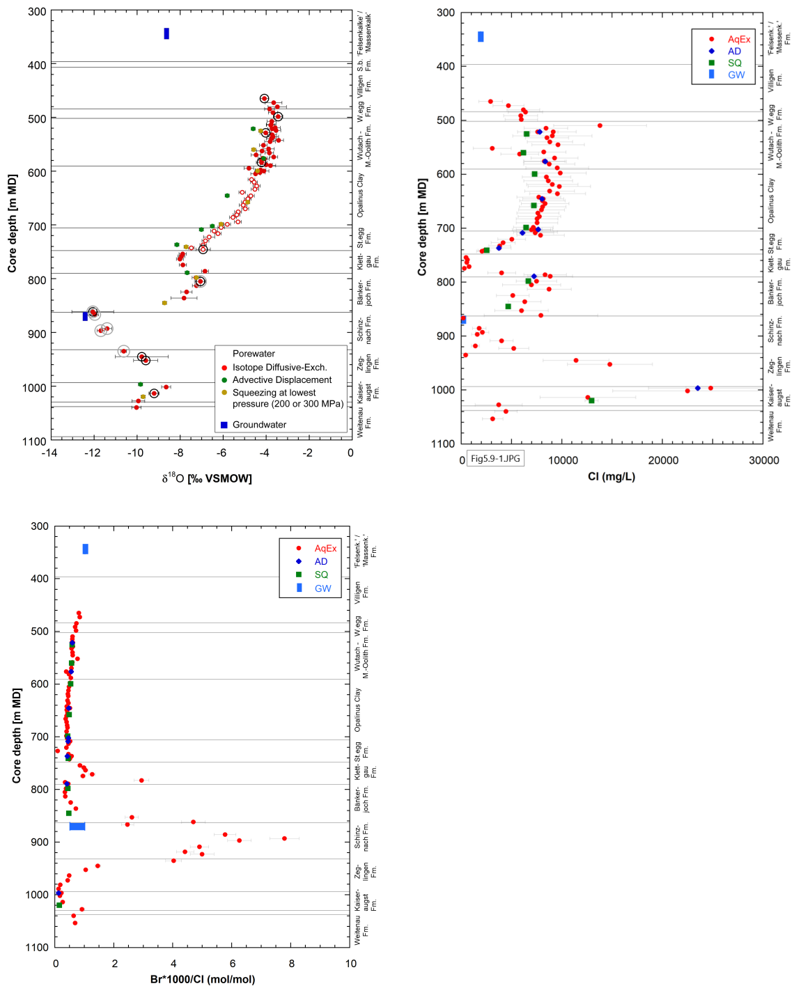
Fig. 5.9-1: Depth profiles for \delta^{18}\text{O} , Cl and Br/Cl
