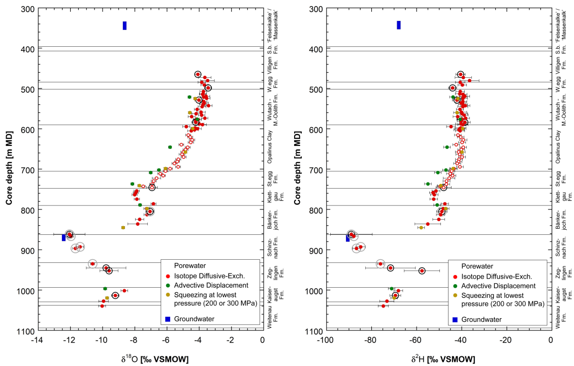
Fig. 5.8-1: Depth trends of \delta^{18}\text{O} and \delta^2\text{H} in groundwater and porewater derived by all techniques
