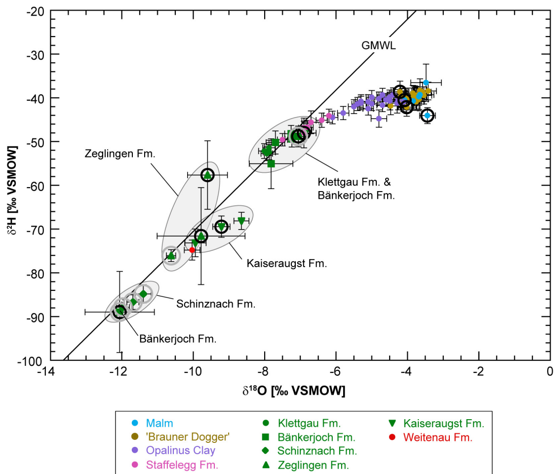
Fig. 4.8-5: \delta^{18}\text{O} vs. \delta^2\text{H} values of porewater obtained from isotope diffusive-exchange experiments
