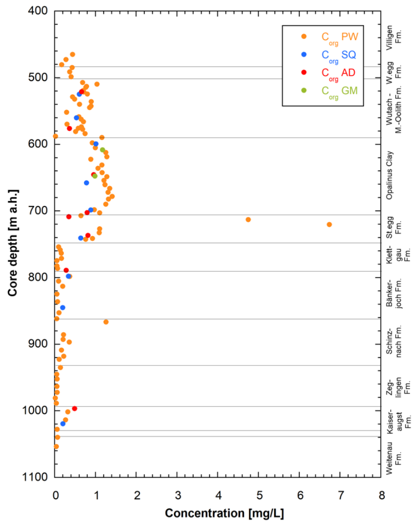
Fig. 5.5-1: Organic carbon in rock samples Colour coding is according to sample type.
