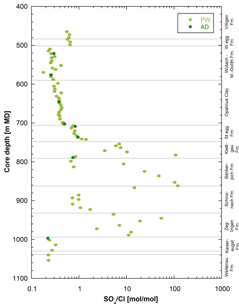
Fig. 4.4-3: Depth profile of \text{SO}_4/\text{Cl} molar concentration ratio in aqueous extracts at a S/L ratio of about 1
