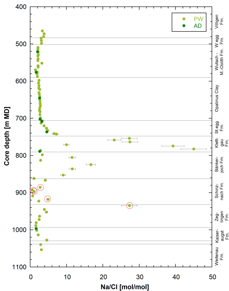
Fig. 4.4-4: Depth profile of the Na/Cl molar concentration ratio in aqueous extracts at a S/L ratio of about 1
