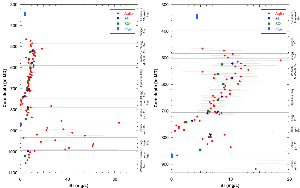
Fig. 5.2-3: Br with data at two different depth scales from squeezing, advective displacement, aqueous extraction and groundwater samples
