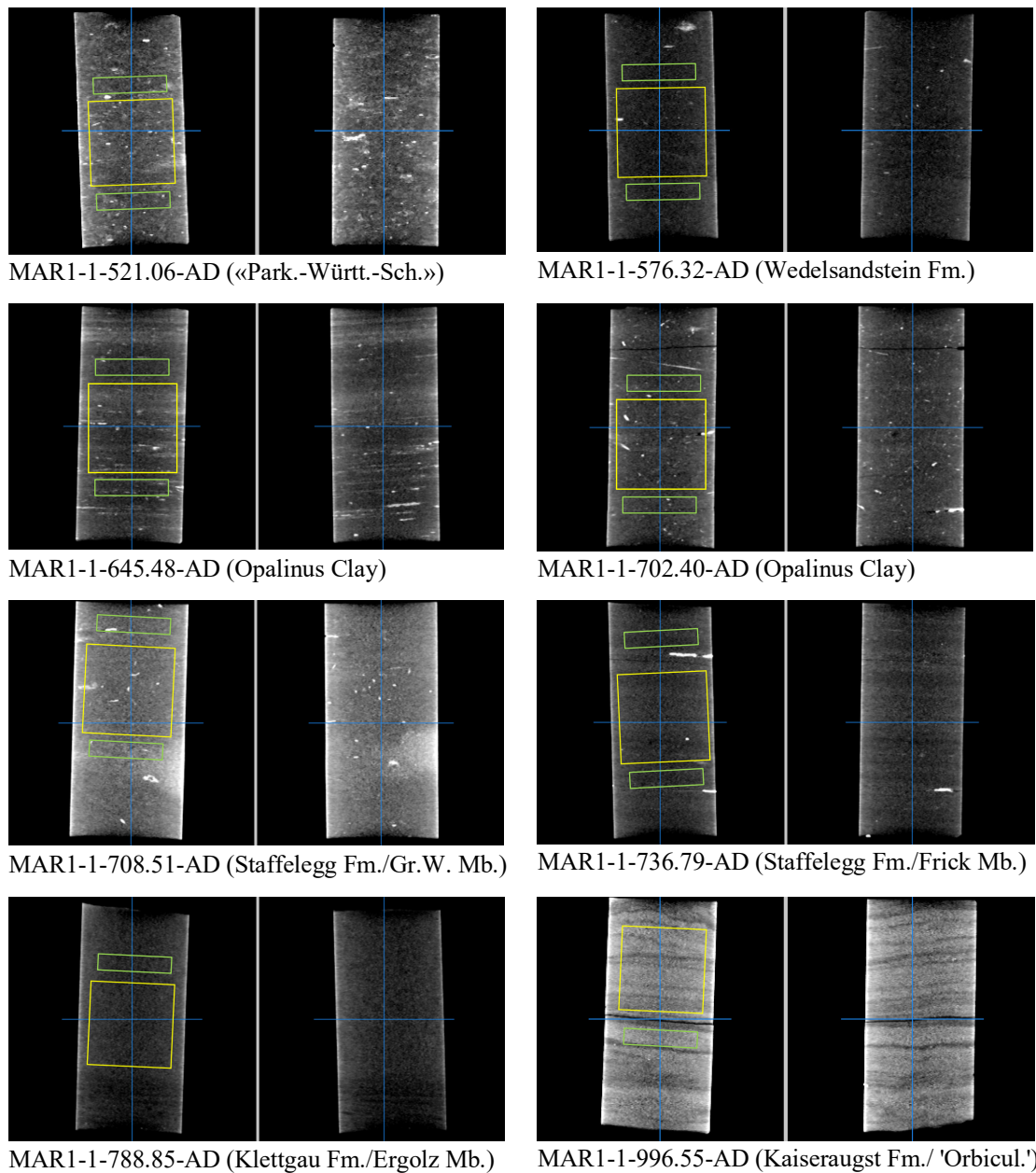
Fig. 4.7-2: X-ray CT images of AD samples
