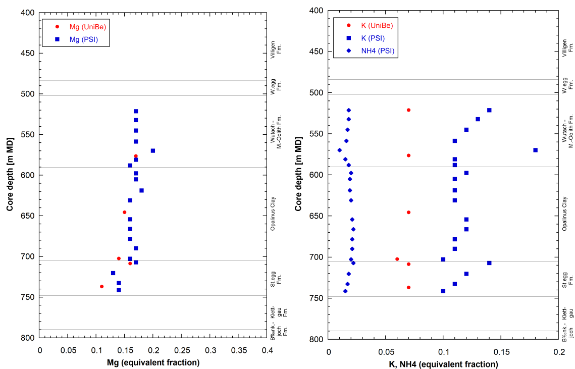
Fig. 5.7-7: Mg (left) and K, NH 4 (right) occupancies according to Uni Bern and PSI data
