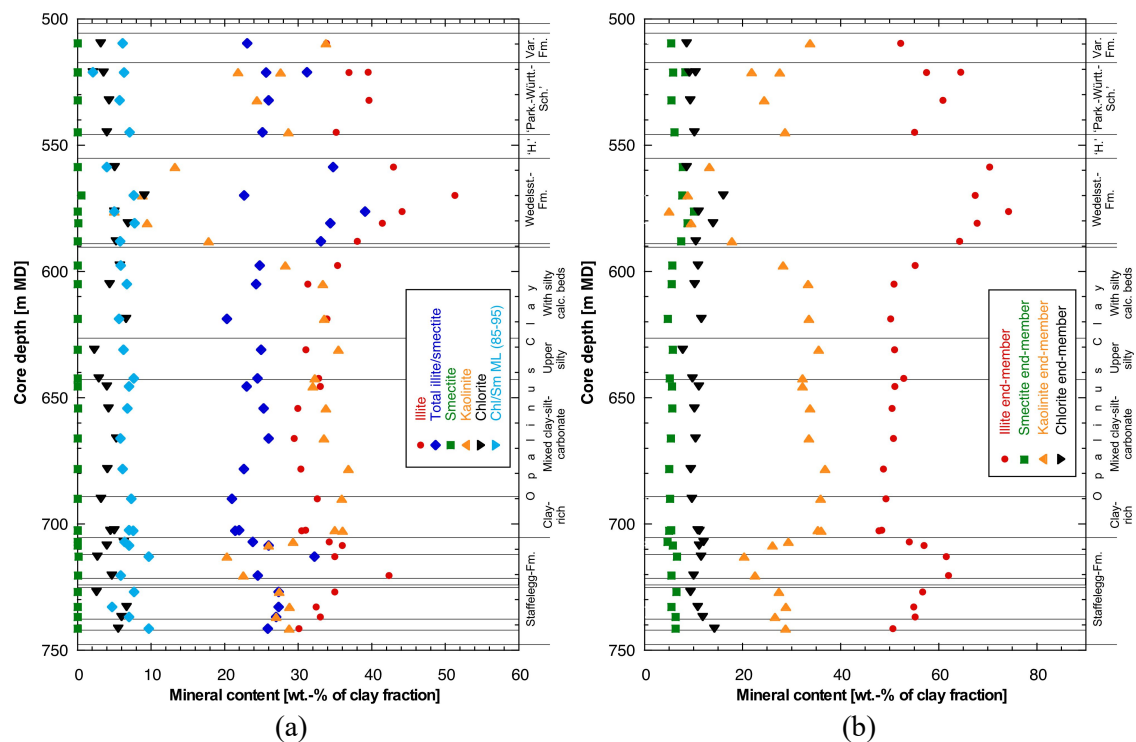
Fig. 4.2-6: Mineralogical composition of the clay fraction as a function of depth in the Lias – Dogger interval; (a) individual clay minerals, (b) end-member clays
