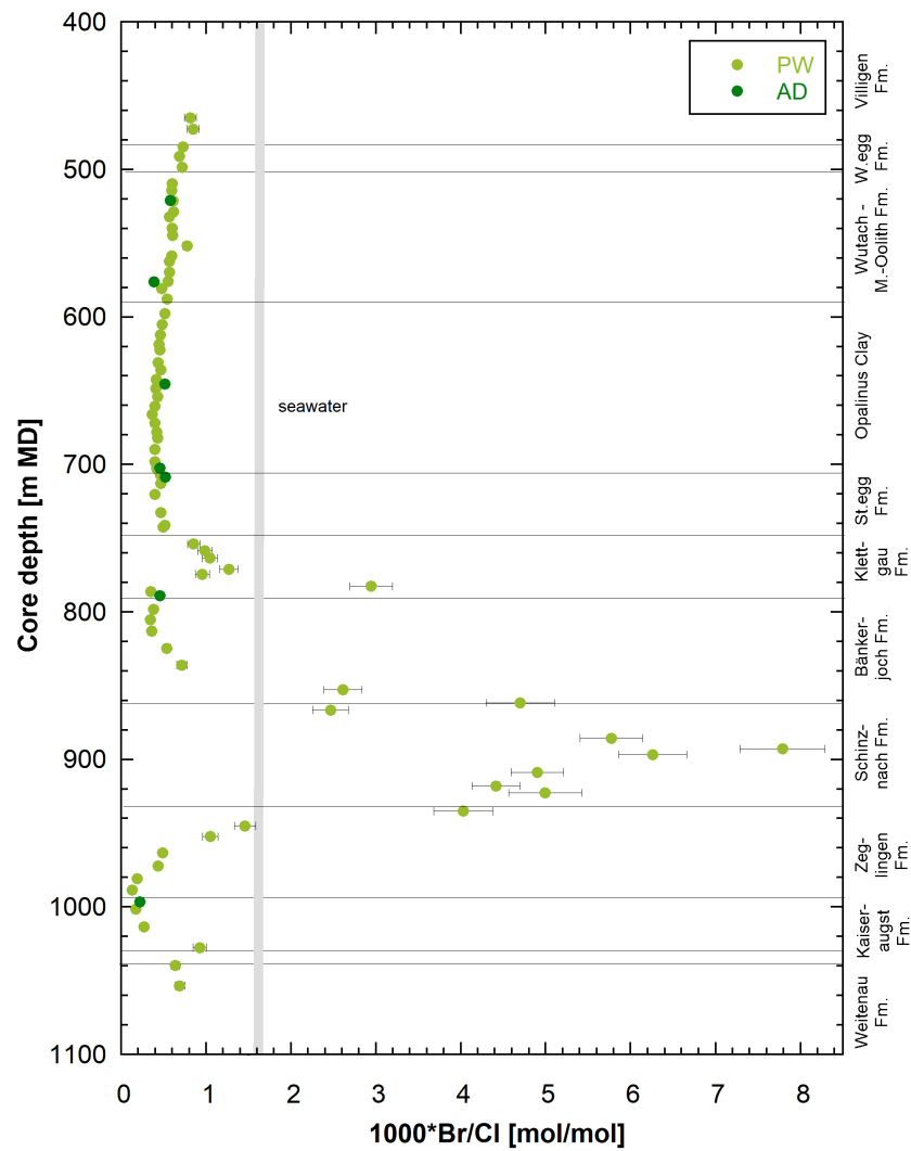
Fig. 4.4-2: Depth profile of the molar Br/Cl ratio in aqueous extracts at a S/L ratio of about 1
