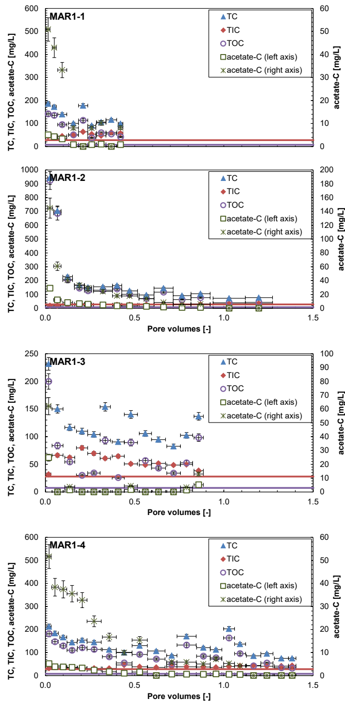
Fig. 4.7-12: Evolution of carbon system during advective displacement experiments
