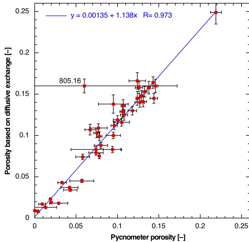
Fig. 4.3-8: Correlation of pycnometer porosity and porosity from isotope diffusive exchange Bars indicate propagated errors. Outlier 805.16 was excluded from the regression line.
