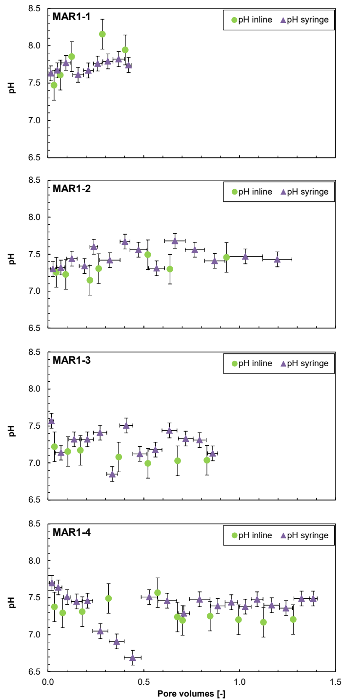
Fig. 4.7-14: Evolution of pH during advective displacement experiments
