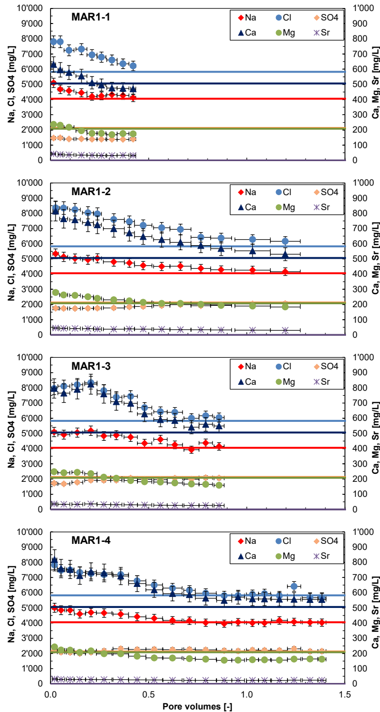
Fig. 4.7-8: Evolution of major components during advective displacement experiments
