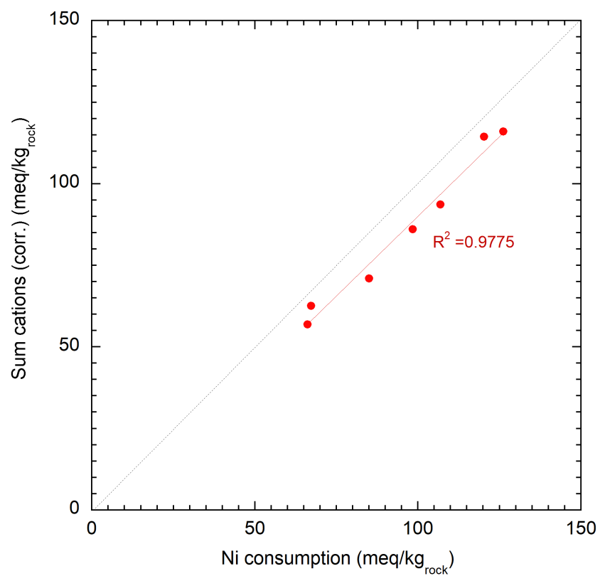
Fig. 5.7-1: Ni consumption vs. corrected sum of cations (data of Uni Bern)
