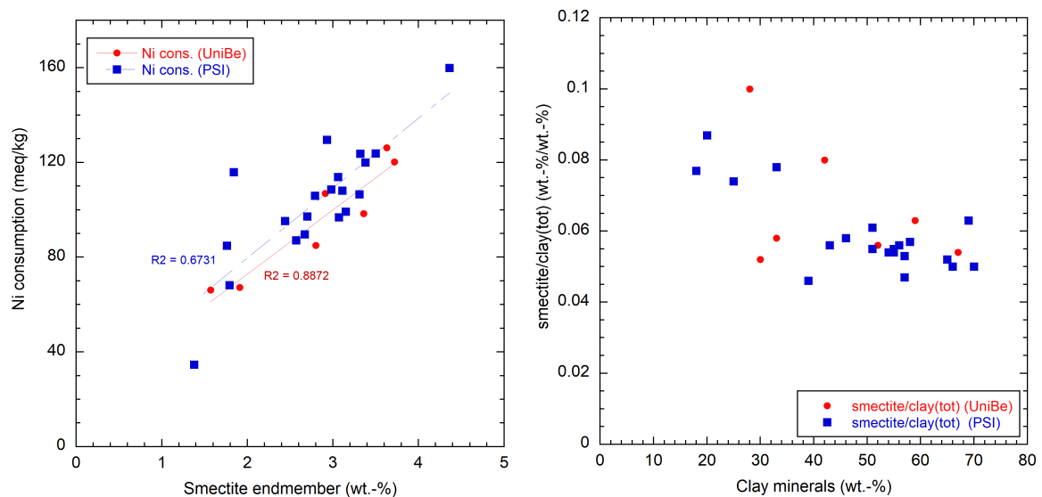
Fig. 5.7-5: Ni consumption as function of the smectite end-member (left) and smectite end-member/clay-mineral content ratio as a function of the clay-mineral content (right)
