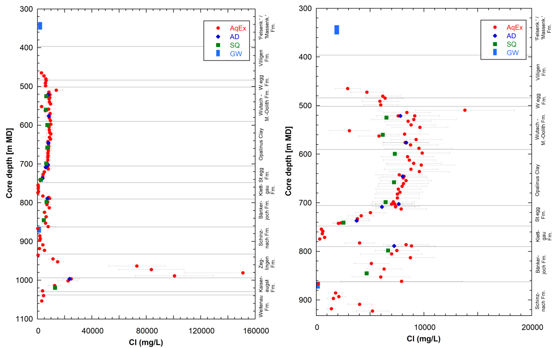
Fig. 5.2-1: Cl profiles at different depth scales with data from squeezing, advective displacement, aqueous extraction, and groundwater samples
