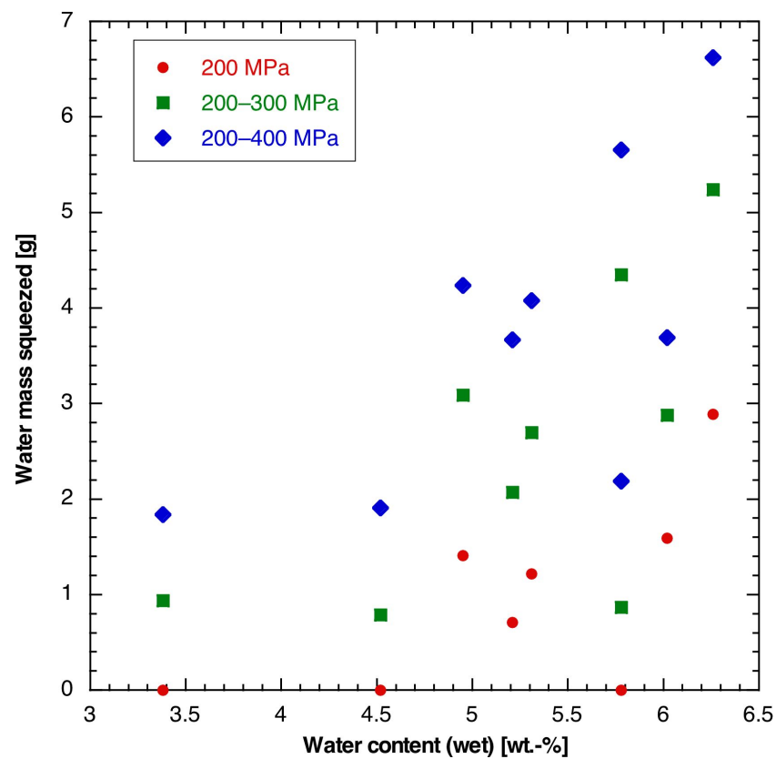
Fig. 4.6-2: Correlation of the original water content and the water mass obtained by squeezing
