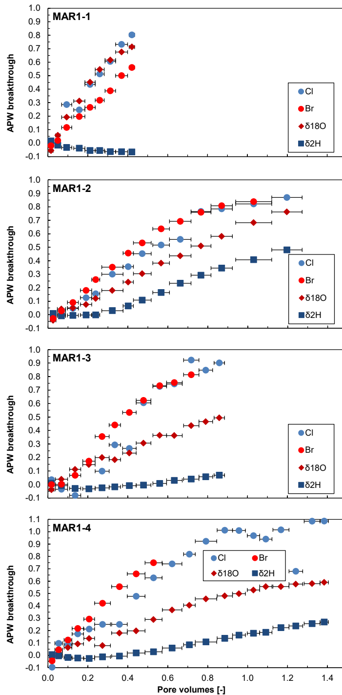
Fig. 4.7-17: Breakthrough of Cl, Br, \delta^2\text{H} and \delta^{18}\text{O} during advective displacement experiments
