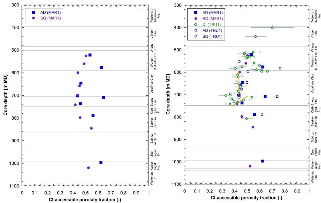
Fig. 5.1-3: CI-accessible porosity fraction ( f_{CI} ) as a function of depth; left: MAR1-1 data; right: MAR1-1 and TRU1-1 data
