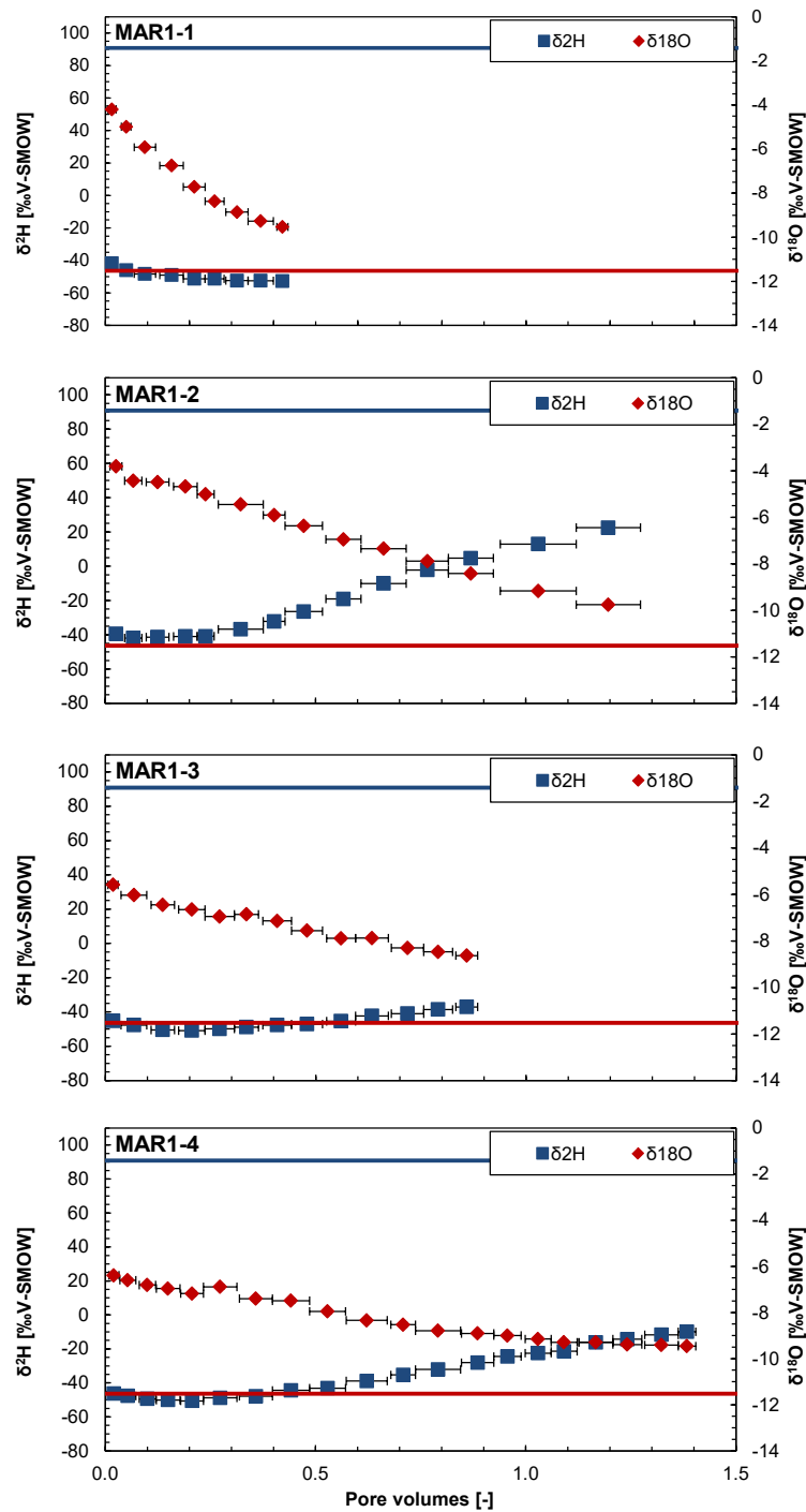
Fig. 4.7-15: Evolution of \delta^2\text{H} and \delta^{18}\text{O} during advective displacement experiments
