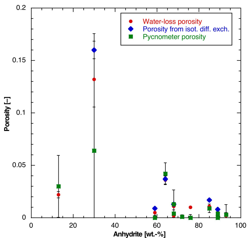
Fig. 4.3-13: Porosity of anhydrite-bearing samples
